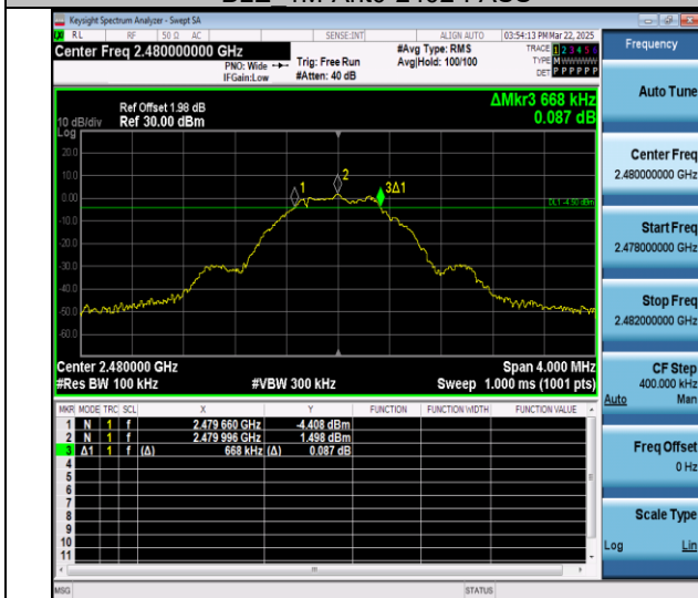
BLE_1M-Ant0-2480-PASS
