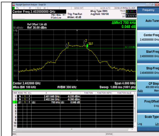
BLE_1M-Ant0-2402-PASS
