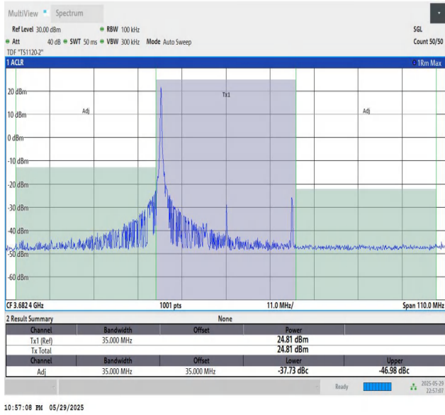
48-48-20MHz-15MHz-16QAM-16QAM-56491-56662-1RB#0-0R B#75-PASS
