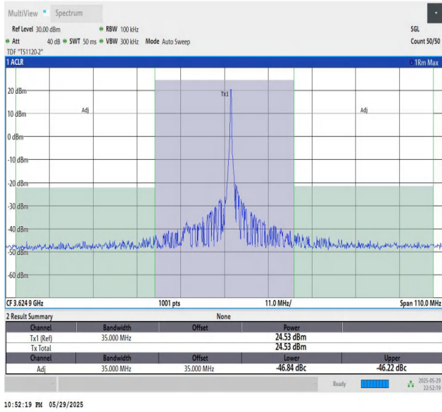
48-48-20MHz-15MHz-16QAM-16QAM-55916-56087-1RB#99-0 RB#0-PASS
