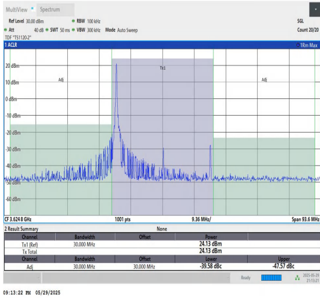
48-48-20MHz-10MHz-64QAM-64QAM-55941-56085-1RB#0-0R B#0-PASS
