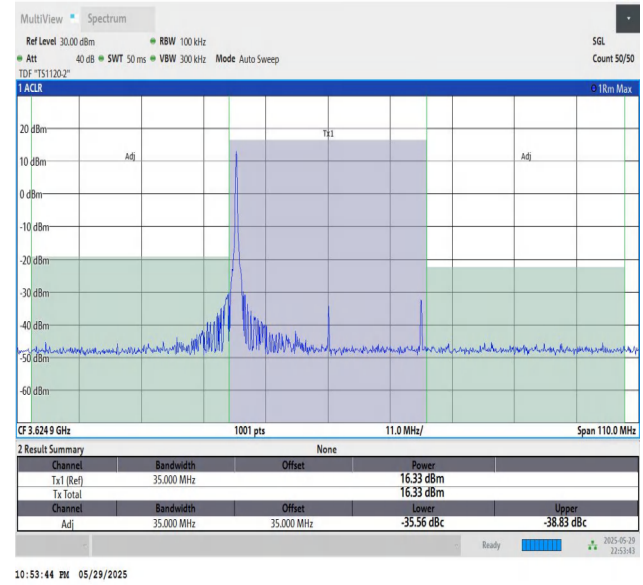
48-48-20MHz-15MHz-64QAM-64QAM-55916-56087-1RB#0-1RB#7 4-PASS
