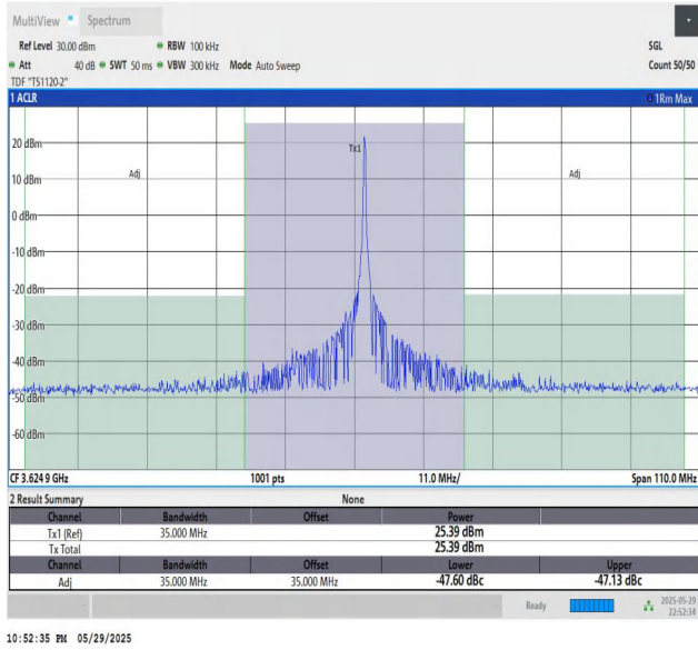
48-48-20MHz-15MHz-64QAM-64QAM-55916-56087-1RB#99-0 RB#0-PASS
