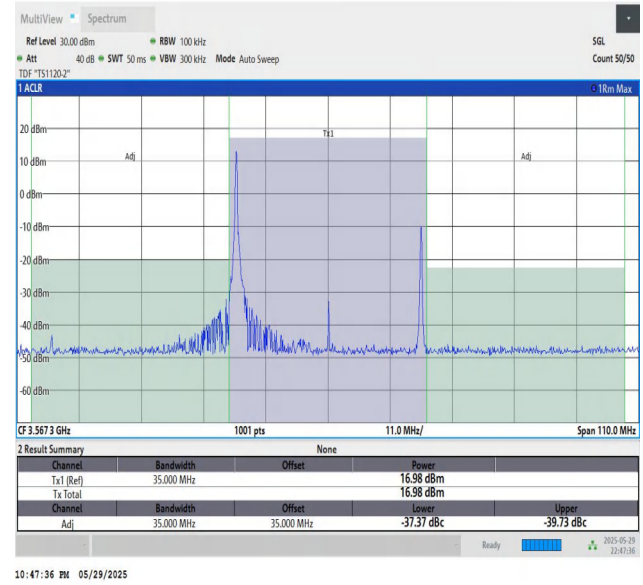
48-48-20MHz-15MHz-16QAM-16QAM-55340-55511-1RB#0-1RB#7 4-PASS
