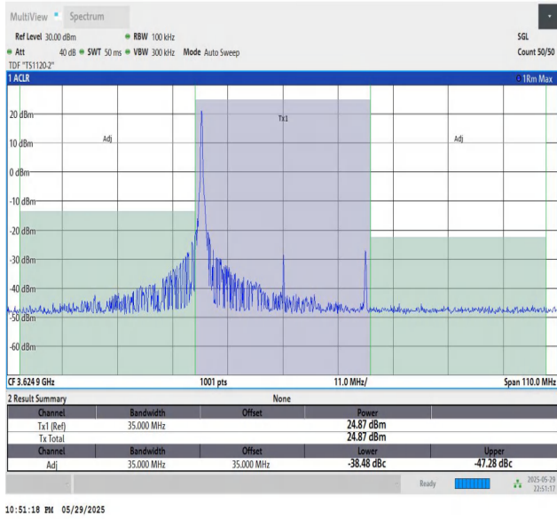
48-48-20MHz-15MHz-16QAM-16QAM-55916-56087-1RB#0-0R B#75-PASS
