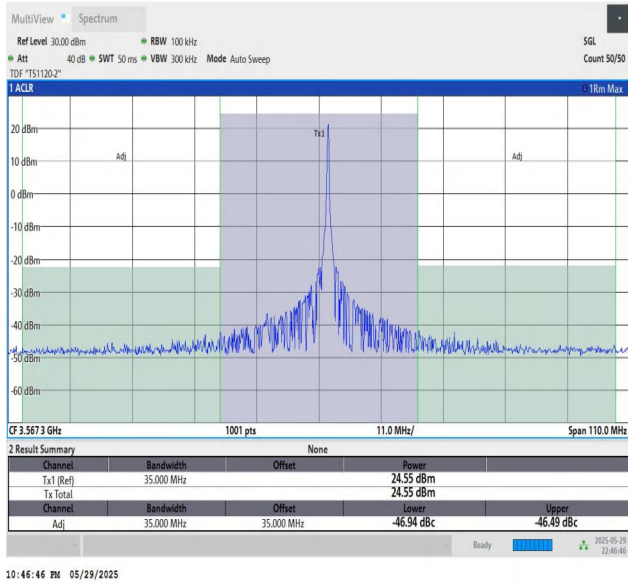
48-48-20MHz-15MHz-64QAM-64QAM-55340-55511-1RB#99-0 RB#0-PASS
