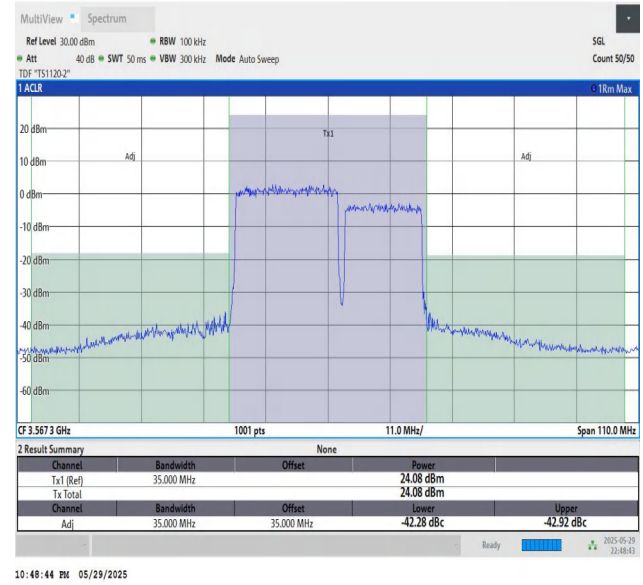
48-48-20MHz-15MHz-16QAM-16QAM-55340-55511-100RB#0-75R B#0-PASS
