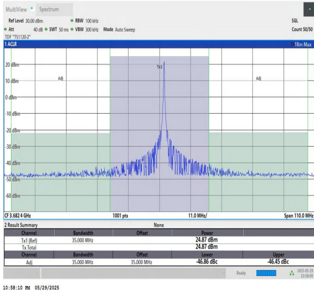
48-48-20MHz-15MHz-16QAM-16QAM-56491-56662-1RB#99-0 RB#0-PASS
