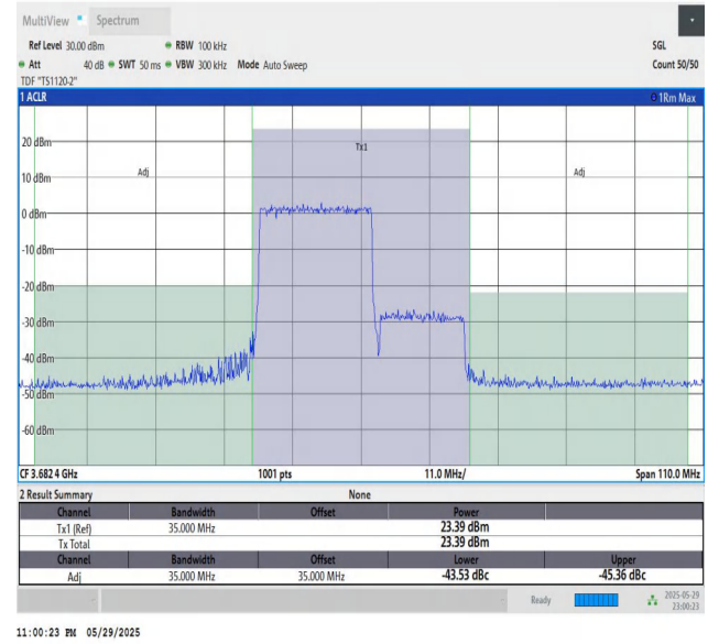
48-48-20MHz-15MHz-16QAM-16QAM-56491-56662-100RB#0-75R B#0-PASS
