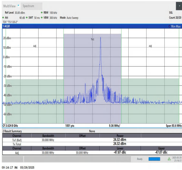
48-48-20MHz-10MHz-64QAM-64QAM-55941-56085-1RB#99-0 RB#0-PASS
