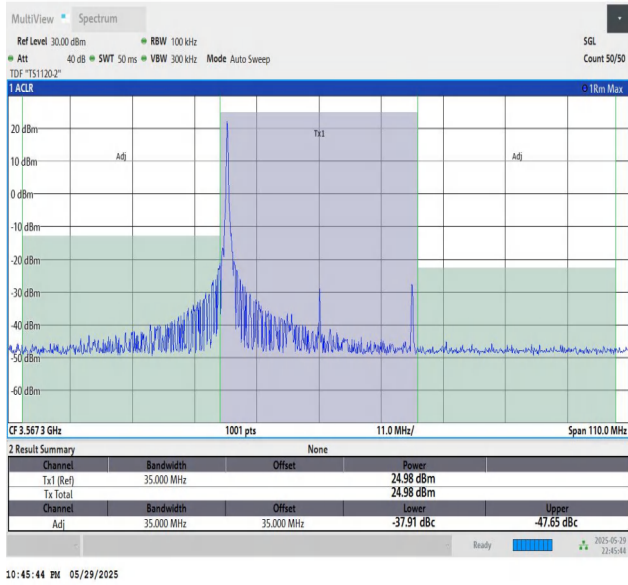
48-48-20MHz-15MHz-64QAM-64QAM-55340-55511-1RB#0-0R B#75-PASS
