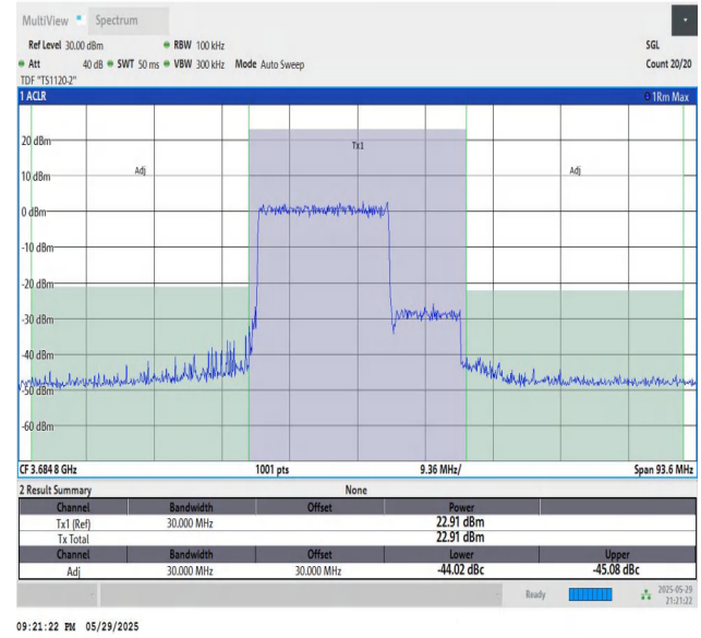
48-48-20MHz-10MHz-64QAM-64QAM-56541-56685-100RB#0-50R B#0-PASS
