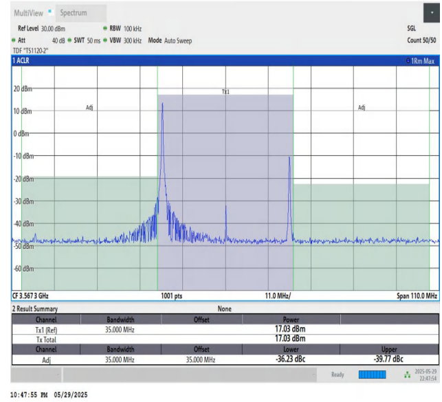
48-48-20MHz-15MHz-64QAM-64QAM-55340-55511-1RB#0-1RB#7 4-PASS
