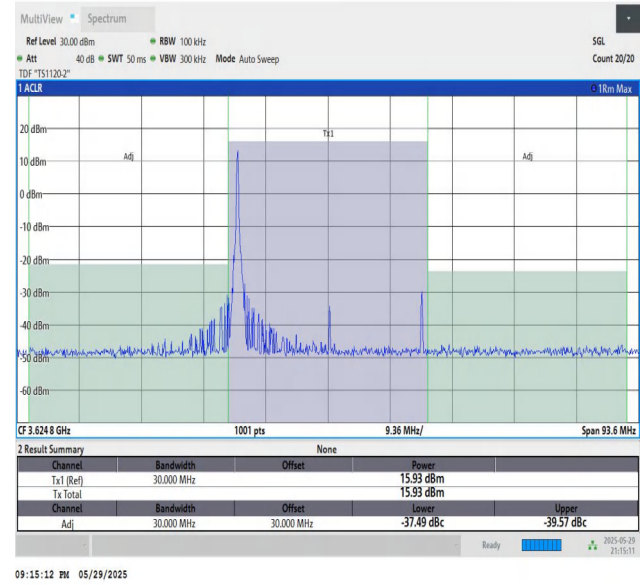
48-48-20MHz-10MHz-64QAM-64QAM-55941-56085-1RB#0-1RB#4 9-PASS
