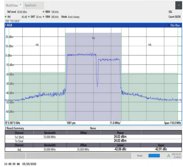
48-48-20MHz-15MHz-64QAM-64QAM-55340-55511-100RB#0-75R B#0-PASS
