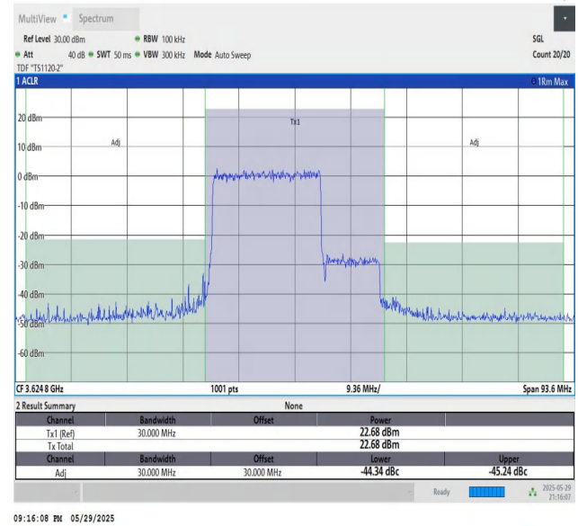
48-48-20MHz-10MHz-64QAM-64QAM-55941-56085-100RB#0-50R B#0-PASS
