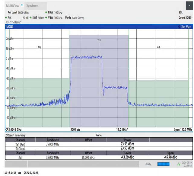
48-48-20MHz-15MHz-64QAM-64QAM-55916-56087-100RB#0-75R B#0-PASS
