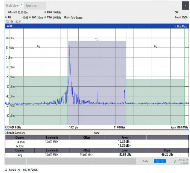
48-48-20MHz-15MHz-16QAM-16QAM-55916-56087-1RB#0-1RB#7 4-PASS
