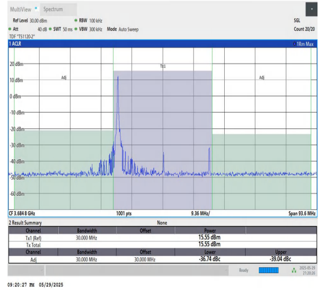
48-48-20MHz-10MHz-64QAM-64QAM-56541-56685-1RB#0-1RB#4 9-PASS
