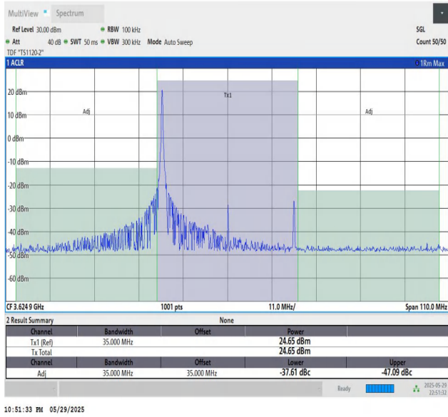
48-48-20MHz-15MHz-64QAM-64QAM-55916-56087-1RB#0-0R B#75-PASS
