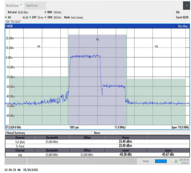
48-48-20MHz-15MHz-16QAM-16QAM-55916-56087-100RB#0-75R B#0-PASS
