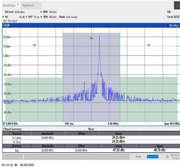
48-48-20MHz-10MHz-64QAM-64QAM-56541-56685-1RB#99-0 RB#0-PASS
