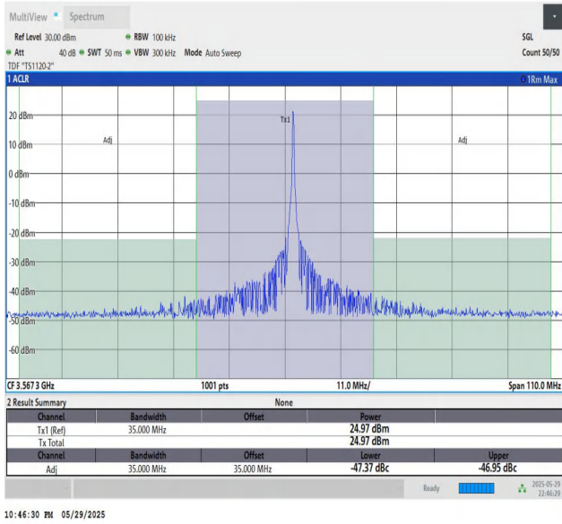
48-48-20MHz-15MHz-16QAM-16QAM-55340-55511-1RB#99-0 RB#0-PASS
