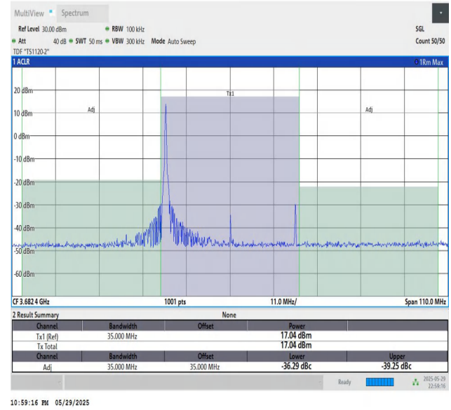
48-48-20MHz-15MHz-16QAM-16QAM-56491-56662-1RB#0-1RB#7 4-PASS
