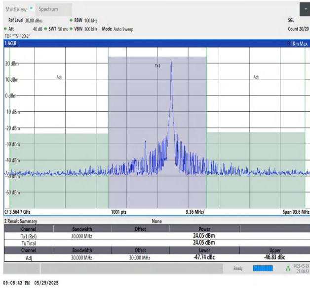
48-48-20MHz-10MHz-16QAM-16QAM-55340-55484-1RB#99-0 RB#0-PASS
