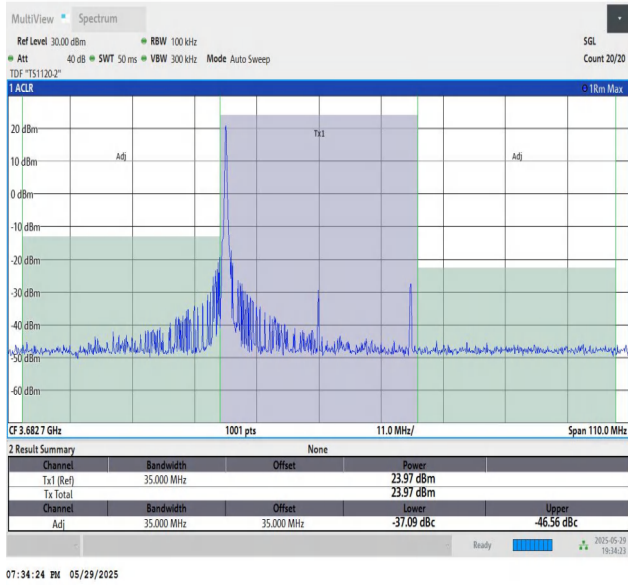
48-48-15MHz-20MHz-64QAM-64QAM-56469-56640-1RB#0-0R B#0-PASS
