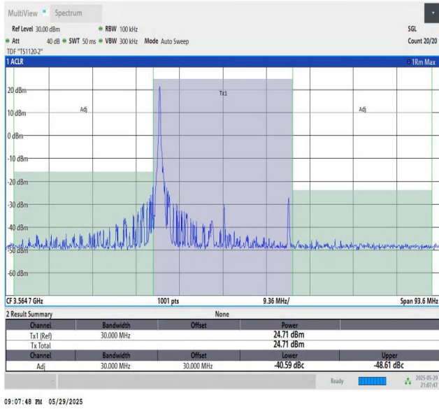
48-48-20MHz-10MHz-16QAM-16QAM-55340-55484-1RB#0-0R B#0-PASS
