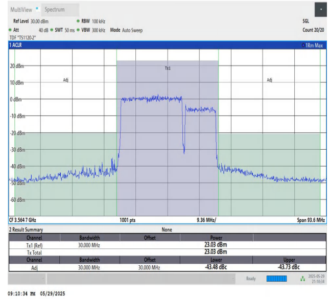
48-48-20MHz-10MHz-16QAM-16QAM-55340-55484-100RB#0-50R B#0-PASS
