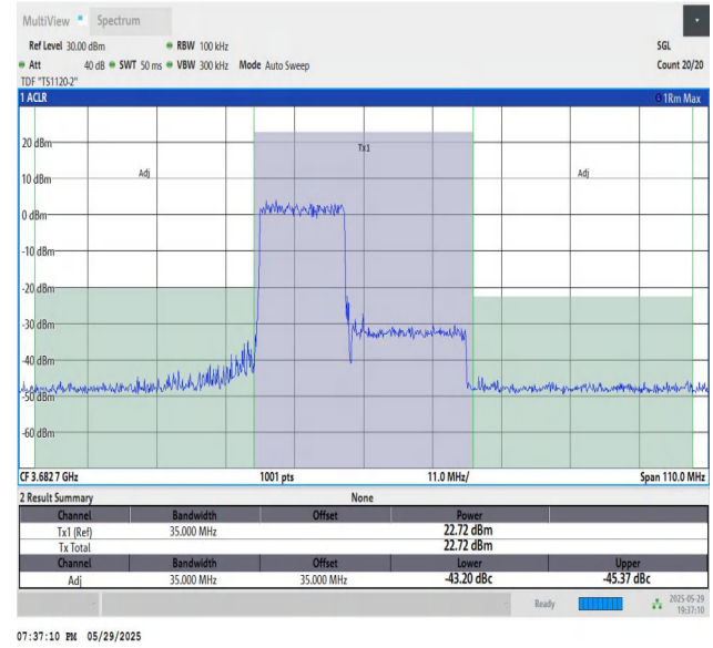
48-48-15MHz-20MHz-64QAM-64QAM-56469-56640-75RB#0-100R B#0-PASS
