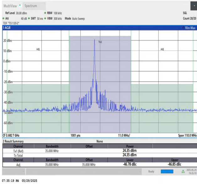
48-48-15MHz-20MHz-64QAM-64QAM-56469-56640-1RB#74-0 RB#0-PASS
