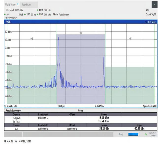
48-48-20MHz-10MHz-16QAM-16QAM-55340-55484-1RB#0-1RB#4 9-PASS
