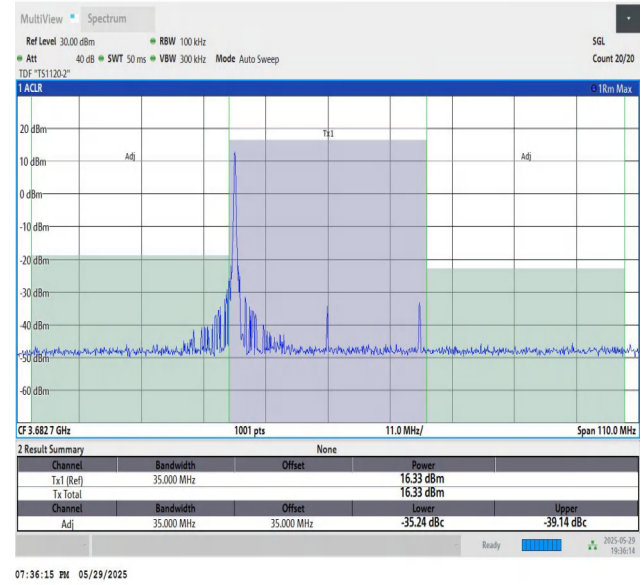
48-48-15MHz-20MHz-64QAM-64QAM-56469-56640-1RB#9 9-PASS
