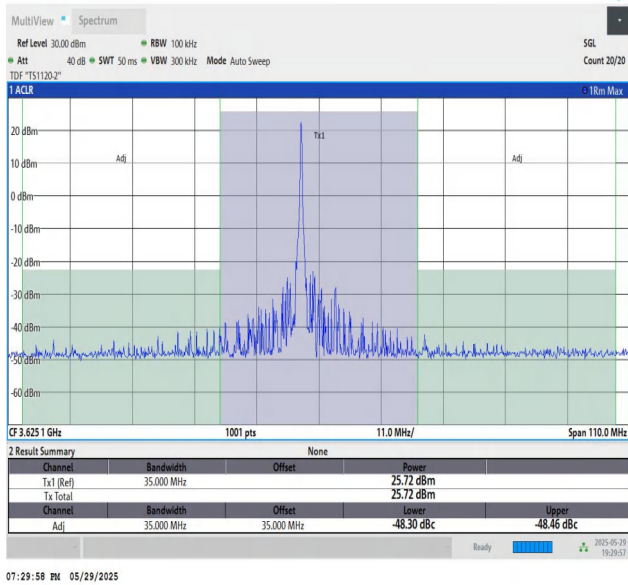
48-48-15MHz-20MHz-64QAM-64QAM-55893-56064-1RB#74-0 RB#0-PASS
