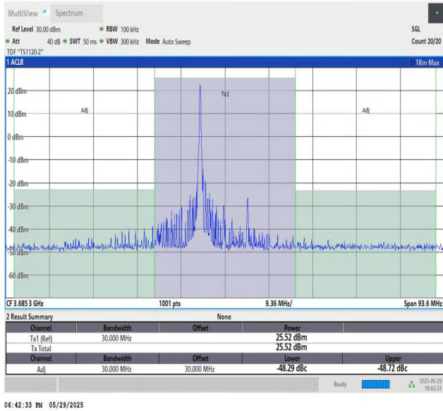
48-48-10MHz-20MHz-64QAM-64QAM-56496-56640-1RB#49-0 RB#0-PASS
