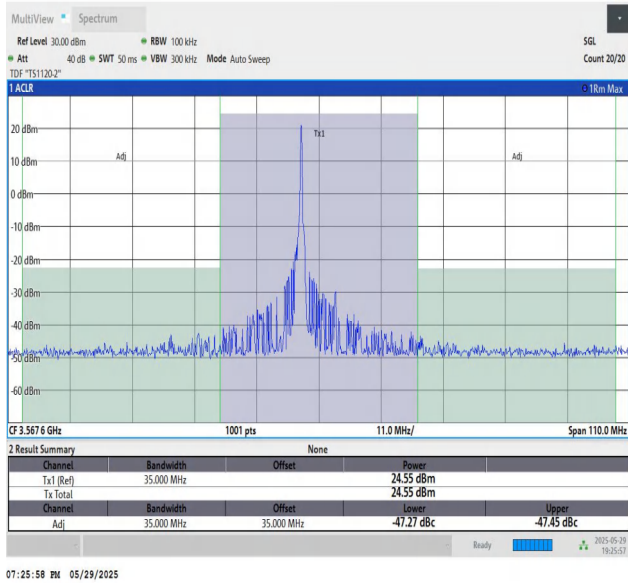
48-48-15MHz-20MHz-16QAM-16QAM-55318-55489-1RB#74-0 RB#0-PASS
