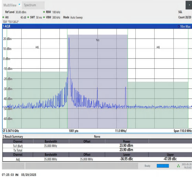
48-48-15MHz-20MHz-16QAM-16QAM-55318-55489-1RB#0-0R B#0-PASS
