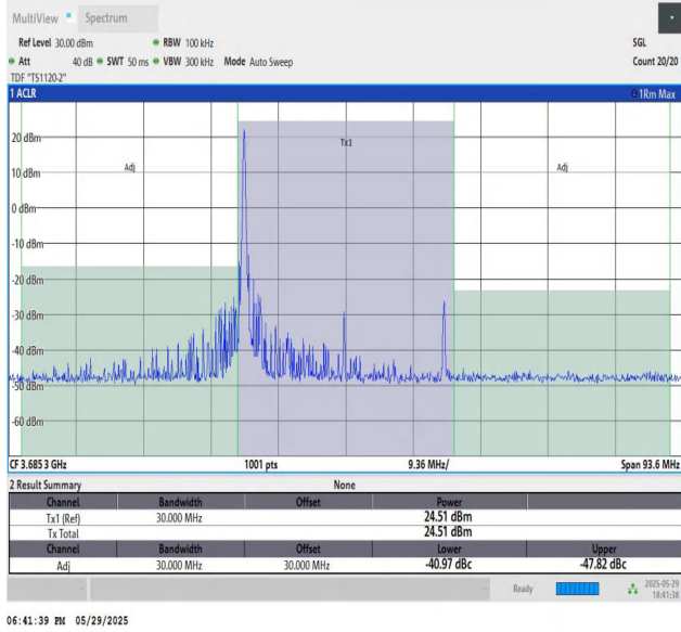
48-48-10MHz-20MHz-64QAM-64QAM-56496-56640-1RB#0-0R B#0-PASS
