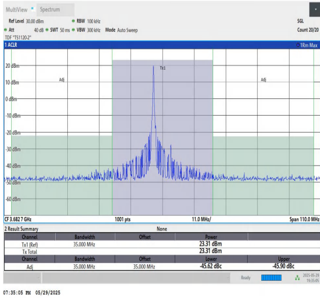
48-48-15MHz-20MHz-16QAM-16QAM-56469-56640-1RB#74-0 RB#0-PASS
