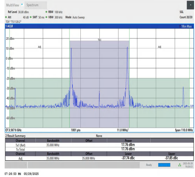
48-48-15MHz-20MHz-16QAM-16QAM-55318-55489-1RB#0-1RB#9 9-PASS
