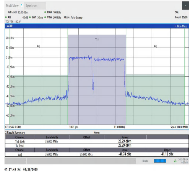
48-48-15MHz-20MHz-16QAM-16QAM-55318-55489-75RB#0-100R B#0-PASS
