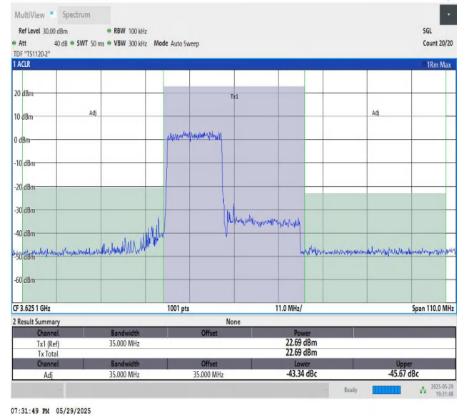
48-48-15MHz-20MHz-64QAM-64QAM-55893-56064-75RB#0-100R B#0-PASS
