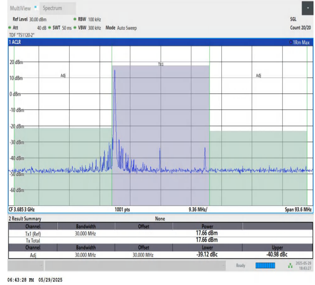
48-48-10MHz-20MHz-64QAM-64QAM-56496-56640-1RB#0-1RB#9 9-PASS
