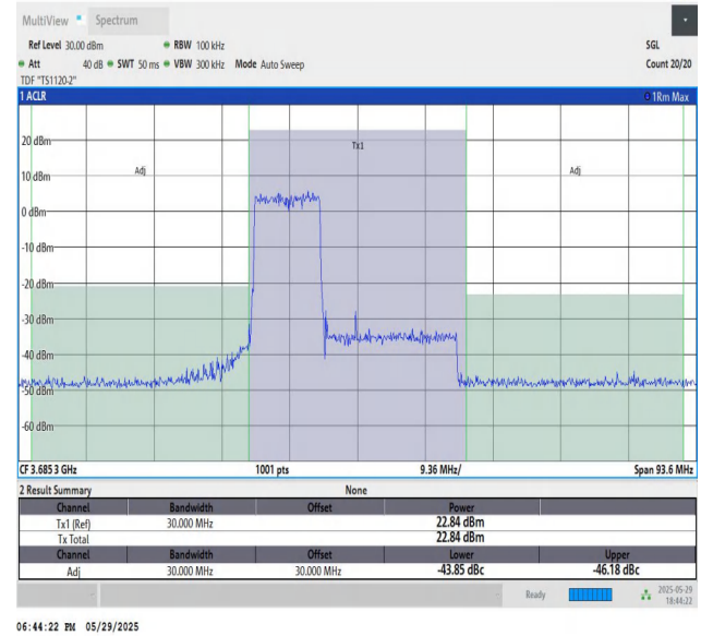
48-48-10MHz-20MHz-64QAM-64QAM-56496-56640-50RB#0-100R B#0-PASS
