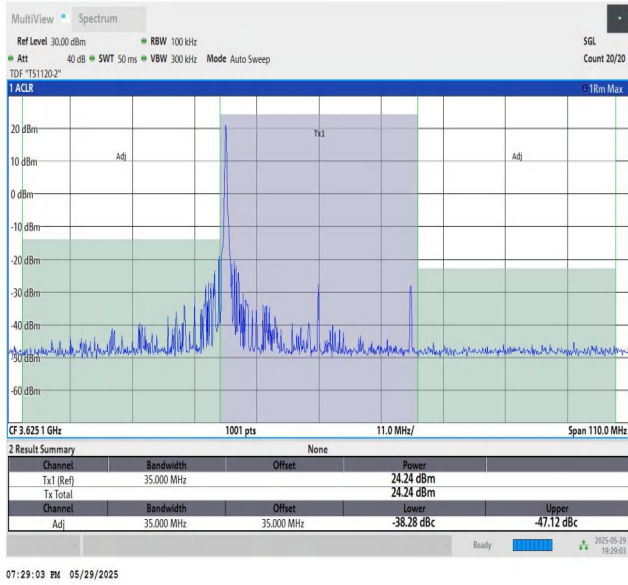
48-48-15MHz-20MHz-64QAM-64QAM-55893-56064-1RB#0-0R B#0-PASS
