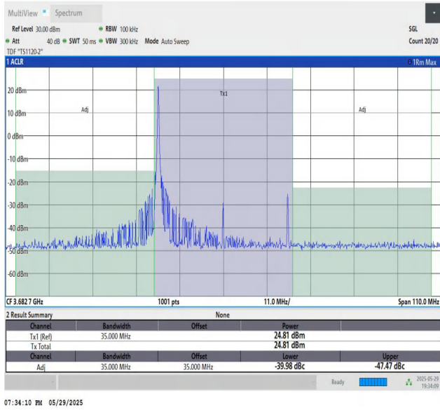
48-48-15MHz-20MHz-16QAM-16QAM-56469-56640-1RB#0-0R B#0-PASS
