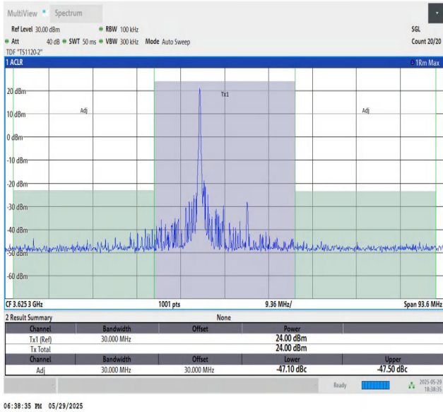
48-48-10MHz-20MHz-16QAM-16QAM-55896-56040-1RB#49-0 RB#0-PASS
