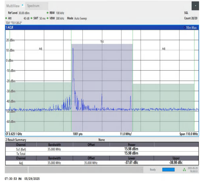
48-48-15MHz-20MHz-64QAM-64QAM-55893-56064-1RB#0-1RB#9 9-PASS
