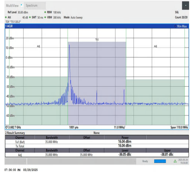
48-48-15MHz-20MHz-16QAM-16QAM-56469-56640-1RB#9 9-PASS
