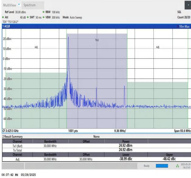
48-48-10MHz-20MHz-16QAM-16QAM-55896-56040-1RB#0-0R B#0-PASS
