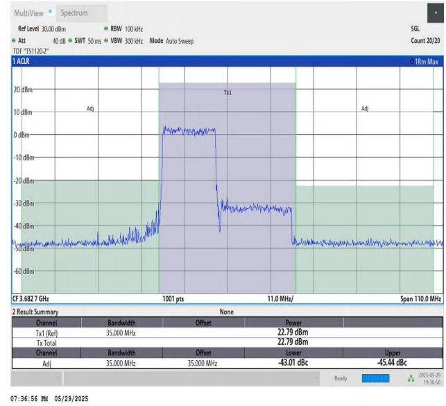
48-48-15MHz-20MHz-16QAM-16QAM-56469-56640-75RB#0-100R B#0-PASS
