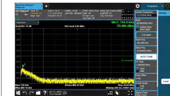
48-48-20MHz-20MHz-QPSK-QPSK-55340-55538-1RB#0-1RB#9-9-0.15~30MHz-PASS
