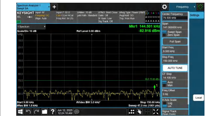
48-48-20MHz-15MHz-QPSK-QPSK-55340-55511-1RB#99-0RB#0 -0.009~0.15MHz-PASS
