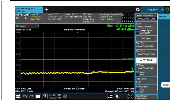
48-48-20MHz-20MHz-QPSK-QPSK-55340-55538-1RB#0-1RB#9 9-6000~18000MHz-PASS
