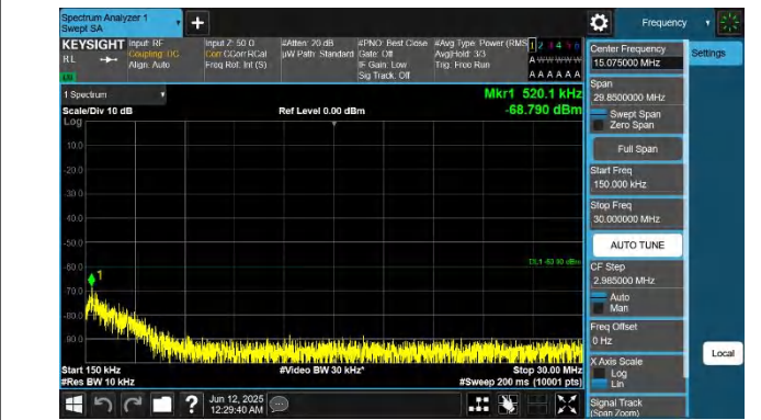
48-48-20MHz-15MHz-QPSK-QPSK-56491-56662-1RB#0-1RB#7 4-0.15~30MHz-PASS
