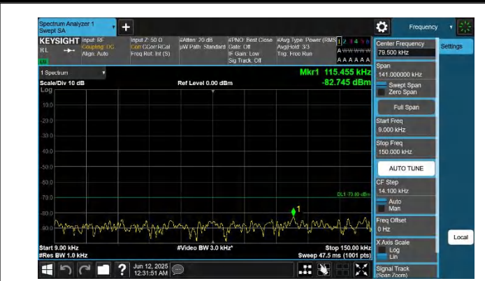
48-48-20MHz-20MHz-QPSK-QPSK-55340-55538-1RB#0-1RB#9-9-0.009~0.15MHz-PASS
