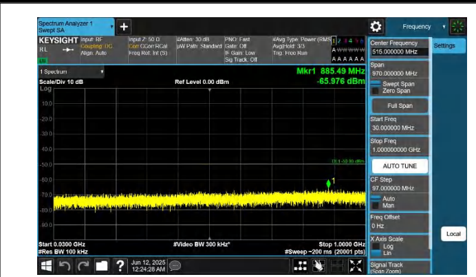
48-48-20MHz-15MHz-QPSK-QPSK-55340-55511-1RB#99-ORB#0 -30~1000MHz-PASS
