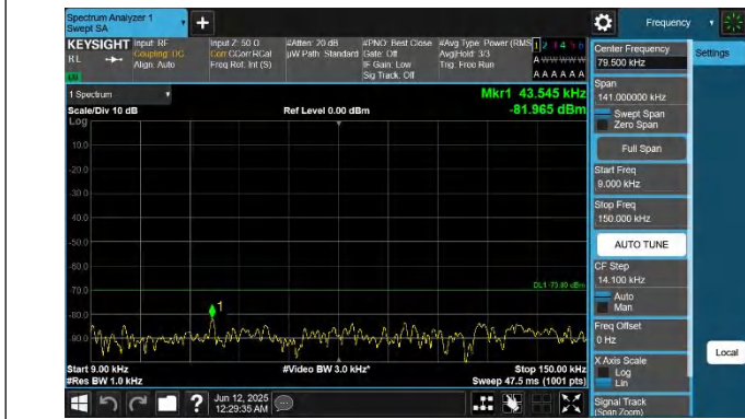
48-48-20MHz-15MHz-QPSK-QPSK-56491-56662-1RB#0-1RB#7 4-0.009~0.15MHz-PASS
