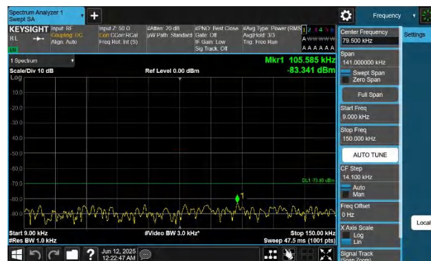
48-48-20MHz-10MHz-QPSK-QPSK-56541-56685-1RB#0-1RB#4 9-0.009~0.15MHz-PASS
