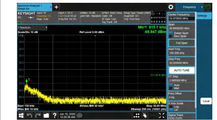
48-48-20MHz-10MHz-QPSK-QPSK-55941-56085-1RB#0-1RB#4 9-0.15~30MHz-PASS
