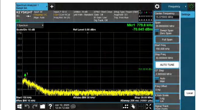
48-48-20MHz-20MHz-QPSK-QPSK-55891-56089-1RB#0-1RB#9 9-0.15~30MHz-PASS
