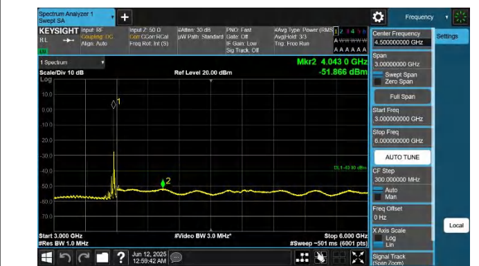
48-48-20MHz-15MHz-QPSK-QPSK-55340-55511-1RB#99-ORB#0 -3000~6000MHz-PASS
