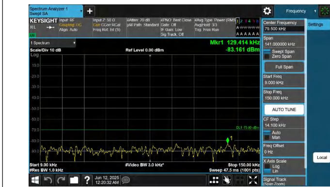
48-48-20MHz-10MHz-QPSK-QPSK-55941-56085-1RB#0-1RB#4 9-0.009~0.15MHz-PASS
