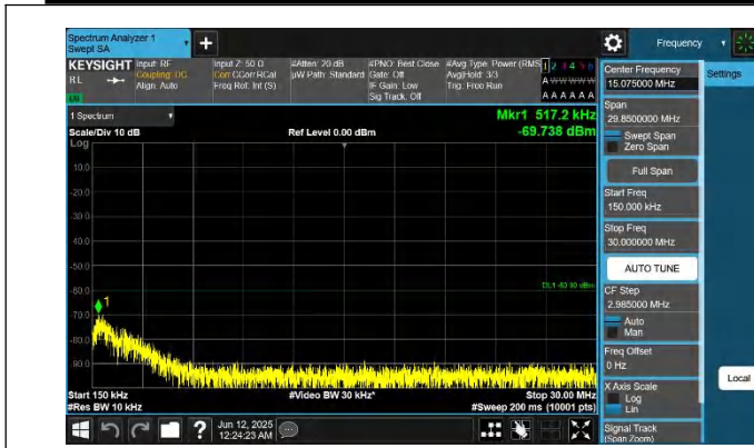
48-48-20MHz-15MHz-QPSK-QPSK-55340-55511-1RB#99-ORB#0 -0.15~30MHz-PASS
