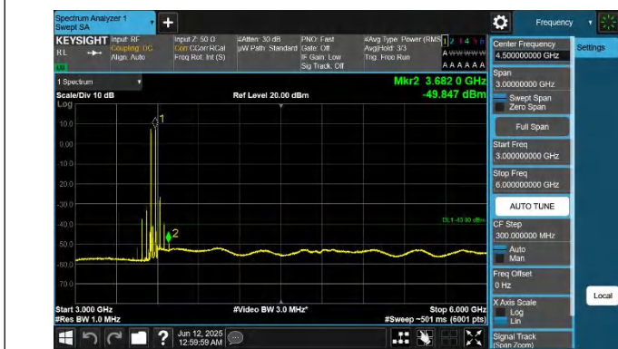
48-48-20MHz-15MHz-QPSK-QPSK-55340-55511-1RB#0-1RB#74 -3000~6000MHz-PASS
