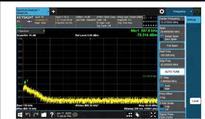
48-48-10MHz-20MHz-QPSK-QPSK-55896-56040-1RB#0-0RB#0- 0.15~30MHz-PASS
