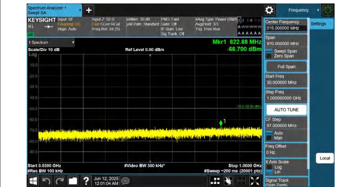
48-48-10MHz-20MHz-QPSK-QPSK-56496-56640-1RB#0-0RB#0- 30~1000MHz-PASS
