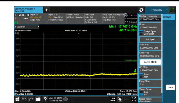
48-48-10MHz-20MHz-QPSK-QPSK-55896-56040-1RB#49-0RB# 0-6000~18000MHz-PASS
