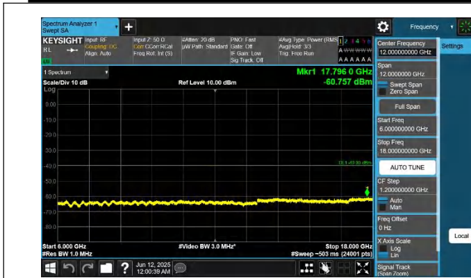
48-48-10MHz-20MHz-QPSK-QPSK-55896-56040-1RB#0-1RB#9 9-6000~18000MHz-PASS
