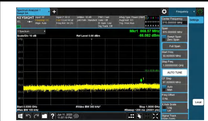
48-48-10MHz-20MHz-QPSK-QPSK-55295-55439-1RB#49-0RB# 0-30~1000MHz-PASS
