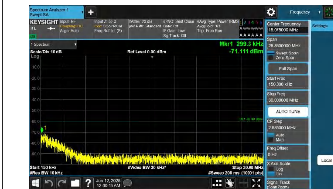
48-48-10MHz-20MHz-QPSK-QPSK-55896-56040-1RB#0-1RB#9-9.0.15~30MHz-PASS
