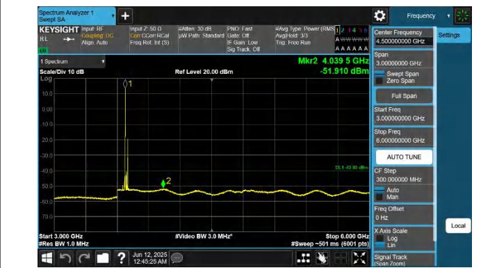
48-48-5MHz-20MHz-QPSK-QPSK-56523-56640-1RB#0-1RB#99- 3000~6000MHz-PASS
