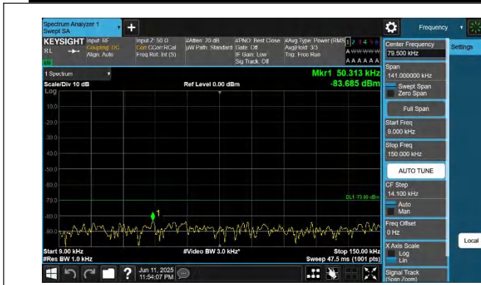
48-48-5MHz-20MHz-QPSK-QPSK-56523-56640-1RB#0-0RB#0-0 .009~0.15MHz-PASS
