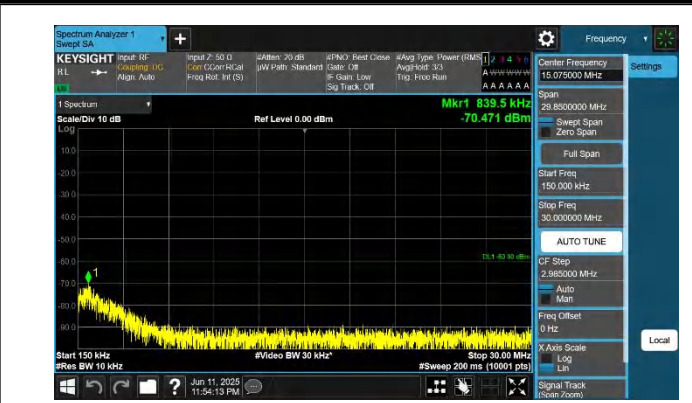
48-48-5MHz-20MHz-QPSK-QPSK-56523-56640-1RB#0-0RB#0-0 .15~30MHz-PASS
