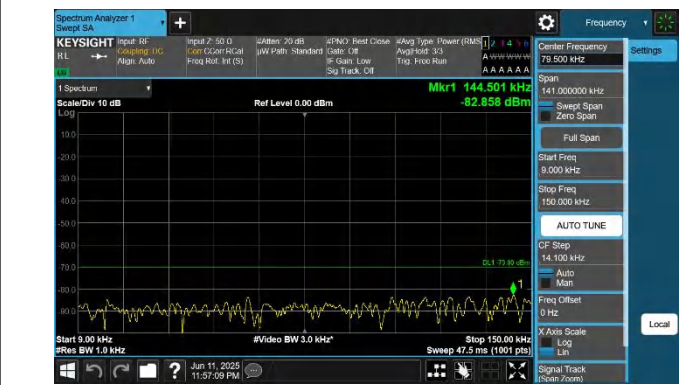
48-48-10MHz-20MHz-QPSK-QPSK-55295-55439-1RB#49-0RB# 0-0.009~0.15MHz-PASS
