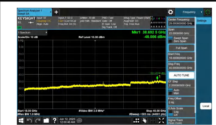
48-48-10MHz-20MHz-QPSK-QPSK-55896-56040-1RB#0-1RB#9 9-18000~40000MHz-PASS
