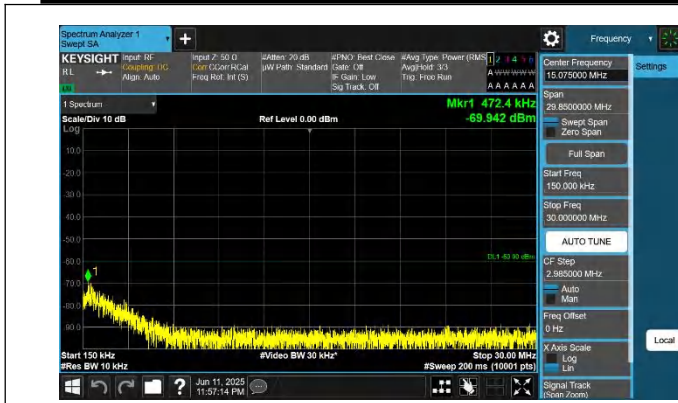
48-48-10MHz-20MHz-QPSK-QPSK-55295-55439-1RB#49-0RB# 0-0.15~30MHz-PASS
