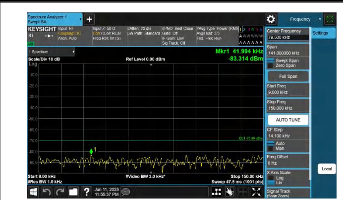
48-48-5MHz-20MHz-QPSK-QPSK-56523-56640-1RB#0-1RB#99- 0.009~0.15MHz-PASS
