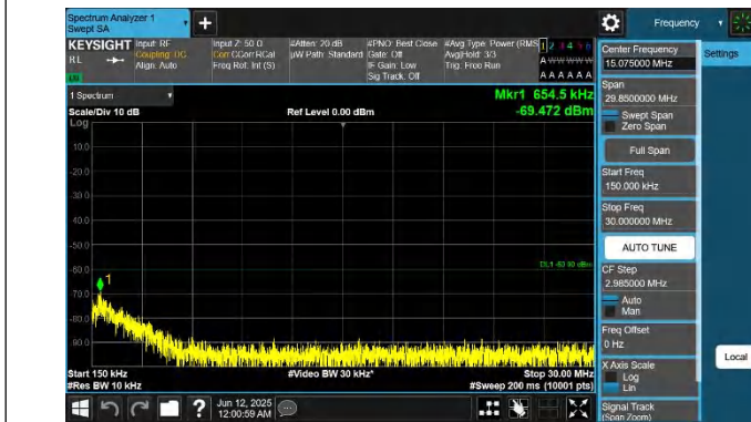
48-48-10MHz-20MHz-QPSK-QPSK-56496-56640-1RB#0-0RB#0- 0.15~30MHz-PASS
