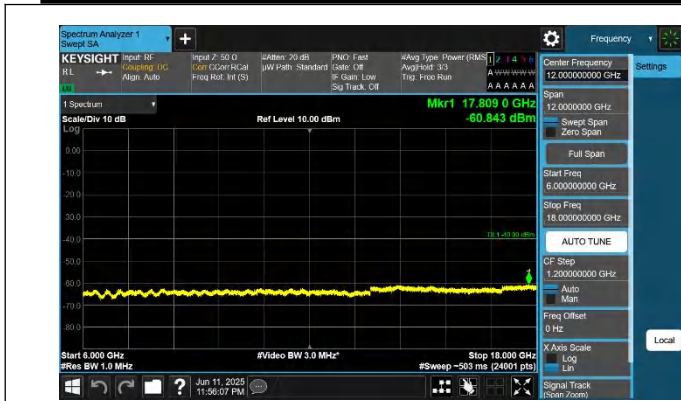
48-48-5MHz-20MHz-QPSK-QPSK-56523-56640-1RB#0-1RB#99- 6000~18000MHz-PASS
