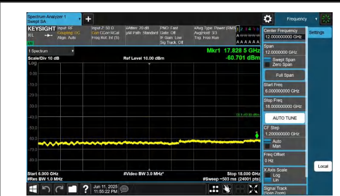
48-48-5MHz-20MHz-QPSK-QPSK-56523-56640-1RB#24-0RB#0- 6000~18000MHz-PASS
