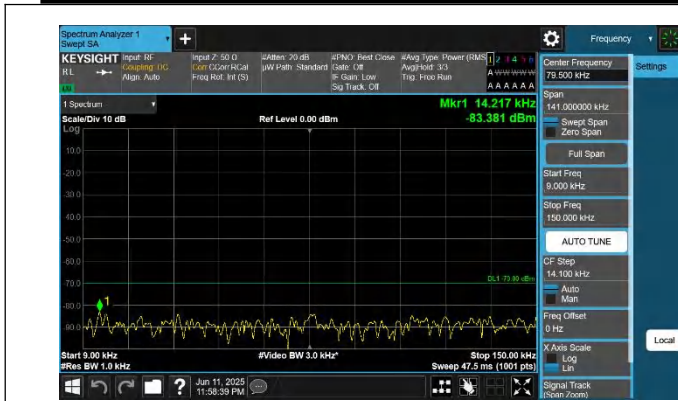
48-48-10MHz-20MHz-QPSK-QPSK-55896-56040-1RB#0-0RB#0- 0.009~0.15MHz-PASS
