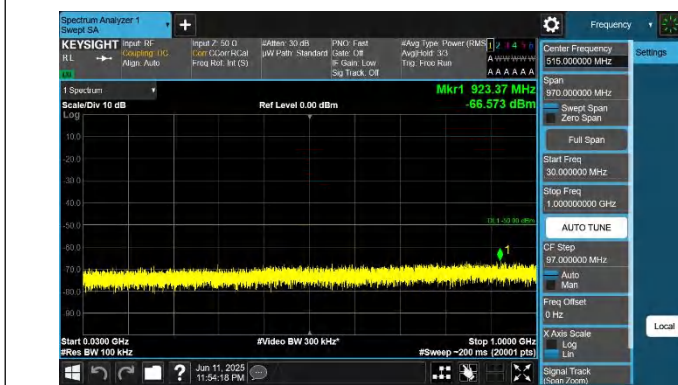
48-48-5MHz-20MHz-QPSK-QPSK-56523-56640-1RB#0-0RB#0-3 0~1000MHz-PASS
