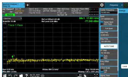
NTNV-n48-PC3-30-10-L-CP-QPSK-Inner_1RB_Left-0.009-0.15-PASS
