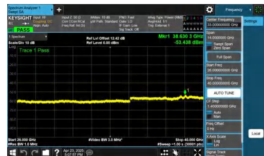
NTNV-n48-PC3-30-20-H-CP-QPSK-Inner_1RB_Right-26000-40000 -PASS
