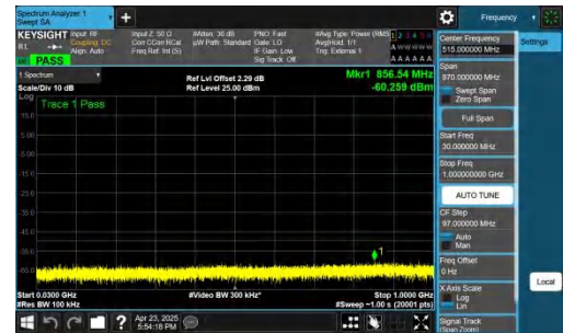
NTNV-n48-PC3-30-10-M-CP-QPSK-Inner_1RB_Right-30-1000-PA SS
