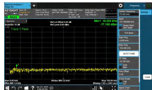
NTNV-n48-PC3-30-40-L-CP-QPSK-Inner_1RB_Right-0.009-0.15-P
