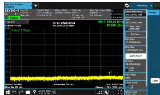
NTNV-n48-PC3-30-20-M-CP-QPSK-Inner_1RB_Right-30-1000-PA SS
