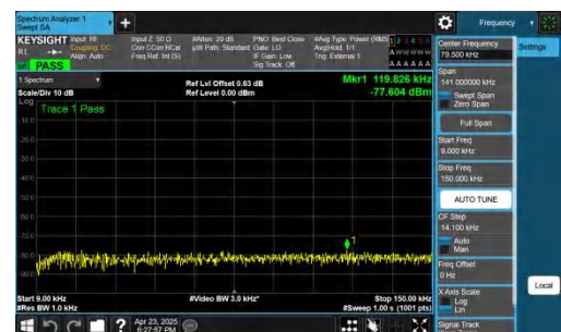
NTNV-n48-PC3-30-20-H-CP-QPSK-Inner_1RB_Right-0.009-0.15-P ASS
