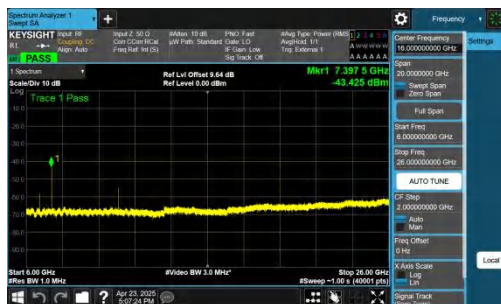
NTNV-n48-PC3-30-20-H-CP-QPSK-Inner_1RB_Right-6000-26000 -PASS
