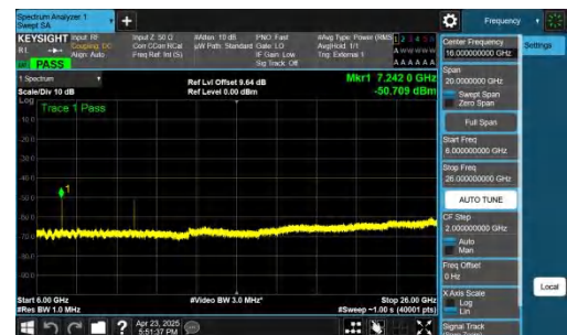
NTNV-n48-PC3-30-10-M-CP-QPSK-Inner_1RB_Left-6000-26000-P ASS
