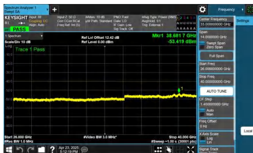
NTNV-n48-PC3-30-40-L-CP-QPSK-Inner_1RB_Left-26000-40000-PASS
