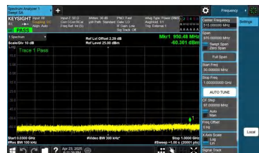
NTNV-n48-PC3-30-20-L-CP-QPSK-Inner_1RB_Right-30-1000-PAS S
