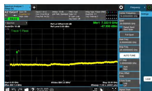
NTNV-n48-PC3-30-40-H-CP-QPSK-Inner_1RB_Left-6000-26000-PASS
