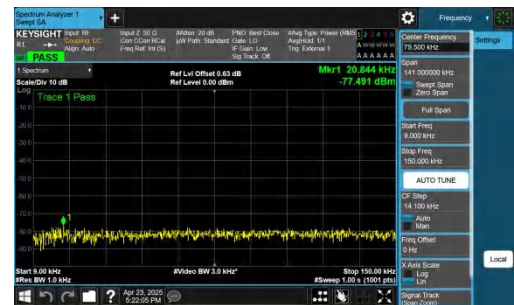
NTNV-n48-PC3-30-40-M-CP-QPSK-Inner_1RB_Right-0.009-0.15-P ASS
