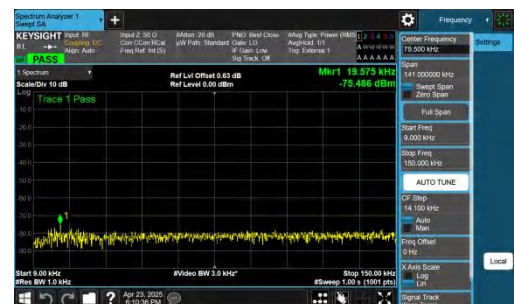
NTNV-n48-PC3-30-20-L-CP-QPSK-Inner_1RB_Right-0.009-0.15-P ASS
