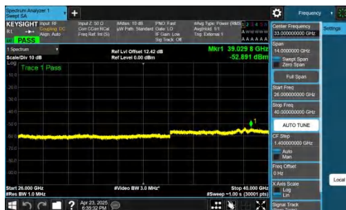
NTNV-n48-PC3-30-40-L-CP-QPSK-Inner_1RB_Left-26000-40000-
