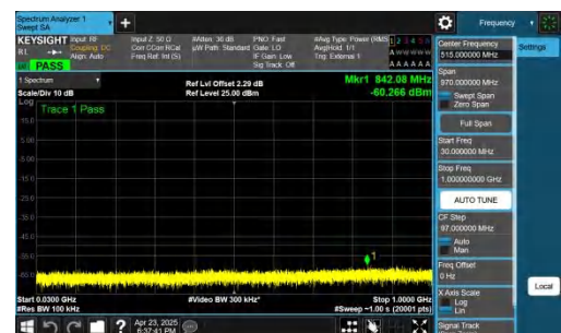
NTNV-n48-PC3-30-40-L-CP-QPSK-Inner_1RB_Right-30-1000-PAS
