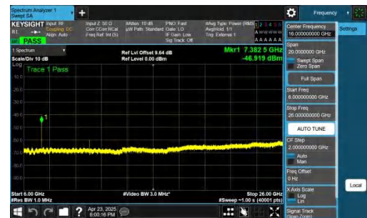
NTNV-n48-PC3-30-10-H-CP-QPSK-Inner_1RB_Left-6000-26000-P
