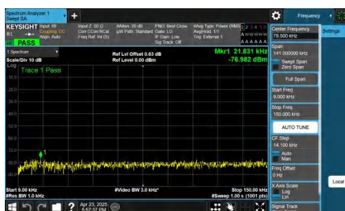
NTNV-n48-PC3-30-10-H-CP-QPSK-Inner_1RB_Left-0.009-0.15-P ASS
