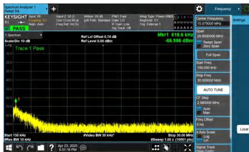
NTNV-n48-PC3-30-40-H-CP-QPSK-Inner_1RB_Right-0.15-30-PA SS
