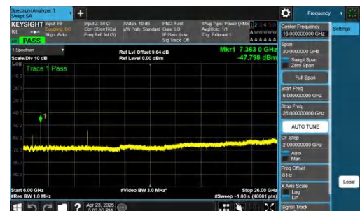
NTNV-n48-PC3-30-20-H-CP-QPSK-Inner_1RB_Left-6000-26000-P ASS
