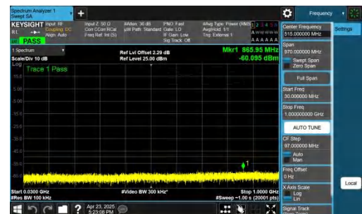
NTNV-n48-PC3-30-40-M-CP-QPSK-Inner_1RB_Right-30-1000-PA SS
