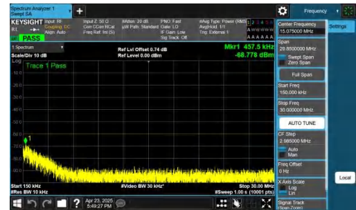
NTNV-n48-PC3-30-10-M-CP-QPSK-Inner_1RB_Left-0.15-30-PASS
