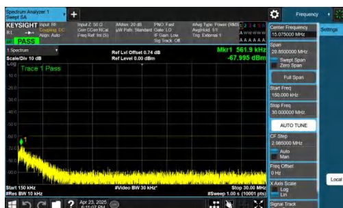
NTNV-n48-PC3-30-20-L-CP-QPSK-Inner_1RB_Right-0.15-30-PA SS
