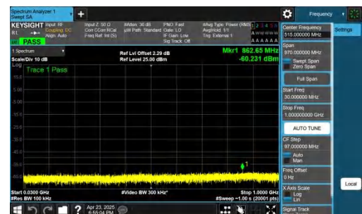
NTNV-n48-PC3-30-40-H-CP-QPSK-Inner_1RB_Right-30-1000-PA SS
