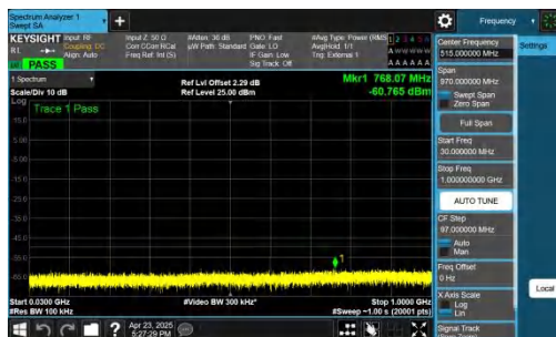
NTNV-n48-PC3-30-40-H-CP-QPSK-Inner_1RB_Left-30-1000-PASS
