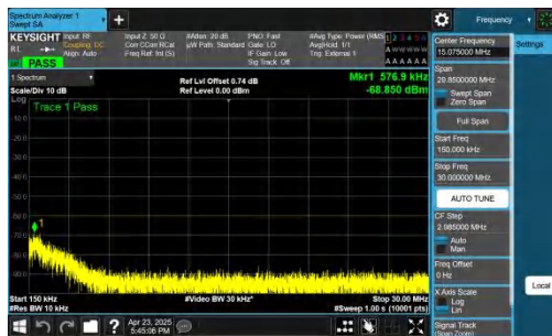
NTNV-n48-PC3-30-10-L-CP-QPSK-Inner_1RB_Right-0.15-30-PA-SS
