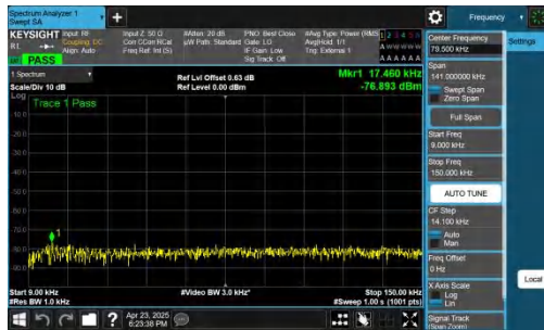
NTNV-n48-PC3-30-20-H-CP-QPSK-Inner_1RB_Left-0.009-0.15-P ASS
