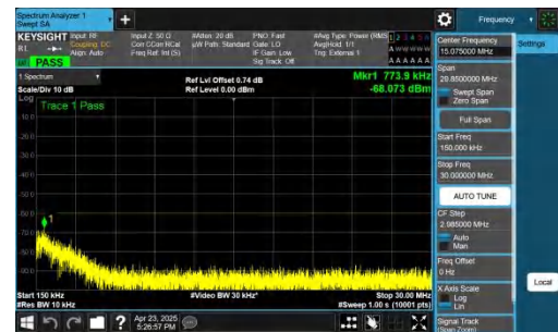
NTNV-n48-PC3-30-40-H-CP-QPSK-Inner_1RB_Left-0.15-30-PASS
