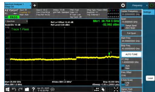
NTNV-n48-PC3-30-40-L-CP-QPSK-Inner_1RB_Right-26000-40000-PASS
