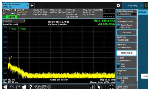
NTNV-n48-PC3-30-40-M-CP-QPSK-Inner_1RB_Right-0.15-30-PA SS
