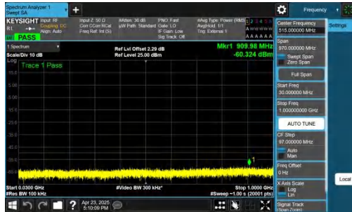
NTNV-n48-PC3-30-40-L-CP-QPSK-Inner_1RB_Left-30-1000-PAS
