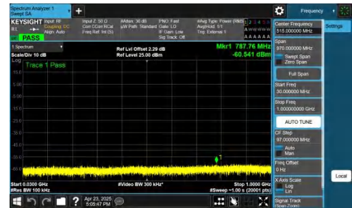
NTNV-n48-PC3-30-20-H-CP-QPSK-Inner_1RB_Right-30-1000-PA SS
