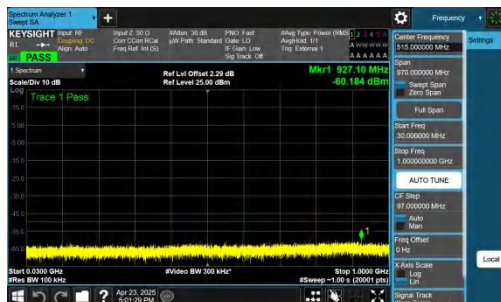
NTNV-n48-PC3-30-20-H-CP-QPSK-Inner_1RB_Left-30-1000-PAS S
