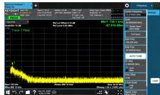
NTNV-n48-PC3-30-40-H-CP-QPSK-Inner_1RB_Left-0.15-30-PASS
