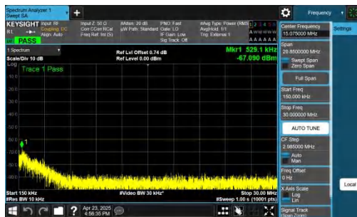
NTNV-n48-PC3-30-20-M-CP-QPSK-Inner_1RB_Right-0.15-30-PA SS
