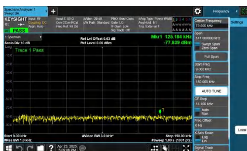
NTNV-n48-PC3-30-40-L-CP-QPSK-Inner_1RB_Left-0.009-0.15-P ASS
