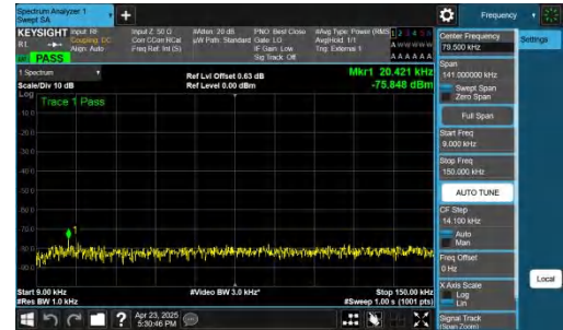
NTNV-n48-PC3-30-40-H-CP-QPSK-Inner_1RB_Right-0.009-0.15-P ASS
