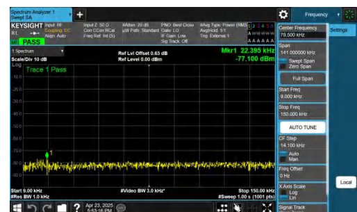
NTNV-n48-PC3-30-10-M-CP-QPSK-Inner_1RB_Right-0.009-0.15-P ASS
