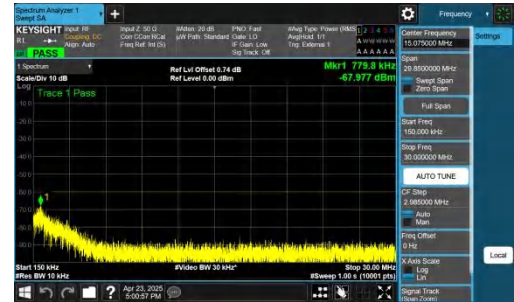
NTNV-n48-PC3-30-20-H-CP-QPSK-Inner_1RB_Left-0.15-30-PASS
