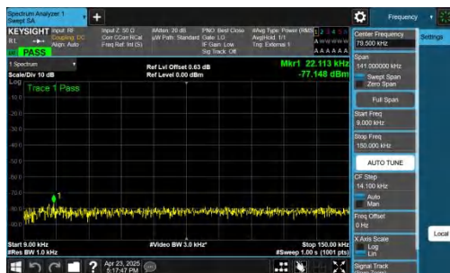
NTNV-n48-PC3-30-40-M-CP-QPSK-Inner_1RB_Left-0.009-0.15-PASS
