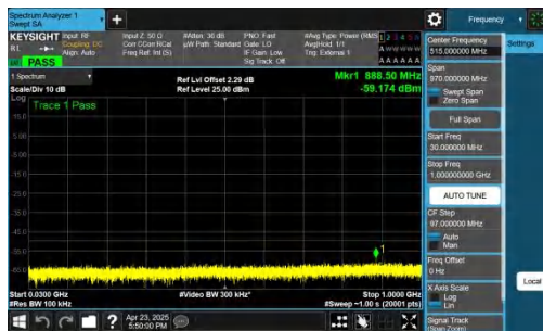
NTNV-n48-PC3-30-10-M-CP-QPSK-Inner_1RB_Left-30-1000-PAS S
