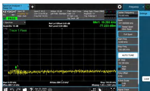
NTNV-n48-PC3-30-40-L-CP-QPSK-Inner_1RB_Left-0.009-0.15-P ASS
