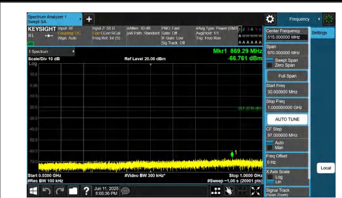
66-66-20MHz-5MHz-QPSK-QPSK-132522-132639-1RB#0-1RB# 24-30~1000MHz-PASS
