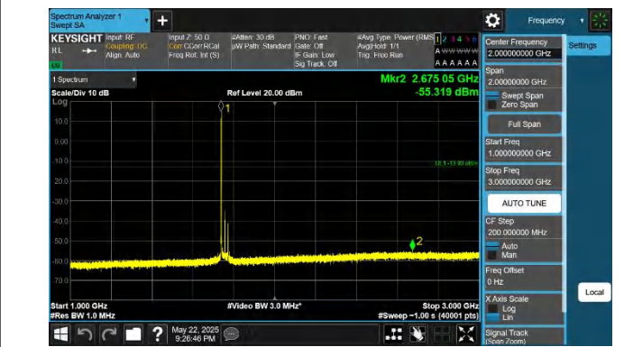
66-66-20MHz-15MHz-QPSK-QPSK-132348-132519-1RB#0-1RB #74-1000~3000MHz-PASS
