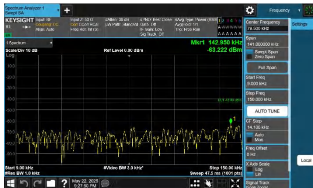
66-66-20MHz-15MHz-QPSK-QPSK-132423-132594-1RB#99-0R B#0-0.009~0.15MHz-PASS
