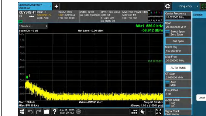
66-66-20MHz-15MHz-QPSK-QPSK-132348-132519-1RB#0-0RB #0-0.15~30MHz-PASS
