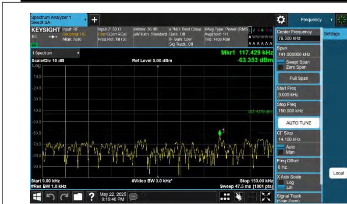
66-66-20MHz-15MHz-QPSK-QPSK-132072-132243-1RB#0-0RB #0-0.009~0.15MHz-PASS
