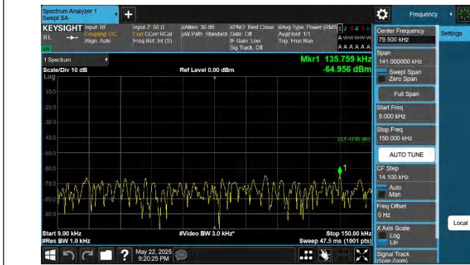
66-66-20MHz-15MHz-QPSK-QPSK-132072-132243-1RB#99-0R B#0-0.009~0.15MHz-PASS
