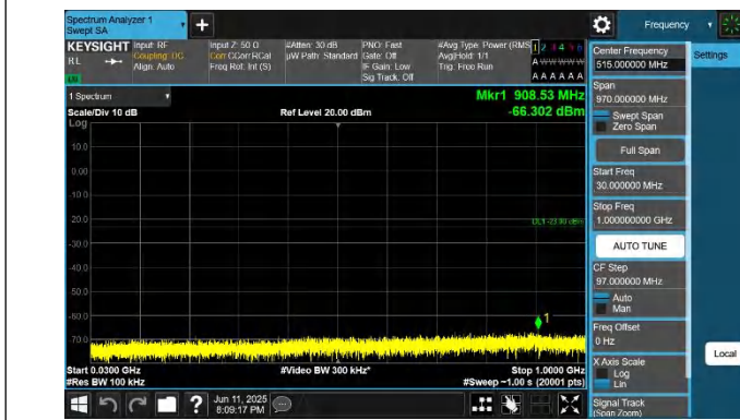
66-66-20MHz-15MHz-QPSK-QPSK-132348-132519-1RB#0-1RB #74-30~1000MHz-PASS
