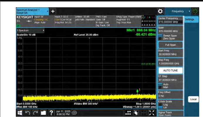
66-66-20MHz-15MHz-QPSK-QPSK-132072-132243-1RB#0-1RB #74-30~1000MHz-PASS
