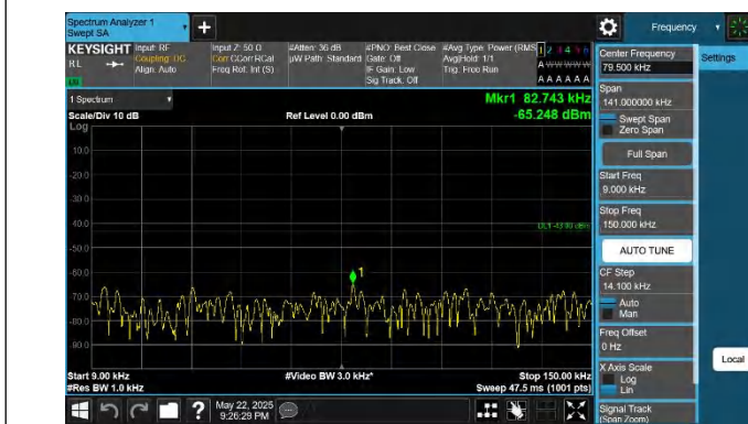
66-66-20MHz-15MHz-QPSK-QPSK-132348-132519-1RB#0-1RB #74-0.009~0.15MHz-PASS
