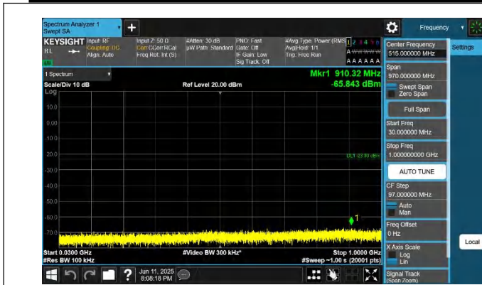
66-66-20MHz-15MHz-QPSK-QPSK-132072-132243-1RB#99-0R B#0-30~1000MHz-PASS
