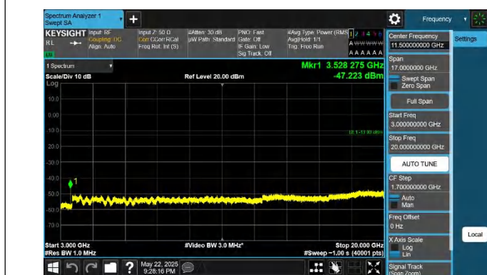
66-66-20MHz-15MHz-QPSK-QPSK-132423-132594-1RB#99-0R B#0-3000~20000MHz-PASS
