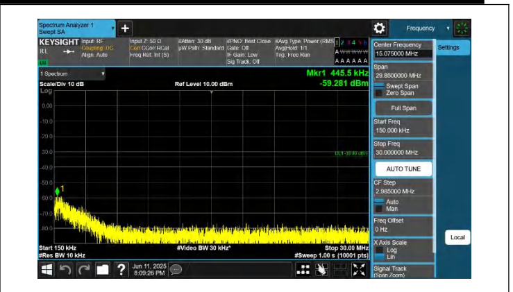
66-66-20MHz-15MHz-QPSK-QPSK-132423-132594-1RB#0-0RB #0-0.15~30MHz-PASS
