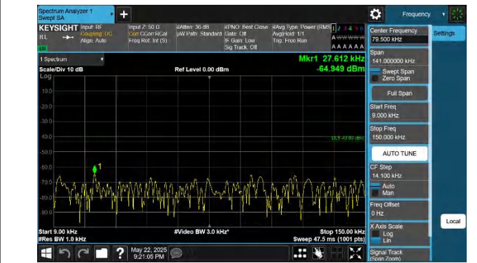
66-66-20MHz-15MHz-QPSK-QPSK-132072-132243-1RB#0-1RB #74-0.009~0.15MHz-PASS
