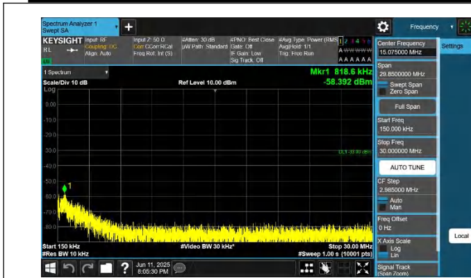
66-66-20MHz-5MHz-QPSK-QPSK-132522-132639-1RB#0-1RB# 24-0.15~30MHz-PASS
