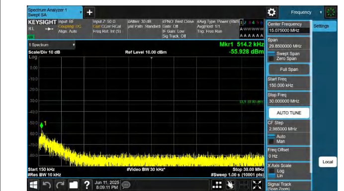
66-66-20MHz-15MHz-QPSK-QPSK-132348-132519-1RB#0-1RB #74-0.15~30MHz-PASS
