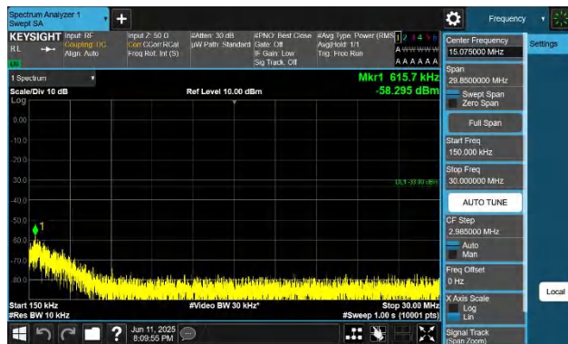
66-66-20MHz-15MHz-QPSK-QPSK-132423-132594-1RB#0-1RB #74-0.15~30MHz-PASS
