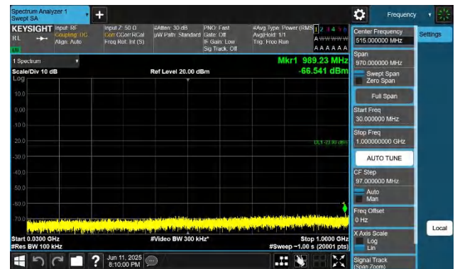
66-66-20MHz-15MHz-QPSK-QPSK-132423-132594-1RB#0-1RB #74-30~1000MHz-PASS
