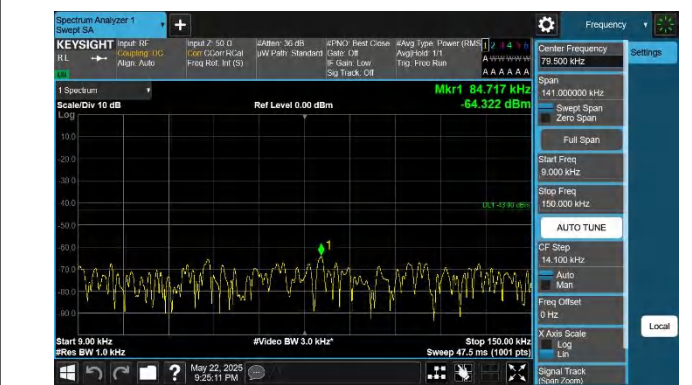
66-66-20MHz-15MHz-QPSK-QPSK-132348-132519-1RB#0-0RB #0-0.009~0.15MHz-PASS
