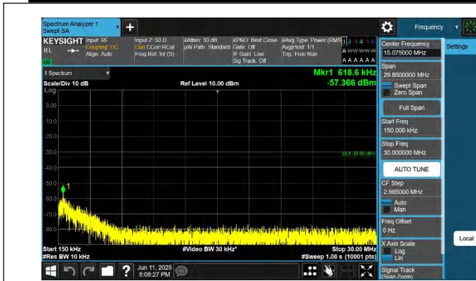
66-66-20MHz-15MHz-QPSK-QPSK-132072-132243-1RB#0-1RB #74-0.15~30MHz-PASS
