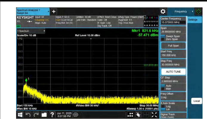
66-66-20MHz-15MHz-QPSK-QPSK-132072-132243-1RB#0-0RB #0-0.15~30MHz-PASS
