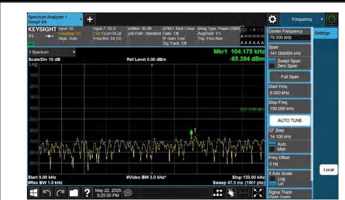
66-66-20MHz-15MHz-QPSK-QPSK-132348-132519-1RB#99-0R B#0-0.009~0.15MHz-PASS
