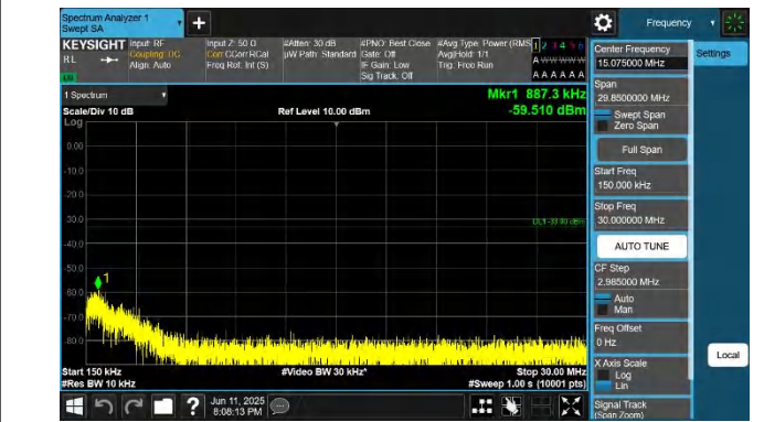
66-66-20MHz-15MHz-QPSK-QPSK-132072-132243-1RB#99-0R B#0-0.15~30MHz-PASS
