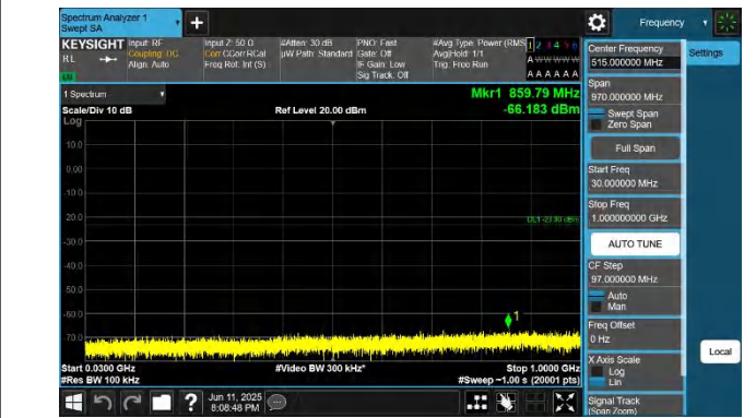
66-66-20MHz-15MHz-QPSK-QPSK-132348-132519-1RB#0-0RB #0-30~1000MHz-PASS
