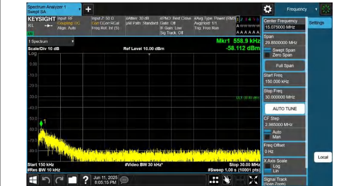
66-66-20MHz-5MHz-QPSK-QPSK-132522-132639-1RB#99-0RB #0-0.15~30MHz-PASS
