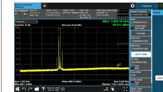
66-66-20MHz-15MHz-QPSK-QPSK-132072-132243-1RB#0-1RB #74-1000~3000MHz-PASS
