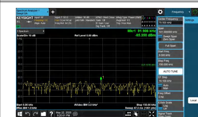
66-66-15MHz-20MHz-QPSK-QPSK-132050-132221-1RB#0-0RB #0-0.009~0.15MHz-PASS
