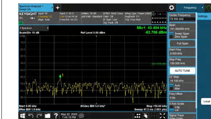
66-66-15MHz-10MHz-QPSK-QPSK-132499-132619-1RB#0-1RB #49-0.009~0.15MHz-PASS
