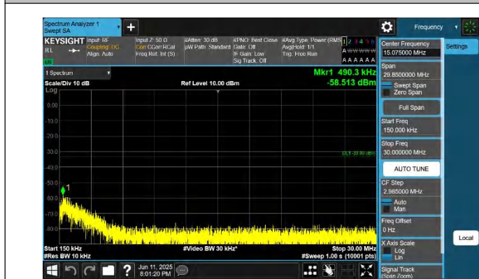
66-66-15MHz-20MHz-QPSK-QPSK-132050-132221-1RB#0-0RB #0-0.15~30MHz-PASS
