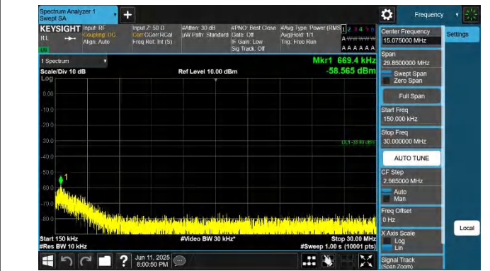
66-66-15MHz-15MHz-QPSK-QPSK-132447-132597-1RB#74-0R B#0-0.15~30MHz-PASS
