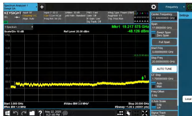
66-66-15MHz-20MHz-QPSK-QPSK-132050-132221-1RB#74-0R B#0-3000~20000MHz-PASS
