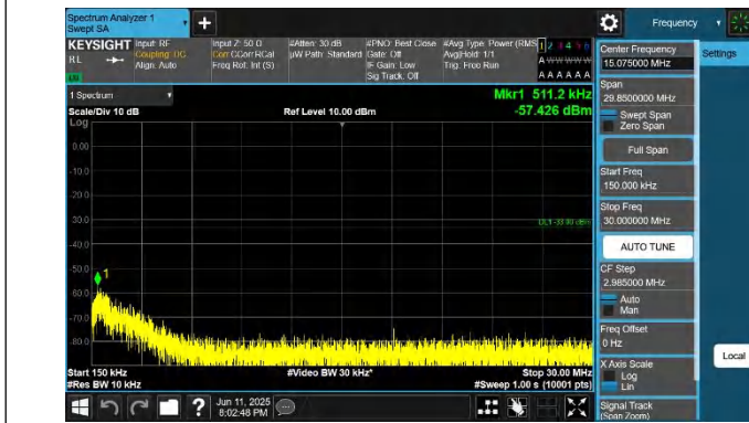
66-66-15MHz-20MHz-QPSK-QPSK-132401-132572-1RB#0-0RB #0-0.15~30MHz-PASS
