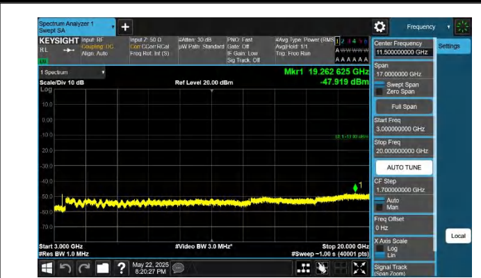
66-66-15MHz-20MHz-QPSK-QPSK-132050-132221-1RB#0-0RB #0-3000~20000MHz-PASS
