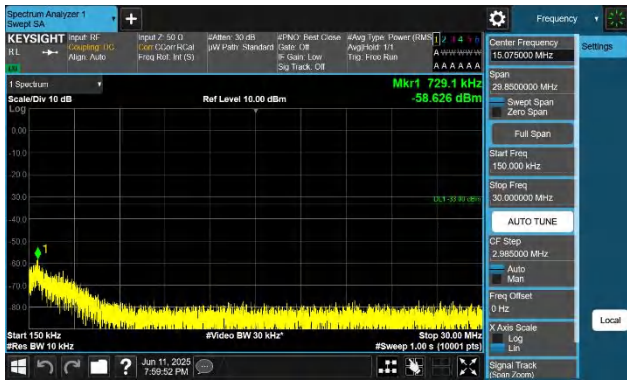
66-66-15MHz-15MHz-QPSK-QPSK-132347-132497-1RB#0-0RB #0-0.15~30MHz-PASS
