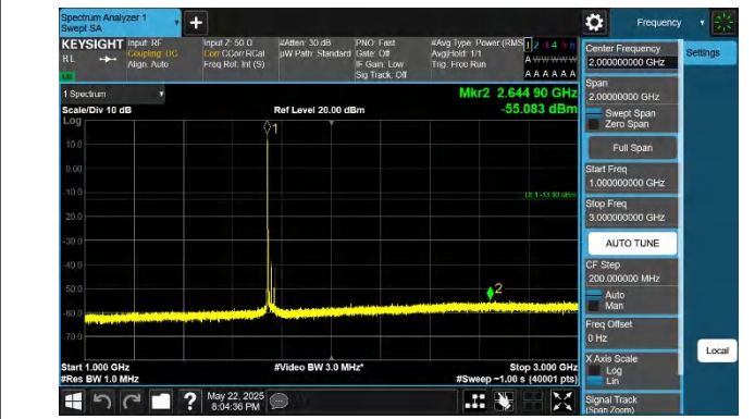
66-66-15MHz-15MHz-QPSK-QPSK-132347-132497-1RB#0-1RB #74-1000~3000MHz-PASS
