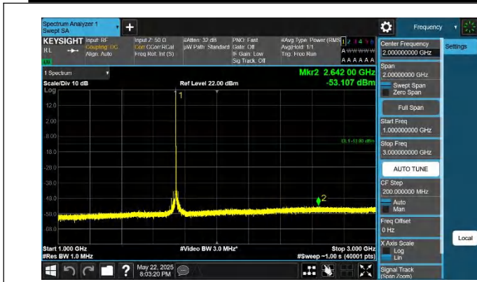
66-66-15MHz-15MHz-QPSK-QPSK-132347-132497-1RB#0-0RB #0-1000~3000MHz-PASS
