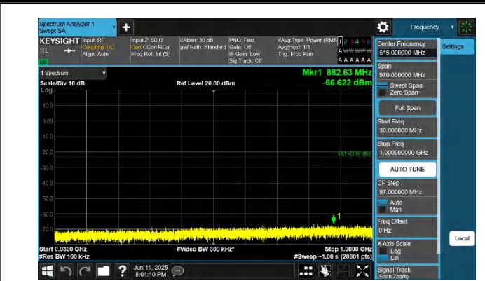
66-66-15MHz-15MHz-QPSK-QPSK-132447-132597-1RB#0-1RB #74-30~1000MHz-PASS
