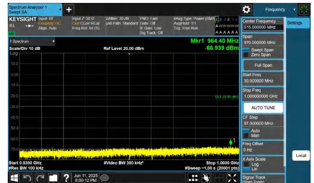
66-66-15MHz-15MHz-QPSK-QPSK-132347-132497-1RB#74-0R B#0-30~1000MHz-PASS
