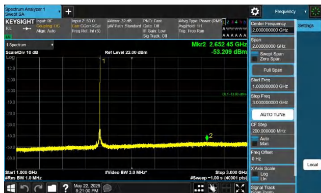
66-66-15MHz-20MHz-QPSK-QPSK-132050-132221-1RB#74-0R B#0-1000~3000MHz-PASS
