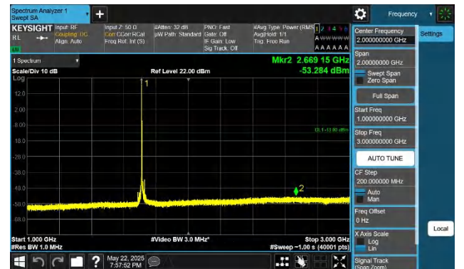
66-66-15MHz-15MHz-QPSK-QPSK-132047-132197-1RB#0-0RB #0-1000~3000MHz-PASS
