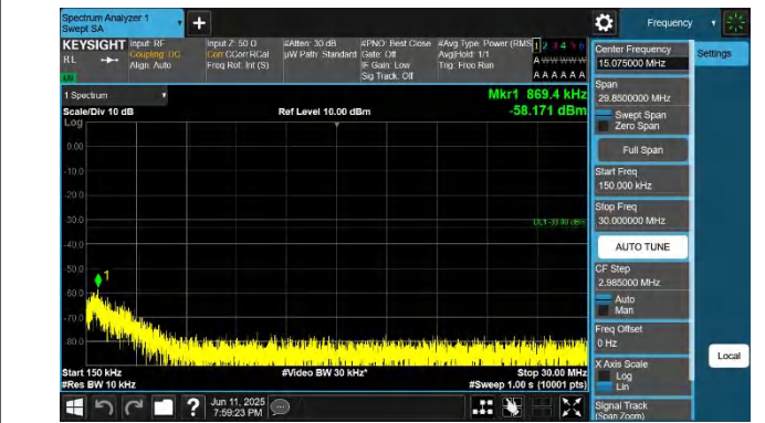
66-66-15MHz-15MHz-QPSK-QPSK-132047-132197-1RB#74-0R B#0-0.15~30MHz-PASS
