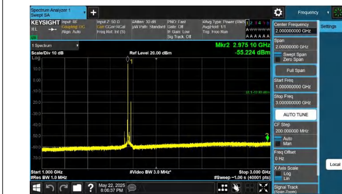
66-66-15MHz-15MHz-QPSK-QPSK-132447-132597-1RB#0-1RB #74-1000~3000MHz-PASS
