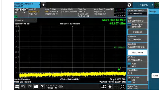
66-66-15MHz-10MHz-QPSK-QPSK-132499-132619-1RB#0-1RB #49-30~1000MHz-PASS
