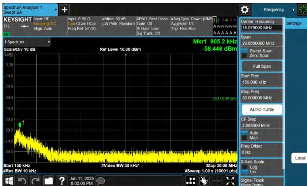
66-66-15MHz-15MHz-QPSK-QPSK-132347-132497-1RB#74-0R B#0-0.15~30MHz-PASS
