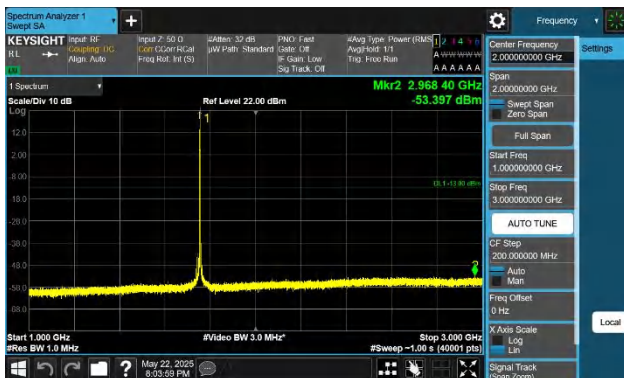
66-66-15MHz-15MHz-QPSK-QPSK-132347-132497-1RB#74-0R B#0-1000~3000MHz-PASS
