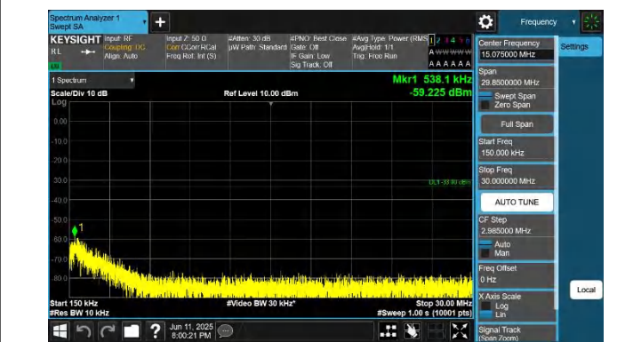
66-66-15MHz-15MHz-QPSK-QPSK-132347-132497-1RB#0-1RB #74-0.15~30MHz-PASS
