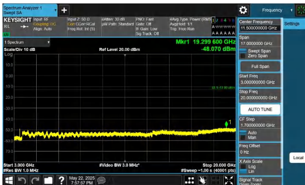
66-66-15MHz-15MHz-QPSK-QPSK-132047-132197-1RB#0-0RB #0-3000~20000MHz-PASS
