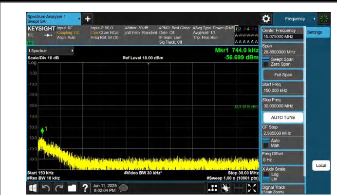
66-66-15MHz-20MHz-QPSK-QPSK-132325-132496-1RB#0-0RB #0-0.15~30MHz-PASS
