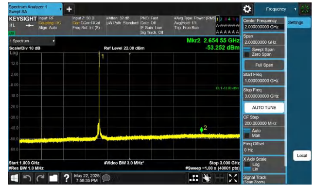
66-66-15MHz-15MHz-QPSK-QPSK-132047-132197-1RB#74-0R B#0-1000~3000MHz-PASS
