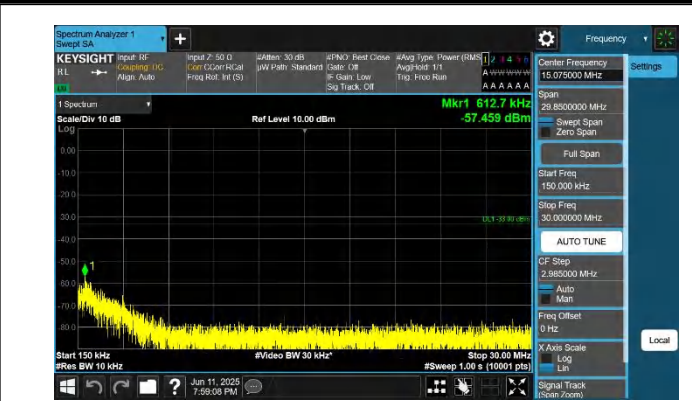
66-66-15MHz-15MHz-QPSK-QPSK-132047-132197-1RB#0-0RB #0-0.15~30MHz-PASS
