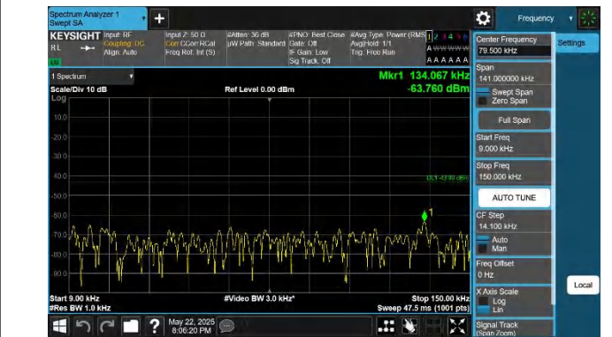
66-66-15MHz-15MHz-QPSK-QPSK-132447-132597-1RB#0-1RB #74-0.009~0.15MHz-PASS
