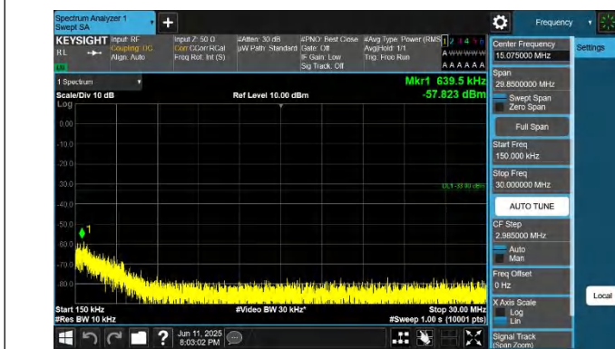
66-66-15MHz-20MHz-QPSK-QPSK-132401-132572-1RB#74-0R B#0-0.15~30MHz-PASS
