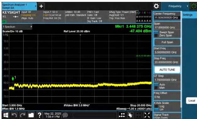
66-66-15MHz-15MHz-QPSK-QPSK-132047-132197-1RB#74-0R B#0-3000~20000MHz-PASS
