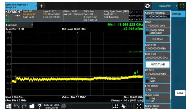
66-66-15MHz-15MHz-QPSK-QPSK-132347-132497-1RB#74-0R B#0-3000~20000MHz-PASS
