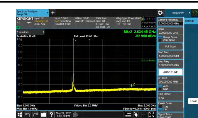
66-66-15MHz-15MHz-QPSK-QPSK-132447-132597-1RB#74-0R B#0-1000~3000MHz-PASS
