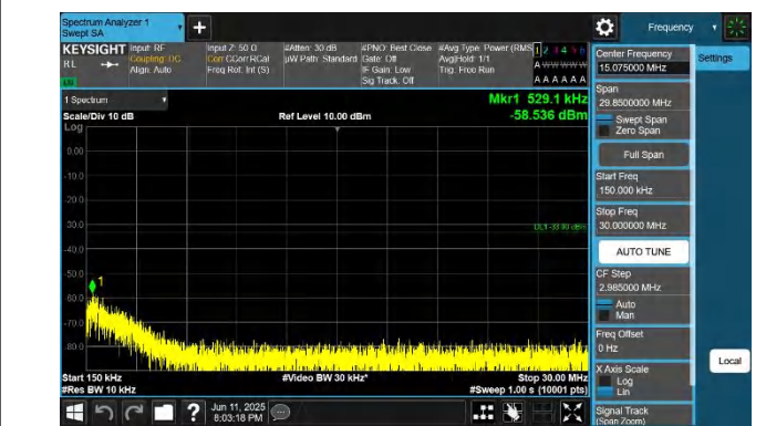
66-66-15MHz-20MHz-QPSK-QPSK-132401-132572-1RB#0-1RB #99-0.15~30MHz-PASS
