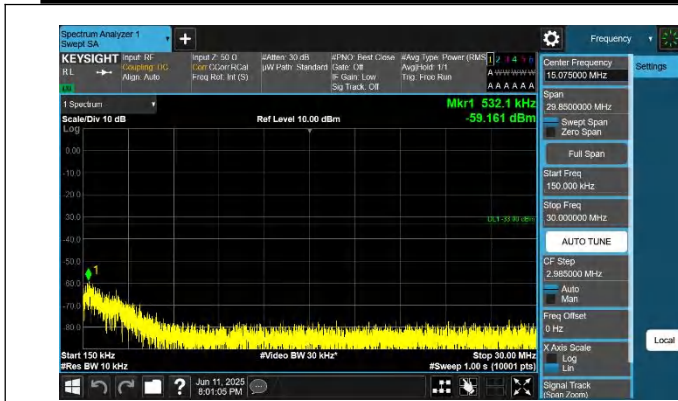
66-66-15MHz-15MHz-QPSK-QPSK-132447-132597-1RB#0-1RB #74-0.15~30MHz-PASS
