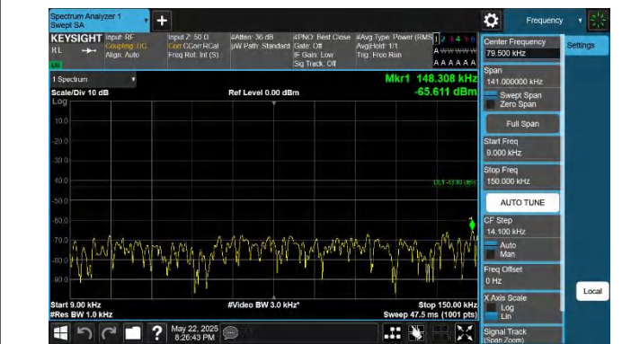
66-66-15MHz-20MHz-QPSK-QPSK-132325-132496-1RB#0-1RB #99-0.009~0.15MHz-PASS
