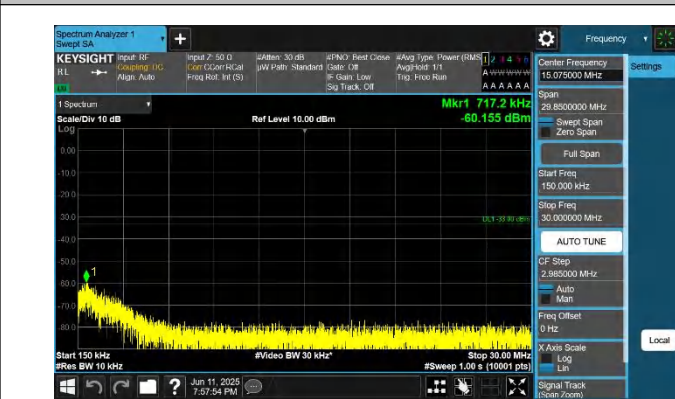
66-66-15MHz-10MHz-QPSK-QPSK-132373-132493-1RB#74-0R B#0-0.15~30MHz-PASS
