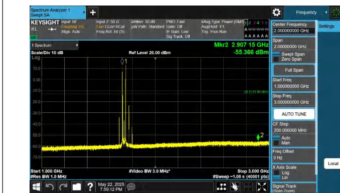
66-66-15MHz-15MHz-QPSK-QPSK-132047-132197-1RB#0-1RB #74-1000~3000MHz-PASS
