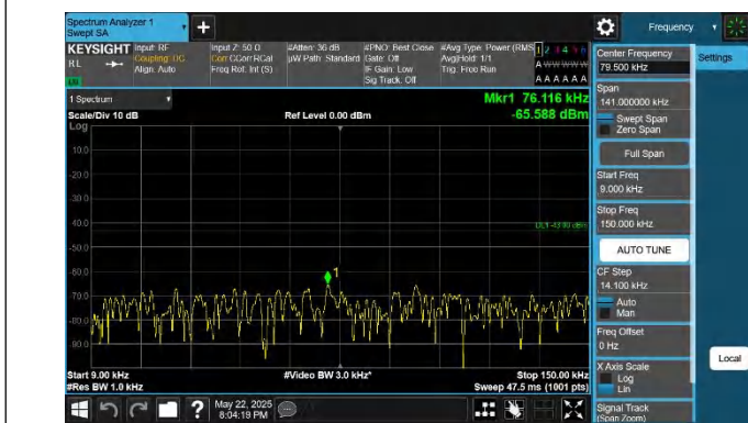
66-66-15MHz-15MHz-QPSK-QPSK-132347-132497-1RB#0-1RB #74-0.009~0.15MHz-PASS
