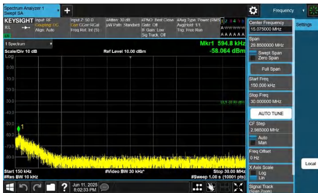
66-66-15MHz-20MHz-QPSK-QPSK-132325-132496-1RB#0-1RB #99-0.15~30MHz-PASS
