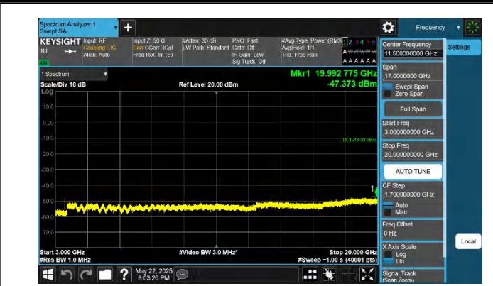
66-66-15MHz-15MHz-QPSK-QPSK-132347-132497-1RB#0-0RB #0-3000~20000MHz-PASS
