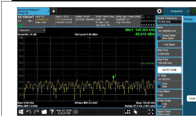
66-66-15MHz-20MHz-QPSK-QPSK-132325-132496-1RB#0-0RB #0-0.009~0.15MHz-PASS
