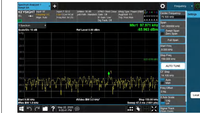
66-66-15MHz-15MHz-QPSK-QPSK-132447-132597-1RB#74-0R B#0-0.009~0.15MHz-PASS
