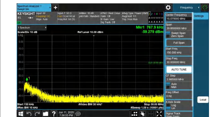
66-66-15MHz-10MHz-QPSK-QPSK-132499-132619-1RB#0-1RB #49-0.15~30MHz-PASS
