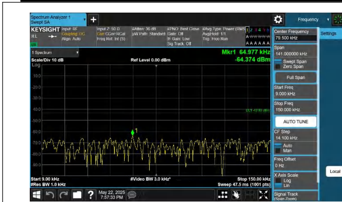
66-66-15MHz-15MHz-QPSK-QPSK-132047-132197-1RB#0-0RB #0-0.009~0.15MHz-PASS
