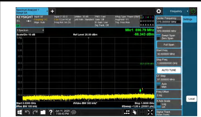
66-66-15MHz-15MHz-QPSK-QPSK-132047-132197-1RB#0-1RB #74-30~1000MHz-PASS
