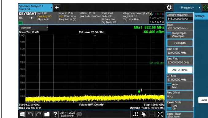
66-66-15MHz-20MHz-QPSK-QPSK-132325-132496-1RB#0-0RB #0-30~1000MHz-PASS
