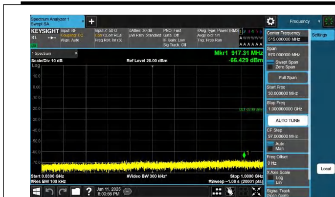
66-66-15MHz-15MHz-QPSK-QPSK-132447-132597-1RB#74-0R B#0-30~1000MHz-PASS
