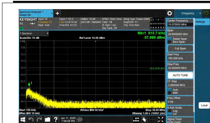
66-66-15MHz-10MHz-QPSK-QPSK-132373-132493-1RB#0-1RB #49-0.15~30MHz-PASS
