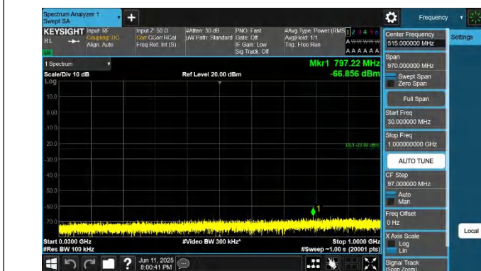
66-66-15MHz-15MHz-QPSK-QPSK-132447-132597-1RB#0-0RB #0-30~1000MHz-PASS
