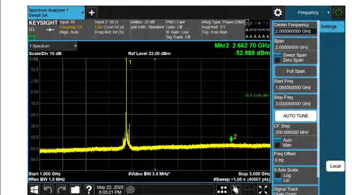
66-66-15MHz-15MHz-QPSK-QPSK-132447-132597-1RB#0-0RB #0-1000~3000MHz-PASS
