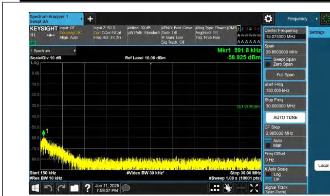
66-66-15MHz-15MHz-QPSK-QPSK-132047-132197-1RB#0-1RB #74-0.15~30MHz-PASS
