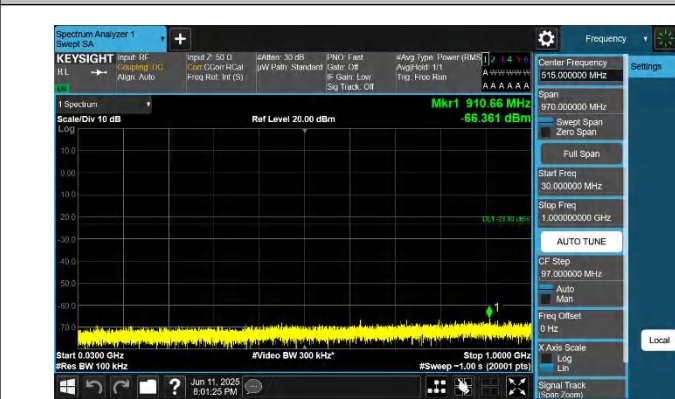
66-66-15MHz-20MHz-QPSK-QPSK-132050-132221-1RB#0-0RB #0-30~1000MHz-PASS
