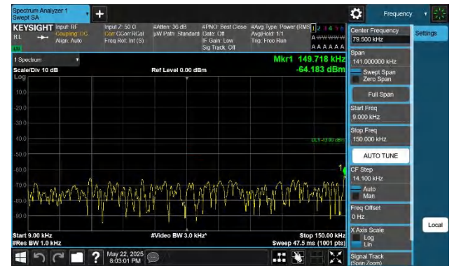
66-66-15MHz-15MHz-QPSK-QPSK-132347-132497-1RB#0-0RB #0-0.009~0.15MHz-PASS
