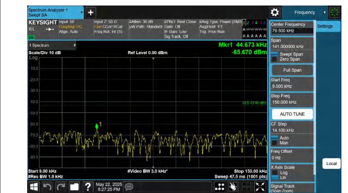
66-66-15MHz-20MHz-QPSK-QPSK-132401-132572-1RB#0-0RB #0-0.009~0.15MHz-PASS
