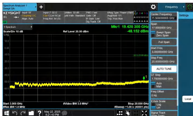
66-66-15MHz-20MHz-QPSK-QPSK-132050-132221-1RB#0-1RB #99-3000~20000MHz-PASS
