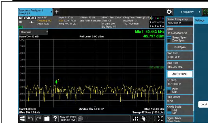
66-66-15MHz-15MHz-QPSK-QPSK-132447-132597-1RB#0-0RB #0-0.009~0.15MHz-PASS
