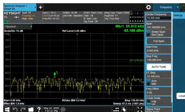
66-66-15MHz-10MHz-QPSK-QPSK-132047-132167-1RB#0-0RB #0-0.009~0.15MHz-PASS
