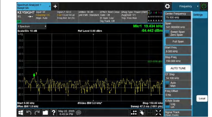
66-66-10MHz-15MHz-QPSK-QPSK-132351-132471-1RB#0-1RB #74-0.009~0.15MHz-PASS
