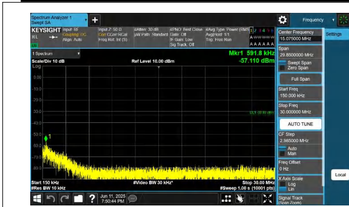
66-66-5MHz-20MHz-QPSK-QPSK-132027-132171-1RB#0-1RB# 99-0.15~30MHz-PASS
