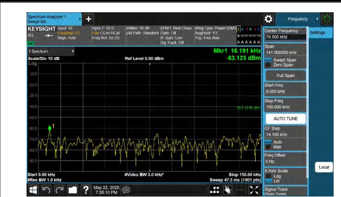
66-66-15MHz-10MHz-QPSK-QPSK-132047-132167-1RB#74-0R B#0-0.009~0.15MHz-PASS
