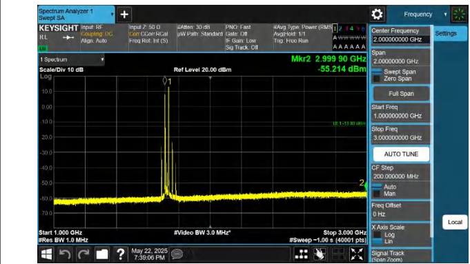
66-66-15MHz-10MHz-QPSK-QPSK-132047-132167-1RB#0-1RB #49-1000~3000MHz-PASS
