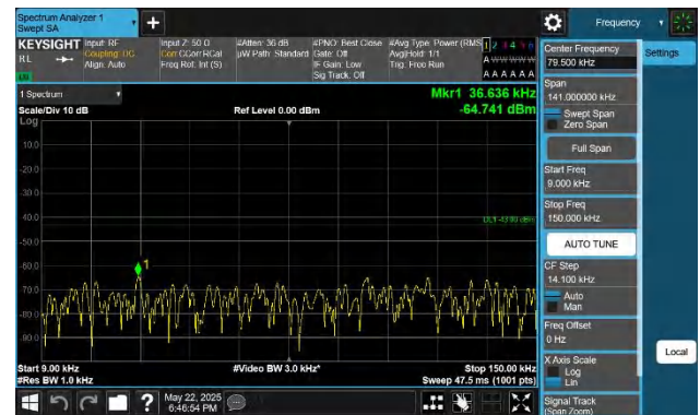
66-66-10MHz-15MHz-QPSK-QPSK-132025-132145-1RB#49-0R B#0-0.009~0.15MHz-PASS
