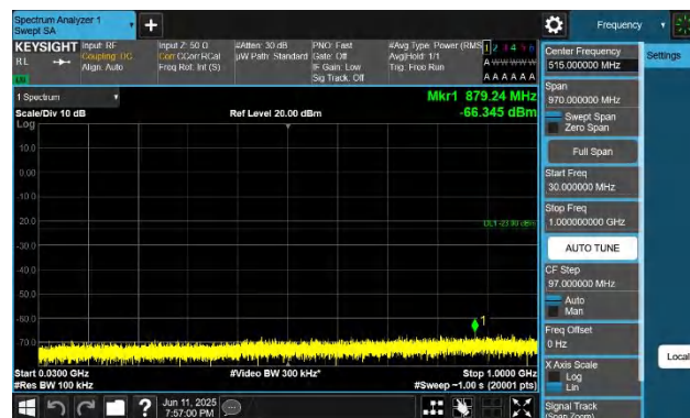
66-66-15MHz-10MHz-QPSK-QPSK-132047-132167-1RB#0-0RB #0-30~1000MHz-PASS
