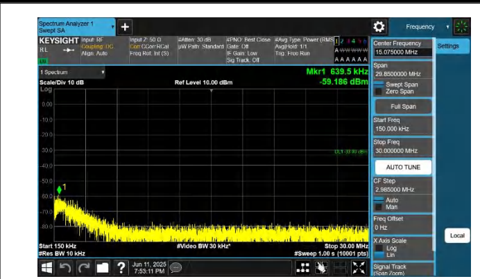
66-66-10MHz-15MHz-QPSK-QPSK-132351-132471-1RB#0-0RB #0-0.15~30MHz-PASS
