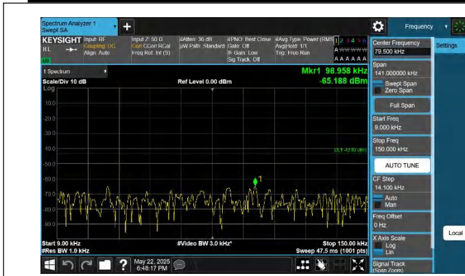
66-66-10MHz-15MHz-QPSK-QPSK-132351-132471-1RB#0-0RB #0-0.009~0.15MHz-PASS
