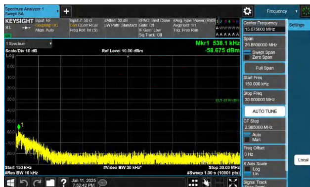
66-66-10MHz-15MHz-QPSK-QPSK-132025-132145-1RB#49-0R B#0-0.15~30MHz-PASS
