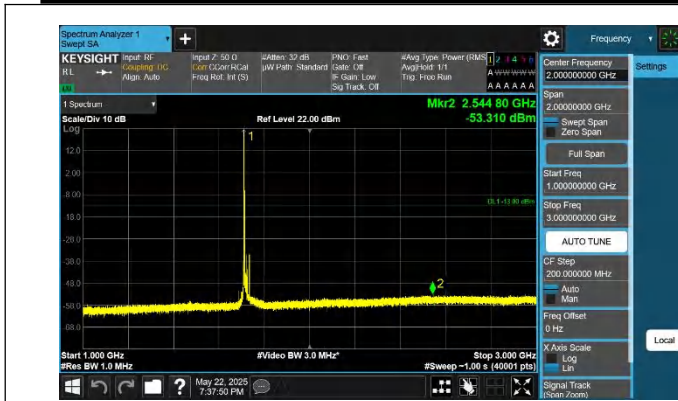
66-66-15MHz-10MHz-QPSK-QPSK-132047-132167-1RB#0-0RB #0-1000~3000MHz-PASS
