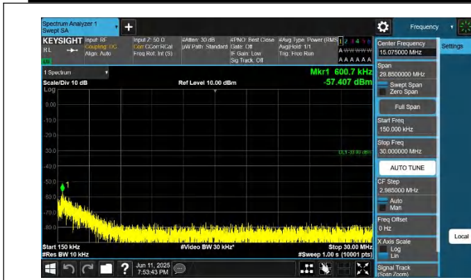
66-66-10MHz-15MHz-QPSK-QPSK-132351-132471-1RB#0-1RB #74-0.15~30MHz-PASS
