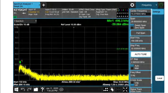
66-66-5MHz-20MHz-QPSK-QPSK-132027-132171-1RB#24-0RB #0-0.15~30MHz-PASS
