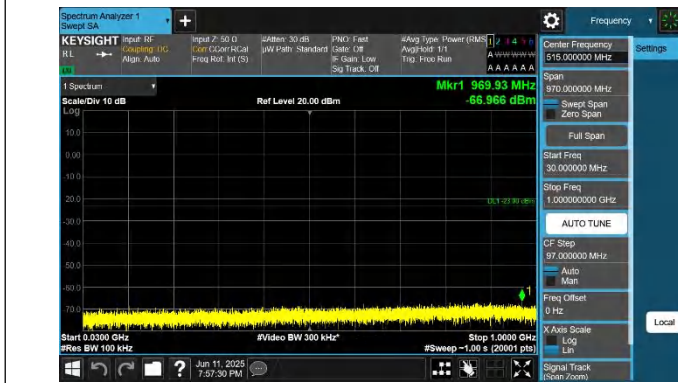
66-66-15MHz-10MHz-QPSK-QPSK-132047-132167-1RB#0-1RB #49-30~1000MHz-PASS
