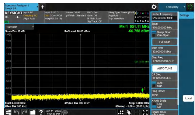
66-66-10MHz-15MHz-QPSK-QPSK-132025-132145-1RB#49-0R B#0-30~1000MHz-PASS
