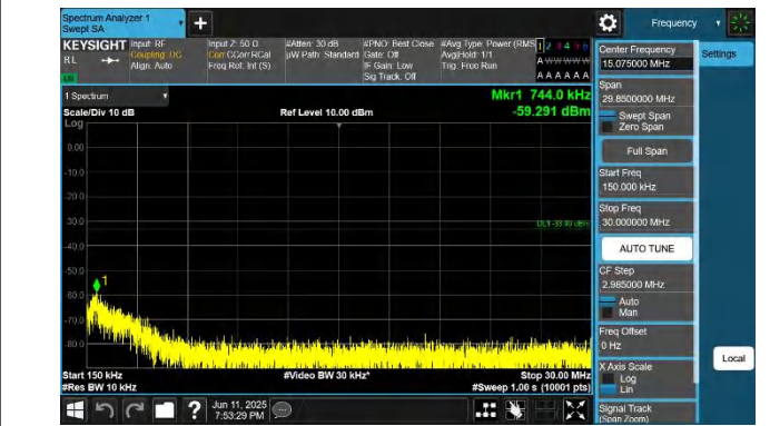
66-66-10MHz-15MHz-QPSK-QPSK-132351-132471-1RB#49-0R B#0-0.15~30MHz-PASS
