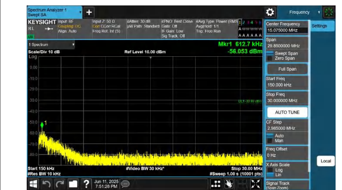
66-66-5MHz-20MHz-QPSK-QPSK-132328-132472-1RB#0-1RB# 99-0.15~30MHz-PASS
