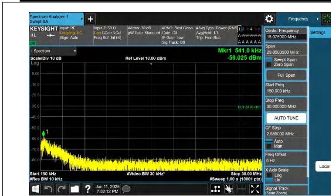
66-66-5MHz-20MHz-QPSK-QPSK-132428-132572-1RB#0-1RB# 99-0.15~30MHz-PASS
