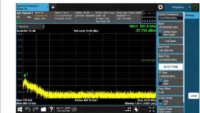
66-66-15MHz-10MHz-QPSK-QPSK-132047-132167-1RB#0-1RB #49-0.15~30MHz-PASS
