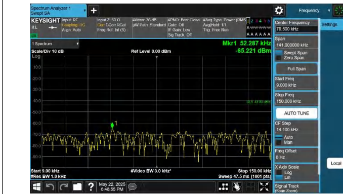
66-66-10MHz-15MHz-QPSK-QPSK-132351-132471-1RB#49-0R B#0-0.009~0.15MHz-PASS
