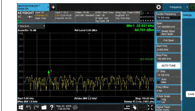
66-66-15MHz-10MHz-QPSK-QPSK-132047-132167-1RB#0-1RB #49-0.009~0.15MHz-PASS
