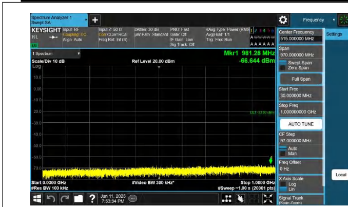
66-66-10MHz-15MHz-QPSK-QPSK-132351-132471-1RB#49-0R B#0-30~1000MHz-PASS
