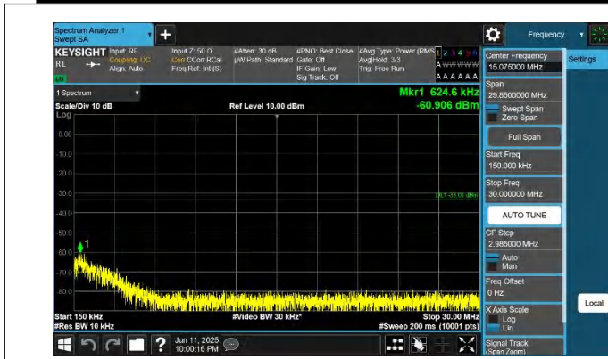
66-66-15MHz-5MHz-QPSK-QPSK-132047-132140-1RB#0-1RB# 24-0.15~30MHz-PASS
