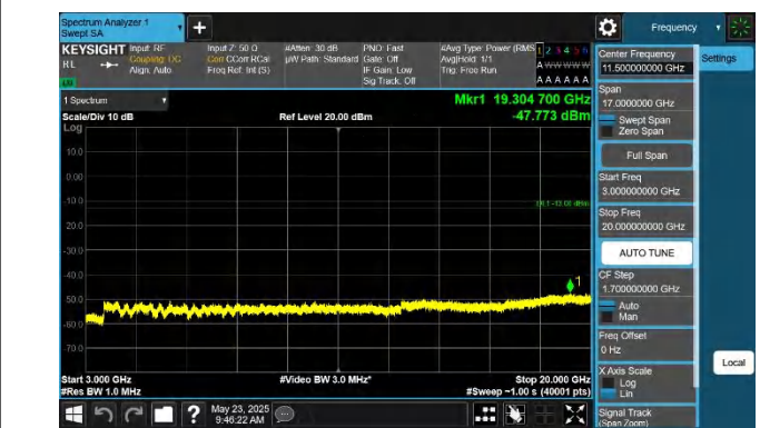
66-66-15MHz-5MHz-QPSK-QPSK-132549-132642-1RB#0-1RB# 24-3000~20000MHz-PASS
