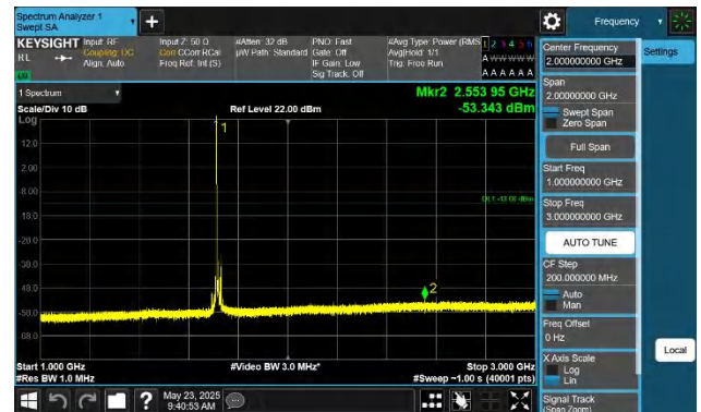
66-66-15MHz-5MHz-QPSK-QPSK-132047-132140-1RB#0-0RB# 0-1000~3000MHz-PASS
