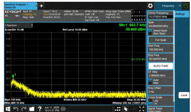
66-66-15MHz-5MHz-QPSK-QPSK-132398-132491-1RB#0-1RB# 24-0.15~30MHz-PASS
