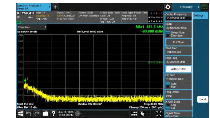
66-66-15MHz-5MHz-QPSK-QPSK-132549-132642-1RB#74-0RB #0-0.15~30MHz-PASS
