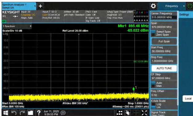
66-66-15MHz-5MHz-QPSK-QPSK-132047-132140-1RB#0-0RB# 0-30~1000MHz-PASS
