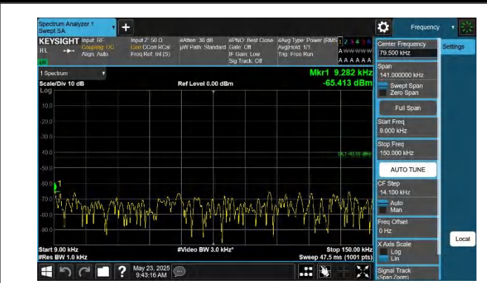
66-66-15MHz-5MHz-QPSK-QPSK-132398-132491-1RB#74-ORB #0-0.009~0.15MHz-PASS
