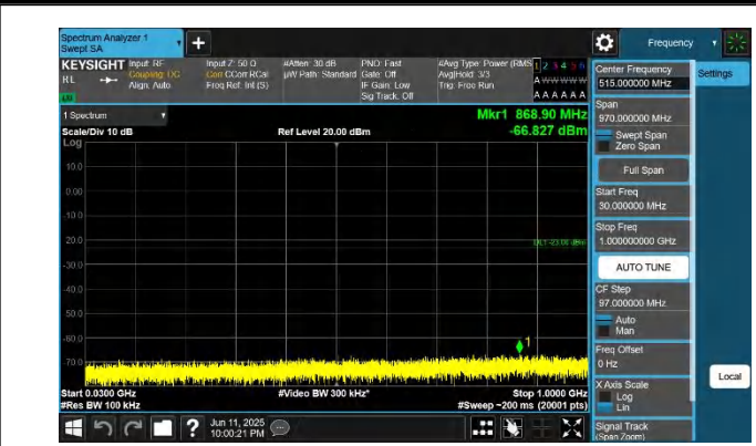
66-66-15MHz-5MHz-QPSK-QPSK-132047-132140-1RB#0-1RB# 24-30~1000MHz-PASS
