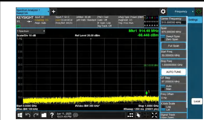
66-66-15MHz-5MHz-QPSK-QPSK-132549-132642-1RB#0-1RB# 24-30~1000MHz-PASS
