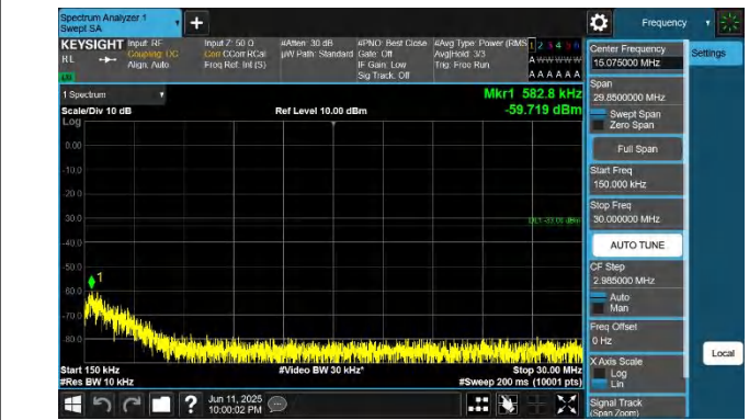
66-66-15MHz-5MHz-QPSK-QPSK-132047-132140-1RB#74-0RB #0-0.15~30MHz-PASS
