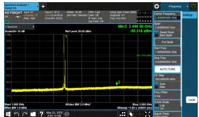
66-66-15MHz-5MHz-QPSK-QPSK-132398-132491-1RB#0-1RB# 24-1000~3000MHz-PASS
