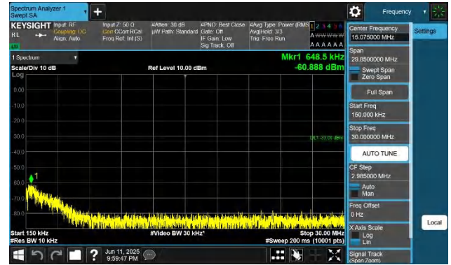
66-66-15MHz-5MHz-QPSK-QPSK-132047-132140-1RB#0-0RB# 0-0.15~30MHz-PASS
