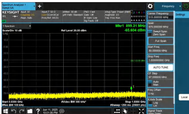
66-66-15MHz-5MHz-QPSK-QPSK-132398-132491-1RB#0-1RB# 24-30~1000MHz-PASS
