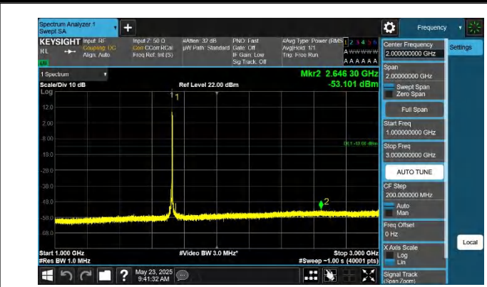
66-66-15MHz-5MHz-QPSK-QPSK-132047-132140-1RB#74-ORB #0-1000~3000MHz-PASS
