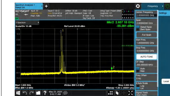
66-66-15MHz-5MHz-QPSK-QPSK-132047-132140-1RB#0-1RB# 24-1000~3000MHz-PASS
