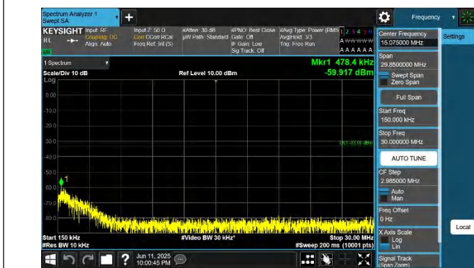
66-66-15MHz-5MHz-QPSK-QPSK-132398-132491-1RB#74-ORB #0-0.15~30MHz-PASS
