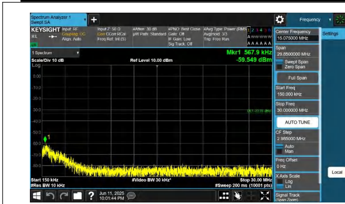
66-66-15MHz-5MHz-QPSK-QPSK-132549-132642-1RB#0-1RB# 24-0.15~30MHz-PASS
