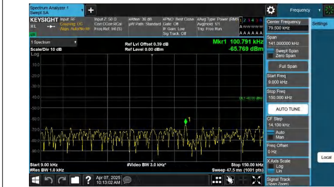
66-66-10MHz-5MHz-QPSK-QPSK-132022-132094-1RB#49-0RB #0-0.009~0.15MHz-PASS
