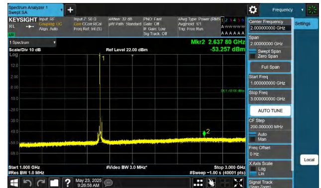
66-66-5MHz-15MHz-QPSK-QPSK-132002-132095-1RB#0-0RB# 0-1000~3000MHz-PASS
