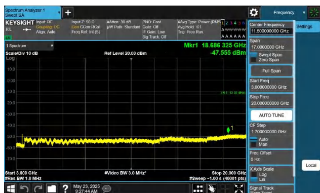
66-66-5MHz-15MHz-QPSK-QPSK-132002-132095-1RB#24-0RB #0-3000~20000MHz-PASS
