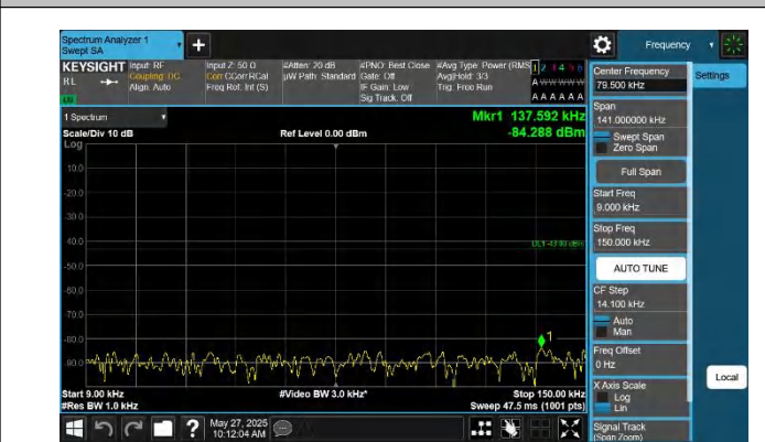
42-42-20MHz-20MHz-QPSK-QPSK-42491-42689-1RB#0-0RB#- 0.009~0.15MHz-PASS
