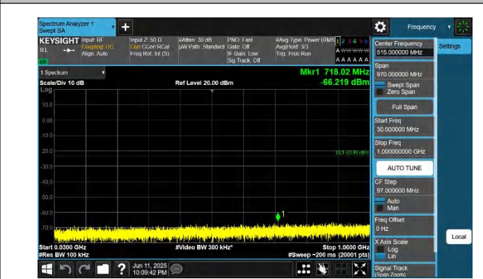
42-42-20MHz-20MHz-QPSK-QPSK-42491-42689-1RB#0-0RB#- 30~1000MHz-PASS
