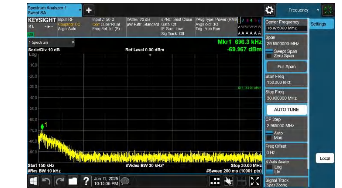
42-42-20MHz-20MHz-QPSK-QPSK-42491-42689-1RB#0-1RB#9 9-0.15~30MHz-PASS
