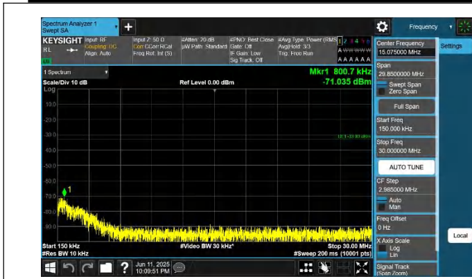
42-42-20MHz-20MHz-QPSK-QPSK-42491-42689-1RB#99-0RB# 0-0.15~30MHz-PASS
