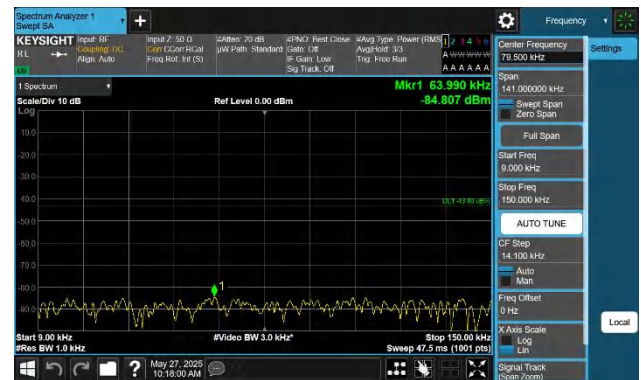
42-42-20MHz-20MHz-QPSK-QPSK-42792-42990-1RB#0-1RB#9 9-0.009~0.15MHz-PASS
