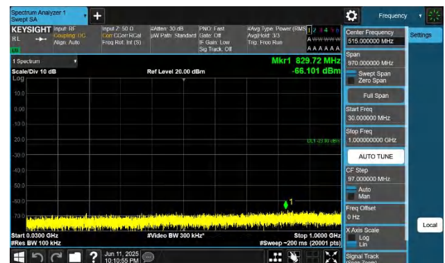
42-42-20MHz-20MHz-QPSK-QPSK-42792-42990-1RB#0-1RB#9 9-30~1000MHz-PASS
