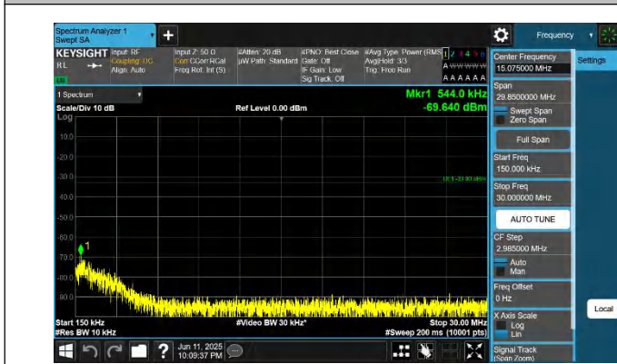
42-42-20MHz-20MHz-QPSK-QPSK-42491-42689-1RB#0-0RB#- 0.15~30MHz-PASS
