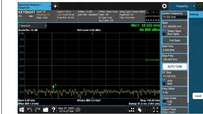
42-42-20MHz-20MHz-QPSK-QPSK-42491-42689-1RB#0-1RB#9 9-0.009~0.15MHz-PASS
