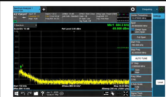
42-42-15MHz-20MHz-QPSK-QPSK-42168-42339-1RB#0-0RB#0- 0.15~30MHz-PASS
