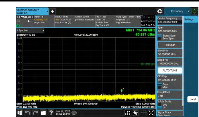
42-42-10MHz-20MHz-QPSK-QPSK-42145-42289-1RB#49-0RB# 0-30~1000MHz-PASS
