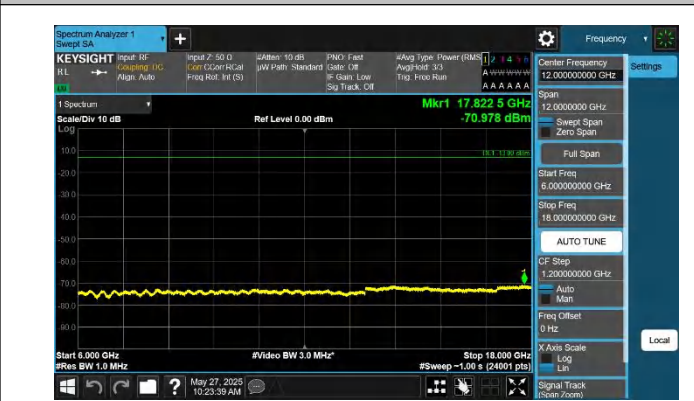
42-42-20MHz-5MHz-QPSK-QPSK-42565-42682-1RB#0-0RB#0-6 000~18000MHz-PASS
