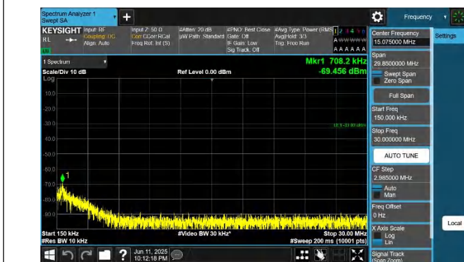
42-42-20MHz-5MHz-QPSK-QPSK-42565-42682-1RB#0-1RB#24- 0.15~30MHz-PASS
