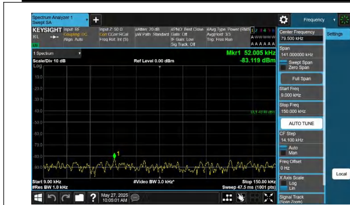
42-42-15MHz-20MHz-QPSK-QPSK-42819-42990-1RB#0-0RB#0- 0.009~0.15MHz-PASS
