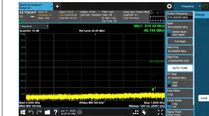
42-42-15MHz-20MHz-QPSK-QPSK-42168-42339-1RB#74-0RB# 0-30~1000MHz-PASS
