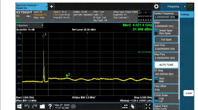
42-42-20MHz-5MHz-QPSK-QPSK-42565-42682-1RB#0-1RB#24- 3000~6000MHz-PASS
