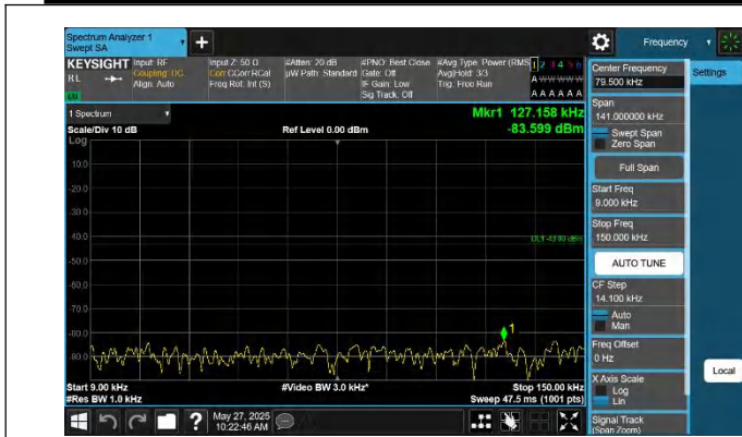
42-42-20MHz-5MHz-QPSK-QPSK-42565-42682-1RB#0-0RB#0-0 .009~0.15MHz-PASS
