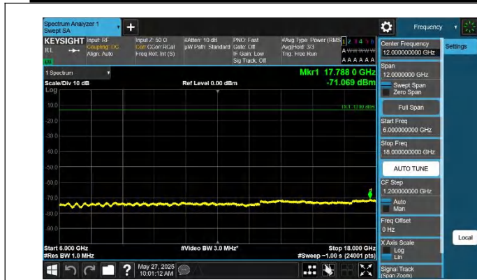
42-42-15MHz-20MHz-QPSK-QPSK-42168-42339-1RB#0-1RB#9 9-6000~18000MHz-PASS
