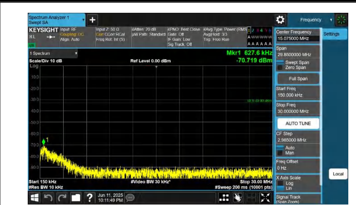
42-42-20MHz-5MHz-QPSK-QPSK-42565-42682-1RB#0-0RB#0-0 .15~30MHz-PASS
