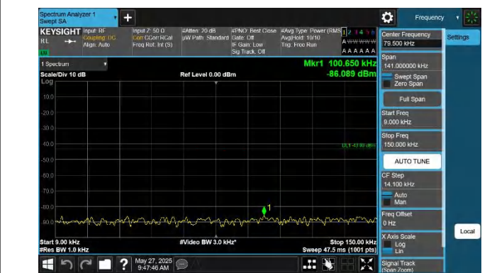
42-42-10MHz-20MHz-QPSK-QPSK-42846-42990-1RB#0-0RB#- 0.009~0.15MHz-PASS
