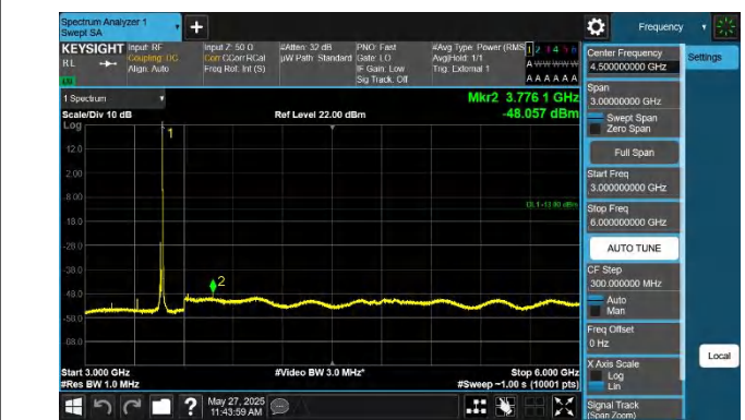
42-42-20MHz-5MHz-QPSK-QPSK-42190-42307-1RB#99-0RB#0-3000~6000MHz-PASS
