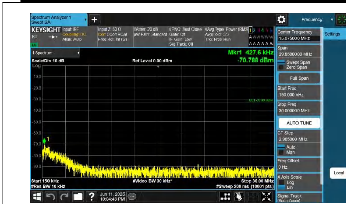
42-42-10MHz-20MHz-QPSK-QPSK-42145-42289-1RB#49-0RB# 0-0.15~30MHz-PASS
