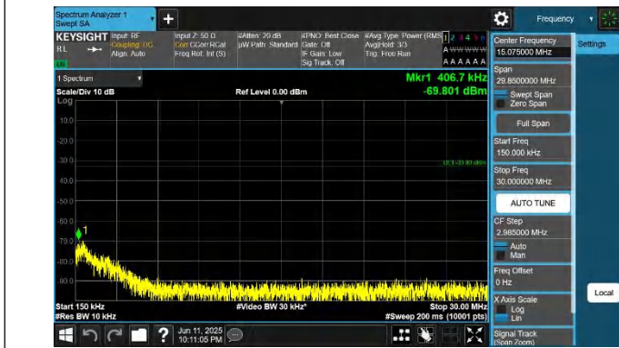
42-42-20MHz-5MHz-QPSK-QPSK-42190-42307-1RB#0-0RB#0-0 .15~30MHz-PASS
