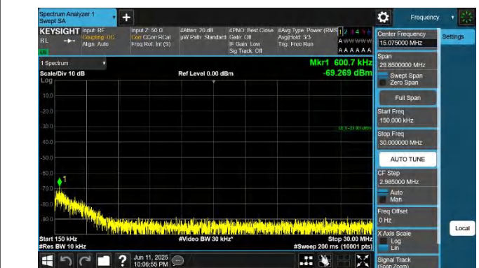
42-42-15MHz-20MHz-QPSK-QPSK-42168-42339-1RB#74-0RB# 0-0.15~30MHz-PASS
