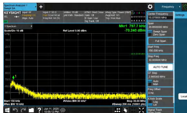
42-42-10MHz-20MHz-QPSK-QPSK-42496-42640-1RB#0-0RB#0- 0.15~30MHz-PASS
