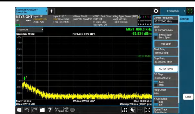
42-42-15MHz-20MHz-QPSK-QPSK-42819-42990-1RB#0-0RB#0- 0.15~30MHz-PASS
