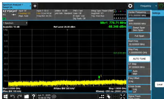
42-42-15MHz-20MHz-QPSK-QPSK-42493-42664-1RB#0-1RB#9 9-30~1000MHz-PASS
