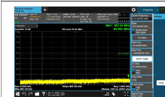
42-42-20MHz-5MHz-QPSK-QPSK-42565-42682-1RB#0-0RB#0-3 0~1000MHz-PASS
