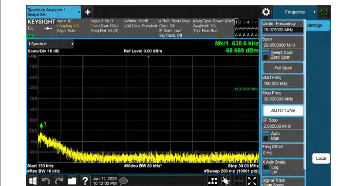
42-42-20MHz-5MHz-QPSK-QPSK-42565-42682-1RB#99-0RB#0- 0.15~30MHz-PASS
