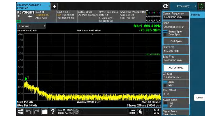
42-42-15MHz-20MHz-QPSK-QPSK-42493-42664-1RB#0-1RB#9 9-0.15~30MHz-PASS
