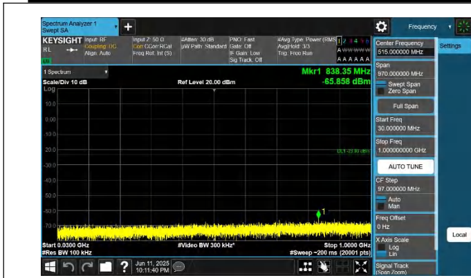
42-42-20MHz-5MHz-QPSK-QPSK-42190-42307-1RB#0-1RB#24- 30~1000MHz-PASS
