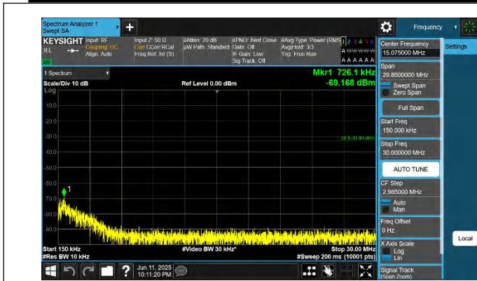
42-42-20MHz-5MHz-QPSK-QPSK-42190-42307-1RB#99-0RB#0-0.15~30MHz-PASS
