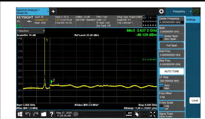
42-42-15MHz-20MHz-QPSK-QPSK-42493-42664-1RB#0-0RB#0- 3000~6000MHz-PASS
