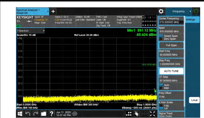
42-42-15MHz-20MHz-QPSK-QPSK-42493-42664-1RB#74-0RB# 0-30~1000MHz-PASS
