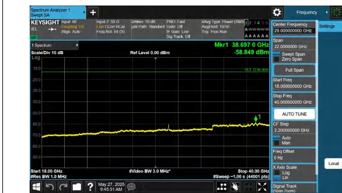
42-42-10MHz-20MHz-QPSK-QPSK-42496-42640-1RB#49-0RB# 0-18000~40000MHz-PASS
