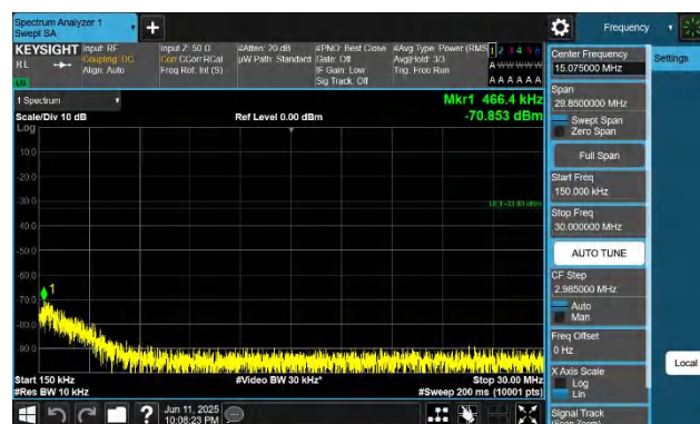
42-42-15MHz-20MHz-QPSK-QPSK-42819-42990-1RB#74-0RB# 0-0.15~30MHz-PASS
