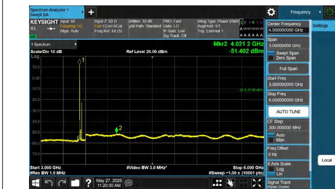
42-42-10MHz-20MHz-QPSK-QPSK-42846-42990-1RB#0-1RB#9 9-3000~6000MHz-PASS
