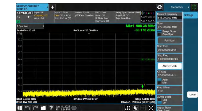
42-42-20MHz-5MHz-QPSK-QPSK-42565-42682-1RB#0-1RB#24- 30~1000MHz-PASS
