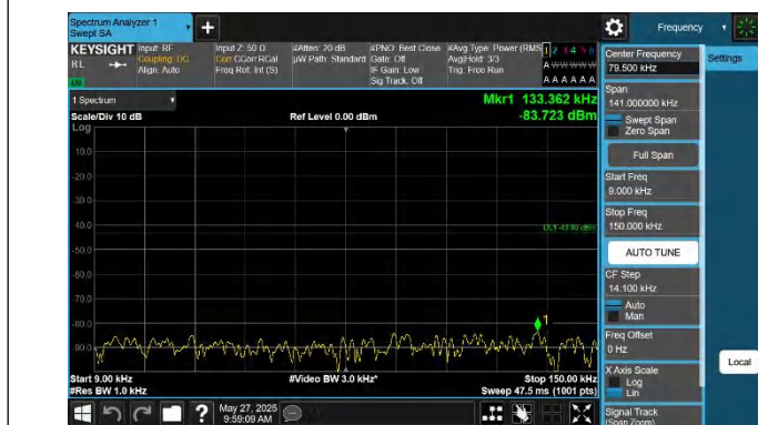
42-42-15MHz-20MHz-QPSK-QPSK-42168-42339-1RB#74-0RB# 0-0.009~0.15MHz-PASS
