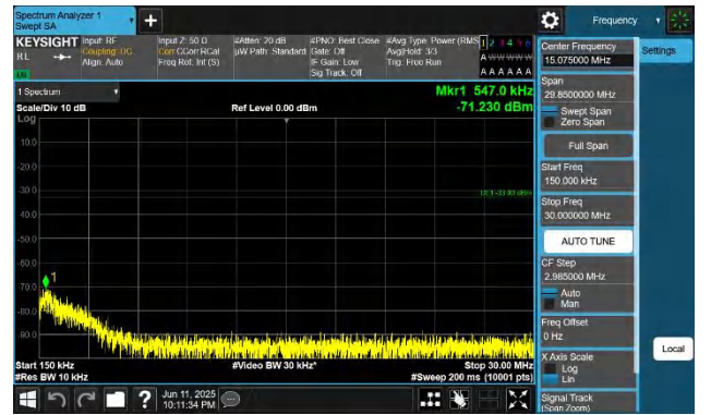
42-42-20MHz-5MHz-QPSK-QPSK-42190-42307-1RB#0-1RB#24- 0.15~30MHz-PASS
