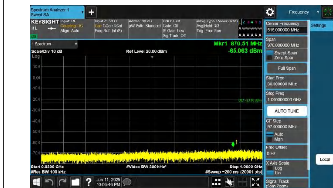
42-42-15MHz-20MHz-QPSK-QPSK-42168-42339-1RB#0-0RB#0- 30~1000MHz-PASS
