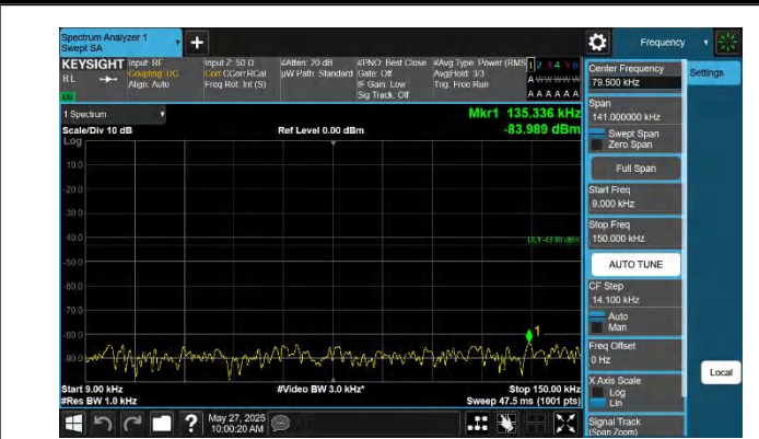
42-42-15MHz-20MHz-QPSK-QPSK-42168-42339-1RB#0-1RB#9-9-0.009~0.15MHz-PASS
