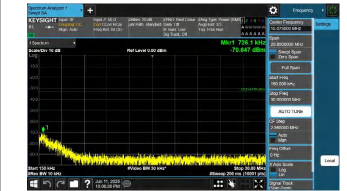
42-42-10MHz-20MHz-QPSK-QPSK-42846-42990-1RB#0-1RB#9 9-0.15~30MHz-PASS
