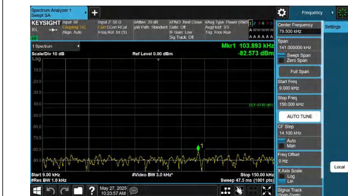
42-42-20MHz-5MHz-QPSK-QPSK-42565-42682-1RB#99-0RB#0- 0.009~0.15MHz-PASS
