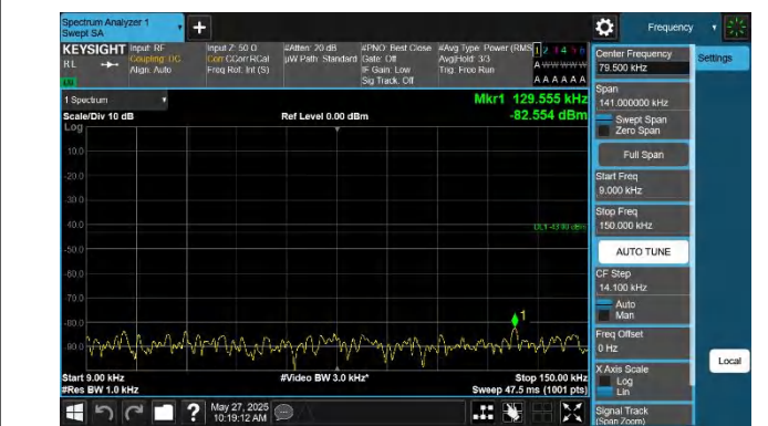
42-42-20MHz-5MHz-QPSK-QPSK-42190-42307-1RB#0-0RB#0-0 .009~0.15MHz-PASS
