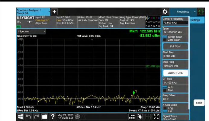
42-42-20MHz-5MHz-QPSK-QPSK-42565-42682-1RB#0-1RB#24- 0.009~0.15MHz-PASS
