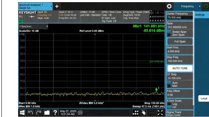
42-42-10MHz-20MHz-QPSK-QPSK-42846-42990-1RB#0-1RB#9 9-0.009~0.15MHz-PASS
