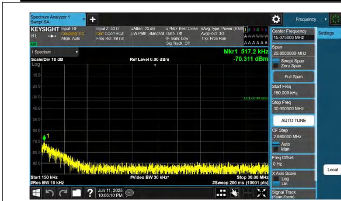
42-42-10MHz-20MHz-QPSK-QPSK-42846-42990-1RB#49-0RB# 0-0.15~30MHz-PASS
