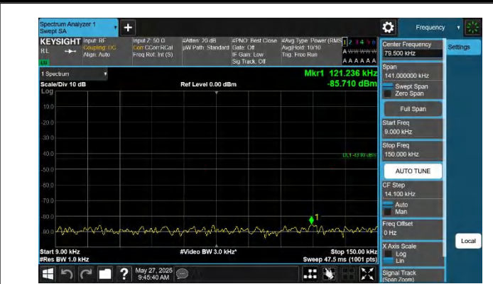
42-42-10MHz-20MHz-QPSK-QPSK-42496-42640-1RB#0-1RB#9 9-0.009~0.15MHz-PASS
