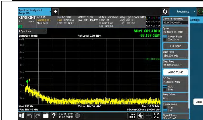
42-42-15MHz-20MHz-QPSK-QPSK-42493-42664-1RB#74-0RB# 0-0.15~30MHz-PASS
