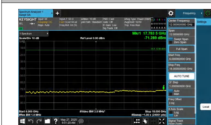
42-42-10MHz-20MHz-QPSK-QPSK-42846-42990-1RB#49-0RB# 0-6000~18000MHz-PASS
