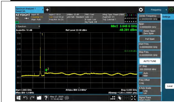
42-42-10MHz-20MHz-QPSK-QPSK-42496-42640-1RB#49-0RB# 0-3000~6000MHz-PASS
