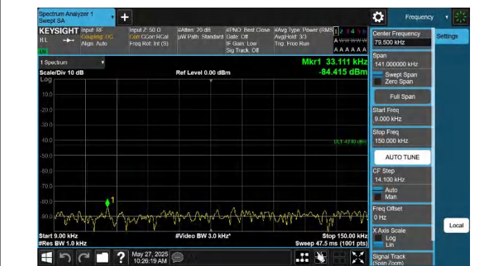
42-42-20MHz-5MHz-QPSK-QPSK-42940-43057-1RB#0-0RB#0-0 .009~0.15MHz-PASS
