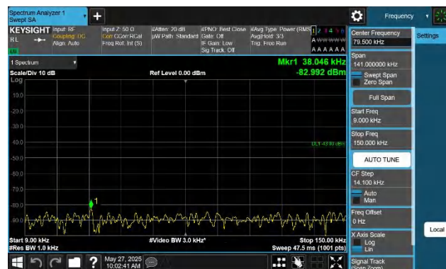
42-42-15MHz-20MHz-QPSK-QPSK-42493-42664-1RB#74-0RB# 0-0.009~0.15MHz-PASS
