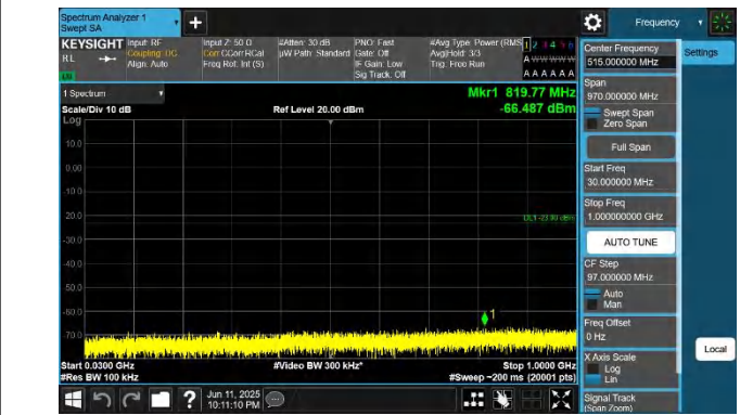
42-42-20MHz-5MHz-QPSK-QPSK-42190-42307-1RB#0-0RB#0-0 0~1000MHz-PASS
