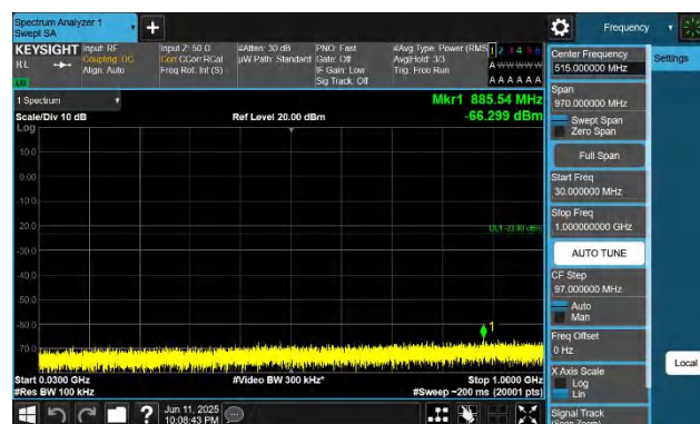
42-42-15MHz-20MHz-QPSK-QPSK-42819-42990-1RB#0-1RB#9 9-30~1000MHz-PASS
