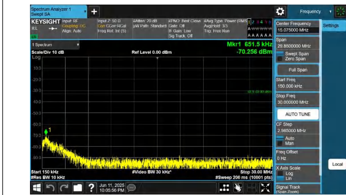
42-42-10MHz-20MHz-QPSK-QPSK-42846-42990-1RB#0-0RB#- 0.15~30MHz-PASS
