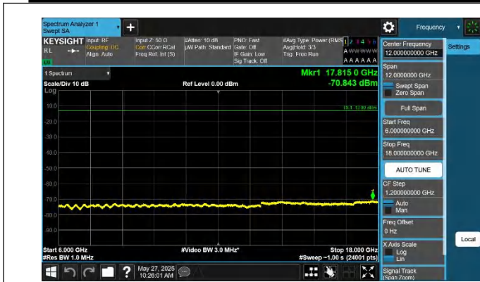
42-42-20MHz-5MHz-QPSK-QPSK-42565-42682-1RB#0-1RB#24- 6000~18000MHz-PASS
