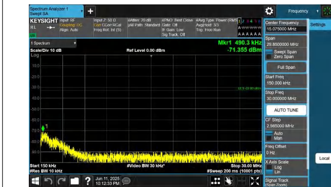
42-42-20MHz-5MHz-QPSK-QPSK-42940-43057-1RB#0-0RB#0-0 .15~30MHz-PASS
