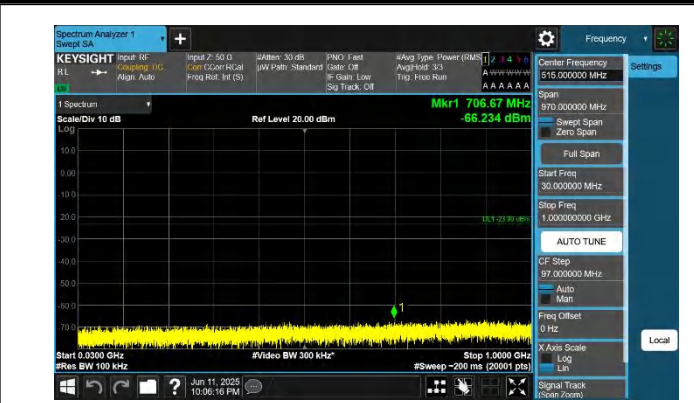
42-42-10MHz-20MHz-QPSK-QPSK-42846-42990-1RB#49-0RB# 0-30~1000MHz-PASS
