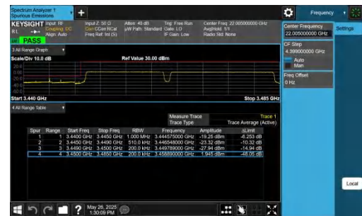
42-42-15MHz-20MHz-QPSK@QPSK-QPSK@QPSK-42168-42339 -75RB#0@75RB#0-100RB#0@100RB#0-PASS
