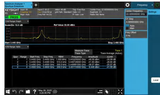
42-42-20MHz-10MHz-QPSK@QPSK-QPSK@QPSK-42190-42334-1RB#0@100RB#0-1RB#49@50RB#0-PASS
