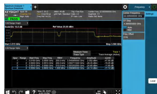
42-42-20MHz-15MHz-QPSK@QPSK-QPSK@QPSK-42841-43012 -100RB#0@100RB#0-75RB#0@75RB#0-PASS
