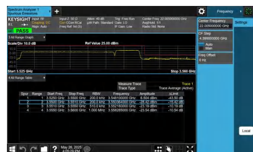
42-42-20MHz-5MHz-QPSK@QPSK-QPSK@QPSK-42940-43057-100RB#0@100RB#0-25RB#0@25RB#0-PASS
