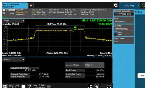
42-42-20MHz-5MHz-QPSK-QPSK-42565-42682-100RB#0-25RB# 0-PASS
