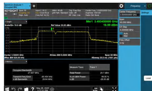
42-42-10MHz-20MHz-16QAM-16QAM-42496-42640-50RB#0-100RB#0-PASS
