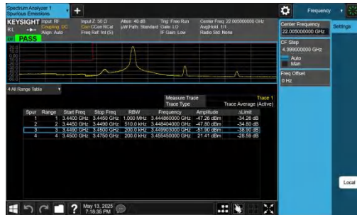
42-42-5MHz-20MHz-QPSK@QPSK-QPSK@QPSK-42123-4224 0-1RB#24@25RB#0-0RB#0@100RB#0-PASS
