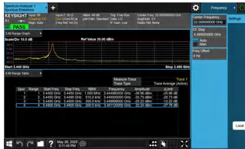
42-42-20MHz-20MHz-QPSK@QPSK-QPSK@QPSK-42190-42388-1RB#0@100RB#0-0RB#0@100RB#0-PASS
