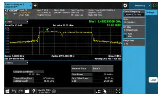
42-42-15MHz-20MHz-16QAM-16QAM-42493-42664-75RB#0-10 0RB#0-PASS
