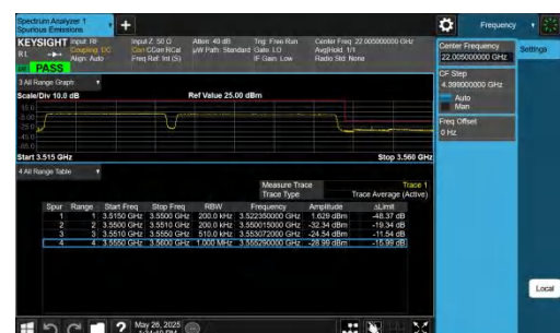
42-42-15MHz-20MHz-QPSK@QPSK-QPSK@QPSK-42819-42990 -75RB#0@75RB#0-100RB#0@100RB#0-PASS
