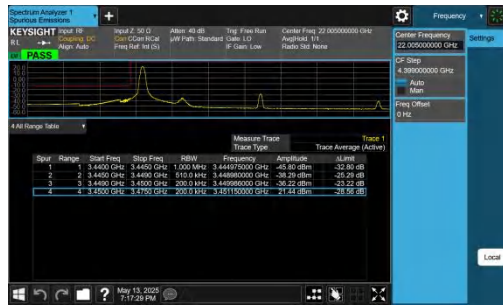
42-42-5MHz-20MHz-QPSK@QPSK-QPSK@QPSK-42123-4224 0-1RB#0@25RB#0-0RB#0@100RB#0-PASS
