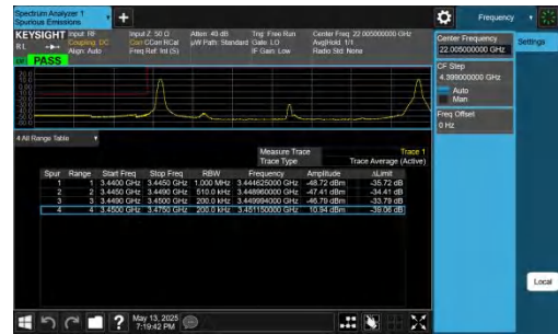
42-42-5MHz-20MHz-QPSK@QPSK-QPSK@QPSK-42123-42240- 1RB#0@25RB#0-1RB#99@100RB#0-PASS
