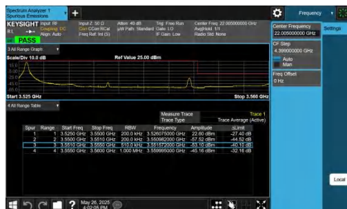
42-42-20MHz-5MHz-QPSK@QPSK-QPSK@QPSK-42940-43057-1RB#0@100RB#0-0RB#0@25RB#0-PASS
