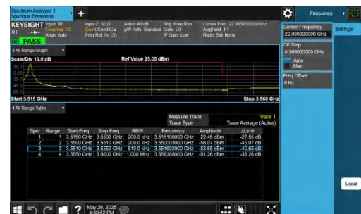
42-42-20MHz-15MHz-QPSK@QPSK-QPSK@QPSK-42841-43012 -1RB#0@100RB#0-0RB#75RB#0-PASS
