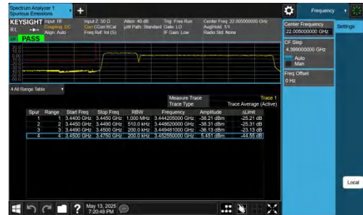
42-42-5MHz-20MHz-QPSK@QPSK-QPSK@QPSK-42123-42240- 25RB#0@25RB#0-100RB#0@100RB#0-PASS
