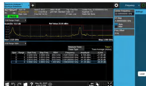
42-42-20MHz-5MHz-QPSK@QPSK-QPSK@QPSK-42940-43057-1RB#0@100RB#0-1RB#24@25RB#0-PASS
