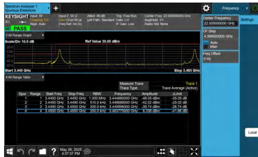
42-42-20MHz-15MHz-QPSK@QPSK-QPSK@QPSK-42190-423 61-1RB#0@99RB#0-1RB#74@75RB#0-PASS
