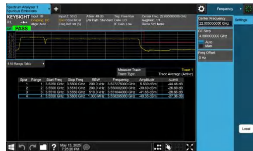
42-42-5MHz-20MHz-QPSK@QPSK-QPSK@QPSK-42873-42990- 25RB#0@25RB#0-100RB#0@100RB#0-PASS
