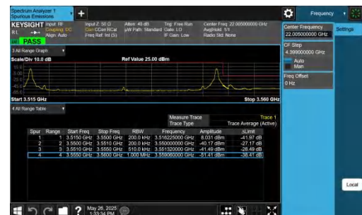
42-42-15MHz-20MHz-QPSK@QPSK-QPSK@QPSK-42819-42990 -1RB#0@75RB#0-1RB#99@100RB#0-PASS
