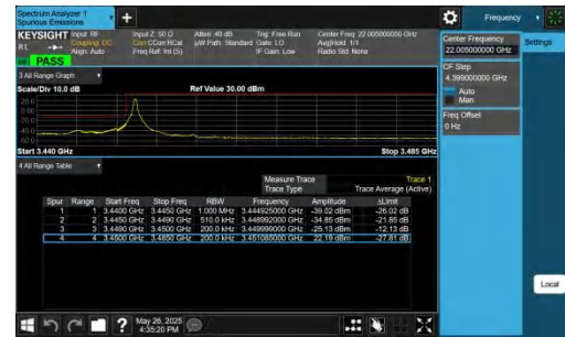
42-42-20MHz-15MHz-QPSK@QPSK-QPSK@QPSK-42190-42361 -1RB#0@100RB#0-0RB#75RB#0-PASS
