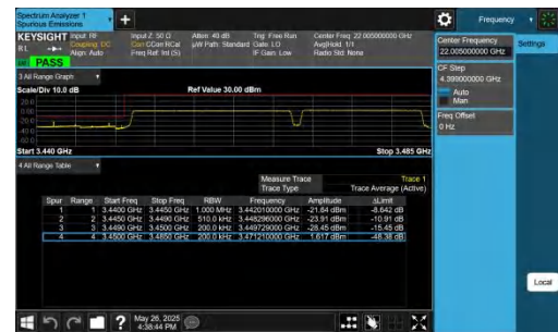
42-42-20MHz-15MHz-QPSK@QPSK-QPSK@QPSK-42190-42361 -100RB#0@100RB#0-75RB#0@75RB#0-PASS
