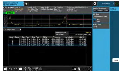
42-42-5MHz-20MHz-QPSK@QPSK-QPSK@QPSK-42873-42990- 1RB#0@25RB#0-1RB#99@100RB#0-PASS
