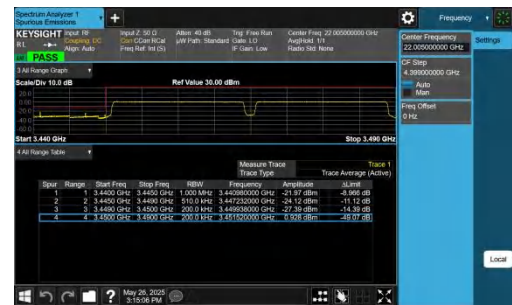
42-42-20MHz-20MHz-QPSK@QPSK-QPSK@QPSK-42190-42388-100RB#0@100RB#0-100RB#0@100RB#0-PASS
