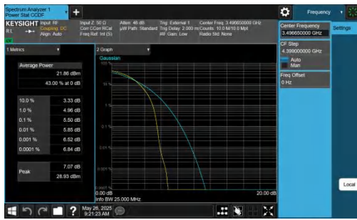
42-42-5MHz-20MHz-QPSK-QPSK-42498-42615-25RB#0-100RB#0-PASS
