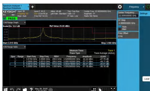
42-42-15MHz-20MHz-QPSK@QPSK-QPSK@QPSK-42819-429 90-1RB#74@75RB#0-0RB#0@100RB#0-PASS
