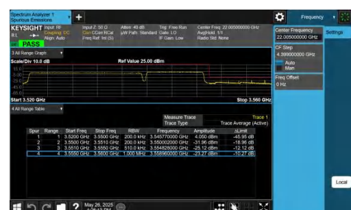
42-42-20MHz-10MHz-QPSK@QPSK-QPSK@QPSK-42891-43035-100RB#0@100RB#0-50RB#0@50RB#0-PASS
