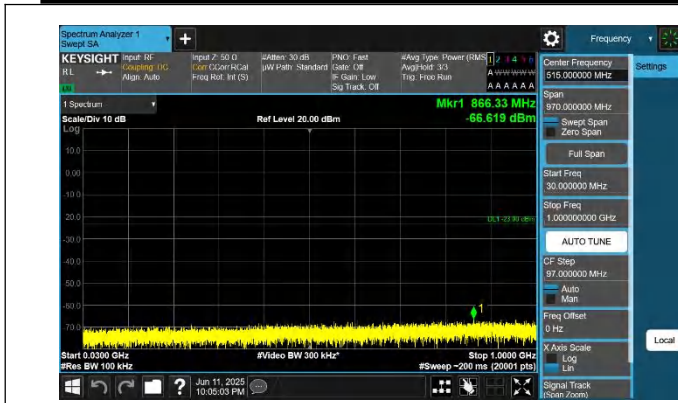
42-42-10MHz-20MHz-QPSK-QPSK-42145-42289-1RB#0-1RB#9 9-30~1000MHz-PASS
