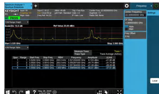
42-42-20MHz-10MHz-QPSK@QPSK-QPSK@QPSK-42891-43035-1RB#0@100RB#0-1RB#49@50RB#0-PASS
