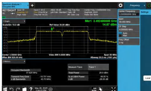
42-42-20MHz-20MHz-256QAM-256QAM-42491-42689-100RB#0-1 00RB#0-PASS
