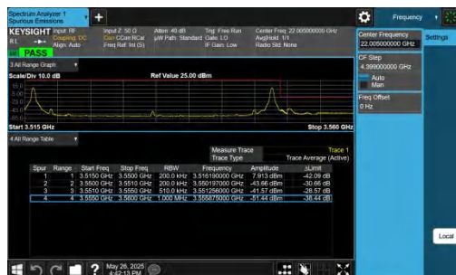
42-42-20MHz-15MHz-QPSK@QPSK-QPSK@QPSK-42841-430 12-1RB#0@99RB#0-1RB#74@75RB#0-PASS
