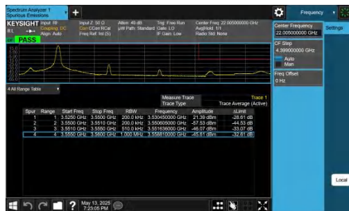
42-42-5MHz-20MHz-QPSK@QPSK-QPSK@QPSK-42873-4299 0-1RB#24@25RB#0-0RB#0@100RB#0-PASS
