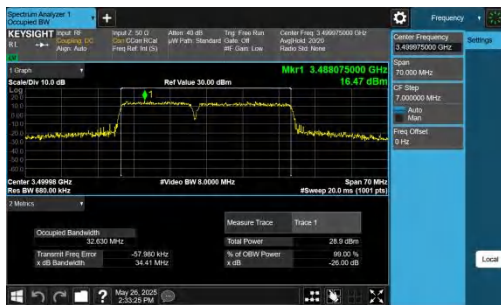
42-42-15MHz-20MHz-256QAM-256QAM-42493-42664-75RB#0-10 0RB#0-PASS
