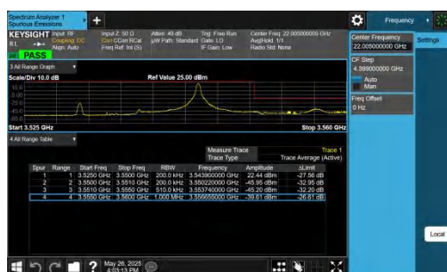
42-42-20MHz-5MHz-QPSK@QPSK-QPSK@QPSK-42940-43057-1RB#99@100RB#0-0RB#0@25RB#0-PASS
