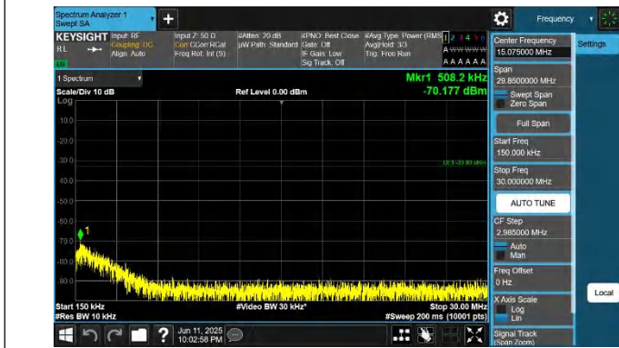
42-42-5MHz-20MHz-QPSK-QPSK-42498-42615-1RB#0-0RB#0-0 .15~30MHz-PASS
