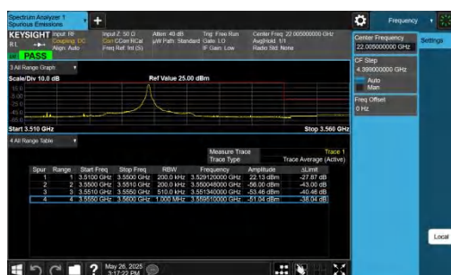
42-42-20MHz-20MHz-QPSK@QPSK-QPSK@QPSK-42792-42990-90-1RB#99@100RB#0-0RB#0@100RB#0-PASS
