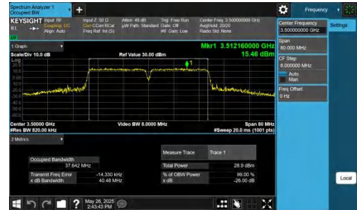
42-42-20MHz-20MHz-64QAM-64QAM-42491-42689-100RB#0-1 00RB#0-PASS
