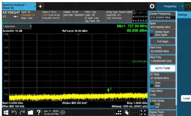
42-42-5MHz-20MHz-QPSK-QPSK-42498-42615-1RB#0-1RB#99- 30~1000MHz-PASS
