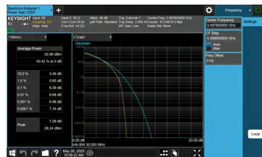
42-42-10MHz-20MHz-16QAM-16QAM-42496-42640-50RB#0-100RB#0-PASS
