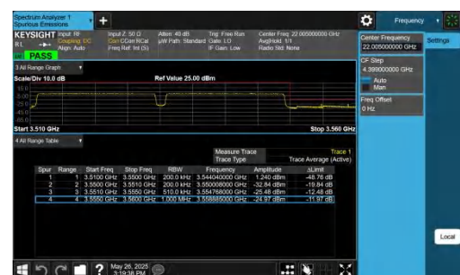
42-42-20MHz-20MHz-QPSK@QPSK-QPSK@QPSK-42792-42990-100RB#0@100RB#0-100RB#0@100RB#0-PASS
