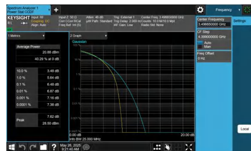
42-42-5MHz-20MHz-16QAM-16QAM-42498-42615-25RB#0-100RB#0-PASS
