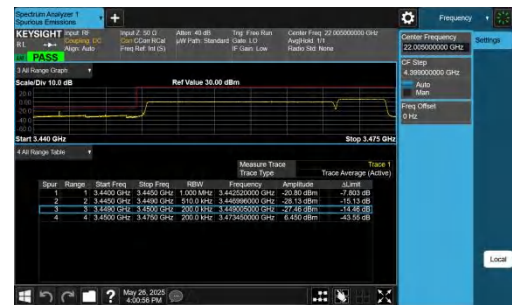
42-42-20MHz-5MHz-QPSK@QPSK-QPSK@QPSK-42190-42307-100RB#0@100RB#0-25RB#0@25RB#0-PASS
