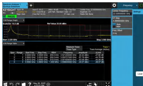
42-42-20MHz-10MHz-QPSK@QPSK-QPSK@QPSK-42891-43035-1RB#0@100RB#0-0RB#0@50RB#0-PASS
