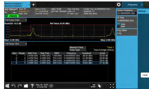
42-42-20MHz-20MHz-QPSK@QPSK-QPSK@QPSK-42190-42388-1RB#0@100RB#0-1RB#99@100RB#0-PASS
