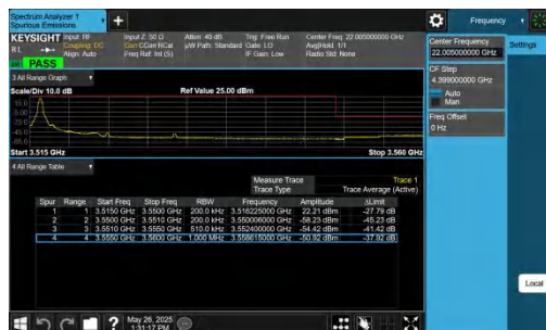
42-42-15MHz-20MHz-QPSK@QPSK-QPSK@QPSK-42819-429 90-1RB#0@75RB#0-0RB#0@100RB#0-PASS
