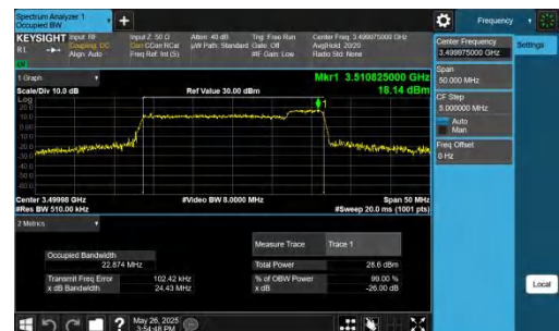
42-42-20MHz-5MHz-64QAM-64QAM-42565-42682-100RB#0-25 RB#0-PASS
