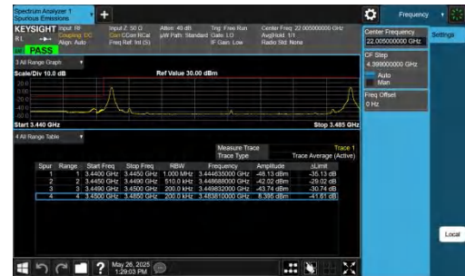
42-42-15MHz-20MHz-QPSK@QPSK-QPSK@QPSK-42168-42339 -1RB#0@75RB#0-1RB#99@100RB#0-PASS
