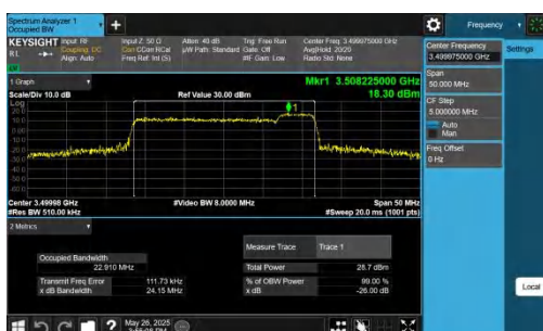
42-42-20MHz-5MHz-256QAM-256QAM-42565-42682-100RB#0-25 RB#0-PASS
