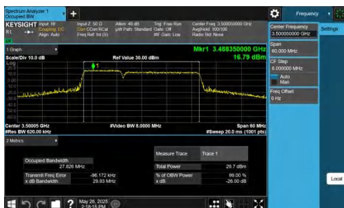
42-42-10MHz-20MHz-256QAM-256QAM-42496-42640-50RB#0-100RB#0-PASS
