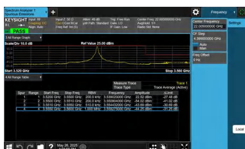
42-42-20MHz-10MHz-QPSK@QPSK-QPSK@QPSK-42891-43035-1RB#99@100RB#0-0RB#0@50RB#0-PASS
