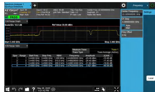
42-42-20MHz-10MHz-QPSK@QPSK-QPSK@QPSK-42190-42334-100RB#0@100RB#0-50RB#0@50RB#0-PASS
