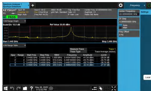
42-42-20MHz-20MHz-QPSK@QPSK-QPSK@QPSK-42190-42388-1RB#99@100RB#0-0RB#0@100RB#0-PASS
