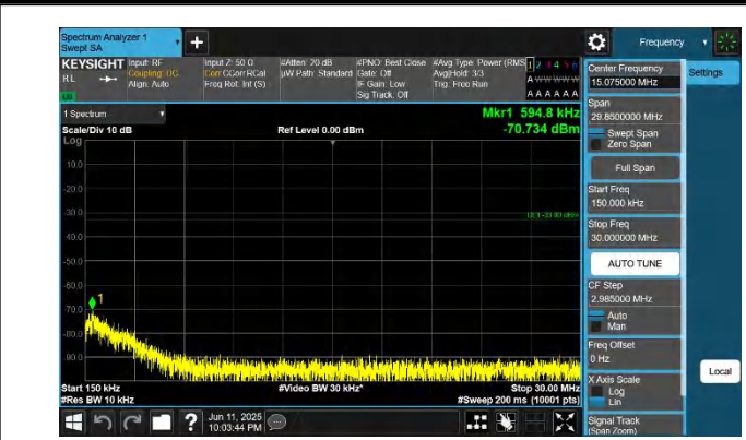
42-42-5MHz-20MHz-QPSK-QPSK-42873-42990-1RB#0-0RB#0-0 .15~30MHz-PASS
