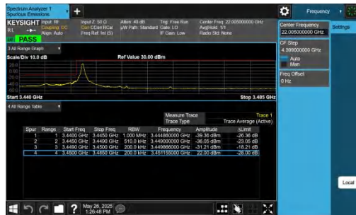
42-42-15MHz-20MHz-QPSK@QPSK-QPSK@QPSK-42168-423 39-1RB#0@75RB#0-0RB#0@100RB#0-PASS
