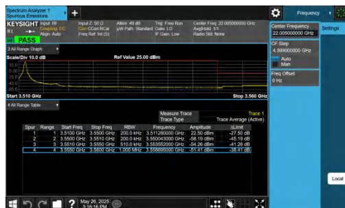
42-42-20MHz-20MHz-QPSK@QPSK-QPSK@QPSK-42792-42990-90-1RB#0@100RB#0-0RB#0@100RB#0-PASS
