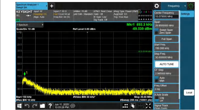
42-42-5MHz-20MHz-QPSK-QPSK-42498-42615-1RB#0-1RB#99- 0.15~30MHz-PASS
