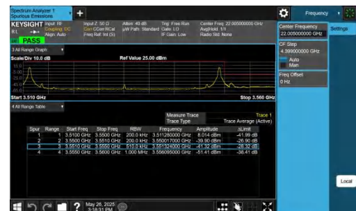
42-42-20MHz-20MHz-QPSK@QPSK-QPSK@QPSK-42792-42990-1RB#0@100RB#0-1RB#99@100RB#0-PASS
