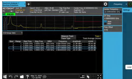
42-42-5MHz-20MHz-QPSK@QPSK-QPSK@QPSK-42873-4299 0-1RB#0@25RB#0-0RB#0@100RB#0-PASS
