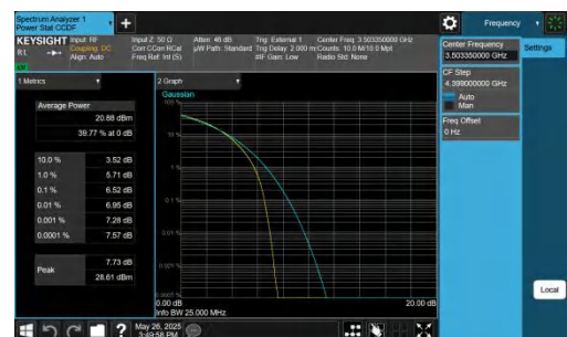
42-42-20MHz-5MHz-16QAM-16QAM-42565-42682-100RB#0-25 RB#0-PASS
