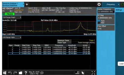
42-42-20MHz-5MHz-QPSK@QPSK-QPSK@QPSK-42190-42307-1RB#99@100RB#0-0RB#0@25RB#0-PASS
