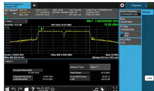
42-42-20MHz-20MHz-16QAM-16QAM-42491-42689-100RB#0-1 00RB#0-PASS
