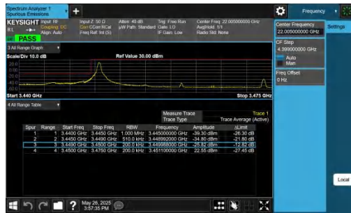
42-42-20MHz-5MHz-QPSK@QPSK-QPSK@QPSK-42190-42307-1RB#0@100RB#0-0RB#0@25RB#0-PASS
