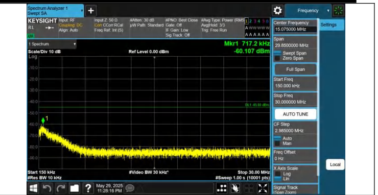
41-41-20MHz-20MHz-QPSK-QPSK-39750-39948-1RB#0-1RB#99 -0.15~30MHz-PASS
