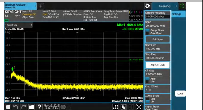
41-41-20MHz-15MHz-QPSK-QPSK-41341-41512-1RB#0-1RB#74 -0.15~30MHz-PASS
