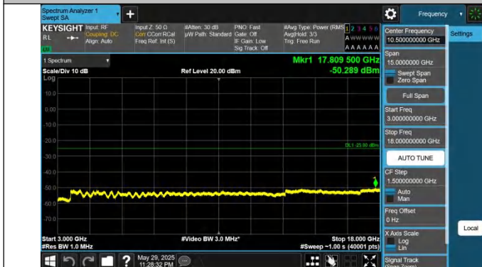
41-41-20MHz-20MHz-QPSK-QPSK-39750-39948-1RB#0-1RB#9 9-3000~18000MHz-PASS
