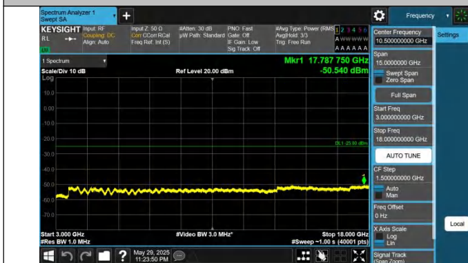
41-41-20MHz-15MHz-QPSK-QPSK-40546-40717-1RB#99-0RB# 0-3000~18000MHz-PASS
