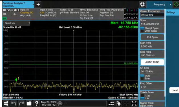
41-41-20MHz-15MHz-QPSK-QPSK-40546-40717-1RB#0-1RB#74-0.009~0.15MHz-PASS
