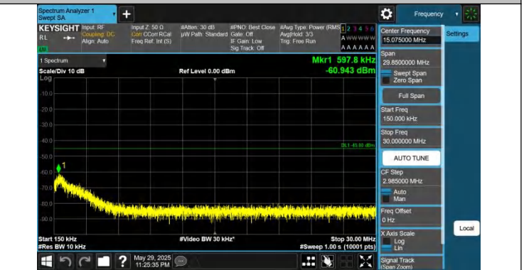
41-41-20MHz-15MHz-QPSK-QPSK-41341-41512-1RB#99-0RB#0 -0.15~30MHz-PASS
