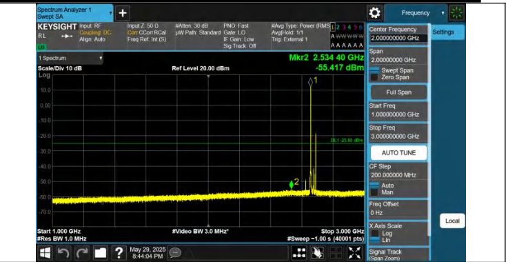
41-41-20MHz-15MHz-QPSK-QPSK-41341-41512-1RB#0-1RB#74 -1000~3000MHz-PASS
