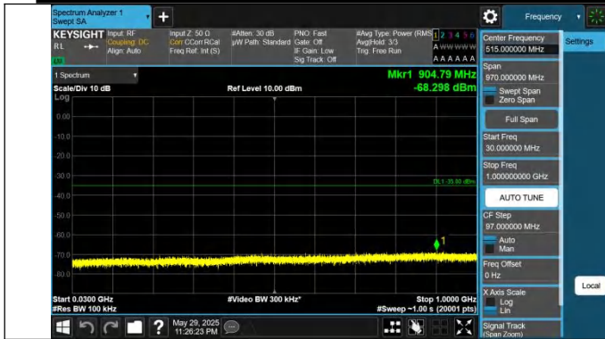
41-41-20MHz-15MHz-QPSK-QPSK-41341-41512-1RB#0-1RB#7 4-30~1000MHz-PASS
