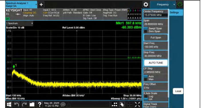
41-41-20MHz-15MHz-QPSK-QPSK-40546-40717-1RB#0-1RB#74-0.15~30MHz-PASS
