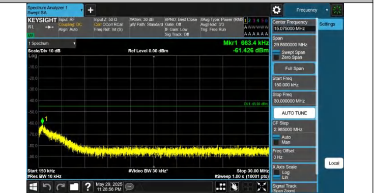
41-41-20MHz-20MHz-QPSK-QPSK-40521-40719-1RB#0-0RB#0- 0.15~30MHz-PASS
