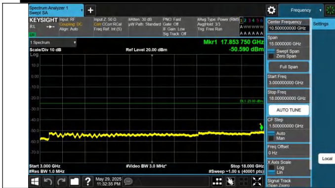
41-41-20MHz-20MHz-QPSK-QPSK-41292-41490-1RB#0-1RB#9 9-3000~18000MHz-PASS
