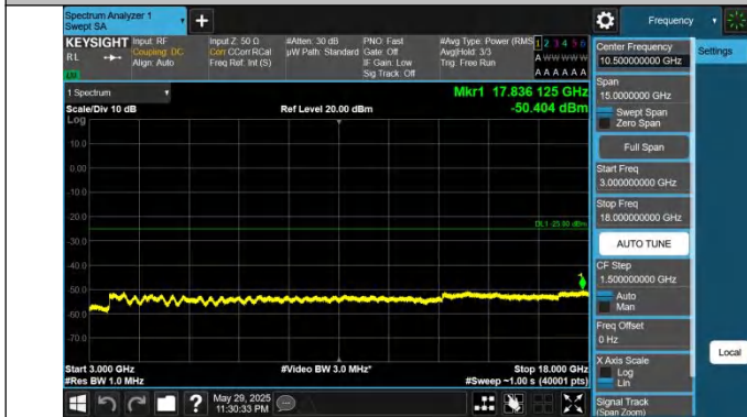
41-41-20MHz-20MHz-QPSK-QPSK-40521-40719-1RB#0-1RB#9-9-3000~18000MHz-PASS
