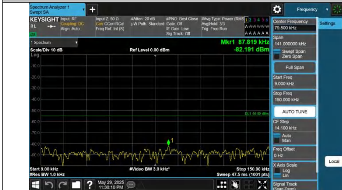
41-41-20MHz-20MHz-QPSK-QPSK-40521-40719-1RB#0-1RB#9-9-0.009~0.15MHz-PASS
