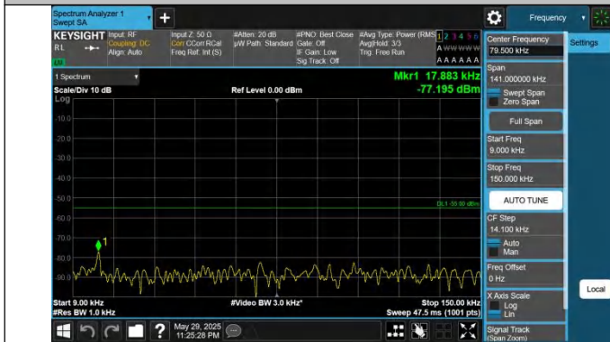
41-41-20MHz-15MHz-QPSK-QPSK-41341-41512-1RB#99-0RB# 0-0.009~0.15MHz-PASS
