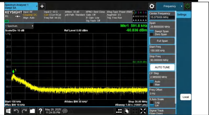
41-41-20MHz-15MHz-QPSK-QPSK-41341-41512-1RB#0-0RB#0- 0.15~30MHz-PASS
