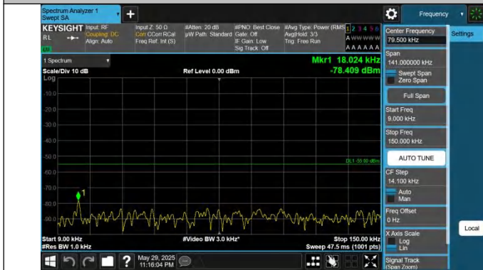
41-41-20MHz-10MHz-QPSK-QPSK-39750-39894-1RB#0-1RB#49-0.009~0.15MHz-PASS
