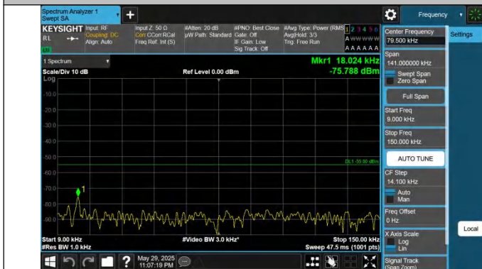
41-41-15MHz-20MHz-QPSK-QPSK-41319-41490-1RB#0-1RB#99-9-0.009~0.15MHz-PASS
