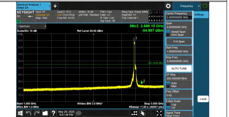
41-41-15MHz-20MHz-QPSK-QPSK-40523-40694-75RB#0-100RB #0-1000~3000MHz-PASS
