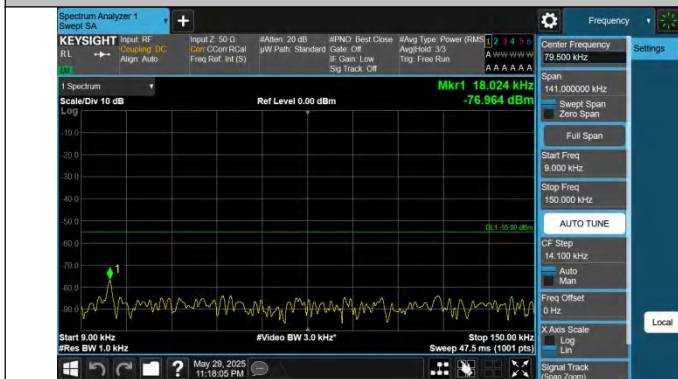
41-41-20MHz-10MHz-QPSK-QPSK-40571-40715-1RB#0-1RB#4 9-0.009~0.15MHz-PASS
