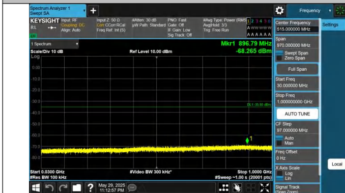
41-41-20MHz-5MHz-QPSK-QPSK-41440-41557-1RB#0-0RB#0-30~1000MHz-PASS
