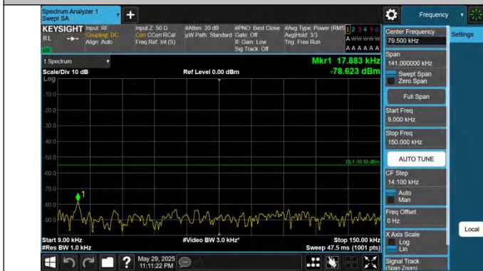
41-41-20MHz-5MHz-QPSK-QPSK-40595-40712-1RB#99-0RB#0-0.009~0.15MHz-PASS
