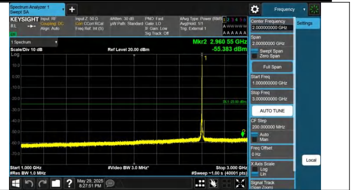
41-41-20MHz-5MHz-QPSK-QPSK-40595-40712-1RB#99-0RB#0-1000~3000MHz-PASS
