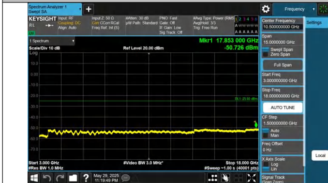
41-41-20MHz-10MHz-QPSK-QPSK-41391-41535-1RB#99-0RB# 0-3000~18000MHz-PASS
