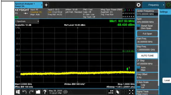
41-41-20MHz-15MHz-QPSK-QPSK-39750-39921-1RB#0-1RB#74-30~1000MHz-PASS
