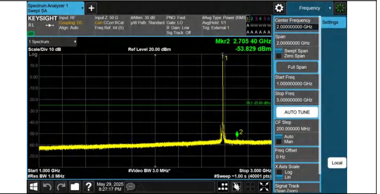
41-41-20MHz-5MHz-QPSK-QPSK-40595-40712-1RB#0-0RB#0-1000~3000MHz-PASS
