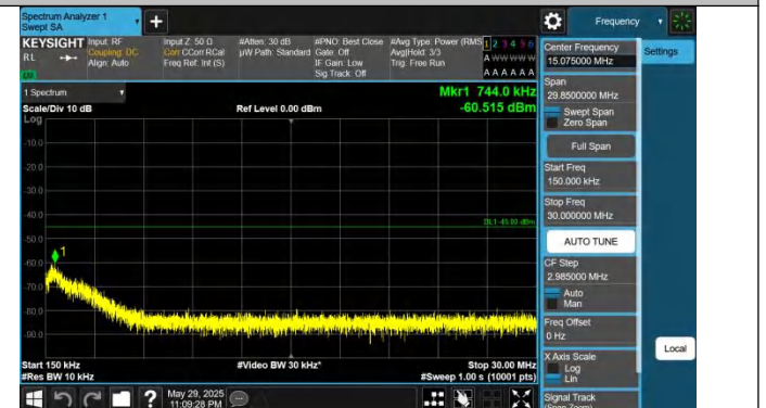
41-41-20MHz-5MHz-QPSK-QPSK-39750-39867-1RB#99-0RB#0-0.15~30MHz-PASS
