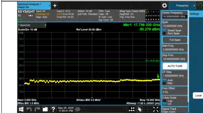
41-41-15MHz-20MHz-QPSK-QPSK-40523-40694-75RB#0-100R B#0-3000~18000MHz-PASS
