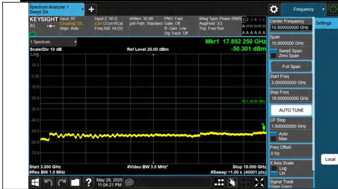
41-41-15MHz-20MHz-QPSK-QPSK-40523-40694-1RB#74-0RB# 0-3000~18000MHz-PASS
