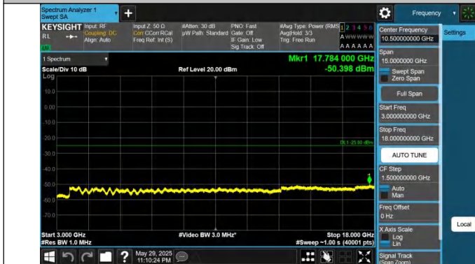
41-41-20MHz-5MHz-QPSK-QPSK-39750-39867-1RB#0-1RB#24-3000~18000MHz-PASS
