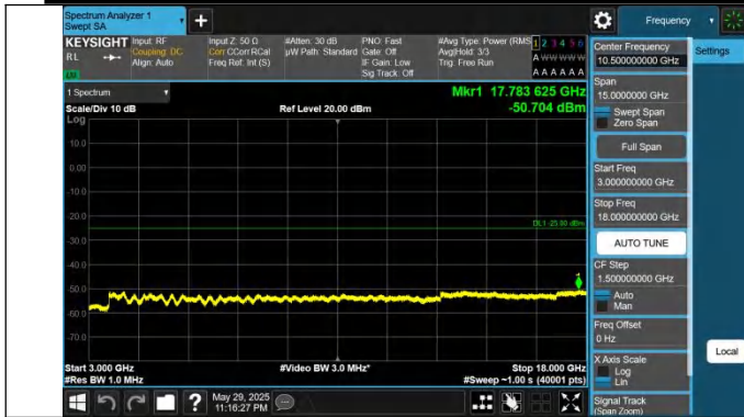
41-41-20MHz-10MHz-QPSK-QPSK-39750-39894-1RB#0-1RB#4 9-3000~18000MHz-PASS
