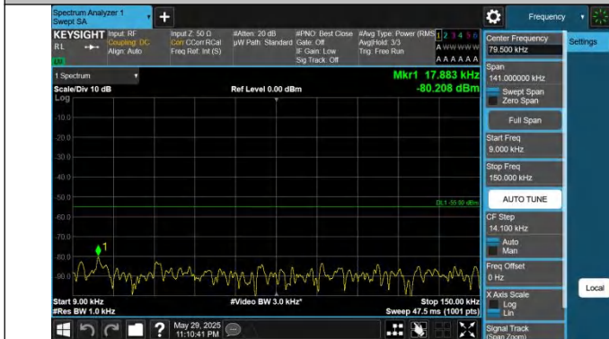
41-41-20MHz-5MHz-QPSK-QPSK-40595-40712-1RB#0-0RB#0-0.009~0.15MHz-PASS
