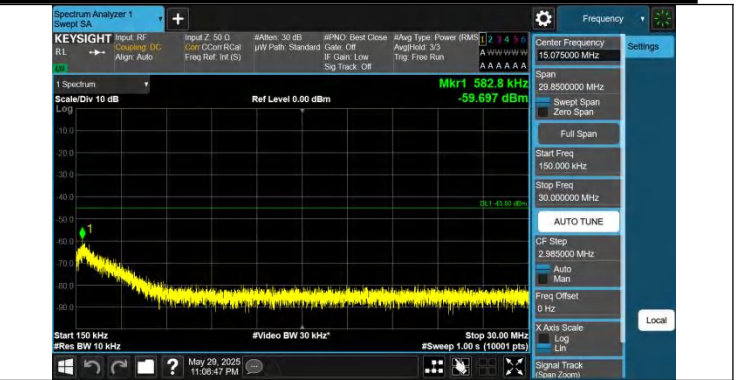
41-41-20MHz-5MHz-QPSK-QPSK-39750-39867-1RB#0-0RB#0-0.15~30MHz-PASS
