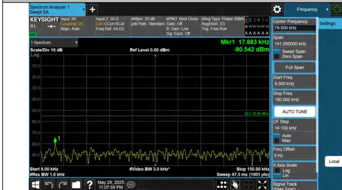
41-41-15MHz-20MHz-QPSK-QPSK-41319-41490-75RB#0-100R B#0-0.009~0.15MHz-PASS
