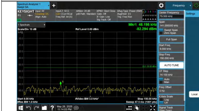
41-41-20MHz-5MHz-QPSK-QPSK-41440-41557-1RB#0-1RB#24- 0.009~0.15MHz-PASS
