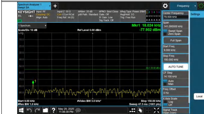
41-41-15MHz-20MHz-QPSK-QPSK-41319-41490-1RB#74-0RB# 0-0.009~0.15MHz-PASS
