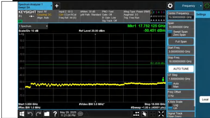
41-41-20MHz-15MHz-QPSK-QPSK-39750-39921-1RB#0-0RB#0-3000~18000MHz-PASS
