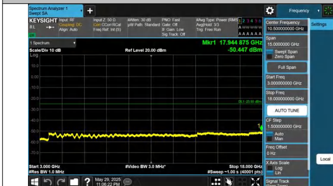
41-41-15MHz-20MHz-QPSK-QPSK-41319-41490-1RB#0-0RB#0-3000~18000MHz-PASS
