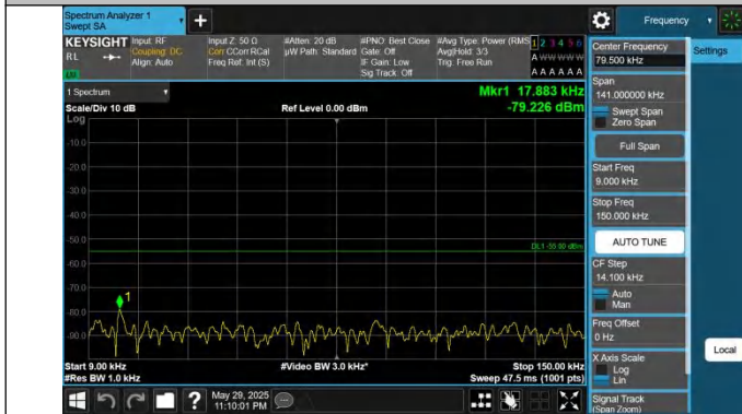
41-41-20MHz-5MHz-QPSK-QPSK-39750-39867-1RB#0-1RB#24-0.009~0.15MHz-PASS
