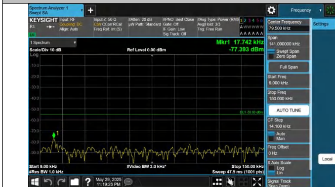
41-41-20MHz-10MHz-QPSK-QPSK-41391-41535-1RB#99-0RB# 0-0.009~0.15MHz-PASS
