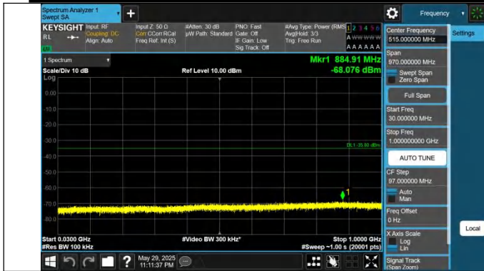
41-41-20MHz-5MHz-QPSK-QPSK-40595-40712-1RB#99-0RB#0-30~1000MHz-PASS
