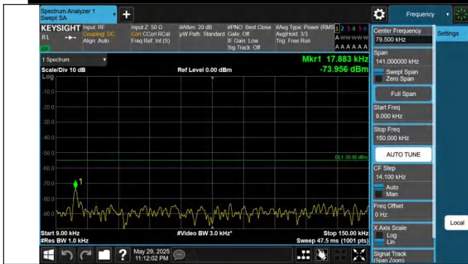
41-41-20MHz-5MHz-QPSK-QPSK-40595-40712-1RB#0-1RB#24-0.009~0.15MHz-PASS
