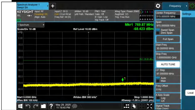
41-41-20MHz-10MHz-QPSK-QPSK-41391-41535-1RB#99-0RB# 0-30~1000MHz-PASS
