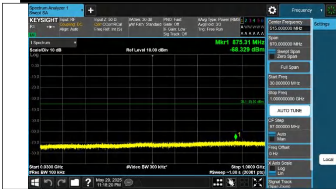
41-41-20MHz-10MHz-QPSK-QPSK-40571-40715-1RB#0-1RB#4 9-30~1000MHz-PASS
