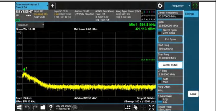
41-41-15MHz-20MHz-QPSK-QPSK-41319-41490-1RB#74-0RB#0 -0.15~30MHz-PASS
