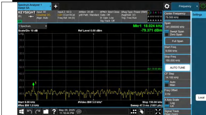
41-41-20MHz-10MHz-QPSK-QPSK-40571-40715-1RB#0-0RB#0- 0.009~0.15MHz-PASS
