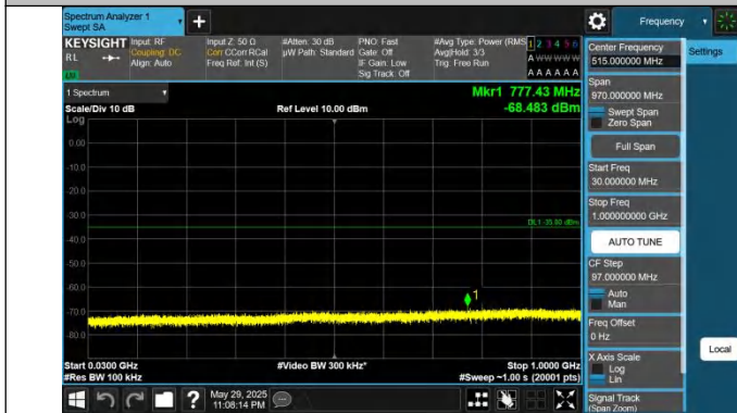
41-41-15MHz-20MHz-QPSK-QPSK-41319-41490-75RB#0-100R B#0-30~1000MHz-PASS
