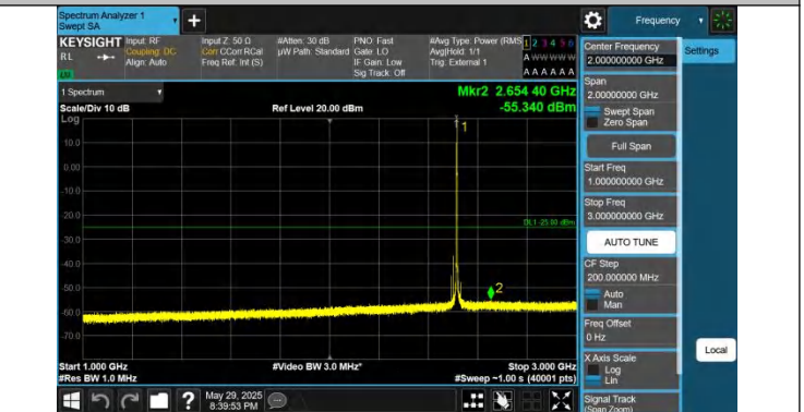
41-41-20MHz-15MHz-QPSK-QPSK-39750-39921-1RB#99-0RB#0 -1000~3000MHz-PASS
