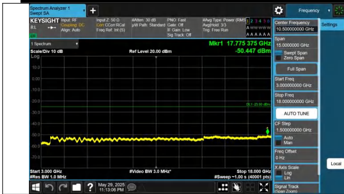
41-41-20MHz-5MHz-QPSK-QPSK-41440-41557-1RB#0-0RB#0-3 000~18000MHz-PASS
