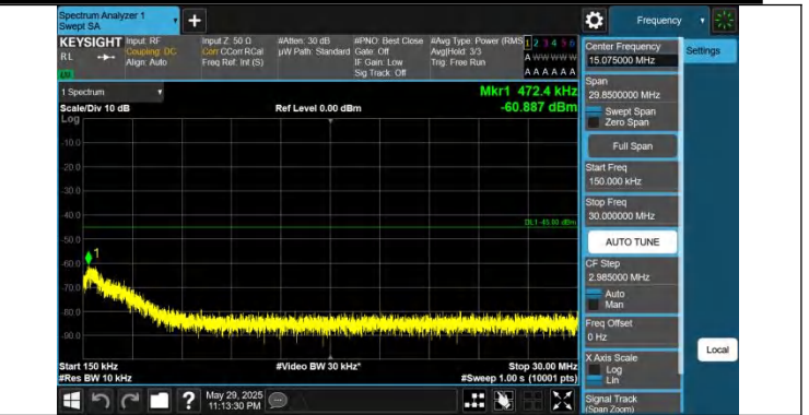
41-41-20MHz-5MHz-QPSK-QPSK-41440-41557-1RB#99-0RB#0-0.15~30MHz-PASS
