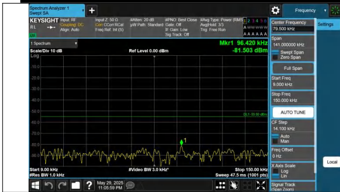
41-41-15MHz-20MHz-QPSK-QPSK-41319-41490-1RB#0-0RB#0-0.009~0.15MHz-PASS
