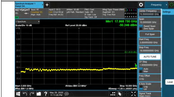
41-41-20MHz-5MHz-QPSK-QPSK-40595-40712-1RB#0-0RB#0-3000~18000MHz-PASS
