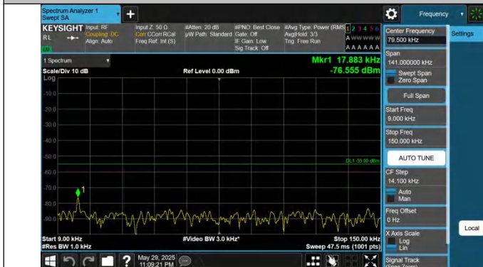
41-41-20MHz-5MHz-QPSK-QPSK-39750-39867-1RB#99-0RB#0-0.009~0.15MHz-PASS
