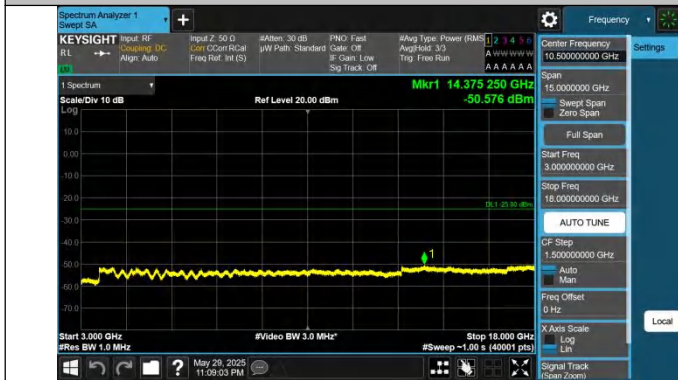
41-41-20MHz-5MHz-QPSK-QPSK-39750-39867-1RB#0-0RB#0-3000~18000MHz-PASS
