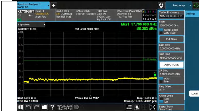
41-41-15MHz-20MHz-QPSK-QPSK-41319-41490-1RB#74-0RB# 0-3000~18000MHz-PASS
