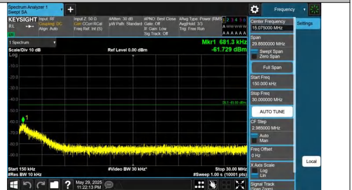
41-41-20MHz-15MHz-QPSK-QPSK-39750-39921-1RB#0-1RB#74-0.15~30MHz-PASS
