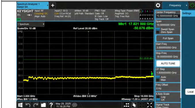
41-41-20MHz-10MHz-QPSK-QPSK-40571-40715-1RB#0-1RB#4 9-3000~18000MHz-PASS
