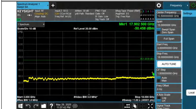
41-41-15MHz-20MHz-QPSK-QPSK-41319-41490-1RB#0-1RB#9 9-3000~18000MHz-PASS
