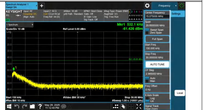
41-41-20MHz-5MHz-QPSK-QPSK-41440-41557-1RB#0-0RB#0-0.15~30MHz-PASS
