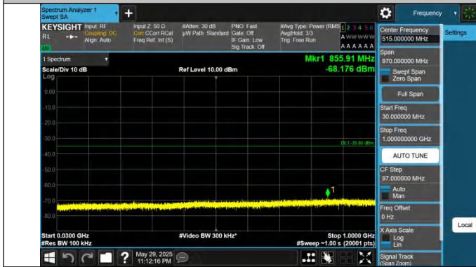
41-41-20MHz-5MHz-QPSK-QPSK-40595-40712-1RB#0-1RB#24-30~1000MHz-PASS
