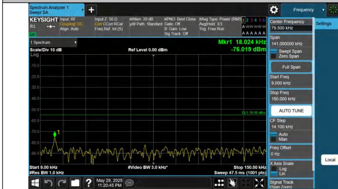
41-41-20MHz-15MHz-QPSK-QPSK-39750-39921-1RB#0-0RB#0- 0.009~0.15MHz-PASS
