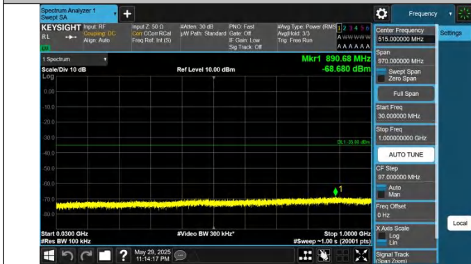
41-41-20MHz-5MHz-QPSK-QPSK-41440-41557-1RB#0-1RB#24- 30~1000MHz-PASS
