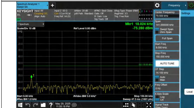
41-41-15MHz-20MHz-QPSK-QPSK-40523-40694-75RB#0-100R B#0-0.009~0.15MHz-PASS
