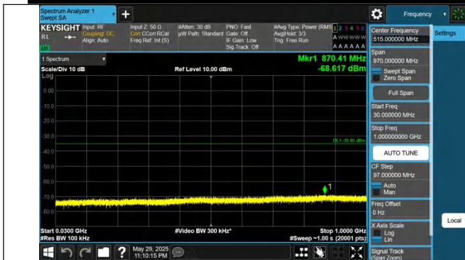
41-41-20MHz-5MHz-QPSK-QPSK-39750-39867-1RB#0-1RB#24-30~1000MHz-PASS
