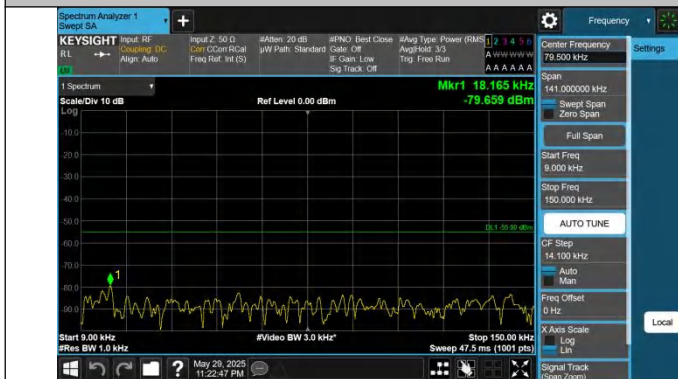
41-41-20MHz-15MHz-QPSK-QPSK-40546-40717-1RB#0-0RB#0- 0.009~0.15MHz-PASS
