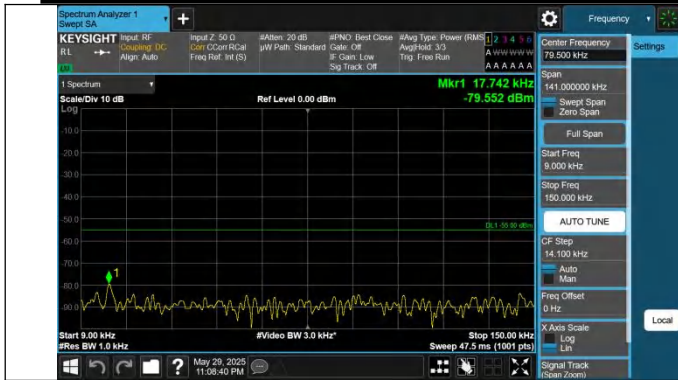
41-41-20MHz-5MHz-QPSK-QPSK-39750-39867-1RB#0-0RB#0-0.009~0.15MHz-PASS
