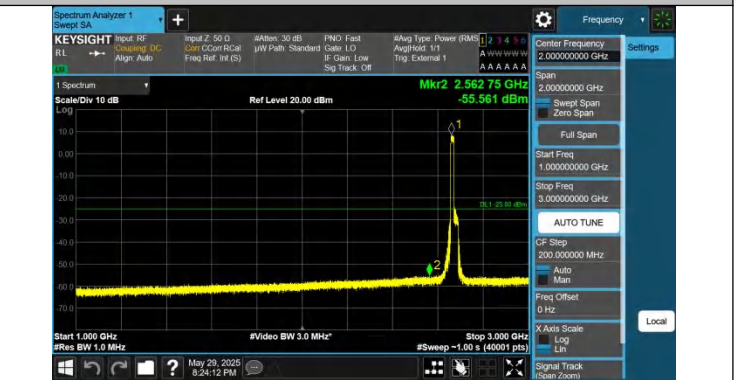
41-41-15MHz-20MHz-QPSK-QPSK-41319-41490-75RB#0-100RB #0-1000~3000MHz-PASS
