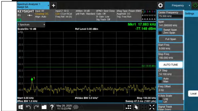
41-41-20MHz-5MHz-QPSK-QPSK-41440-41557-1RB#99-0RB#0-0.009~0.15MHz-PASS
