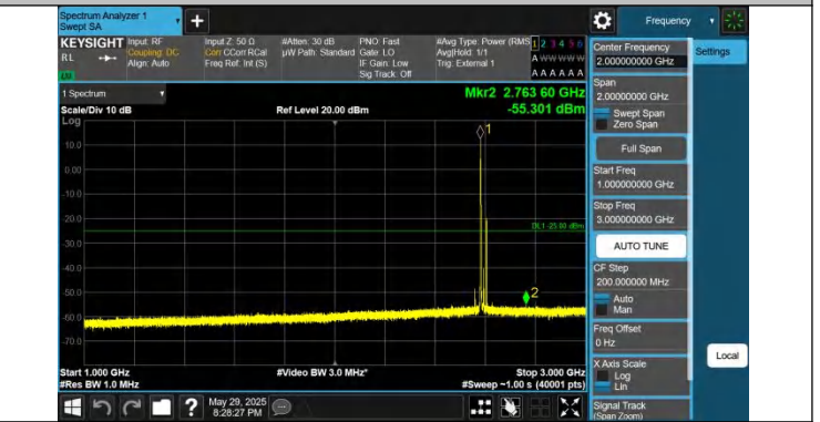
41-41-20MHz-5MHz-QPSK-QPSK-40595-40712-1RB#0-1RB#24-1000~3000MHz-PASS
