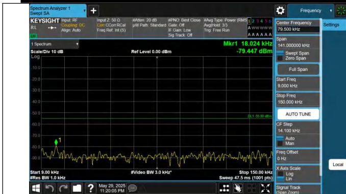
41-41-20MHz-10MHz-QPSK-QPSK-41391-41535-1RB#0-1RB#4 9-0.009~0.15MHz-PASS
