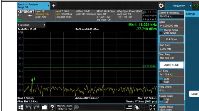
41-41-20MHz-5MHz-QPSK-QPSK-41440-41557-1RB#0-0RB#0-0.009~0.15MHz-PASS
