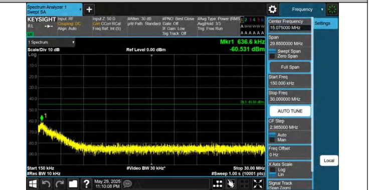
41-41-20MHz-5MHz-QPSK-QPSK-39750-39867-1RB#0-1RB#24-0.15~30MHz-PASS
