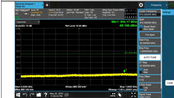
41-41-15MHz-20MHz-QPSK-QPSK-40523-40694-75RB#0-100R B#0-30~1000MHz-PASS
