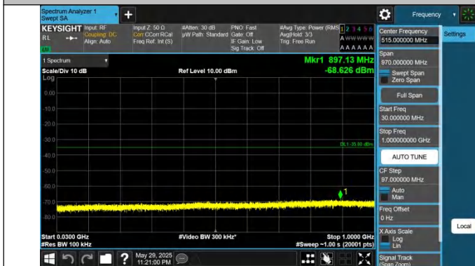
41-41-20MHz-15MHz-QPSK-QPSK-39750-39921-1RB#0-0RB#0- 30~1000MHz-PASS
