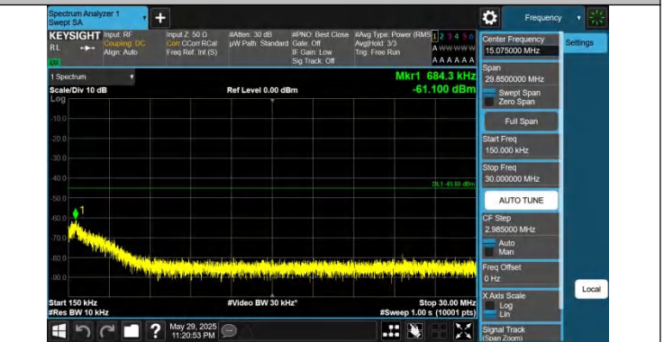
41-41-20MHz-15MHz-QPSK-QPSK-39750-39921-1RB#0-0RB#0- 0.15~30MHz-PASS
