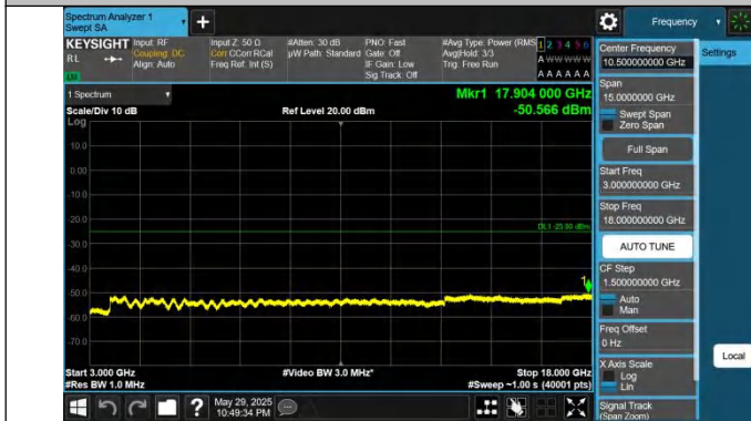
41-41-15MHz-10MHz-QPSK-QPSK-39725-39845-1RB#74-0RB# 0-3000~18000MHz-PASS
