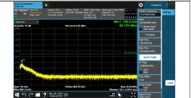
41-41-15MHz-15MHz-QPSK-QPSK-40545-40695-1RB#0-0RB#0- 0.15~30MHz-PASS
