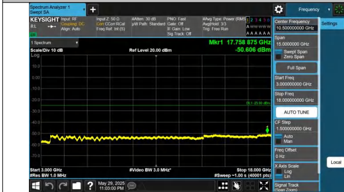
41-41-15MHz-20MHz-QPSK-QPSK-39728-39899-75RB#0-100RB B#0-3000~18000MHz-PASS
