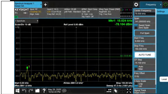
41-41-15MHz-10MHz-QPSK-QPSK-41417-41537-1RB#0-0RB#0- 0.009~0.15MHz-PASS
