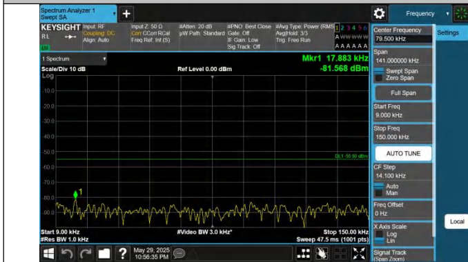
41-41-15MHz-15MHz-QPSK-QPSK-40545-40695-1RB#0-0RB#0- 0.009~0.15MHz-PASS
