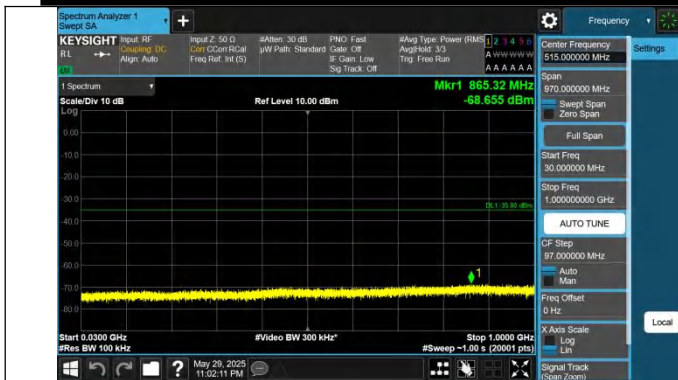
41-41-15MHz-20MHz-QPSK-QPSK-39728-39899-1RB#0-1RB#9 9-30~1000MHz-PASS
