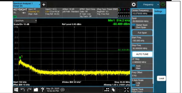
41-41-15MHz-10MHz-QPSK-QPSK-41417-41537-1RB#0-0RB#0- 0.15~30MHz-PASS
