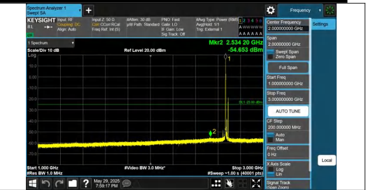
41-41-15MHz-10MHz-QPSK-QPSK-41417-41537-1RB#0-1RB#49 -1000~3000MHz-PASS
