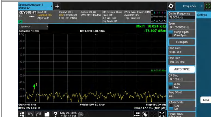
41-41-15MHz-20MHz-QPSK-QPSK-39728-39899-1RB#74-0RB# 0-0.009~0.15MHz-PASS
