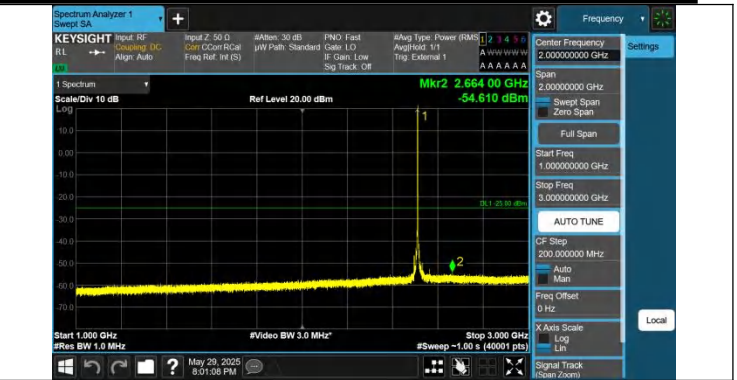
41-41-15MHz-15MHz-QPSK-QPSK-39725-39875-1RB#74-0RB#0 -1000~3000MHz-PASS
