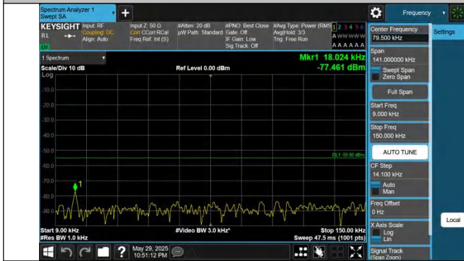
41-15MHz-10MHz-QPSK-QPSK-40571-40691-1RB#74-0RB# 0-0.009~0.15MHz-PASS
