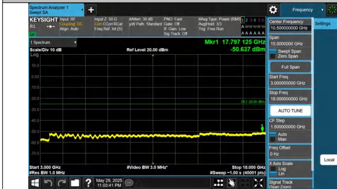
41-41-15MHz-20MHz-QPSK-QPSK-40523-40694-1RB#0-0RB#0- 3000~18000MHz-PASS
