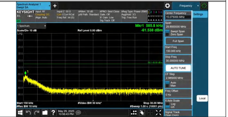
41-15MHz-15MHz-QPSK-QPSK-41365-41515-1RB#0-0RB#0- 0.15~30MHz-PASS
