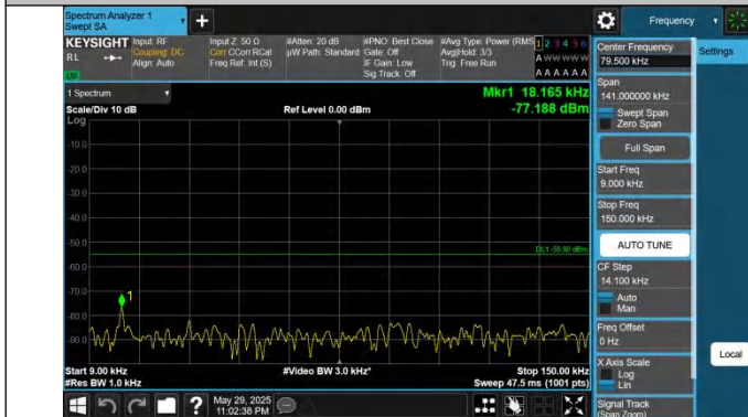
41-41-15MHz-20MHz-QPSK-QPSK-39728-39899-75RB#0-100RB B#0-0.009~0.15MHz-PASS
