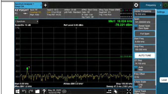
41-41-15MHz-10MHz-QPSK-QPSK-41417-41537-1RB#0-1RB#4 9-0.009~0.15MHz-PASS
