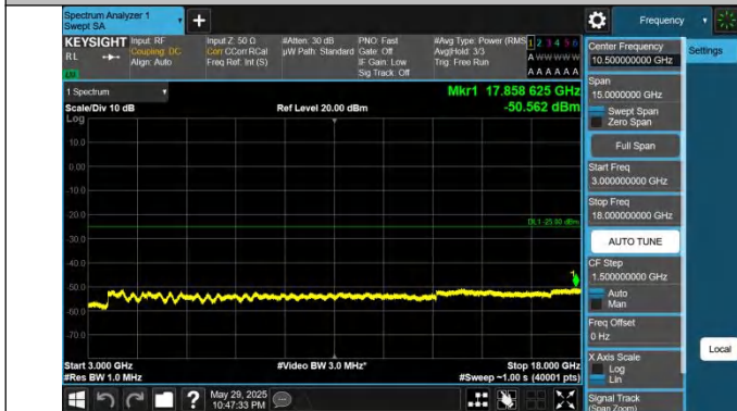
41-41-10MHz-20MHz-QPSK-QPSK-41346-41490-1RB#49-0RB# 0-3000~18000MHz-PASS
