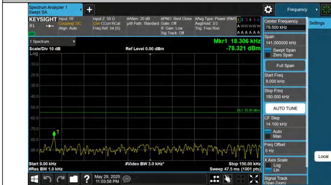
41-41-15MHz-20MHz-QPSK-QPSK-40523-40694-1RB#74-0RB# 0-0.009~0.15MHz-PASS
