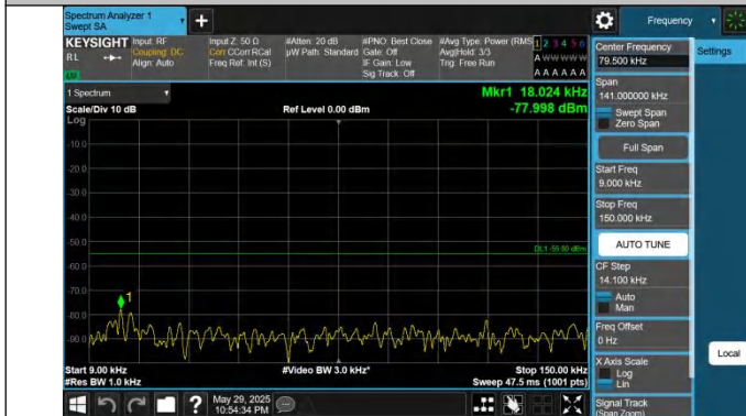
41-41-15MHz-15MHz-QPSK-QPSK-39725-39875-1RB#0-0RB#0- 0.009~0.15MHz-PASS
