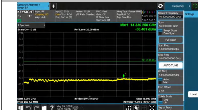
41-41-15MHz-15MHz-QPSK-QPSK-41365-41515-1RB#74-0RB# 0-3000~18000MHz-PASS
