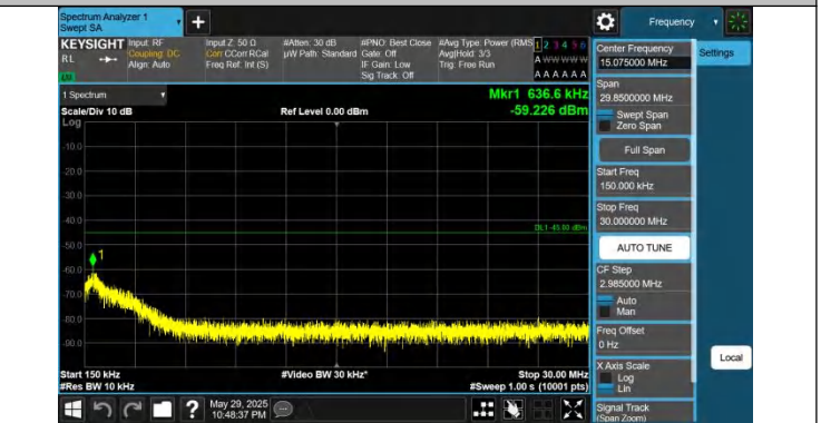
41-41-15MHz-10MHz-QPSK-QPSK-39725-39845-1RB#0-0RB#0- 0.15~30MHz-PASS
