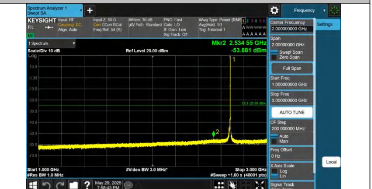
41-41-15MHz-10MHz-QPSK-QPSK-41417-41537-1RB#74-0RB#0 -1000~3000MHz-PASS
