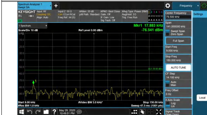
41-41-15MHz-10MHz-QPSK-QPSK-39725-39845-1RB#0-1RB#49-0.009~0.15MHz-PASS
