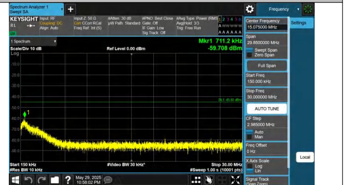
41-41-15MHz-15MHz-QPSK-QPSK-40545-40695-1RB#0-1RB#74-0.15~30MHz-PASS
