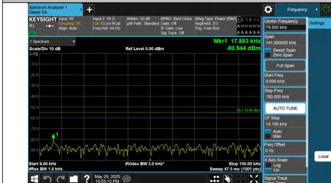
41-41-15MHz-10MHz-QPSK-QPSK-41417-41537-1RB#74-0RB# 0-0.009~0.15MHz-PASS
