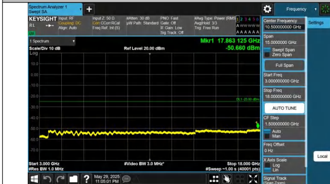
41-41-15MHz-20MHz-QPSK-QPSK-40523-40694-1RB#0-1RB#9 9-3000~18000MHz-PASS
