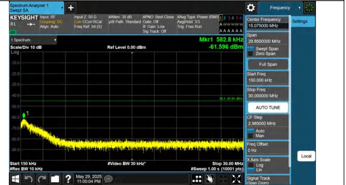
41-41-15MHz-15MHz-QPSK-QPSK-41365-41515-1RB#0-1RB#74-0.15~30MHz-PASS
