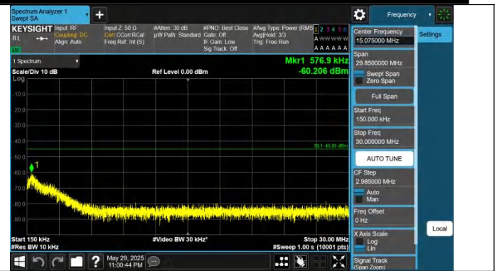
41-41-15MHz-20MHz-QPSK-QPSK-39728-39899-1RB#0-0RB#0- 0.15~30MHz-PASS
