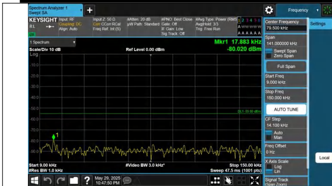
41-41-10MHz-20MHz-QPSK-QPSK-41346-41490-1RB#0-1RB#9 9-0.009~0.15MHz-PASS
