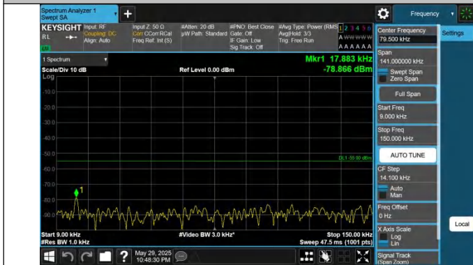
41-41-15MHz-10MHz-QPSK-QPSK-39725-39845-1RB#0-0RB#0- 0.009~0.15MHz-PASS
