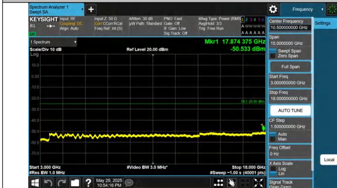
41-41-15MHz-10MHz-QPSK-QPSK-41417-41537-1RB#0-1RB#4 9-3000~18000MHz-PASS
