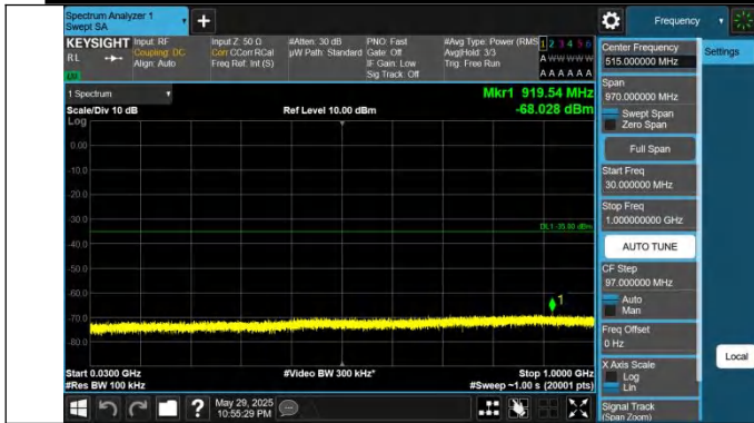
41-41-15MHz-15MHz-QPSK-QPSK-39725-39875-1RB#74-0RB# 0-30~1000MHz-PASS
