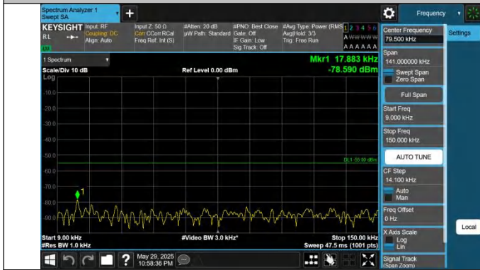
41-15MHz-15MHz-QPSK-QPSK-41365-41515-1RB#0-0RB#0- 0.009~0.15MHz-PASS
