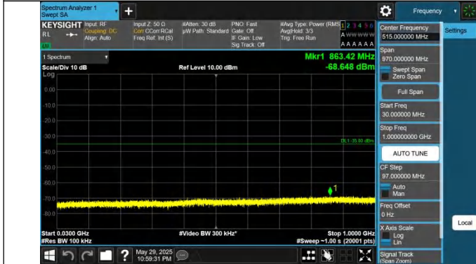
41-41-15MHz-15MHz-QPSK-QPSK-41365-41515-1RB#74-0RB# 0-30~1000MHz-PASS
