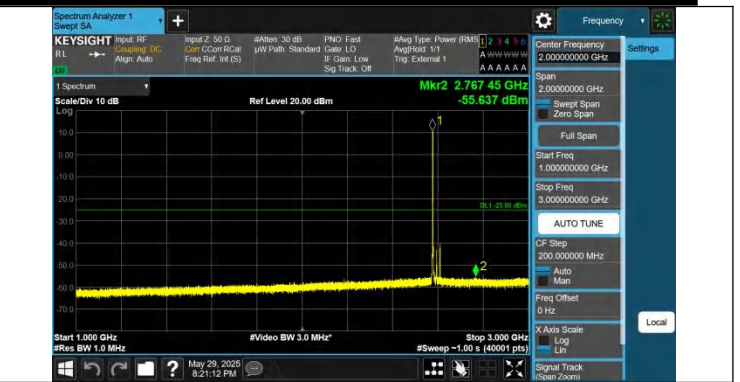
41-41-15MHz-20MHz-QPSK-QPSK-40523-40694-1RB#0-1RB#99 -1000~3000MHz-PASS
