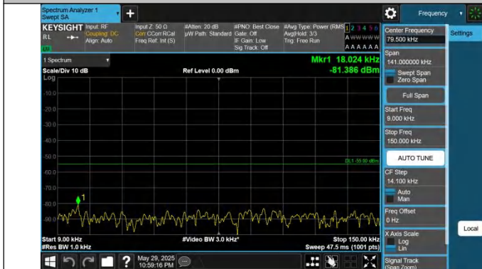
41-41-15MHz-15MHz-QPSK-QPSK-41365-41515-1RB#74-0RB# 0-0.009~0.15MHz-PASS
