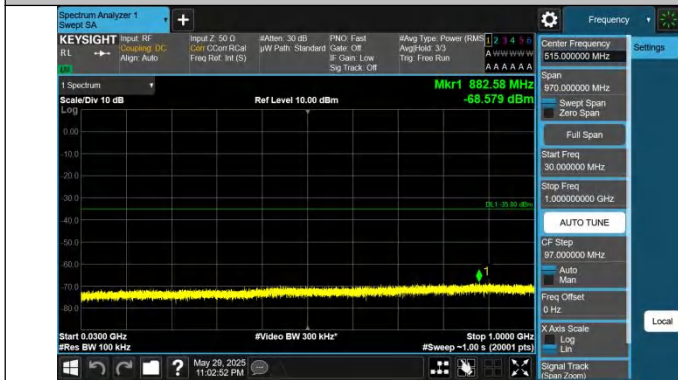
41-41-15MHz-20MHz-QPSK-QPSK-39728-39899-75RB#0-100RB B#0-30~1000MHz-PASS
