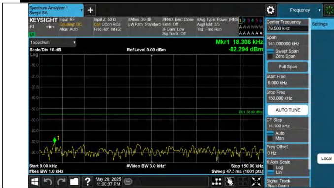
41-41-15MHz-20MHz-QPSK-QPSK-39728-39899-1RB#0-0RB#0- 0.009~0.15MHz-PASS
