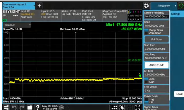
41-41-15MHz-20MHz-QPSK-QPSK-39728-39899-1RB#0-0RB#0- 3000~18000MHz-PASS
