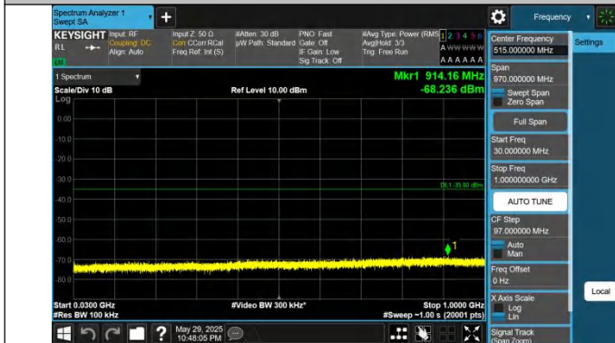
41-41-10MHz-20MHz-QPSK-QPSK-41346-41490-1RB#0-1RB#9 9-30~1000MHz-PASS
