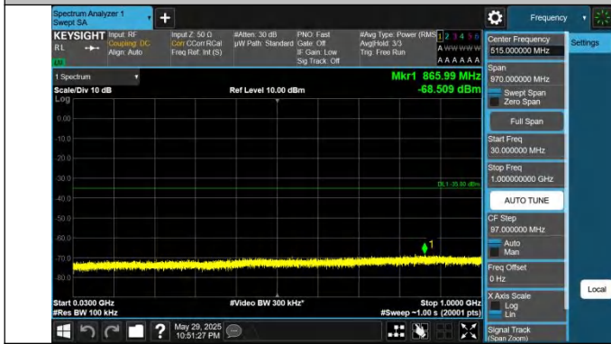
41-15MHz-10MHz-QPSK-QPSK-40571-40691-1RB#74-0RB# 0-30~1000MHz-PASS
