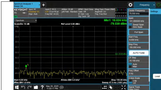
41-41-15MHz-20MHz-QPSK-QPSK-40523-40694-1RB#0-0RB#0- 0.009~0.15MHz-PASS
