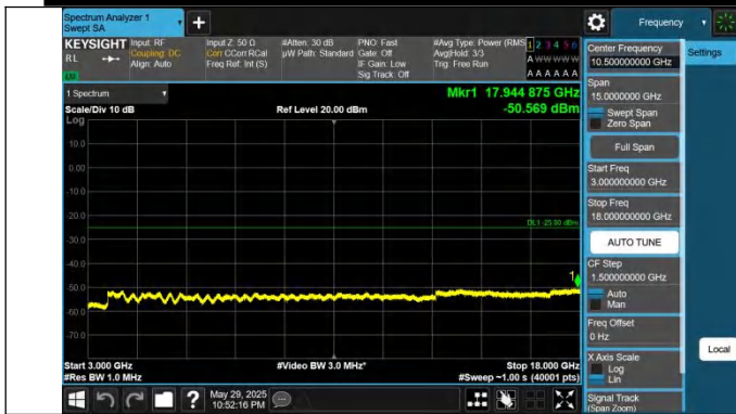
41-15MHz-10MHz-QPSK-QPSK-40571-40691-1RB#0-1RB#4 9-3000~18000MHz-PASS
