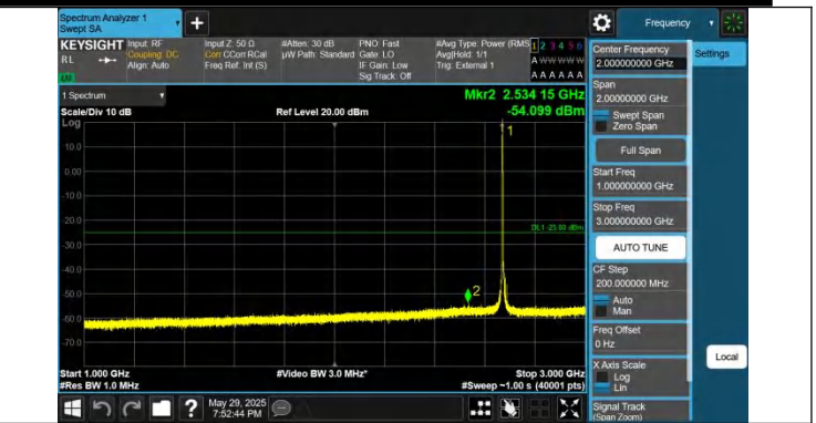
41-41-10MHz-20MHz-QPSK-QPSK-41346-41490-1RB#49-0RB#0 -1000~3000MHz-PASS
