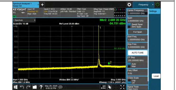
41-41-15MHz-15MHz-QPSK-QPSK-39725-39875-1RB#0-0RB#0- 1000~3000MHz-PASS
