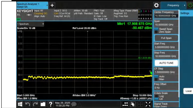
41-41-15MHz-15MHz-QPSK-QPSK-41365-41515-1RB#0-1RB#7 4-3000~18000MHz-PASS
