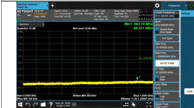
41-41-15MHz-15MHz-QPSK-QPSK-40545-40695-1RB#0-1RB#74-30~1000MHz-PASS
