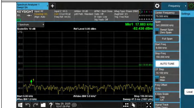
41-41-10MHz-20MHz-QPSK-QPSK-41346-41490-1RB#49-0RB# 0-0.009~0.15MHz-PASS
