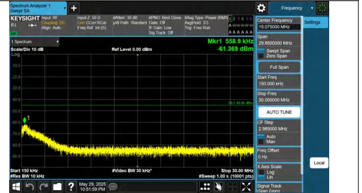
41-41-15MHz-10MHz-QPSK-QPSK-40571-40691-1RB#0-1RB#49-0.15~30MHz-PASS
