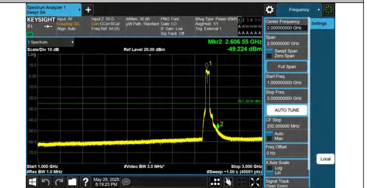
41-41-15MHz-20MHz-QPSK-QPSK-39728-39899-75RB#0-100RB #0-1000~3000MHz-PASS
