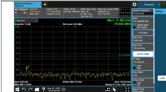
41-41-15MHz-15MHz-QPSK-QPSK-40545-40695-1RB#0-1RB#74-0.009~0.15MHz-PASS
