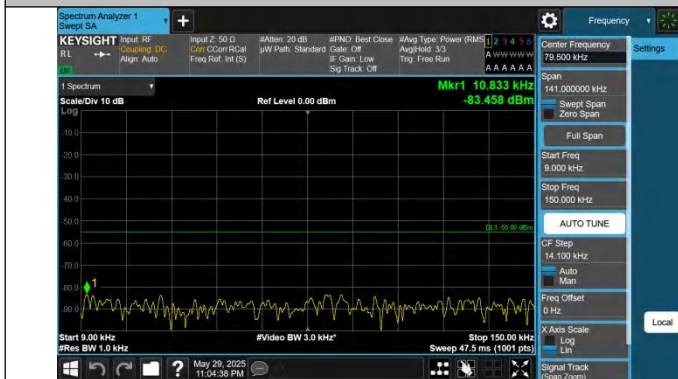
41-41-15MHz-20MHz-QPSK-QPSK-40523-40694-1RB#0-1RB#9 9-0.009~0.15MHz-PASS
