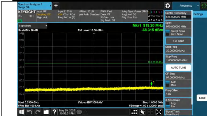
41-41-15MHz-15MHz-QPSK-QPSK-41365-41515-1RB#0-0RB#0-30~1000MHz-PASS
