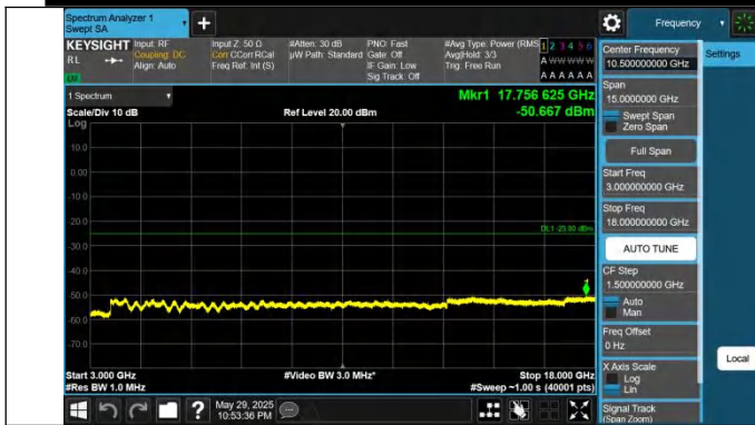
41-41-15MHz-10MHz-QPSK-QPSK-41417-41537-1RB#74-0RB# 0-3000~18000MHz-PASS
