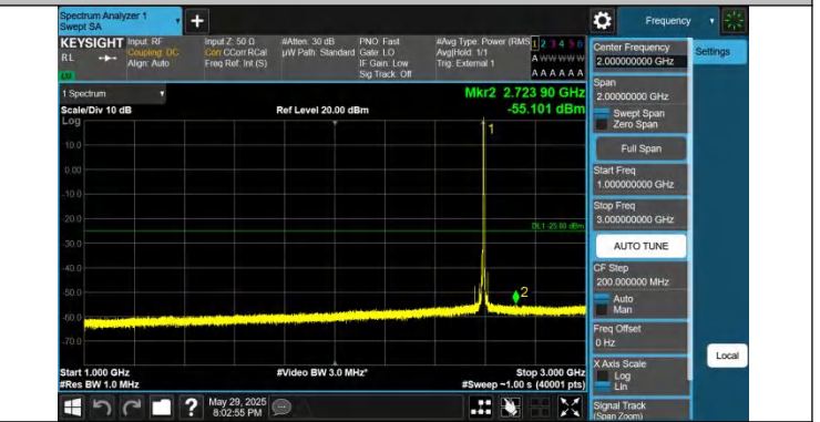
41-15MHz-15MHz-QPSK-QPSK-40545-40695-1RB#74-0RB#0 -1000~3000MHz-PASS
