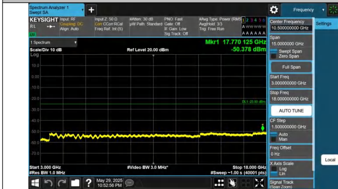
41-41-15MHz-10MHz-QPSK-QPSK-41417-41537-1RB#0-0RB#0- 3000~18000MHz-PASS
