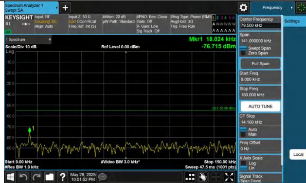
41-41-15MHz-10MHz-QPSK-QPSK-40571-40691-1RB#0-1RB#49-0.009~0.15MHz-PASS
