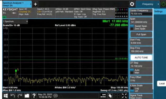
41-41-15MHz-15MHz-QPSK-QPSK-41365-41515-1RB#0-1RB#74-0.009~0.15MHz-PASS
