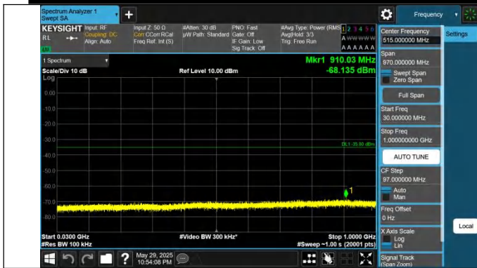
41-41-15MHz-10MHz-QPSK-QPSK-41417-41537-1RB#0-1RB#4 9-30~1000MHz-PASS
