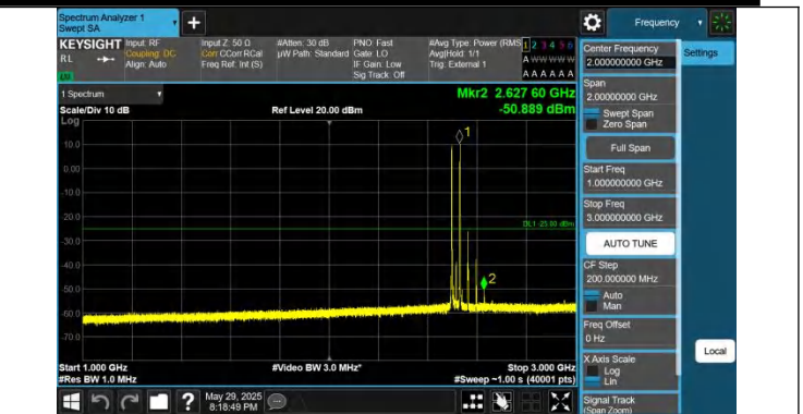
41-41-15MHz-20MHz-QPSK-QPSK-39728-39899-1RB#0-1RB#99 -1000~3000MHz-PASS
