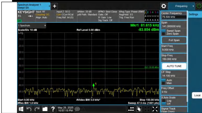
41-15MHz-15MHz-QPSK-QPSK-40545-40695-1RB#74-0RB# 0-0.009~0.15MHz-PASS
