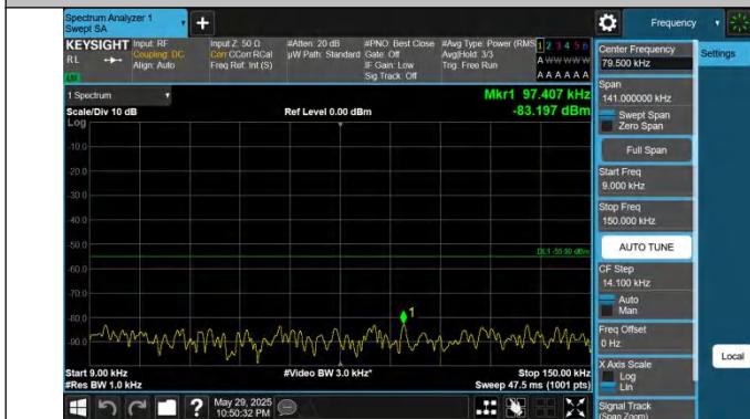
41-41-15MHz-10MHz-QPSK-QPSK-40571-40691-1RB#0-0RB#0- 0.009~0.15MHz-PASS
