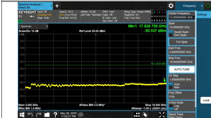
41-41-15MHz-20MHz-QPSK-QPSK-39728-39899-1RB#0-1RB#9 9-3000~18000MHz-PASS
