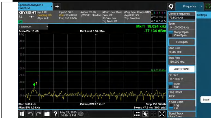
41-41-15MHz-10MHz-QPSK-QPSK-39725-39845-1RB#74-0RB# 0-0.009~0.15MHz-PASS
