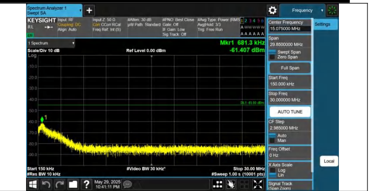
41-41-10MHz-15MHz-QPSK-QPSK-41395-41515-1RB#49-0RB# -0.15~30MHz-PASS
