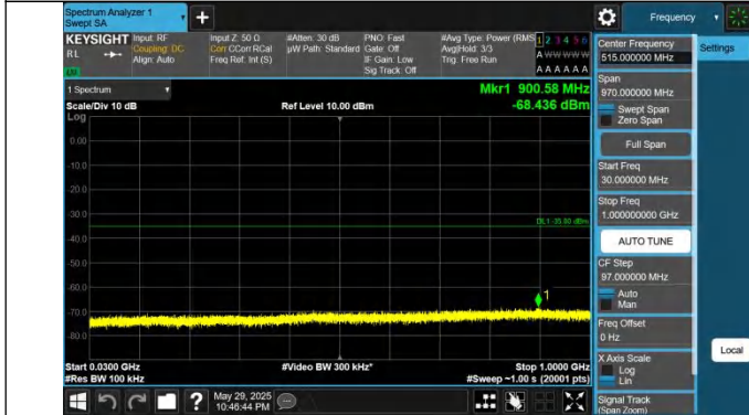
41-41-10MHz-20MHz-QPSK-QPSK-41346-41490-1RB#0-0RB#0- 30~1000MHz-PASS
