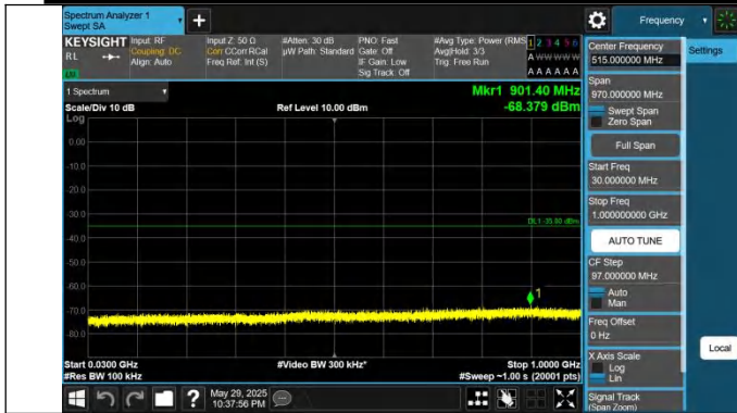
41-41-10MHz-15MHz-QPSK-QPSK-39703-39823-1RB#0-1RB#7 4-30~1000MHz-PASS
