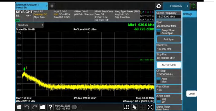
41-41-5MHz-20MHz-QPSK-QPSK-39683-39800-1RB#0-1RB#99- 0.15~30MHz-PASS
