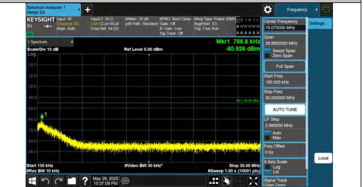
41-41-10MHz-15MHz-QPSK-QPSK-39703-39823-1RB#49-0RB#0 -0.15~30MHz-PASS
