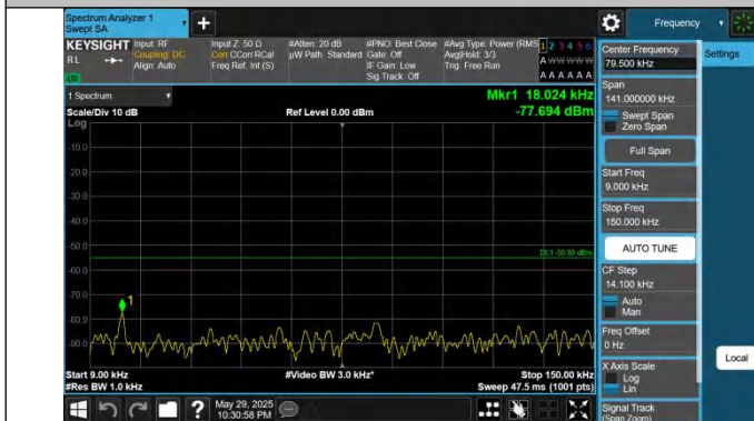
41-41-5MHz-20MHz-QPSK-QPSK-39683-39800-1RB#24-0RB#0- 0.009~0.15MHz-PASS
