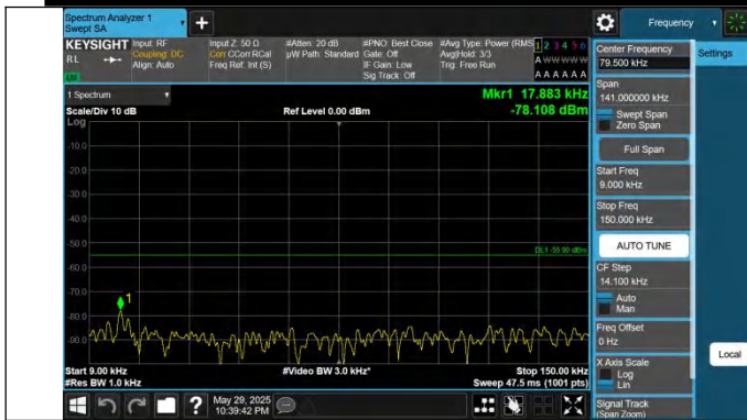
41-41-10MHz-15MHz-QPSK-QPSK-40549-40669-1RB#0-1RB#7 4-0.009~0.15MHz-PASS
