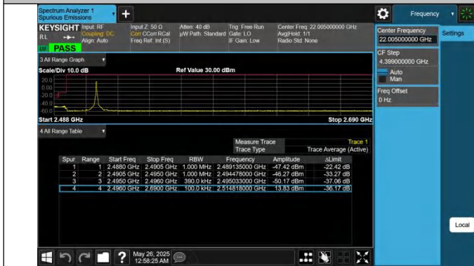
41-41-20MHz-20MHz-QPSK@QPSK-QPSK-39750-399 48-1RB#99@100RB#0-0RB#0@100RB#0-PASS
