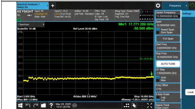
41-41-10MHz-15MHz-QPSK-QPSK-41395-41515-1RB#49-0RB# 0-3000~18000MHz-PASS
