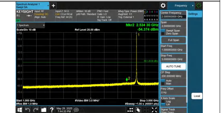
41-41-10MHz-15MHz-QPSK-QPSK-41395-41515-1RB#49-0RB# -1000~3000MHz-PASS
