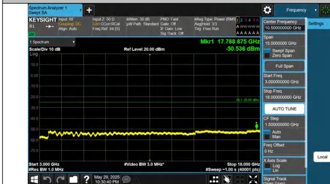
41-41-5MHz-20MHz-QPSK-QPSK-39683-39800-1RB#0-0RB#0-3000~18000MHz-PASS
