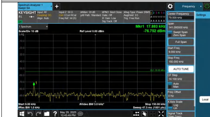
41-41-10MHz-20MHz-QPSK-QPSK-40526-40670-1RB#0-1RB#99-9-0.009~0.15MHz-PASS
