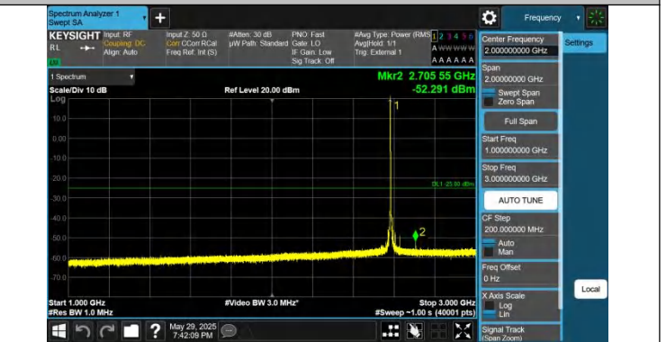
41-41-10MHz-15MHz-QPSK-QPSK-40549-40669-1RB#0-0RB#0- 1000~3000MHz-PASS
