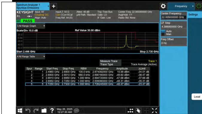
41-41-20MHz-15MHz-QPSK@QPSK-QPSK-41341-415 12-1RB#99@100RB#0-0RB#0@75RB#0-PASS
