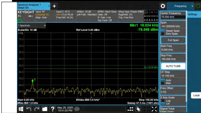
41-41-10MHz-15MHz-QPSK-QPSK-41395-41515-1RB#49-0RB# 0-0.009~0.15MHz-PASS
