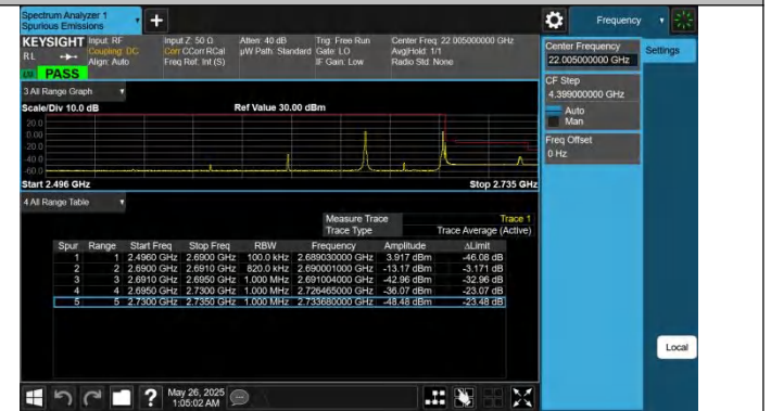
41-41-20MHz-20MHz-QPSK@QPSK-QPSK-41292-41490 -1RB#0@100RB#0-1RB#99@100RB#0-PASS
