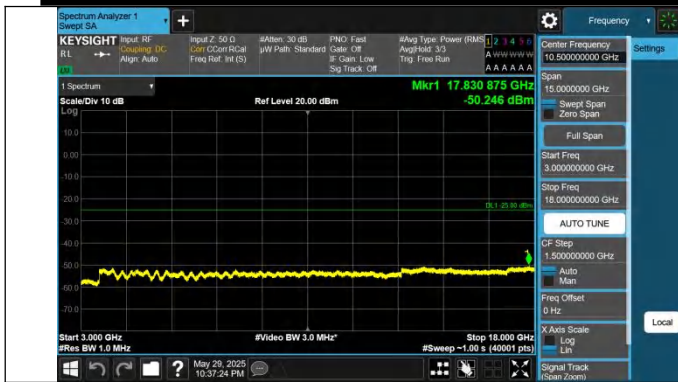
41-41-10MHz-15MHz-QPSK-QPSK-39703-39823-1RB#49-0RB# 0-3000~18000MHz-PASS
