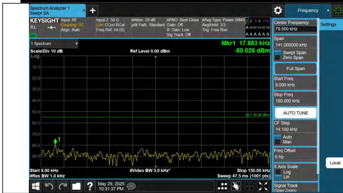
41-41-5MHz-20MHz-QPSK-QPSK-39683-39800-1RB#0-1RB#99- 0.009~0.15MHz-PASS
