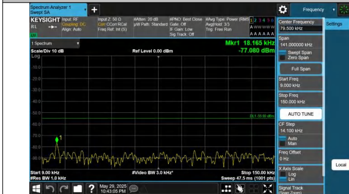
41-41-10MHz-20MHz-QPSK-QPSK-39705-39849-1RB#49-0RB# 0-0.009~0.15MHz-PASS
