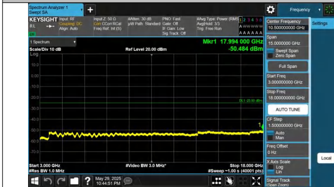
41-41-10MHz-20MHz-QPSK-QPSK-40526-40670-1RB#0-0RB#0-3000~18000MHz-PASS
