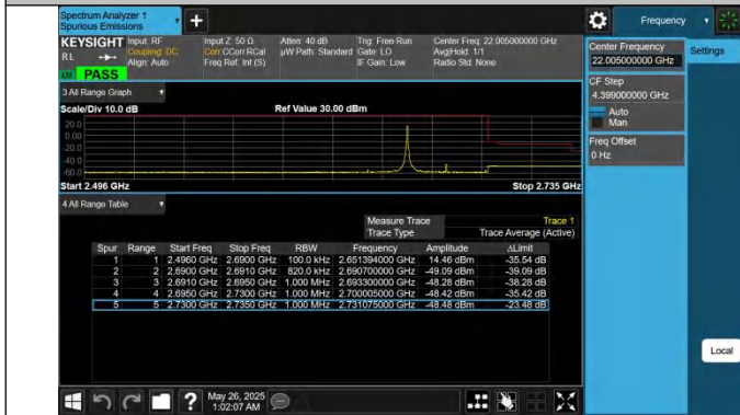
41-41-20MHz-20MHz-QPSK@QPSK-QPSK-41292-414 90-1RB#0@100RB#0-0RB#0@100RB#0-PASS
