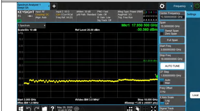
41-41-10MHz-20MHz-QPSK-QPSK-41346-41490-1RB#0-0RB#0- 3000~18000MHz-PASS
