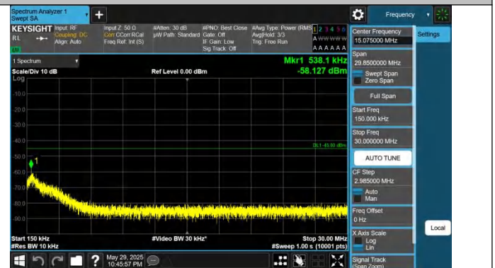
41-41-10MHz-20MHz-QPSK-QPSK-40526-40670-1RB#0-1RB#99-0.15~30MHz-PASS
