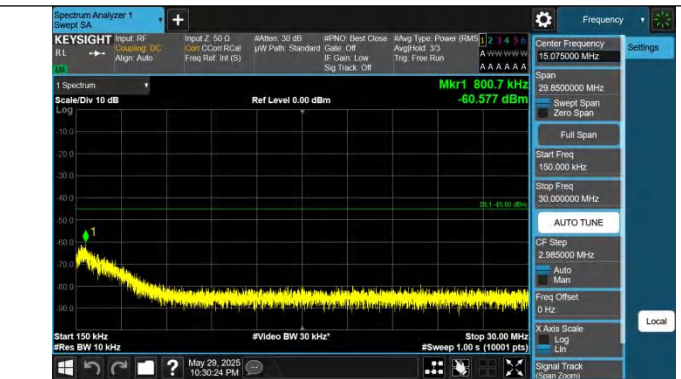
41-41-5MHz-20MHz-QPSK-QPSK-39683-39800-1RB#0-0RB#0-0.15~30MHz-PASS
