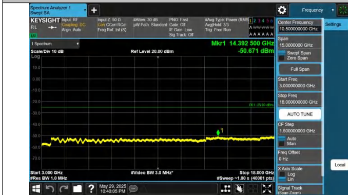
41-41-10MHz-15MHz-QPSK-QPSK-40549-40669-1RB#0-1RB#7 4-3000~18000MHz-PASS
