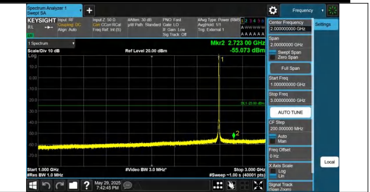
41-41-10MHz-15MHz-QPSK-QPSK-40549-40669-1RB#49-0RB#0 -1000~3000MHz-PASS
