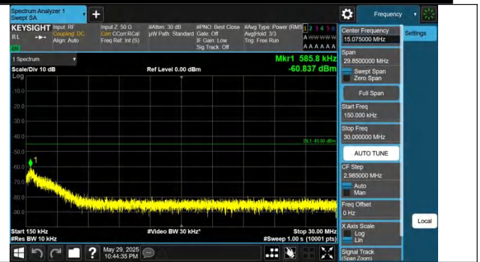
41-41-10MHz-20MHz-QPSK-QPSK-40526-40670-1RB#0-0RB#0-0.15~30MHz-PASS
