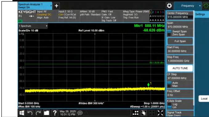
41-41-5MHz-20MHz-QPSK-QPSK-39683-39800-1RB#24-0RB#0-30~1000MHz-PASS
