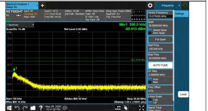
41-41-10MHz-15MHz-QPSK-QPSK-41395-41515-1RB#0-1RB#74-0.15~30MHz-PASS
