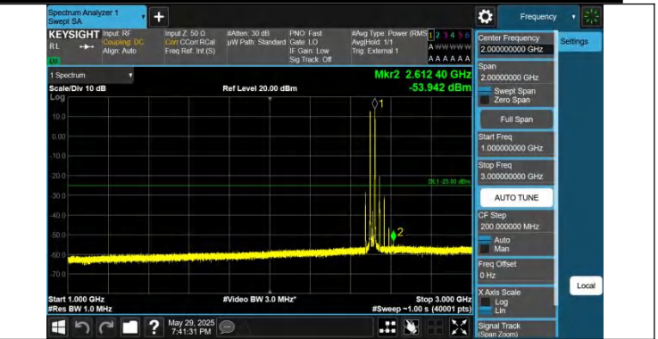
41-41-10MHz-15MHz-QPSK-QPSK-39703-39823-1RB#0-1RB#74 -1000~3000MHz-PASS
