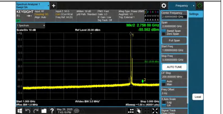
41-41-10MHz-15MHz-QPSK-QPSK-40549-40669-1RB#0-1RB#74 -1000~3000MHz-PASS
