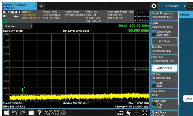
7-7-20MHz-20MHz-QPSK-QPSK-20850-21048-1RB#0-0RB#0-3 0~1000MHz-PASS
