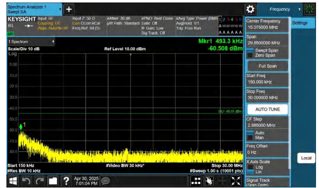
7-7-20MHz-15MHz-QPSK-QPSK-21201-21372-1RB#99-0RB#0-0.15~30MHz-PASS
