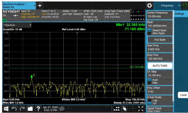
7-7-20MHz-15MHz-QPSK-QPSK-21201-21372-1RB#0-1RB#74- 0.009~0.15MHz-PASS
