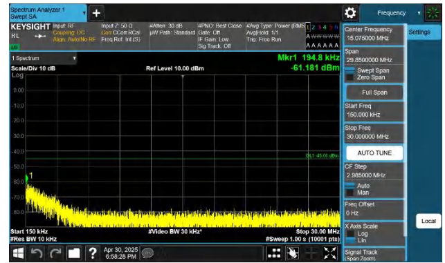
7-7-20MHz-15MHz-QPSK-QPSK-20850-21021-1RB#0-0RB#0-1 5~30MHz-PASS
