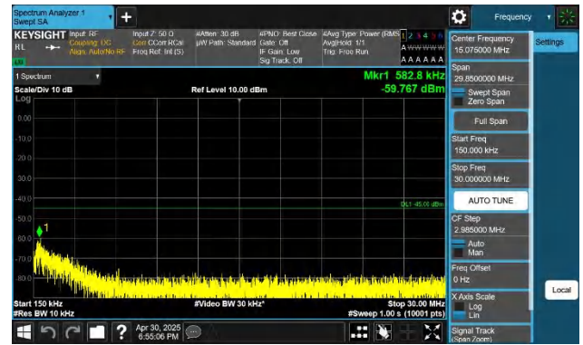
7-7-20MHz-10MHz-QPSK-QPSK-20850-20994-1RB#99-ORB#0-0.15~30MHz-PASS
