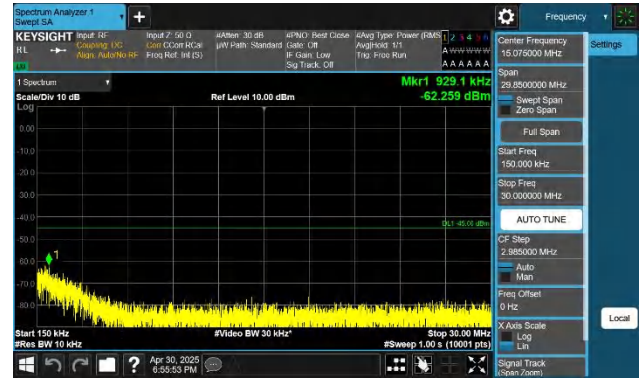
7-7-20MHz-10MHz-QPSK-QPSK-21051-21195-1RB#0-0RB#0-0.1 5~30MHz-PASS
