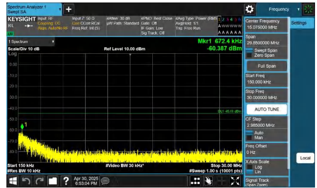
7-7-15MHz-20MHz-QPSK-QPSK-21179-21350-1RB#0-0RB#0-1 5~30MHz-PASS
