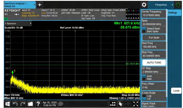
7-7-20MHz-10MHz-QPSK-QPSK-21051-21195-1RB#0-1RB#49-0. 15~30MHz-PASS
