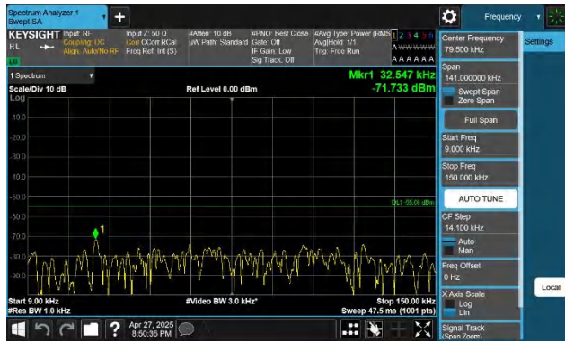
7-7-20MHz-15MHz-QPSK-QPSK-20850-21021-1RB#0-1RB#74- 0.009~0.15MHz-PASS
