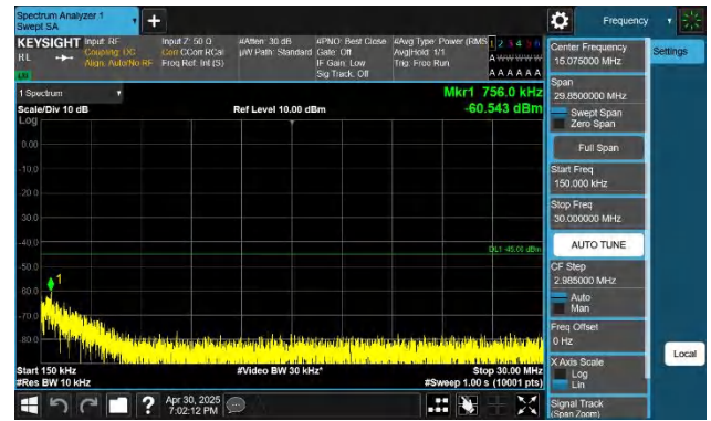
7-7-20MHz-20MHz-QPSK-QPSK-20850-21048-1RB#0-0RB#0-1 5~30MHz-PASS
