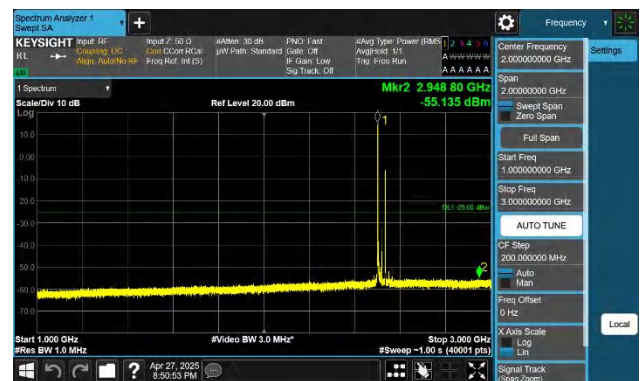
7-7-20MHz-15MHz-QPSK-QPSK-20850-21021-1RB#0-1RB#74-1 000~3000MHz-PASS
