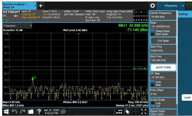
7-7-20MHz-10MHz-QPSK-QPSK-20850-20994-1RB#0-1RB#49- 0.009~0.15MHz-PASS
