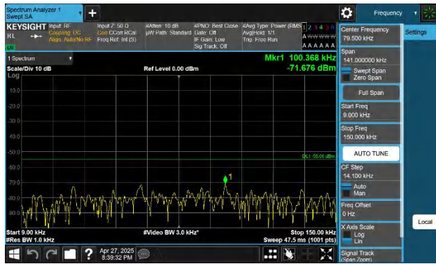
7-7-15MHz-20MHz-QPSK-QPSK-21179-21350-1RB#0-1RB#99-0 .009~0.15MHz-PASS
