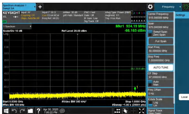
7-7-20MHz-15MHz-QPSK-QPSK-21026-21197-1RB#0-1RB#74-3 0~1000MHz-PASS
