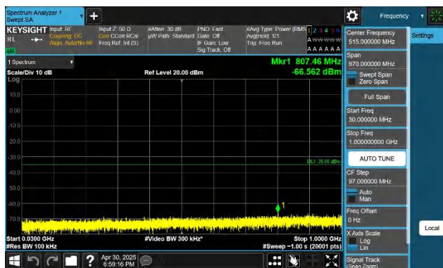
7-7-20MHz-15MHz-QPSK-QPSK-20850-21021-1RB#0-1RB#74- 30~1000MHz-PASS
