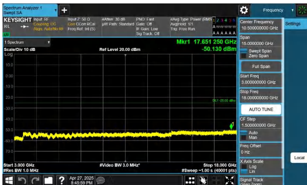
7-7-20MHz-10MHz-QPSK-QPSK-21051-21195-1RB#0-1RB#49-3 000~18000MHz-PASS
