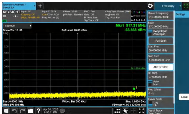
7-7-20MHz-10MHz-QPSK-QPSK-20850-20994-1RB#99-ORB#0-30~1000MHz-PASS
