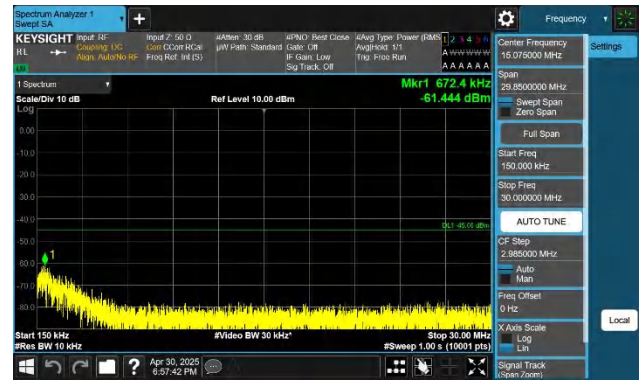
7-7-20MHz-10MHz-QPSK-QPSK-21251-21395-1RB#0-1RB#49-0. 15~30MHz-PASS
