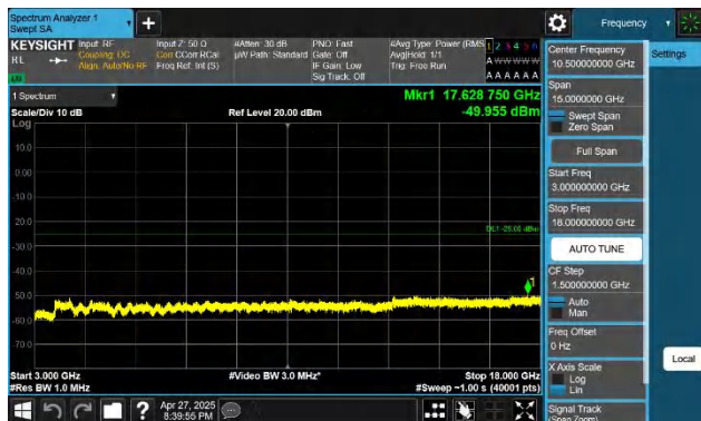
7-7-15MHz-20MHz-QPSK-QPSK-21179-21350-1RB#0-1RB#99-3 000~18000MHz-PASS
