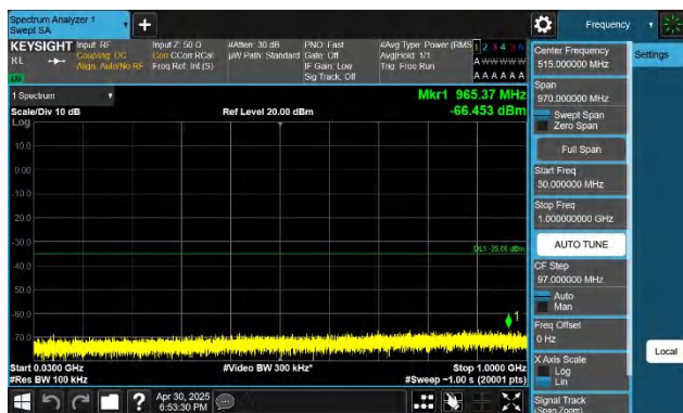
7-7-15MHz-20MHz-QPSK-QPSK-21179-21350-1RB#74-0RB#0-3 0~1000MHz-PASS
