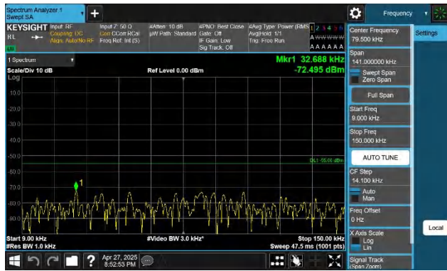
7-7-20MHz-15MHz-QPSK-QPSK-21026-21197-1RB#0-1RB#74-0 0.009~0.15MHz-PASS
