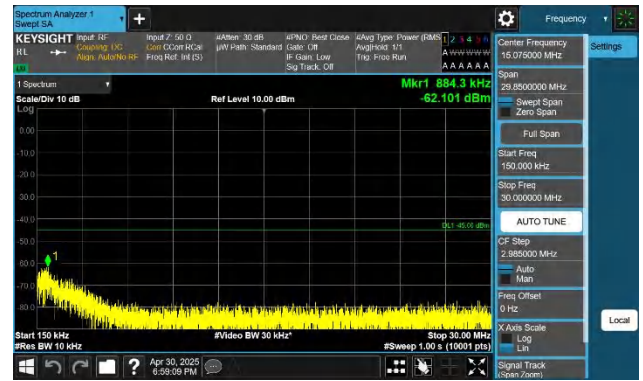
7-7-20MHz-15MHz-QPSK-QPSK-20850-21021-1RB#0-1RB#74-0. 15~30MHz-PASS
