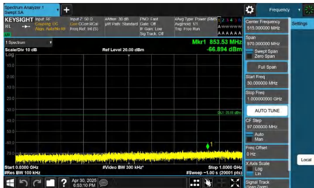
7-7-15MHz-20MHz-QPSK-QPSK-21179-21350-1RB#0-0RB#0-30 ~1000MHz-PASS
