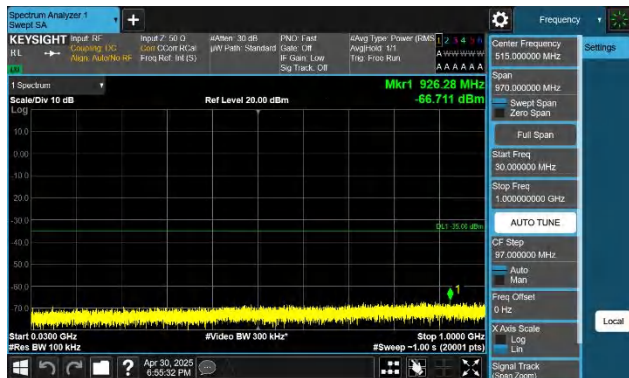
7-7-20MHz-10MHz-QPSK-QPSK-20850-20994-1RB#0-1RB#49- 30~1000MHz-PASS
