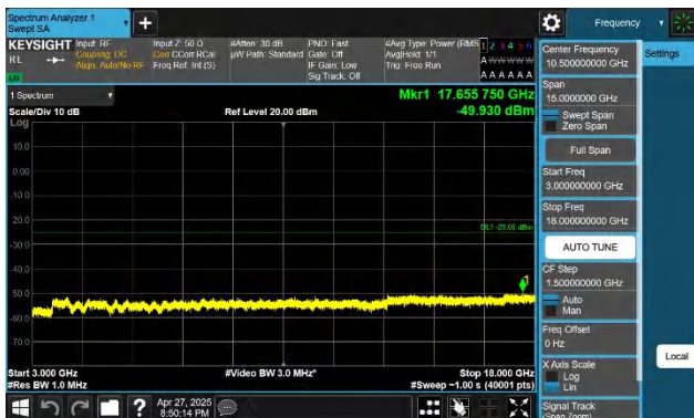
7-7-20MHz-15MHz-QPSK-QPSK-20850-21021-1RB#99-0RB#0- 3000~18000MHz-PASS
