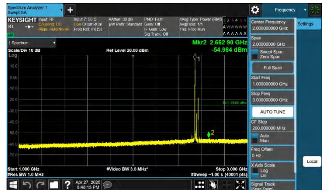
7-7-20MHz-10MHz-QPSK-QPSK-21251-21395-1RB#0-1RB#49-1 000~3000MHz-PASS
