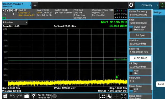
7-7-15MHz-20MHz-QPSK-QPSK-21179-21350-1RB#0-1RB#99-3 0~1000MHz-PASS
