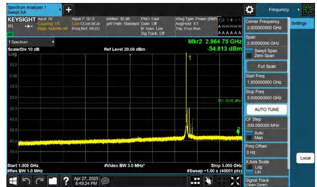
7-7-20MHz-15MHz-QPSK-QPSK-20850-21021-1RB#0-0RB#0-10 00~3000MHz-PASS
