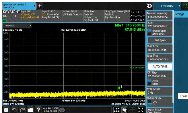
7-7-20MHz-10MHz-QPSK-QPSK-21051-21195-1RB#0-0RB#0-30 ~1000MHz-PASS
