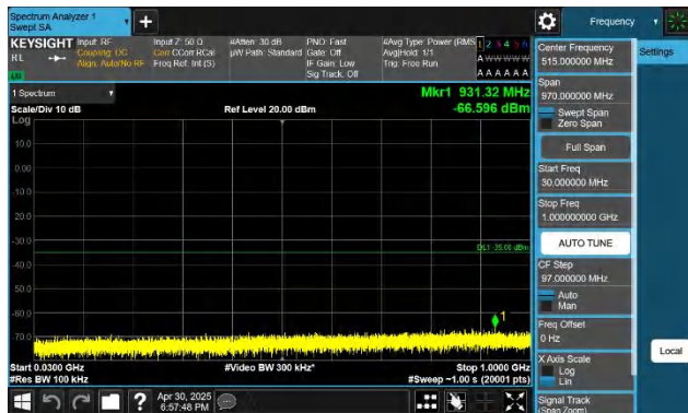
7-7-20MHz-10MHz-QPSK-QPSK-21251-21395-1RB#0-1RB#49- 30~1000MHz-PASS
