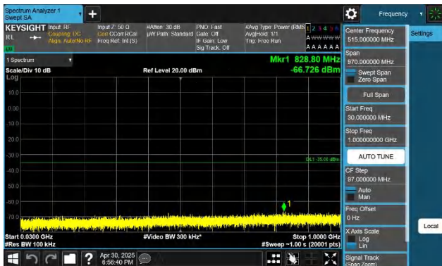
7-7-20MHz-10MHz-QPSK-QPSK-21051-21195-1RB#0-1RB#49-3 0~1000MHz-PASS
