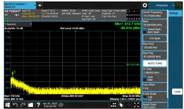
7-7-20MHz-15MHz-QPSK-QPSK-20850-21021-1RB#99-0RB#0-0. 15~30MHz-PASS
