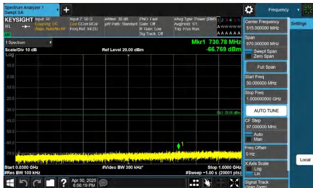
7-7-20MHz-10MHz-QPSK-QPSK-21051-21195-1RB#99-ORB#0-3 0~1000MHz-PASS
