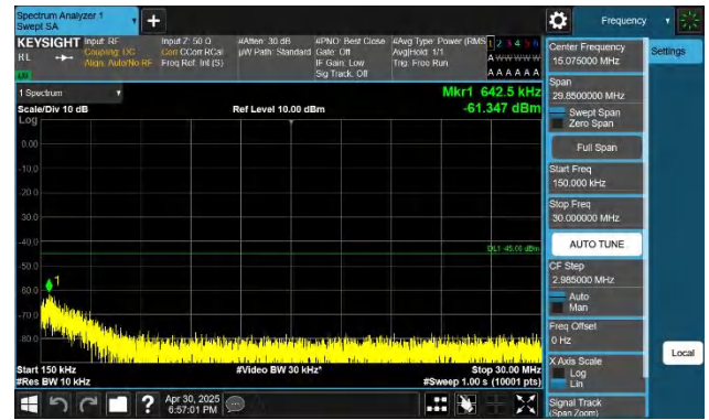
7-7-20MHz-10MHz-QPSK-QPSK-21251-21395-1RB#0-0RB#0-1 5~30MHz-PASS
