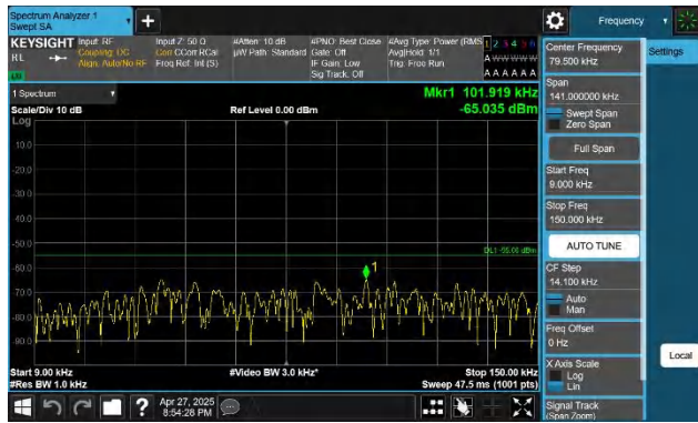
7-7-20MHz-15MHz-QPSK-QPSK-21201-21372-1RB#99-0RB#0-0.009~0.15MHz-PASS
