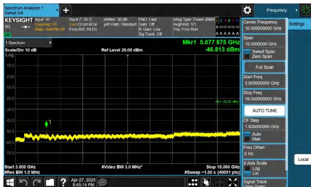
7-7-20MHz-10MHz-QPSK-QPSK-21051-21195-1RB#99-ORB#0-3 000~18000MHz-PASS
