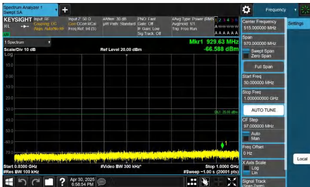
7-7-20MHz-15MHz-QPSK-QPSK-20850-21021-1RB#99-0RB#0- 30~1000MHz-PASS
