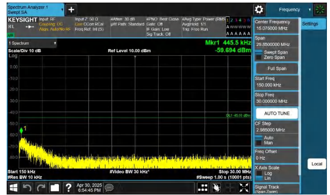
7-7-20MHz-10MHz-QPSK-QPSK-20850-20994-1RB#0-0RB#0-1 5~30MHz-PASS
