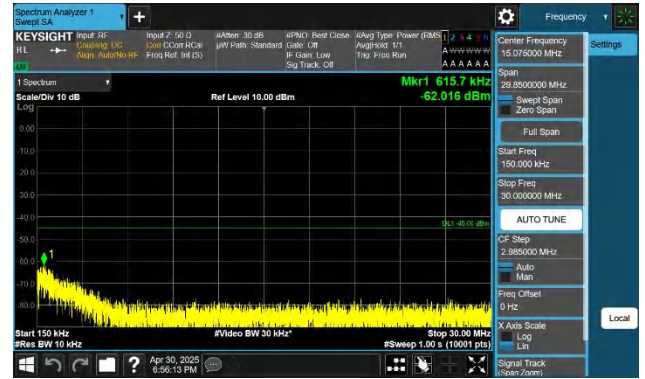
7-7-20MHz-10MHz-QPSK-QPSK-21051-21195-1RB#99-ORB#0-0. 15~30MHz-PASS
