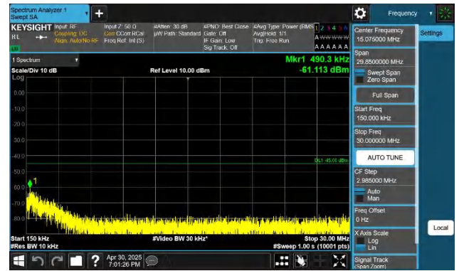
7-7-20MHz-15MHz-QPSK-QPSK-21201-21372-1RB#0-1RB#74-0. 15~30MHz-PASS
