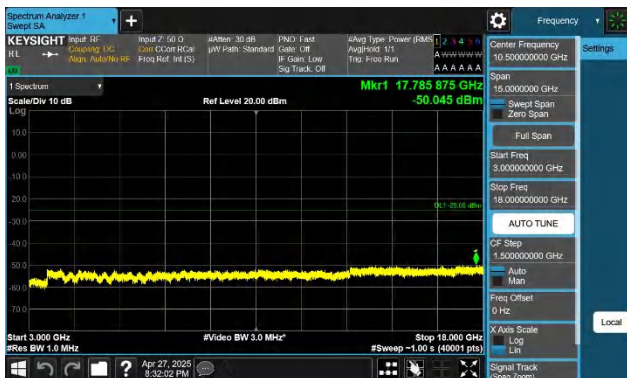
7-7-15MHz-15MHz-QPSK-QPSK-21225-21375-1RB#0-1RB#74-3000~18000MHz-PASS
