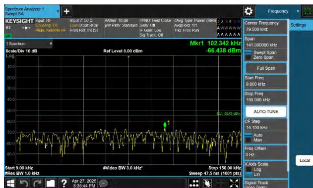
7-7-15MHz-20MHz-QPSK-QPSK-21003-21174-1RB#0-0RB#0-0. 009~0.15MHz-PASS
