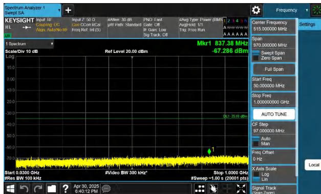
7-7-15MHz-10MHz-QPSK-QPSK-20825-20945-1RB#74-0RB#0- 30~1000MHz-PASS
