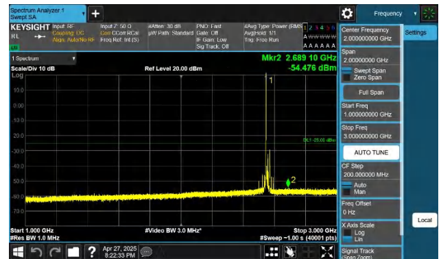
7-7-15MHz-10MHz-QPSK-QPSK-21277-21397-1RB#0-0RB#0-10 00~3000MHz-PASS
