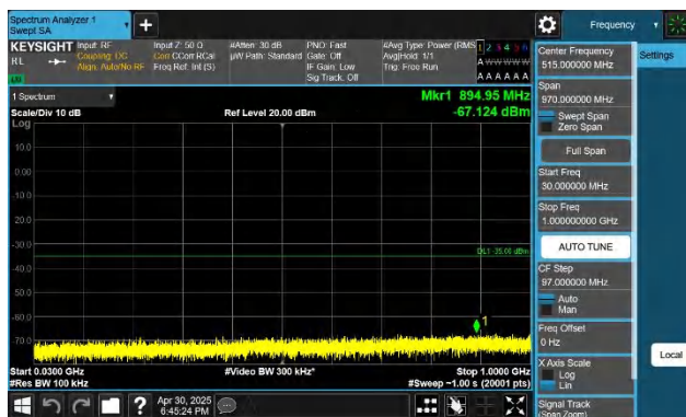
7-7-15MHz-15MHz-QPSK-QPSK-21025-21175-1RB#0-1RB#74-3 0~1000MHz-PASS
