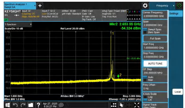
7-7-15MHz-15MHz-QPSK-QPSK-21225-21375-1RB#0-0RB#0-10 00~3000MHz-PASS
