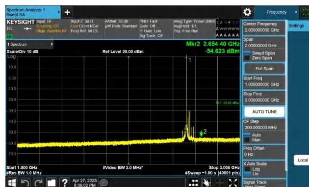
7-7-15MHz-20MHz-QPSK-QPSK-21003-21174-1RB#0-0RB#0-10 00~3000MHz-PASS
