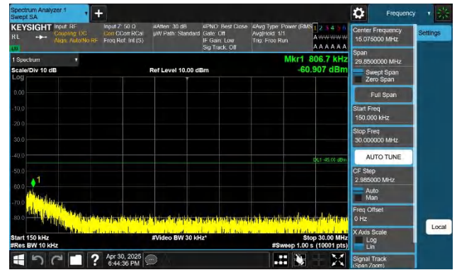
7-7-15MHz-15MHz-QPSK-QPSK-21025-21175-1RB#0-0RB#0-1 5~30MHz-PASS
