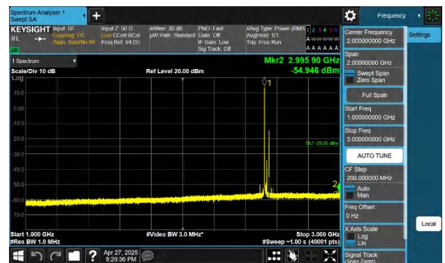
7-7-15MHz-15MHz-QPSK-QPSK-21025-21175-1RB#0-1RB#74-1 000~3000MHz-PASS
