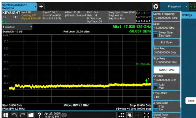
7-7-15MHz-10MHz-QPSK-QPSK-20825-20945-1RB#0-1RB#49- 3000~18000MHz-PASS
