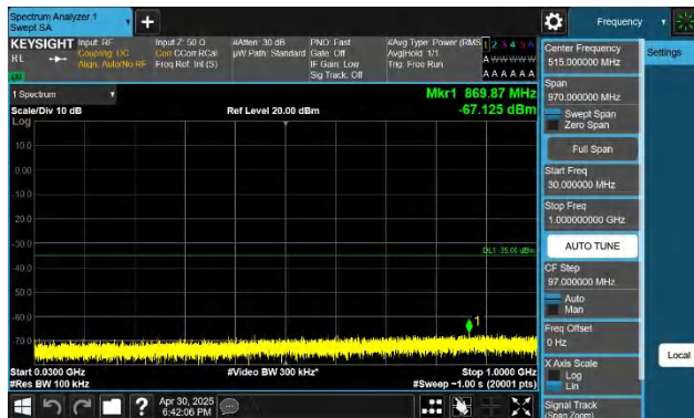
7-7-15MHz-10MHz-QPSK-QPSK-21277-21397-1RB#0-0RB#0-3 0~1000MHz-PASS
