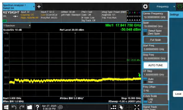
7-7-15MHz-20MHz-QPSK-QPSK-21003-21174-1RB#0-0RB#0-30 00~18000MHz-PASS
