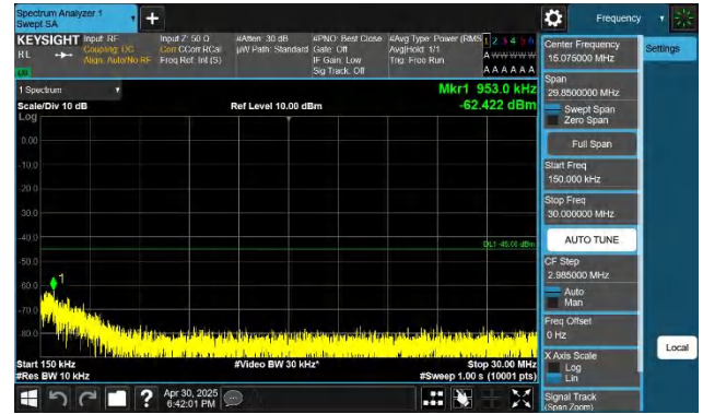
7-7-15MHz-10MHz-QPSK-QPSK-21277-21397-1RB#0-0RB#0-1 5~30MHz-PASS
