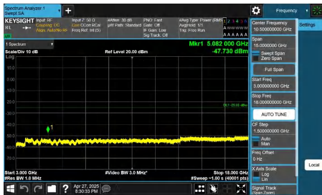
7-7-15MHz-15MHz-QPSK-QPSK-21225-21375-1RB#0-0RB#0-3 000~18000MHz-PASS
