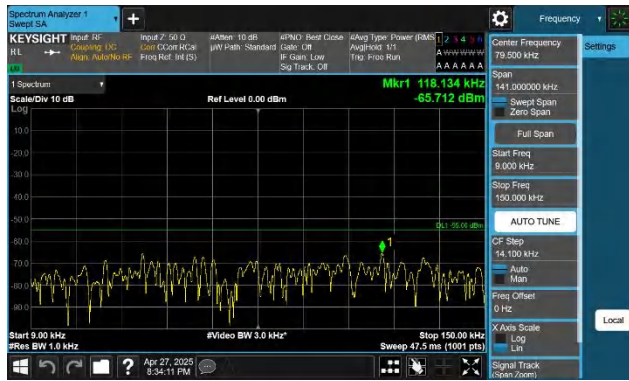
7-7-15MHz-20MHz-QPSK-QPSK-20828-20999-1RB#74-0RB#0- 0.009~0.15MHz-PASS
