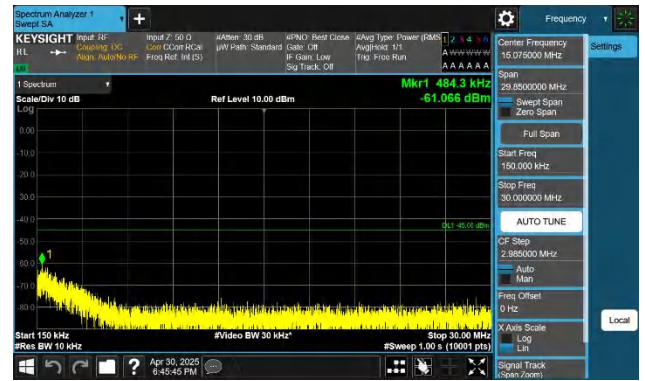
7-7-15MHz-15MHz-QPSK-QPSK-21225-21375-1RB#0-0RB#0-1 5~30MHz-PASS
