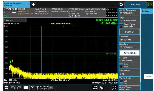
7-7-15MHz-15MHz-QPSK-QPSK-21025-21175-1RB#0-1RB#74-0. 15~30MHz-PASS
