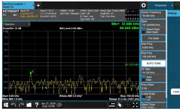
7-7-15MHz-15MHz-QPSK-QPSK-21025-21175-1RB#0-1RB#74-0 .009~0.15MHz-PASS
