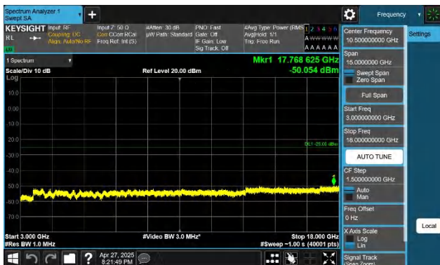
7-7-15MHz-10MHz-QPSK-QPSK-21051-21171-1RB#0-1RB#49-3 000~18000MHz-PASS
