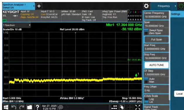
7-7-15MHz-15MHz-QPSK-QPSK-21025-21175-1RB#0-0RB#0-30 00~18000MHz-PASS
