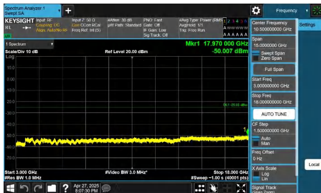
7-7-10MHz-20MHz-QPSK-QPSK-20805-20949-1RB#49-ORB#0-3000~18000MHz-PASS
