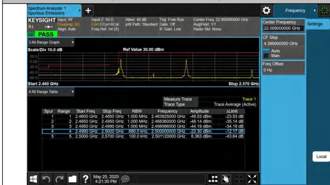
7-7-20MHz-15MHz-QPSK@QPSK-QPSK@QPSK-20850-21021-1RB#0@100RB#0-1RB#74@75RB#0-PASS
