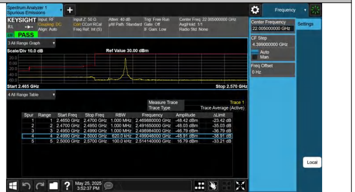
7-7-15MHz-15MHz-QPSK@QPSK-QPSK@QPSK-20825-20975-1RB#74@75RB#0-0RB#0@75RB#0-PASS
