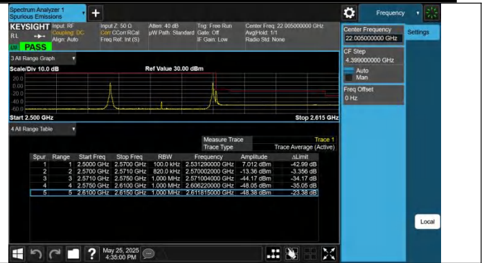
7-7-20MHz-20MHz-QPSK@QPSK-QPSK@QPSK-21152-21350-1RB#0@100RB#0-1RB#99@100RB#0-PASS
