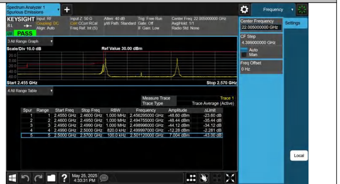
7-7-20MHz-20MHz-QPSK@QPSK-QPSK@QPSK-20850-21048-1RB#99@100RB#0-0RB#0@100RB#0-PASS
