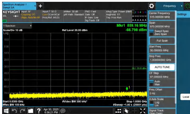
7-7-10MHz-20MHz-QPSK-QPSK-20805-20949-1RB#49-ORB#0-30~1000MHz-PASS
