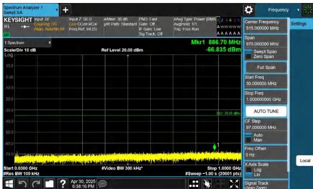
7-7-10MHz-20MHz-QPSK-QPSK-21206-21350-1RB#0-0RB#0-3 0~1000MHz-PASS
