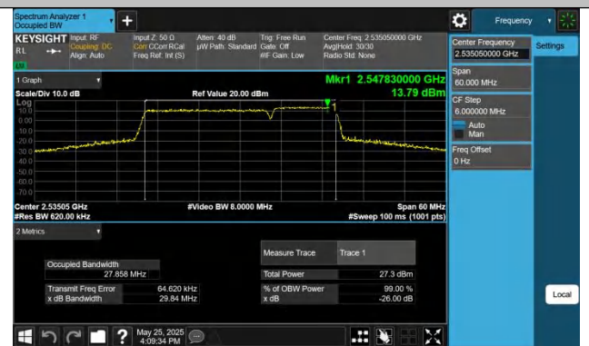
7-7-20MHz-10MHz-64QAM-64QAM-21051-21195-100RB#0-50R B#0-PASS
