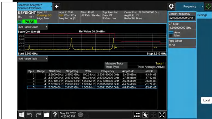
7-7-20MHz-15MHz-QPSK@QPSK-QPSK@QPSK-21201-21372-1RB#0@100RB#0-1RB#74@75RB#0-PASS
