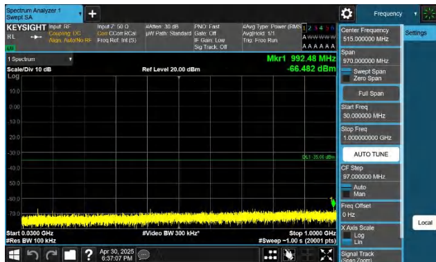
7-7-10MHz-20MHz-QPSK-QPSK-21006-21150-1RB#0-0RB#0-30 ~1000MHz-PASS
