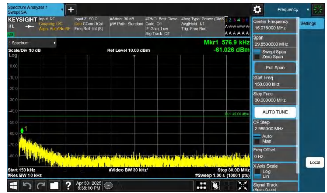
7-7-10MHz-20MHz-QPSK-QPSK-21206-21350-1RB#0-0RB#0-1 5~30MHz-PASS
