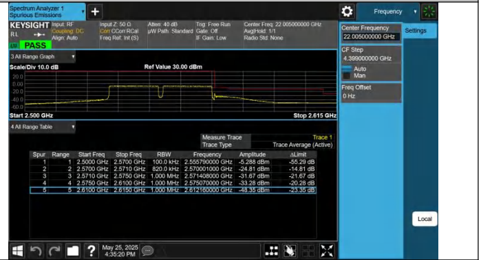
7-7-20MHz-20MHz-QPSK@QPSK-QPSK@QPSK-21152-21350-100RB#0@100RB#0-100RB#0@100RB#0-PASS
