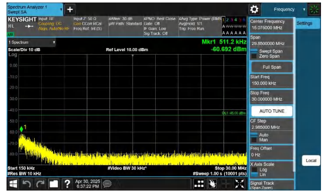
7-7-10MHz-20MHz-QPSK-QPSK-21006-21150-1RB#49-ORB#0-0. 15~30MHz-PASS
