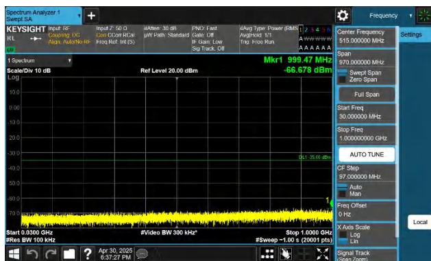
7-7-10MHz-20MHz-QPSK-QPSK-21006-21150-1RB#49-ORB#0-3 0~1000MHz-PASS
