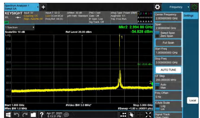
7-7-10MHz-20MHz-QPSK-QPSK-21006-21150-1RB#49-ORB#0-1 000~3000MHz-PASS
