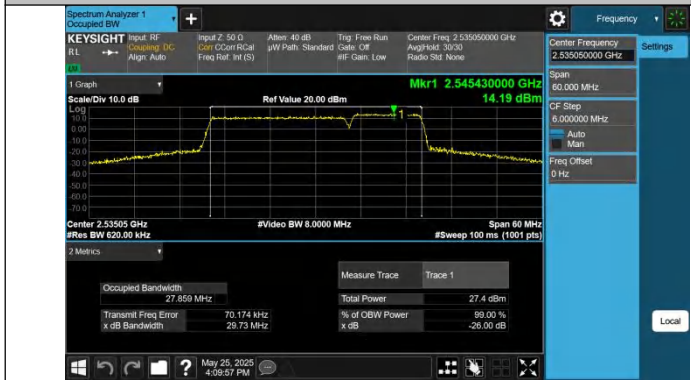
7-7-20MHz-10MHz-256QAM-256QAM-21051-21195-100RB#0-50 RB#0-PASS
