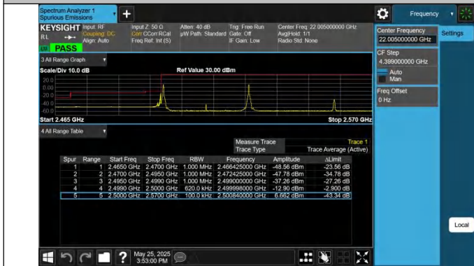
7-7-15MHz-15MHz-QPSK@QPSK-QPSK@QPSK-20825-20975-1RB#0@75RB#0-1RB#74@75RB#0-PASS
