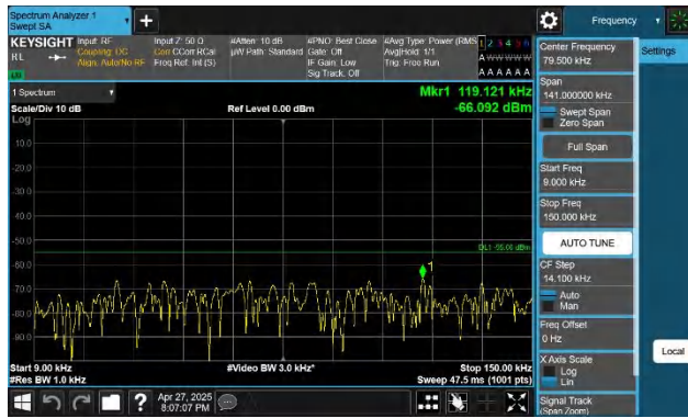
7-7-10MHz-20MHz-QPSK-QPSK-20805-20949-1RB#49-ORB#0-0.009~0.15MHz-PASS
