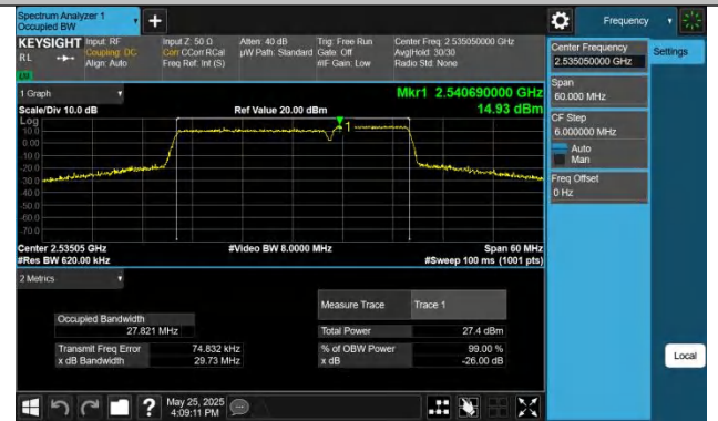
7-7-20MHz-10MHz-16QAM-16QAM-21051-21195-100RB#0-50R B#0-PASS
