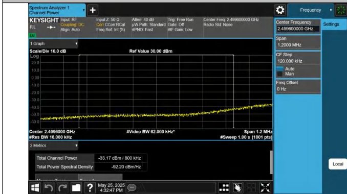
7-7-20MHz-20MHz-QPSK@QPSK-QPSK@QPSK-20850-21048-1RB#0@100RB#0-0RB#0@100RB#0-PASS
