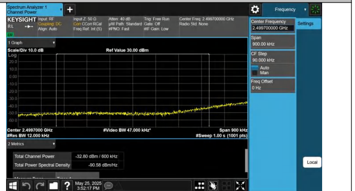
7-7-15MHz-15MHz-QPSK@QPSK-QPSK@QPSK-20825-20975-1RB#0@75RB#0-0RB#0@75RB#0-PASS
