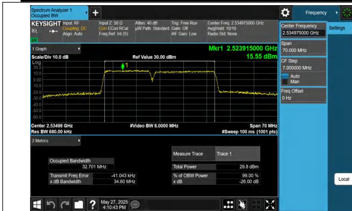
7-7-15MHz-20MHz-256QAM-256QAM-21003-21174-75RB#0-100 RB#0-PASS
