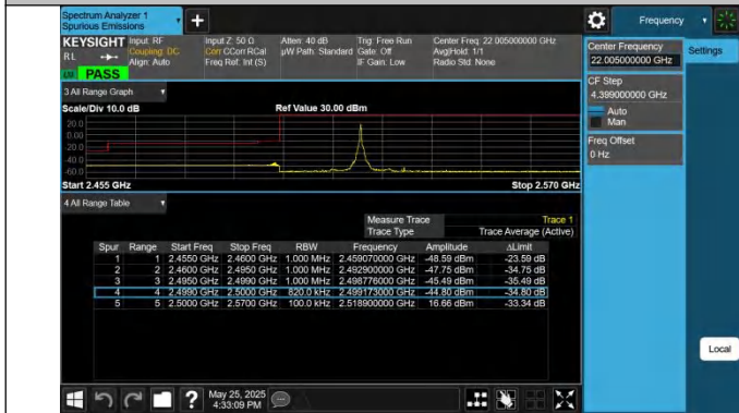
7-7-20MHz-20MHz-QPSK@QPSK-QPSK@QPSK-20850-21048-1RB#99@100RB#0-0RB#0@100RB#0-PASS
