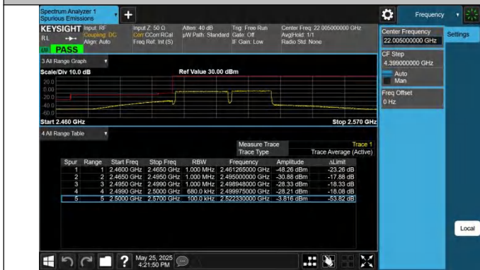
7-7-20MHz-15MHz-QPSK@QPSK-QPSK@QPSK-20850-21021-100RB#0@100RB#0-75RB#0@75RB#0-PASS
