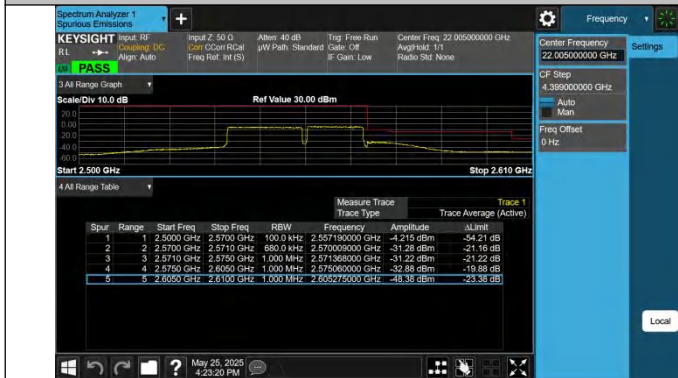
7-7-20MHz-15MHz-QPSK@QPSK-QPSK@QPSK-21201-21372-100RB#0@100RB#0-75RB#0@75RB#0-PASS
