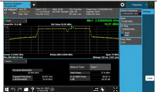
7-7-20MHz-15MHz-64QAM-64QAM-21026-21197-100RB#0-75R
