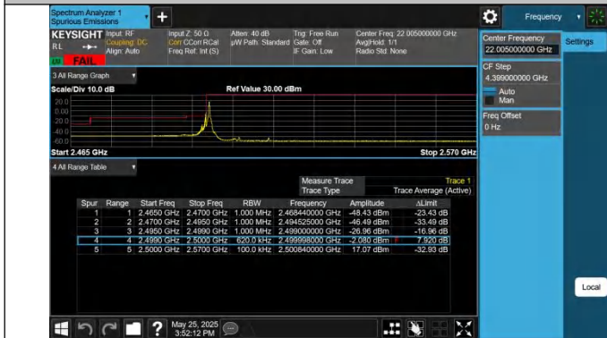
7-7-15MHz-15MHz-QPSK@QPSK-QPSK@QPSK-20825-20975-1RB#0@75RB#0-0RB#0@75RB#0
