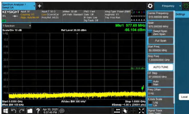
7-7-10MHz-20MHz-QPSK-QPSK-21006-21150-1RB#0-1RB#99-3 0~1000MHz-PASS
