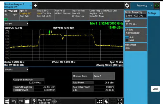
7-7-15MHz-20MHz-16QAM-16QAM-21003-21174-75RB#0-100R B#0-PASS
