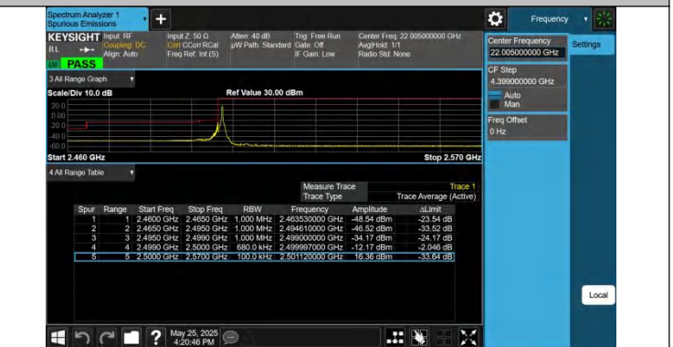
7-7-20MHz-15MHz-QPSK@QPSK-QPSK@QPSK-20850-21021-1RB#0@100RB#0-0RB#0@75RB#0-PASS
