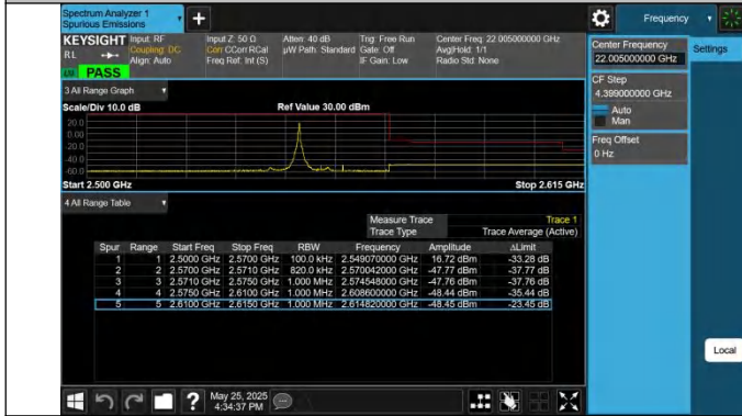
7-7-20MHz-20MHz-QPSK@QPSK-QPSK@QPSK-21152-21350-1RB#99@100RB#0-0RB#0@100RB#0-PASS
