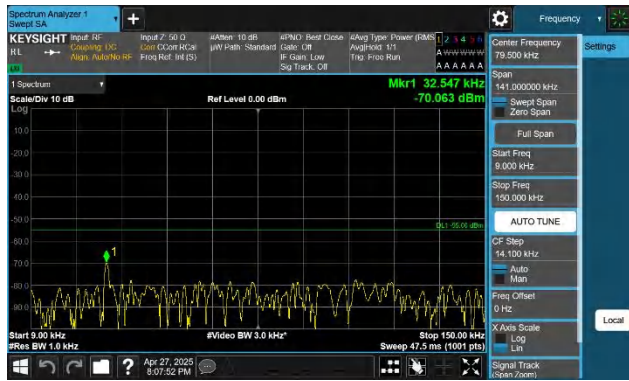
7-7-10MHz-20MHz-QPSK-QPSK-20805-20949-1RB#0-1RB#99- 0.009~0.15MHz-PASS
