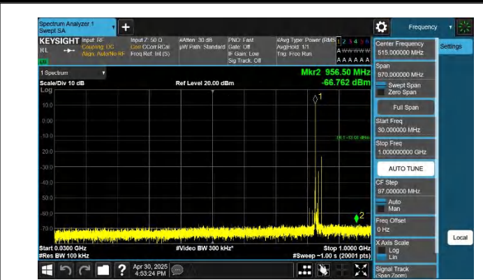
5-5-10MHz-10MHz-QPSK-QPSK-20501-20600-1RB#0-1RB#49-3 0~1000MHz-PASS
