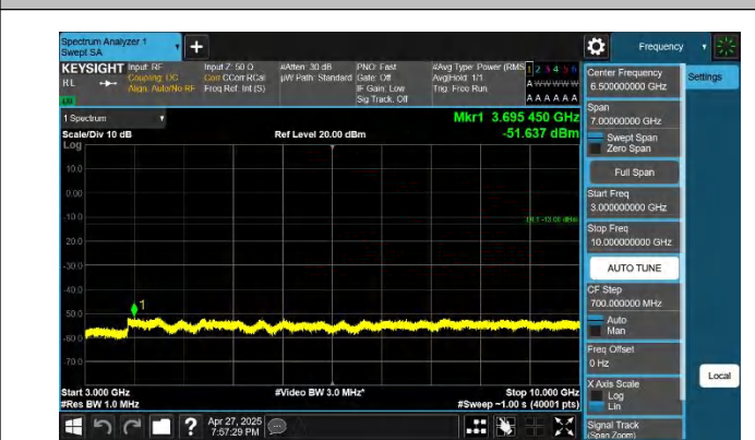
5-5-10MHz-5MHz-QPSK-QPSK-20550-20622-1RB#49-ORB#0-30 00~10000MHz-PASS
