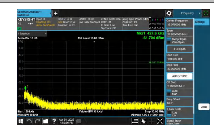
5-5-10MHz-10MHz-QPSK-QPSK-20501-20600-1RB#49-0RB#0-0 .15~30MHz-PASS
