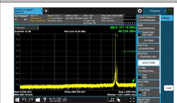
5-5-10MHz-10MHz-QPSK-QPSK-20476-20575-1RB#0-0RB#0-30 ~1000MHz-PASS
