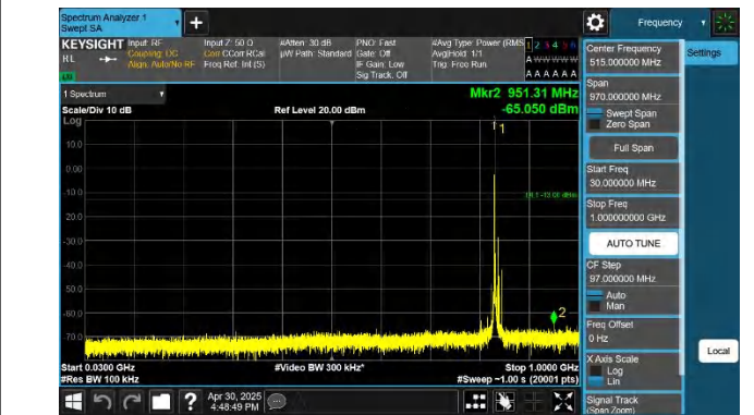
5-5-10MHz-5MHz-QPSK-QPSK-20550-20622-1RB#0-ORB#0-30~ 1000MHz-PASS
