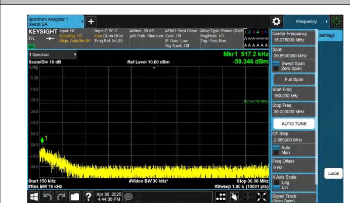
5-5-5MHz-10MHz-QPSK-QPSK-20528-20600-1RB#24-ORB#0-0. 15~30MHz-PASS
