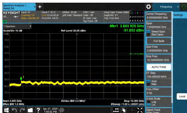
5-5-10MHz-10MHz-QPSK-QPSK-20450-20549-1RB#0-0RB#0-30 00~10000MHz-PASS
