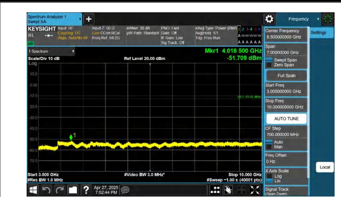
5-5-10MHz-5MHz-QPSK-QPSK-20450-20522-1RB#0-0RB#0-300 0~10000MHz-PASS
