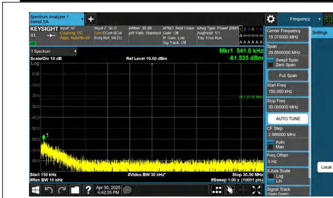
5-5-5MHz-10MHz-QPSK-QPSK-20428-20500-1RB#0-1RB#49-0. 15~30MHz-PASS
