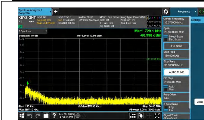
5-5-10MHz-10MHz-QPSK-QPSK-20450-20549-1RB#0-1RB#49-0 .15~30MHz-PASS
