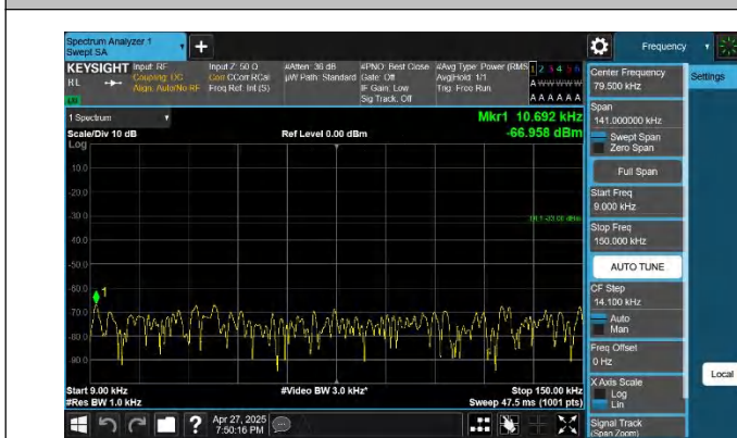
5-5-5MHz-10MHz-QPSK-QPSK-20528-20600-1RB#24-ORB#0-0. 009~0.15MHz-PASS
