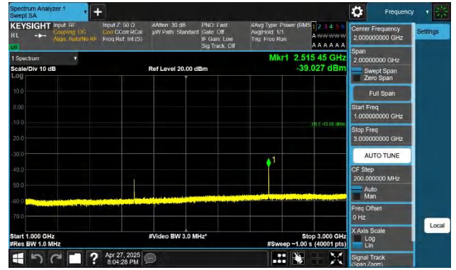
5-5-10MHz-10MHz-QPSK-QPSK-20501-20600-1RB#49-0RB#0-1 000~3000MHz-PASS
