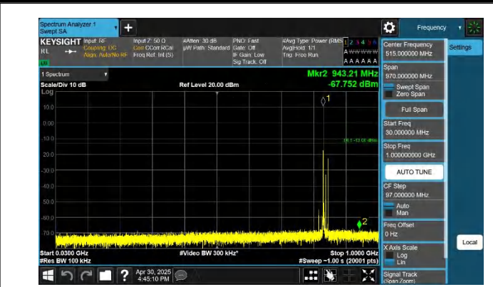
5-5-5MHz-10MHz-QPSK-QPSK-20528-20600-1RB#0-1RB#49-30 ~1000MHz-PASS
