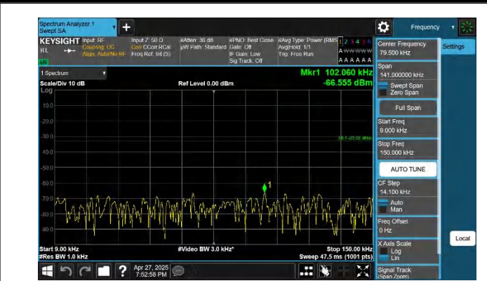
5-5-10MHz-5MHz-QPSK-QPSK-20450-20522-1RB#49-0RB#0-0. 009~0.15MHz-PASS
