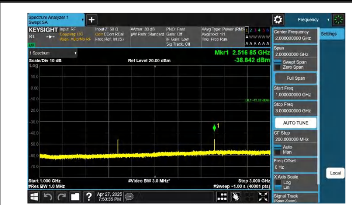
5-5-5MHz-10MHz-QPSK-QPSK-20528-20600-1RB#24-ORB#0-10 00~3000MHz-PASS
