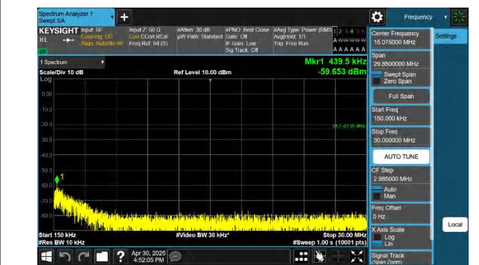
5-5-10MHz-10MHz-QPSK-QPSK-20476-20575-1RB#0-1RB#49-0 .15~30MHz-PASS
