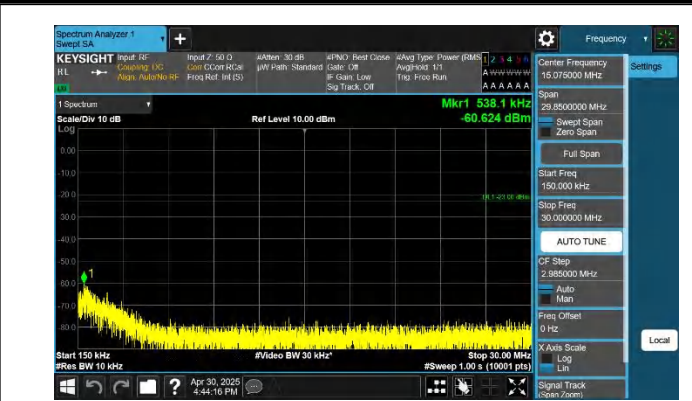
5-5-5MHz-10MHz-QPSK-QPSK-20528-20600-1RB#0-ORB#0-0.1 5~30MHz-PASS
