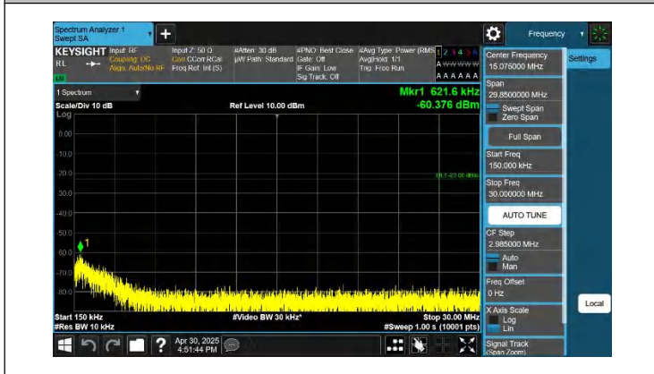
5-5-10MHz-10MHz-QPSK-QPSK-20476-20575-1RB#49-0RB#0-0 .15~30MHz-PASS
