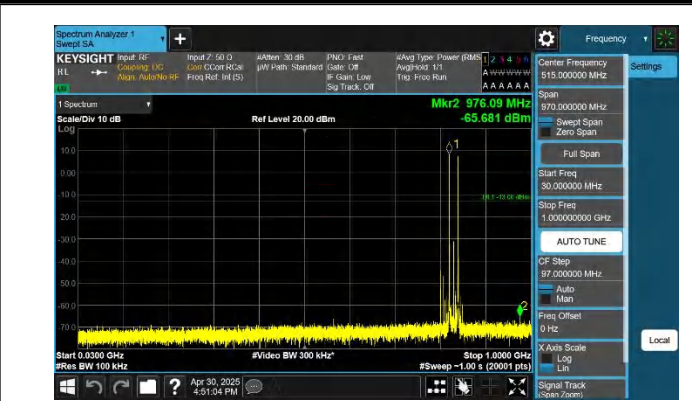
5-5-10MHz-10MHz-QPSK-QPSK-20450-20549-1RB#0-1RB#49-3 0~1000MHz-PASS
