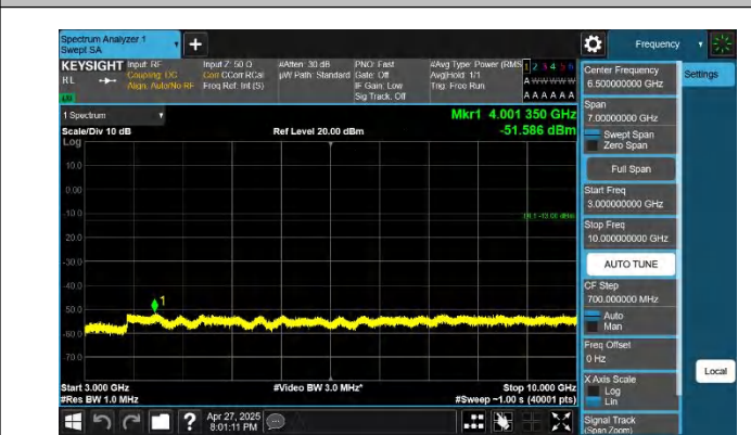
5-5-10MHz-10MHz-QPSK-QPSK-20450-20549-1RB#0-1RB#49-3 000~10000MHz-PASS
