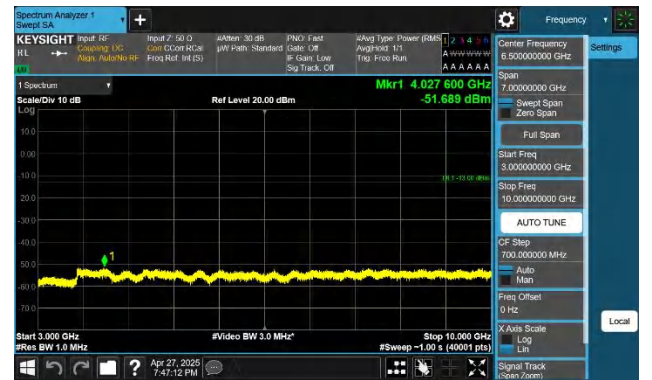
5-5-5MHz-10MHz-QPSK-QPSK-20428-20500-1RB#0-1RB#49-30 00~10000MHz-PASS
