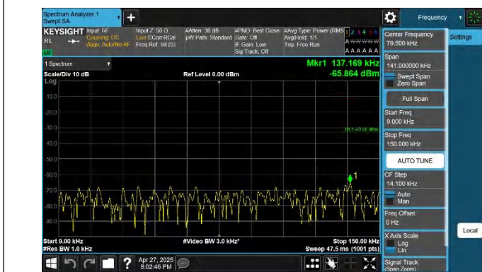
5-5-10MHz-10MHz-QPSK-QPSK-20476-20575-1RB#0-1RB#49-0 .009~0.15MHz-PASS
