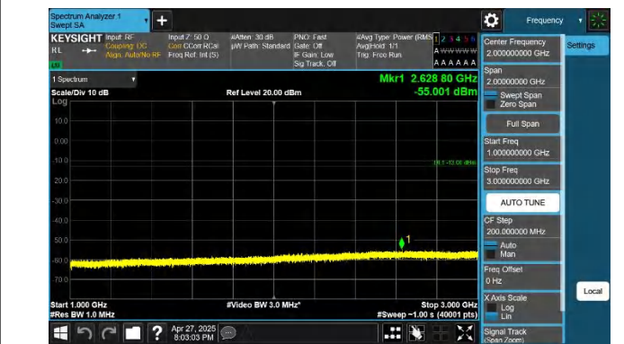
5-5-10MHz-10MHz-QPSK-QPSK-20476-20575-1RB#0-1RB#49-1 000~3000MHz-PASS
