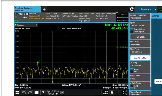
5-5-10MHz-10MHz-QPSK-QPSK-20450-20549-1RB#49-0RB#0-0 .009~0.15MHz-PASS
