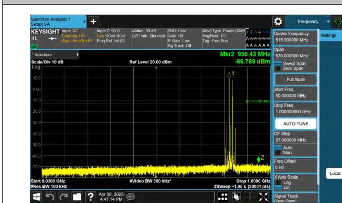
5-5-10MHz-5MHz-QPSK-QPSK-20450-20522-1RB#0-1RB#24-30 ~1000MHz-PASS
