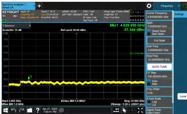
5-5-5MHz-10MHz-QPSK-QPSK-20528-20600-1RB#24-ORB#0-30 00~10000MHz-PASS
