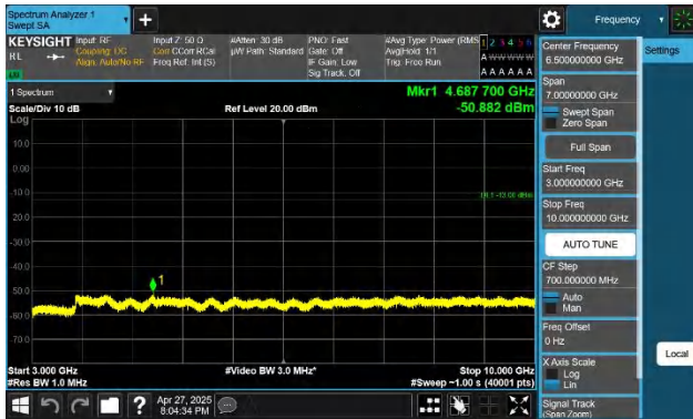
5-5-10MHz-10MHz-QPSK-QPSK-20501-20600-1RB#49-0RB#0-3 000~10000MHz-PASS
