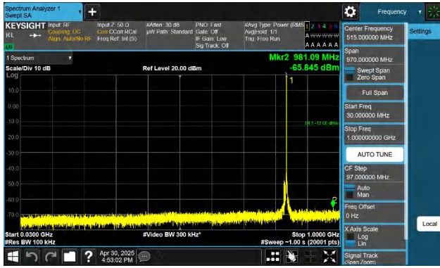
5-5-10MHz-10MHz-QPSK-QPSK-20501-20600-1RB#49-0RB#0-3 0~1000MHz-PASS
