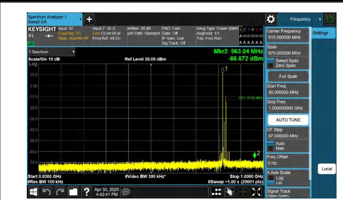
5-5-5MHz-10MHz-QPSK-QPSK-20428-20500-1RB#0-1RB#49-30 ~1000MHz-PASS
