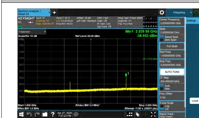
5-5-10MHz-5MHz-QPSK-QPSK-20550-20622-1RB#49-ORB#0-10 00~3000MHz-PASS
