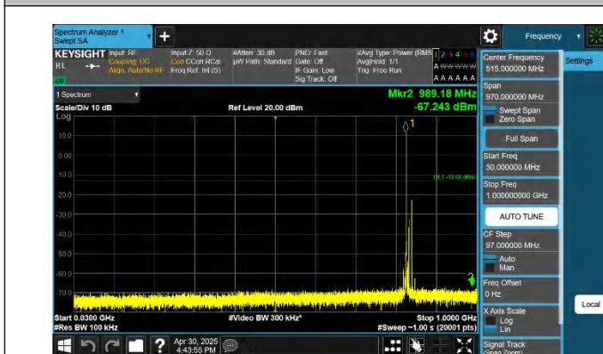
5-5-5MHz-10MHz-QPSK-QPSK-20478-20550-1RB#0-1RB#49-30 ~1000MHz-PASS
