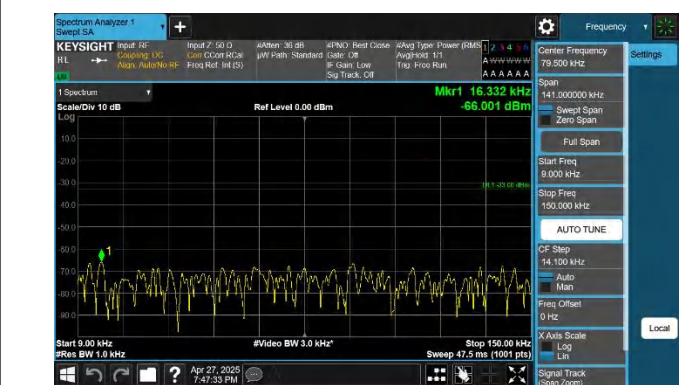
5-5-5MHz-10MHz-QPSK-QPSK-20478-20550-1RB#0-ORB#0-0.0 09~0.15MHz-PASS
