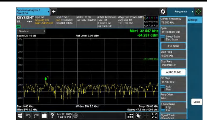
5-5-5MHz-10MHz-QPSK-QPSK-20478-20550-1RB#24-0RB#0-0. 009~0.15MHz-PASS
