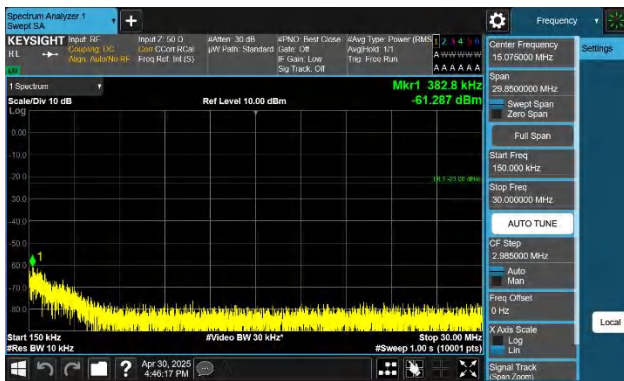
5-5-10MHz-5MHz-QPSK-QPSK-20450-20522-1RB#0-ORB#0-0.1 5~30MHz-PASS
