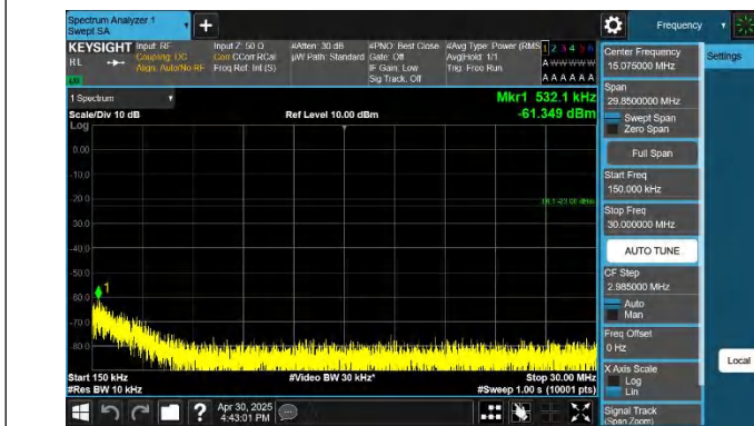
5-5-5MHz-10MHz-QPSK-QPSK-20478-20550-1RB#0-ORB#0-0.1 5~30MHz-PASS
