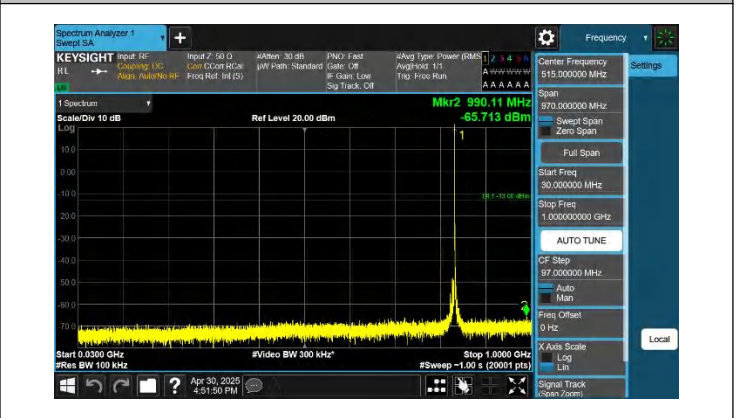
5-5-10MHz-10MHz-QPSK-QPSK-20476-20575-1RB#49-0RB#0-3 0~1000MHz-PASS
