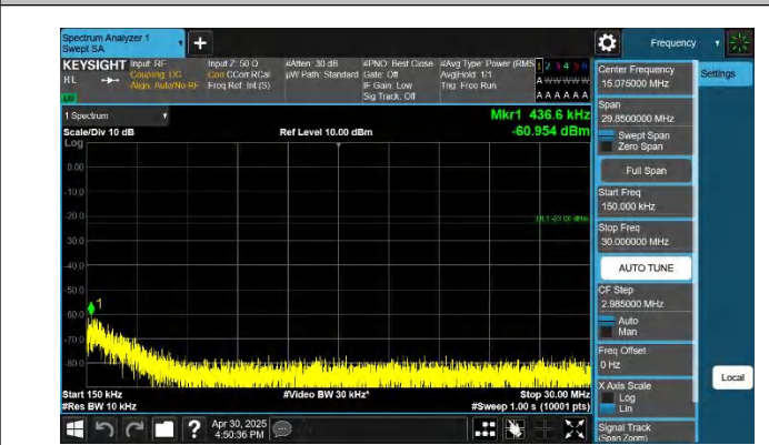
5-5-10MHz-10MHz-QPSK-QPSK-20450-20549-1RB#49-0RB#0-0 .15~30MHz-PASS
