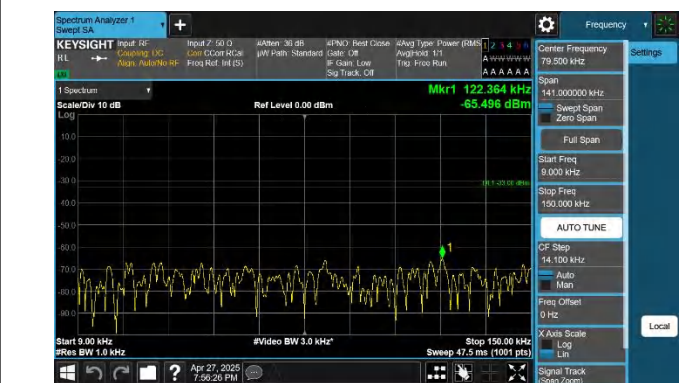
5-5-10MHz-5MHz-QPSK-QPSK-20550-20622-1RB#0-ORB#0-0.0 09~0.15MHz-PASS
