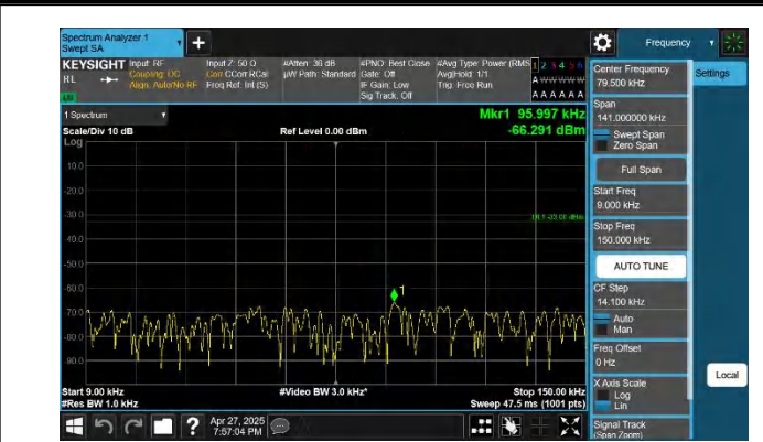
5-5-10MHz-5MHz-QPSK-QPSK-20550-20622-1RB#49-ORB#0-0. 009~0.15MHz-PASS
