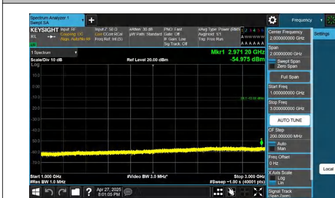
5-5-10MHz-10MHz-QPSK-QPSK-20450-20549-1RB#0-1RB#49-1 000~3000MHz-PASS
