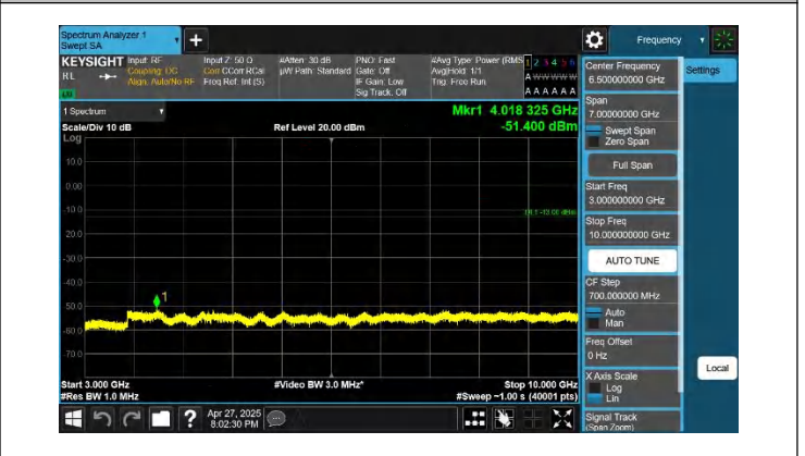
5-5-10MHz-10MHz-QPSK-QPSK-20476-20575-1RB#49-0RB#0-3 000~1000MHz-PASS
