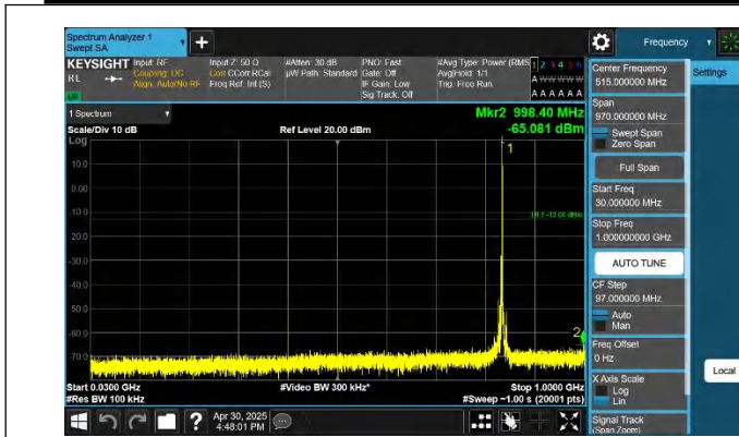
5-5-10MHz-5MHz-QPSK-QPSK-20500-20572-1RB#49-ORB#0-30 ~1000MHz-PASS
