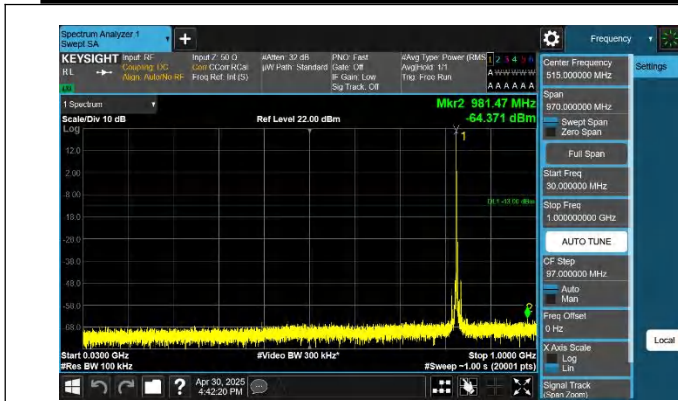
5-5-5MHz-10MHz-QPSK-QPSK-20428-20500-1RB#24-ORB#0-30 ~1000MHz-PASS
