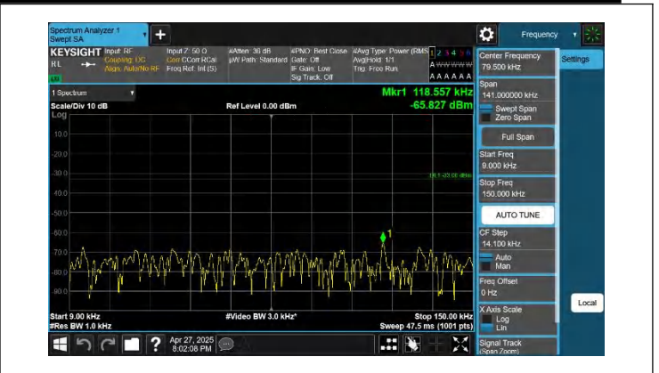
5-5-10MHz-10MHz-QPSK-QPSK-20476-20575-1RB#49-0RB#0-0 .009~0.15MHz-PASS
