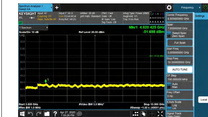
5-5-10MHz-5MHz-QPSK-QPSK-20500-20572-1RB#49-ORB#0-30 00~10000MHz-PASS
