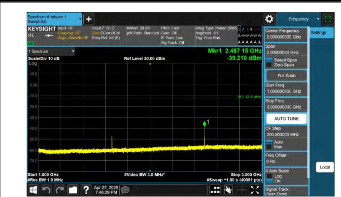
5-5-5MHz-10MHz-QPSK-QPSK-20428-20500-1RB#24-ORB#0-10 00~3000MHz-PASS
