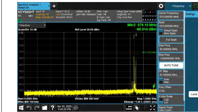
5-5-10MHz-5MHz-QPSK-QPSK-20550-20622-1RB#0-1RB#24-30 ~1000MHz-PASS
