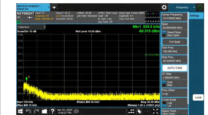
5-5-10MHz-5MHz-QPSK-QPSK-20550-20622-1RB#0-1RB#24-0. 15~30MHz-PASS
