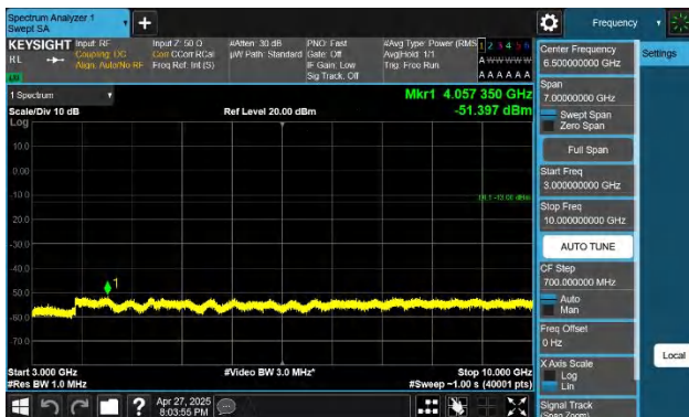
5-5-10MHz-10MHz-QPSK-QPSK-20501-20600-1RB#0-0RB#0-30 00~10000MHz-PASS
