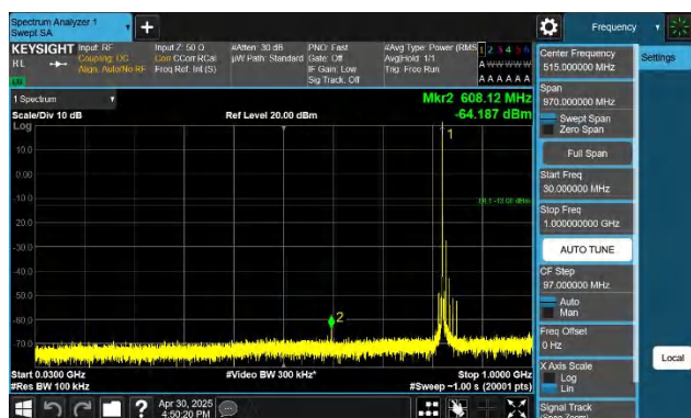
5-5-10MHz-10MHz-QPSK-QPSK-20450-20549-1RB#0-0RB#0-30 ~1000MHz-PASS
