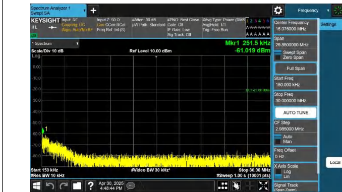
5-5-10MHz-5MHz-QPSK-QPSK-20550-20622-1RB#0-ORB#0-0.1 5~30MHz-PASS
