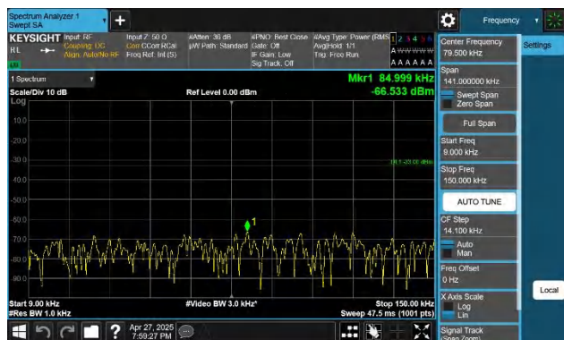
5-5-10MHz-10MHz-QPSK-QPSK-20450-20549-1RB#0-0RB#0-0. 009~0.15MHz-PASS
