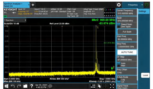
5-5-10MHz-5MHz-QPSK-QPSK-20450-20522-1RB#0-ORB#0-30~ 1000MHz-PASS
