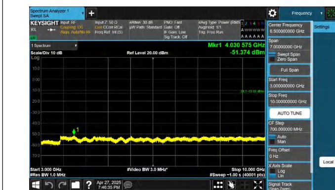
5-5-5MHz-10MHz-QPSK-QPSK-20428-20500-1RB#24-ORB#0-30 00~10000MHz-PASS
