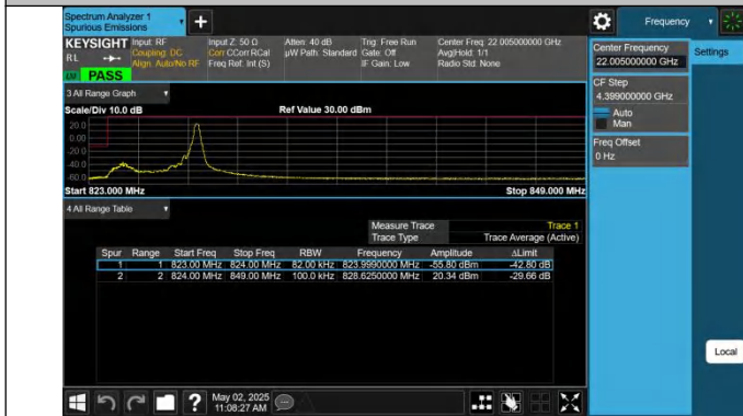
5-5-5MHz-3MHz-QPSK@QPSK-QPSK@QPSK-20425-20464-1R B#24@25RB#0-0RB#0@15RB#0-PASS
