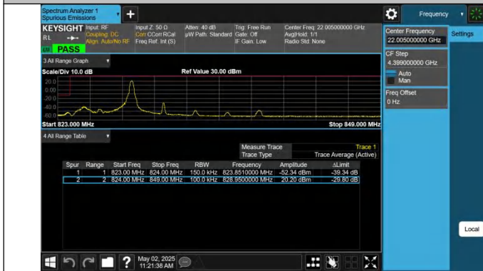
5-5-5MHz-10MHz-QPSK@QPSK-QPSK-20428-20500-1 RB#24@25RB#0-0RB#0@50RB#0-PASS
