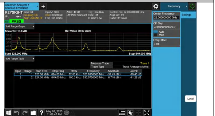
5-5-5MHz-3MHz-QPSK@QPSK-QPSK@QPSK-20425-20464-1R B#0@25RB#0-1RB#15@15RB#0-PASS
