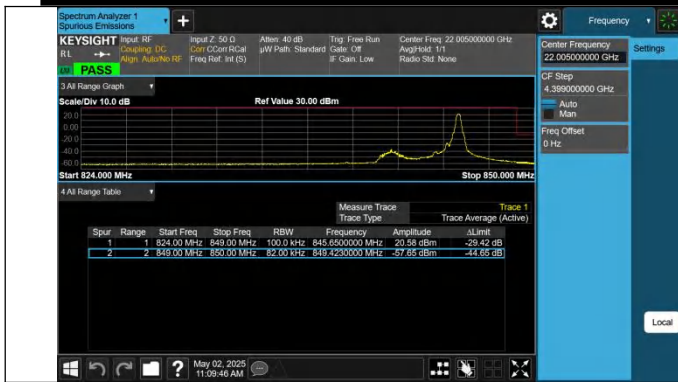
5-5-5MHz-3MHz-QPSK@QPSK-QPSK-20595-20634-1R B#24@25RB#0-0RB#0@15RB#0-PASS
