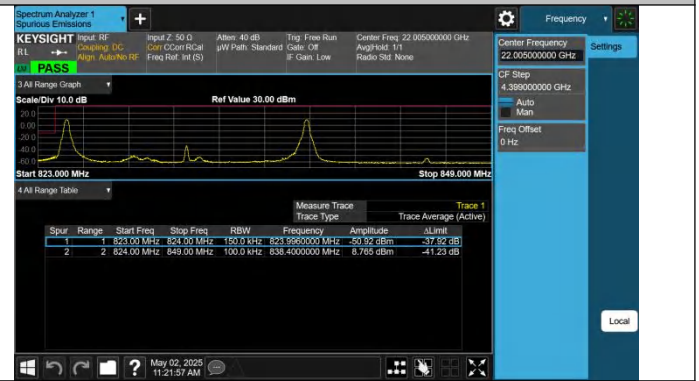
5-5-5MHz-10MHz-QPSK@QPSK-QPSK-20428-20500-1 RB#0@25RB#0-1RB#49@50RB#0-PASS
