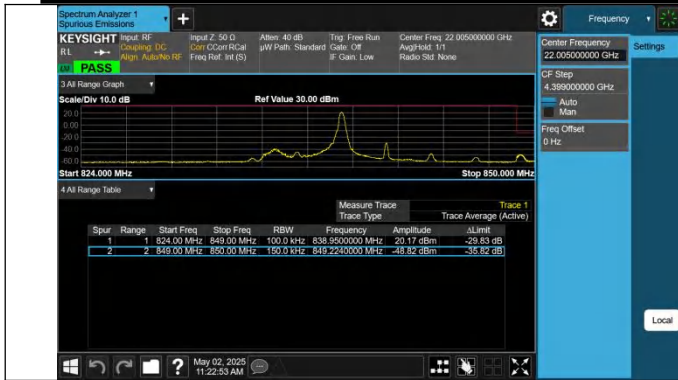
5-5-5MHz-10MHz-QPSK@QPSK-QPSK@QPSK-20528-20600-1 RB#24@25RB#0-0RB#0@50RB#0-PASS
