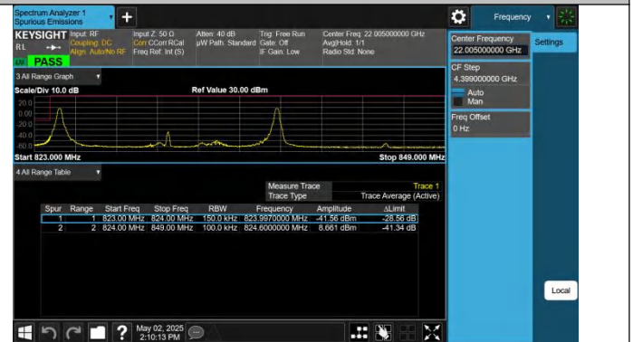
5-5-10MHz-5MHz-QPSK@QPSK-QPSK@QPSK-20450-20522-1 RB#0@50RB#0-1RB#24@25RB#0-PASS
