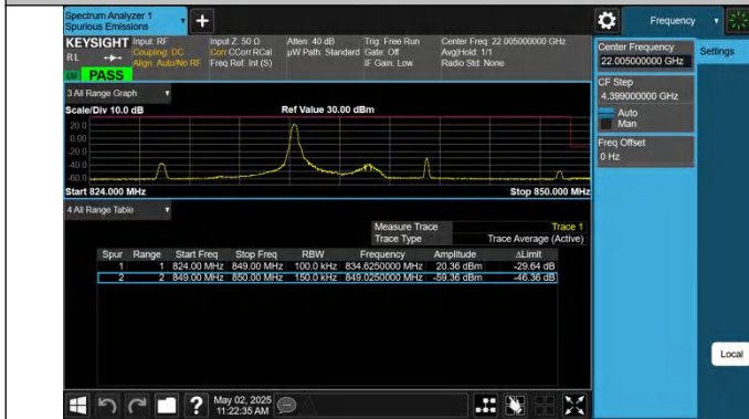
5-5-5MHz-10MHz-QPSK@QPSK-QPSK-20528-20600-1 RB#0@25RB#0-0RB#0@50RB#0-PASS
