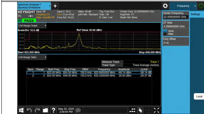
5-5-10MHz-5MHz-QPSK@QPSK-QPSK@QPSK-20450-20522-1 RB#49@50RB#0-0RB#0@25RB#0-PASS
