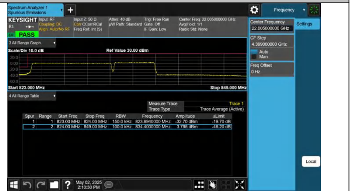
5-5-10MHz-5MHz-QPSK@QPSK-QPSK@QPSK-20450-20522-50 RB#0@50RB#0-25RB#0@25RB#0-PASS
