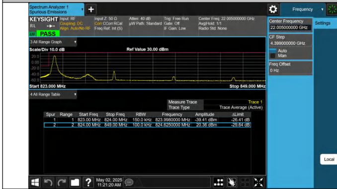
5-5-5MHz-10MHz-QPSK@QPSK-QPSK-20428-20500-1 RB#0@25RB#0-0RB#0@50RB#0-PASS
