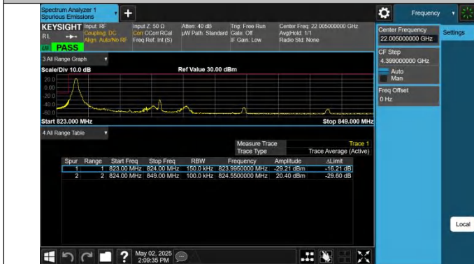
5-5-10MHz-5MHz-QPSK@QPSK-QPSK@QPSK-20450-20522-1 RB#0@50RB#0-0RB#0@25RB#0-PASS
