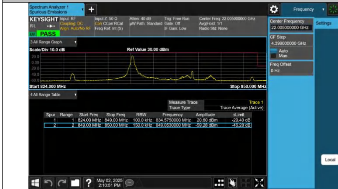
5-5-10MHz-5MHz-QPSK@QPSK-QPSK@QPSK-20550-20622-1 RB#0@50RB#0-0RB#0@25RB#0-PASS
