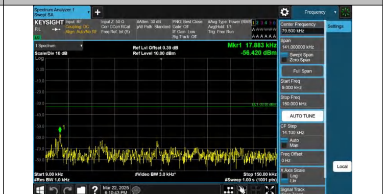
Band71-10MHz-QPSK-133422-1RB#49-0.009~0.15-PASS
