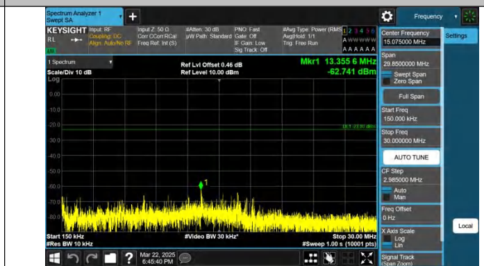
Band71-20MHz-QPSK-133222-1RB#0-0.15~30-PASS
