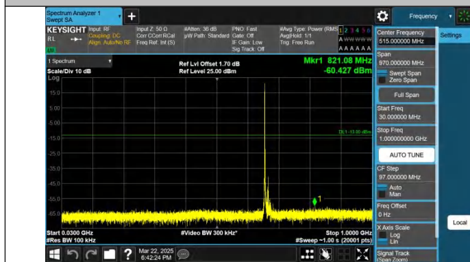
Band71-20MHz-QPSK-133222-1RB#0-30~1000-PASS
