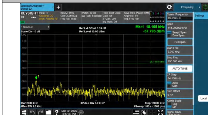
Band71-5MHz-QPSK-133447-1RB#0-0.009~0.15-PASS
