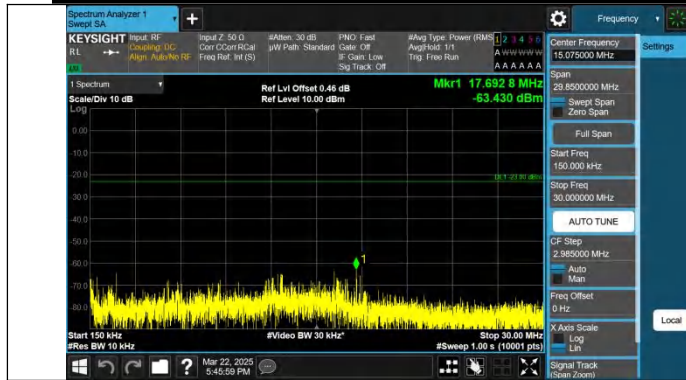
Band71-5MHz-QPSK-133297-1RB#24-0.15~30-PASS
