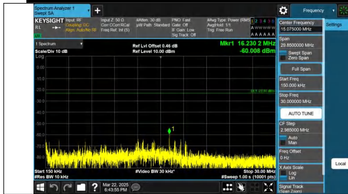
Band71-20MHz-QPSK-133222-1RB#99-0.15~30-PASS
