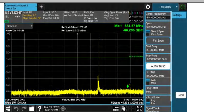
Band71-10MHz-QPSK-133172-1RB#49-30~1000-PASS
