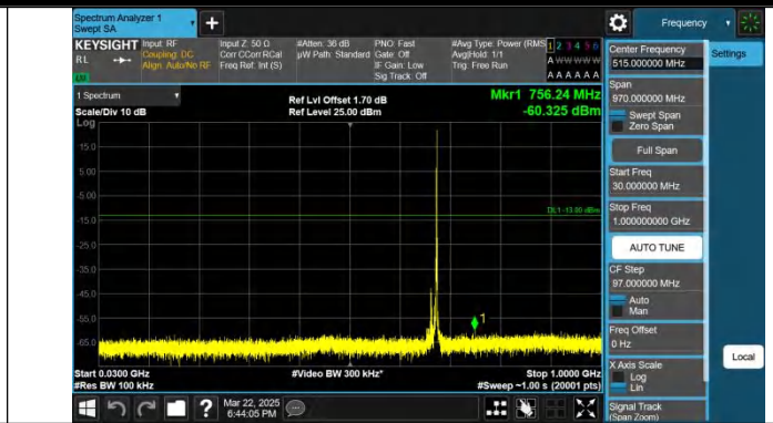
Band71-20MHz-QPSK-133222-1RB#99-30~1000-PASS
