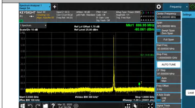
Band71-5MHz-QPSK-133447-1RB#0-30~1000-PASS
