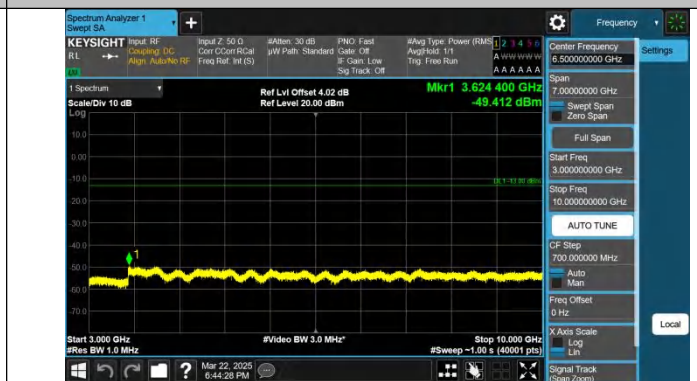
Band71-20MHz-QPSK-133222-1RB#99-3000~10000-PASS
