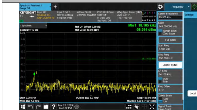
Band71-20MHz-QPSK-133222-1RB#0-0.009~0.15-PASS
