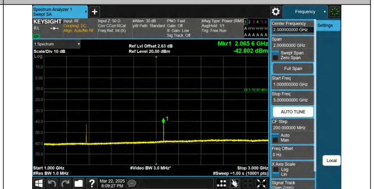
Band71-10MHz-QPSK-133422-1RB#0-1000~3000-PASS
