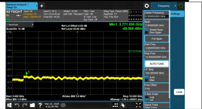
Band71-15MHz-QPSK-133397-1RB#74-3000~10000-PASS
