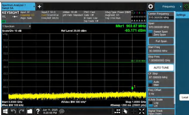
Band43(3700-3800)-20MHz-QPSK-45490-1RB#0-30~1000-PASS
