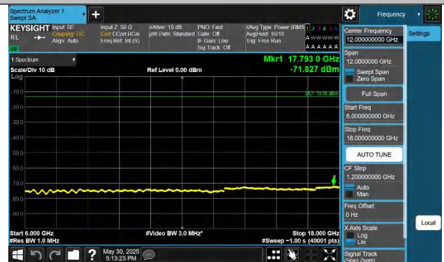
Band43(3700-3800)-20MHz-QPSK-45490-100RB#0-6000~18000-
