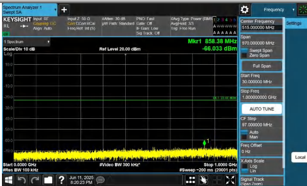
Band43(3700-3800)-20MHz-QPSK-44690-100RB#0-30~1000-PAS
