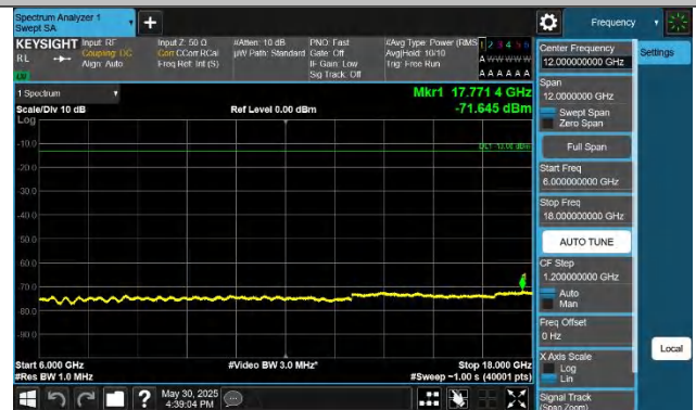
Band43(3700-3800)-10MHz-QPSK-45090-1RB#0-6000~18000-PA
