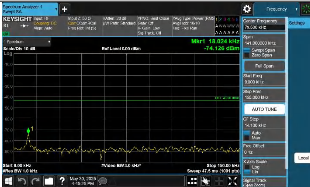
Band43(3700-3800)-15MHz-QPSK-44665-1RB#0-0.009~0.15-PAS
