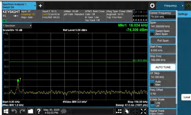
Band43(3700-3800)-15MHz-QPSK-45515-1RB#0-0.009~0.15-PAS
