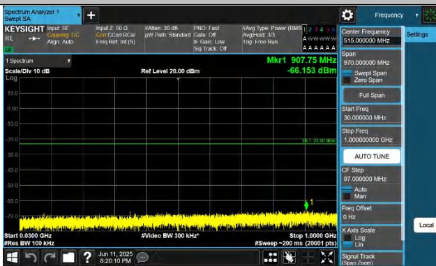
Band43(3700-3800)-20MHz-QPSK-44690-1RB#0-30~1000-PASS
