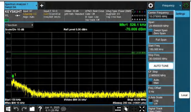
Band43(3700-3800)-10MHz-QPSK-45540-1RB#0-0.15~30-PASS
