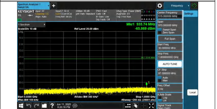
Band43(3700-3800)-20MHz-QPSK-44690-1RB#99-30~1000-PAS
