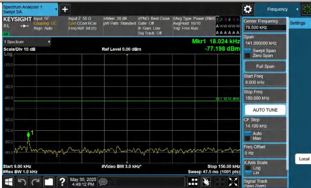
Band43(3700-3800)-15MHz-QPSK-45090-1RB#0-0.009~0.15-PAS
