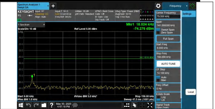
Band43(3700-3800)-15MHz-QPSK-44665-1RB#74-0.009~0.15-PA
