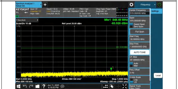
Band43(3700-3800)-15MHz-QPSK-45090-1RB#74-30~1000-PAS S
