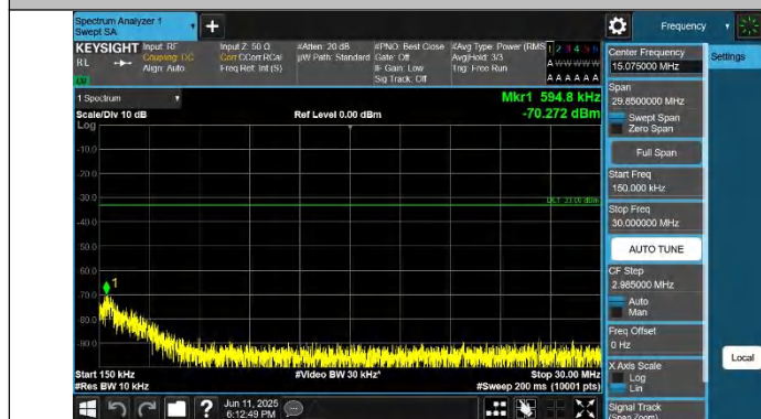
Band43(3700-3800)-20MHz-QPSK-45090-100RB#0-0.15~30-PAS
