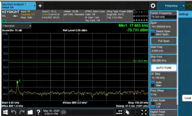
Band43(3700-3800)-20MHz-QPSK-44690-100RB#0-0.009~0.15-P
