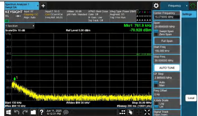
Band43(3700-3800)-20MHz-QPSK-44690-100RB#0-0.15~30-PAS
