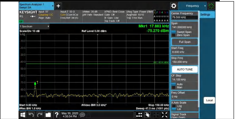
Band43(3700-3800)-10MHz-QPSK-44640-1RB#49-0.009~0.15-PA SS
