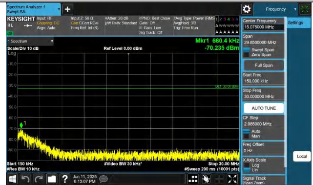
Band43(3700-3800)-20MHz-QPSK-45490-100RB#0-0.15~30-PAS
