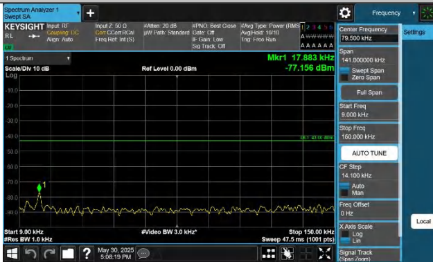
Band43(3700-3800)-20MHz-QPSK-45490-1RB#0-0.009~0.15-PASS
