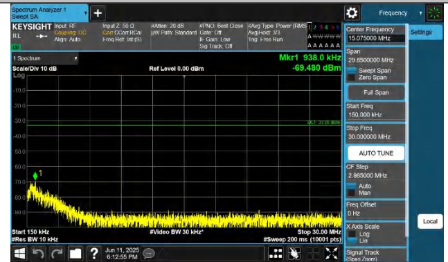
Band43(3700-3800)-20MHz-QPSK-45490-1RB#0-0.15~30-PASS
