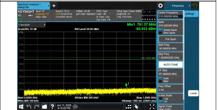
Band43(3700-3800)-10MHz-QPSK-44640-1RB#49-30~1000-PAS S
