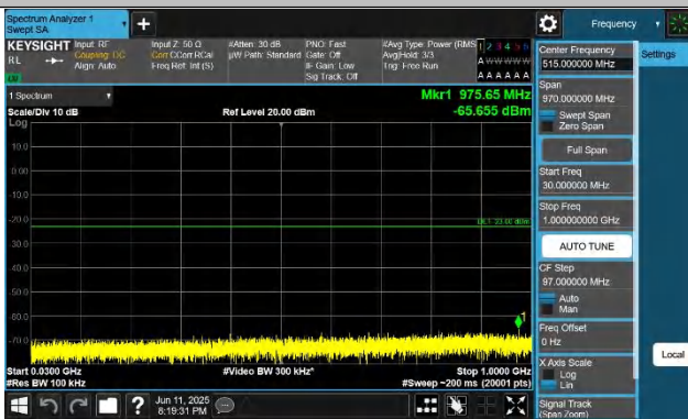
Band43(3700-3800)-15MHz-QPSK-44665-1RB#0-30~1000-PASS
