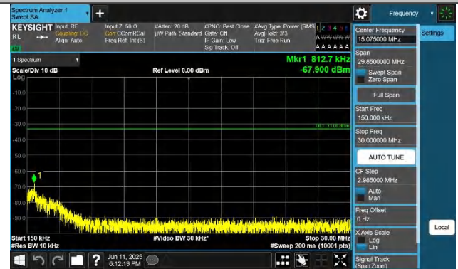
Band43(3700-3800)-20MHz-QPSK-44690-1RB#0-0.15~30-PASS
