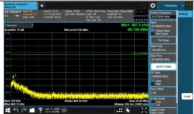
Band43(3700-3800)-10MHz-QPSK-45090-1RB#0-0.15~30-PASS
