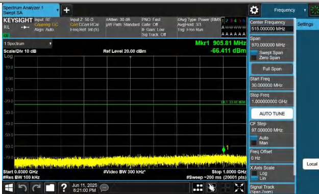
Band43(3700-3800)-20MHz-QPSK-45490-100RB#0-30~1000-PAS
