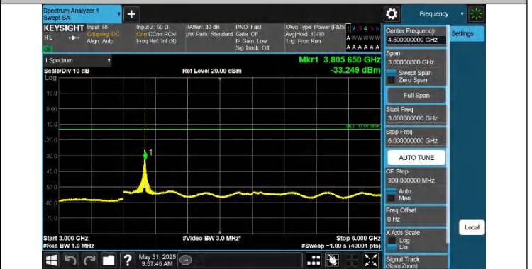
Band43(3700-3800)-20MHz-QPSK-45490-1RB#99-3000~6000-PA
