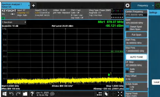
Band43(3700-3800)-15MHz-QPSK-45090-1RB#0-30~1000-PASS
