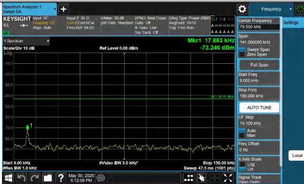
Band43(3700-3800)-20MHz-QPSK-45490-100RB#0-0.009~0.15-P
