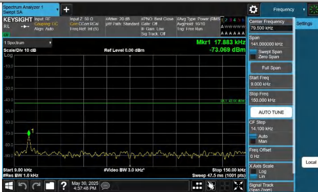
Band43(3700-3800)-10MHz-QPSK-45090-1RB#0-0.009~0.15-PAS
