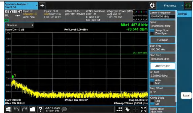
Band43(3700-3800)-15MHz-QPSK-44665-1RB#0-0.15~30-PASS
