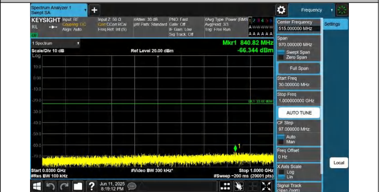
Band43(3700-3800)-10MHz-QPSK-45090-1RB#49-30~1000-PAS
