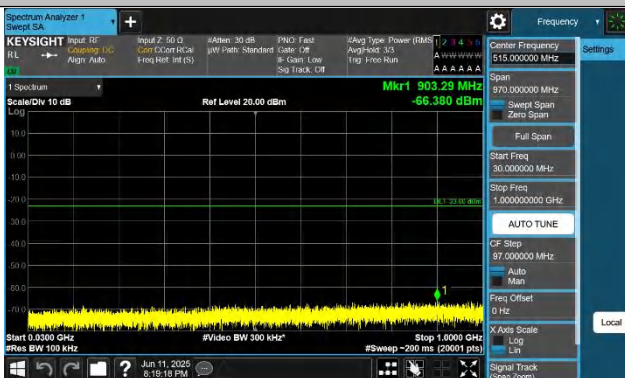
Band43(3700-3800)-10MHz-QPSK-45540-1RB#0-30~1000-PASS
