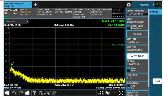
Band43(3700-3800)-15MHz-QPSK-45515-1RB#0-0.15~30-PASS
