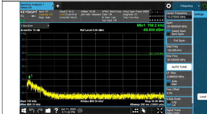
Band43(3700-3800)-10MHz-QPSK-45090-1RB#49-0.15~30-PASS
