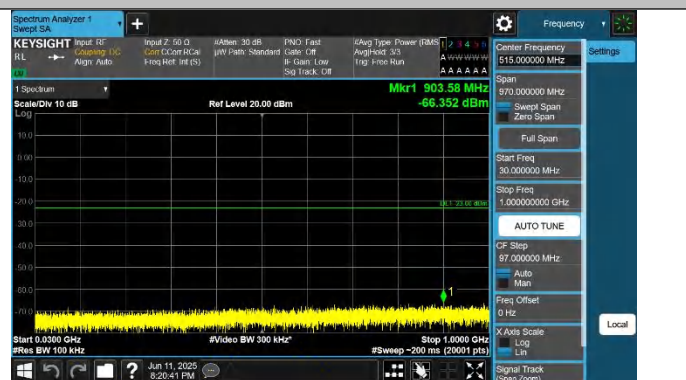
Band43(3700-3800)-20MHz-QPSK-45090-100RB#0-30~1000-PAS
