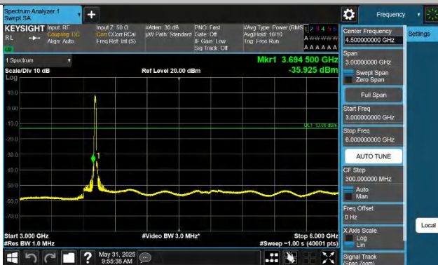
Band43(3700-3800)-20MHz-QPSK-44690-100RB#0-3000~6000-P
