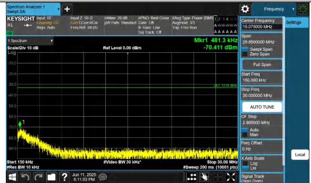
Band43(3700-3800)-15MHz-QPSK-45090-1RB#0-0.15~30-PASS
