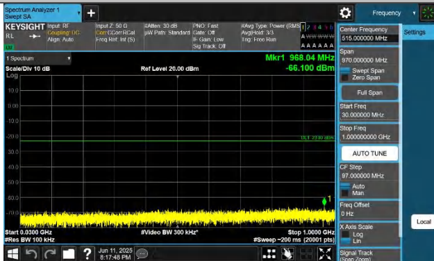
Band42(3450-3550)-20MHz-QPSK-42590-1RB#0-30~1000-PASS
