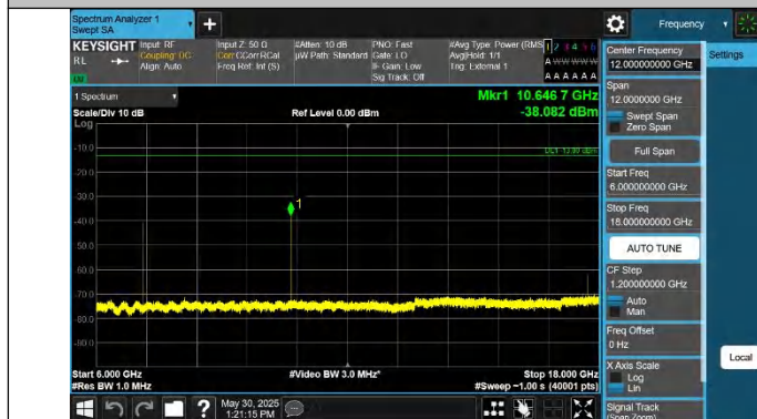
Band42(3450-3550)-20MHz-QPSK-42990-1RB#99-6000~18000-P
