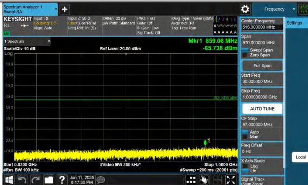
Band42(3450-3550)-20MHz-QPSK-42190-1RB#0-30~1000-PASS
