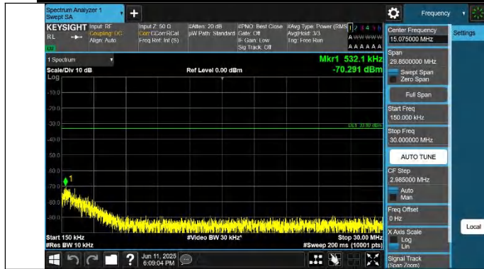
Band42(3450-3550)-10MHz-QPSK-43040-1RB#49-0.15~30-PAS
