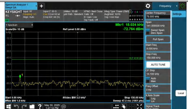
Band42(3450-3550)-15MHz-QPSK-42590-1RB#74-0.009~0.15-PA
