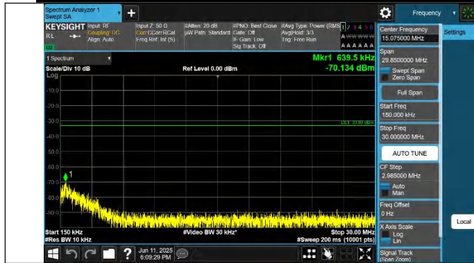
Band42(3450-3550)-15MHz-QPSK-42590-1RB#74-0.15~30-PAS
