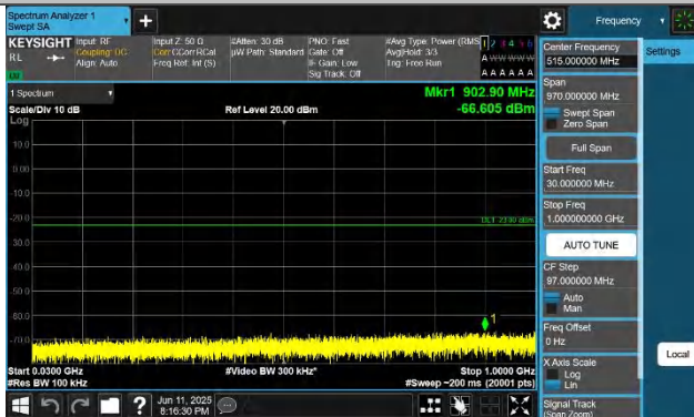
Band42(3450-3550)-10MHz-QPSK-42590-1RB#0-30~1000-PASS
