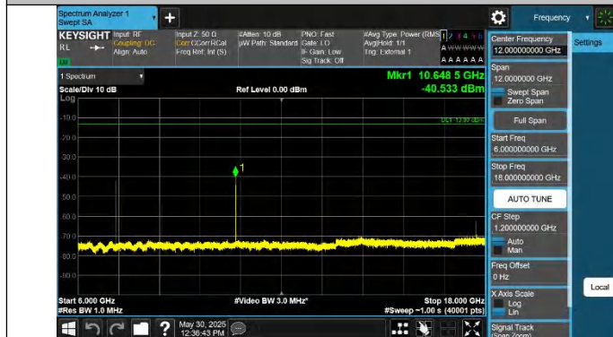
Band42(3450-3550)-10MHz-QPSK-43040-1RB#49-6000~18000-P
