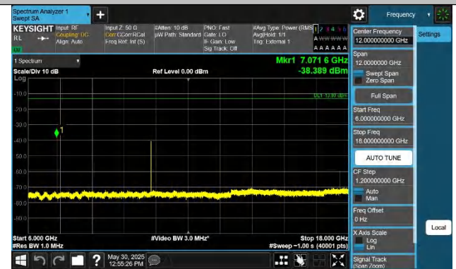
Band42(3450-3550)-15MHz-QPSK-43015-1RB#0-6000~18000-PA
