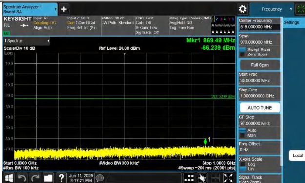
Band42(3450-3550)-15MHz-QPSK-43015-1RB#0-30~1000-PASS
