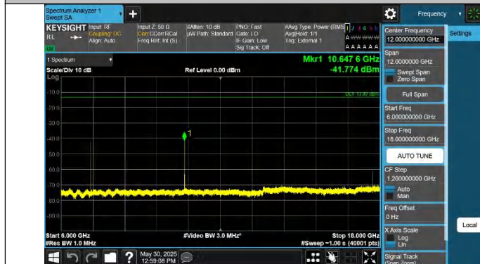
Band42(3450-3550)-15MHz-QPSK-43015-1RB#74-6000~18000-P
