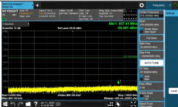
Band42(3450-3550)-15MHz-QPSK-42165-1RB#0-30~1000-PASS
