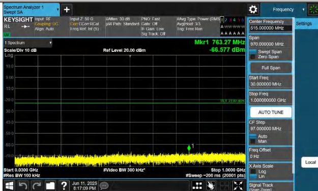
Band42(3450-3550)-15MHz-QPSK-42590-1RB#0-30~1000-PASS
