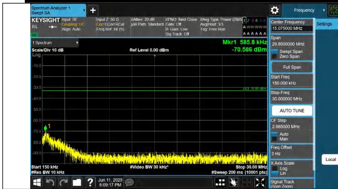
Band42(3450-3550)-15MHz-QPSK-42165-1RB#74-0.15~30-PAS
