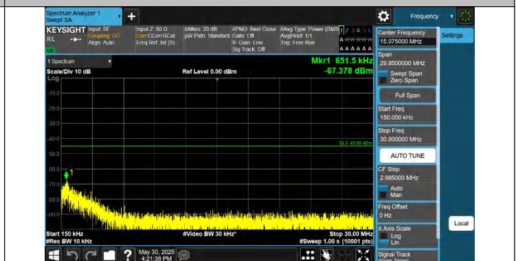
Band41-20MHz-QPSK-41490-1RB#0-0.15~30-PASS
