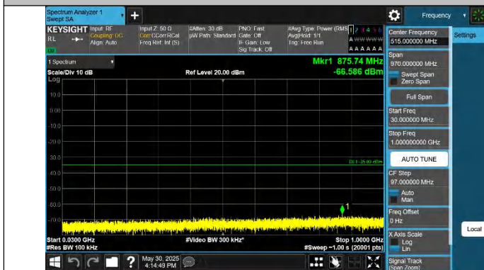
Band41-10MHz-QPSK-40620-1RB#0-30~1000-PASS
