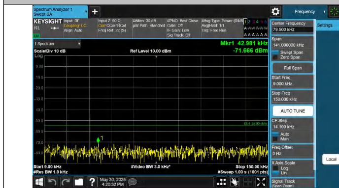
Band41-20MHz-QPSK-40620-1RB#0-0.009~0.15-PASS
