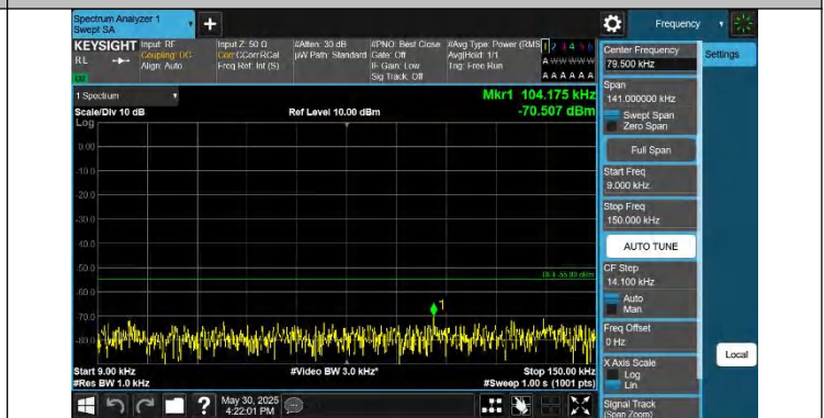
Band41-20MHz-QPSK-41490-1RB#99-0.009~0.15-PASS
