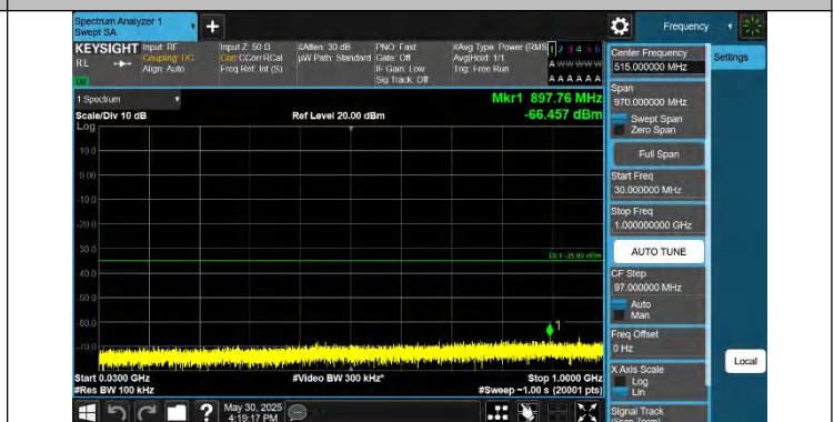
Band41-15MHz-QPSK-41515-1RB#74-30~1000-PASS
