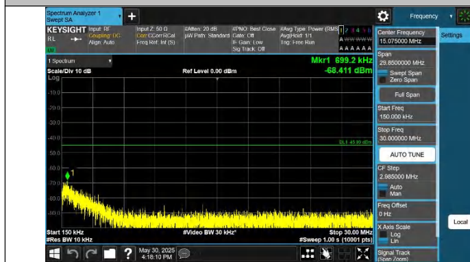
Band41-15MHz-QPSK-40620-1RB#74-0.15~30-PASS
