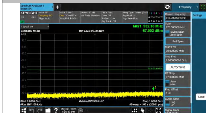
Band41-20MHz-QPSK-40620-1RB#0-30~1000-PASS
