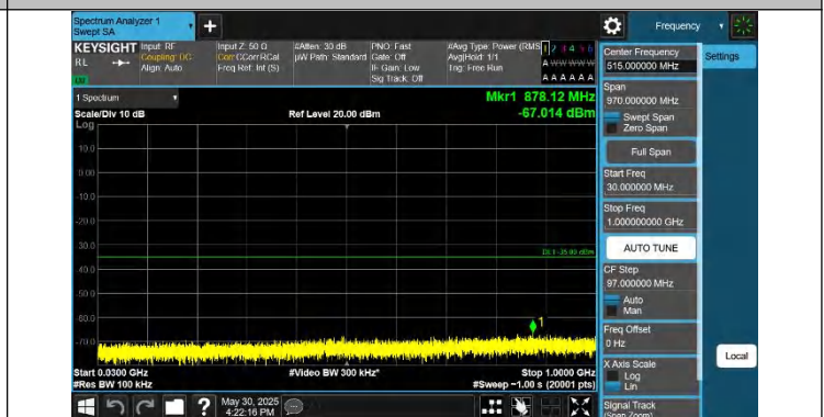
Band41-20MHz-QPSK-41490-1RB#99-30~1000-PASS
