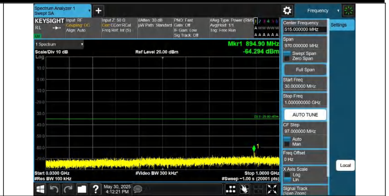
Band41-5MHz-QPSK-40620-1RB#24-30~1000-PASS
