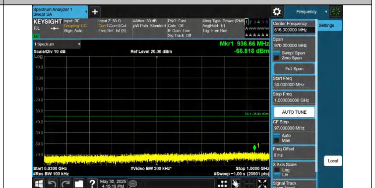
Band41-10MHz-QPSK-40620-1RB#49-30~1000-PASS
