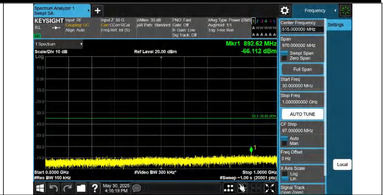
Band41-10MHz-QPSK-41540-1RB#49-30~1000-PASS
