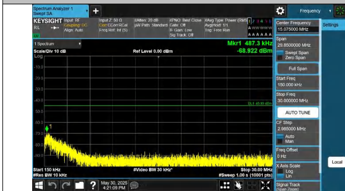
Band41-20MHz-QPSK-40620-1RB#99-0.15~30-PASS
