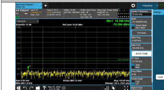
Band41-20MHz-QPSK-41490-1RB#0-0.009~0.15-PASS
