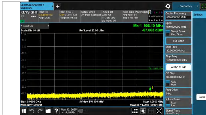
Band41-15MHz-QPSK-40620-1RB#0-30~1000-PASS
