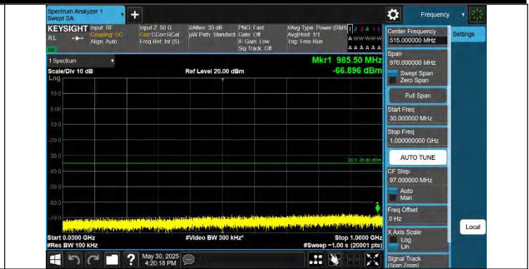
Band41-20MHz-QPSK-39750-1RB#99-30~1000-PASS
