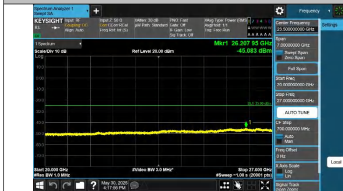
Band41-15MHz-QPSK-40620-1RB#0-20000~27000-PASS
