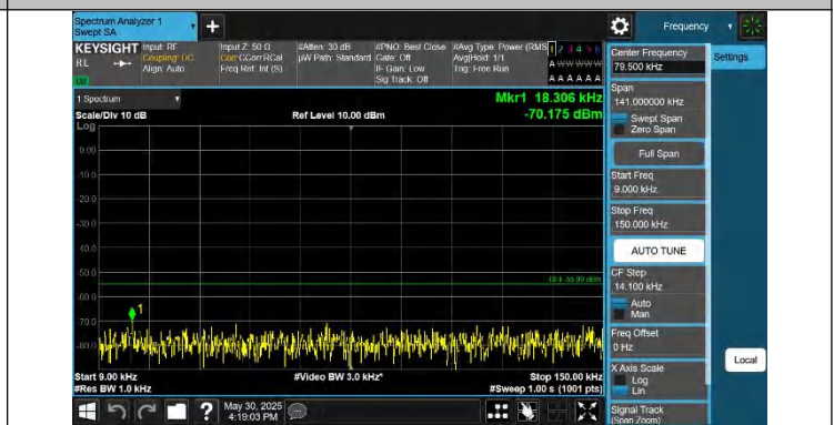
Band41-15MHz-QPSK-41515-1RB#74-0.009~0.15-PASS
