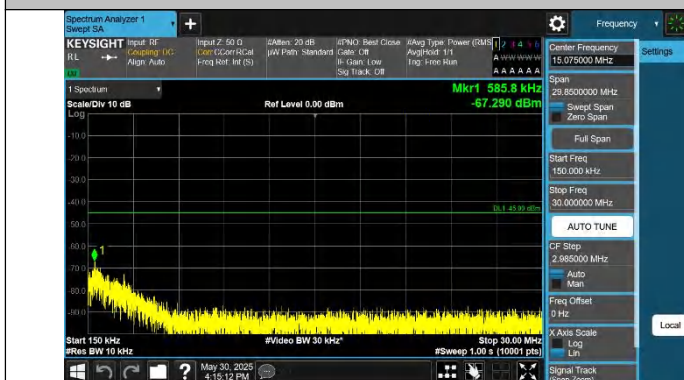
Band41-10MHz-QPSK-40620-1RB#49-0.15~30-PASS
