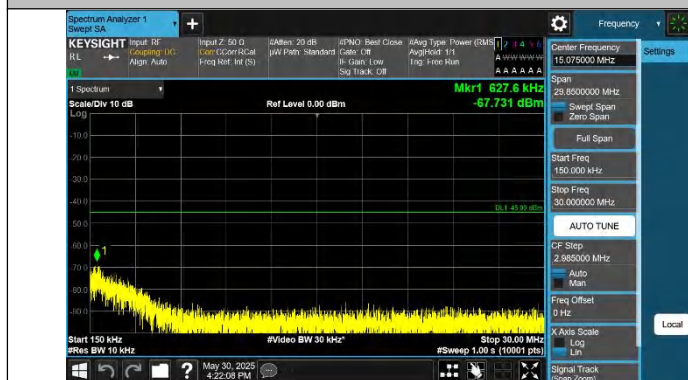
Band41-20MHz-QPSK-41490-1RB#99-0.15~30-PASS
