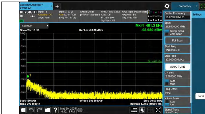
Band41-5MHz-QPSK-40620-1RB#24-0.15~30-PASS
