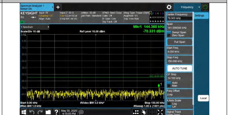
Band41-10MHz-QPSK-40620-1RB#49-0.009~0.15-PASS
