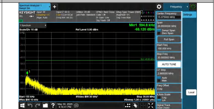
Band41-15MHz-QPSK-39725-1RB#0-0.15~30-PASS
