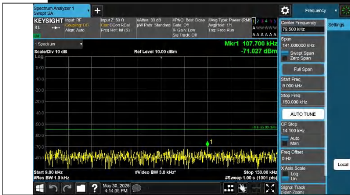
Band41-10MHz-QPSK-40620-1RB#0-0.009~0.15-PASS
