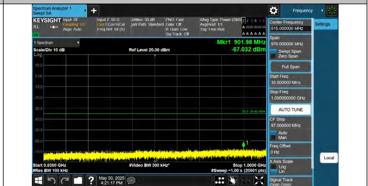
Band41-20MHz-QPSK-40620-1RB#99-30~1000-PASS
