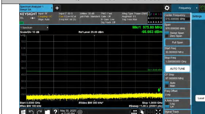
Band41-5MHz-QPSK-41565-1RB#0-30~1000-PASS
