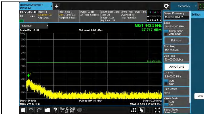
Band41-10MHz-QPSK-41540-1RB#49-0.15~30-PASS
