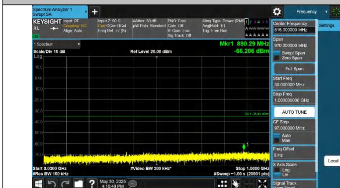
Band41-15MHz-QPSK-39725-1RB#0-30~1000-PASS
