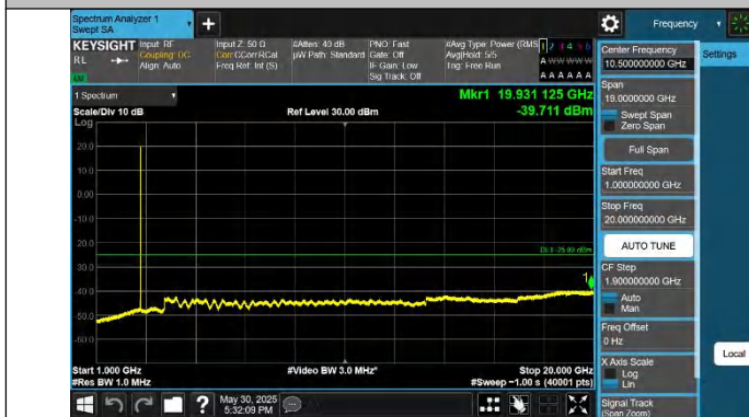
Band41-10MHz-QPSK-41540-1RB#49-1000~20000-PASS
