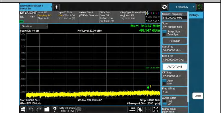
Band41-15MHz-QPSK-40620-1RB#74-30~1000-PASS
