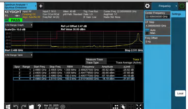
Band41-15MHz-QPSK-39725-1RB#74-PASS
