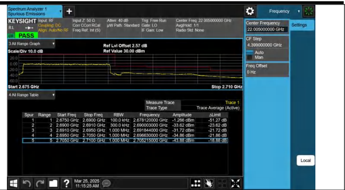
Band41-15MHz-QPSK-41515-75RB#0-PASS
