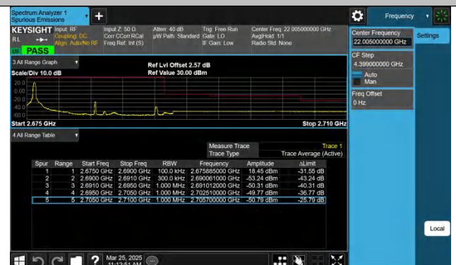
Band41-15MHz-QPSK-41515-1RB#0-PASS
