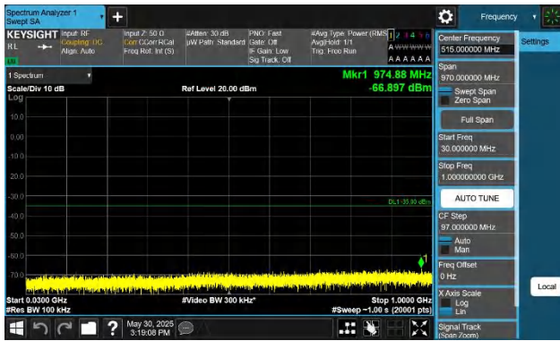
Band38-15MHz-QPSK-38000-1RB#0-30~1000-PASS
