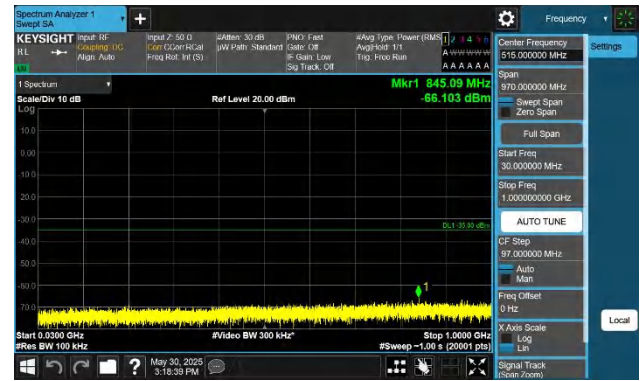
Band38-15MHz-QPSK-37825-1RB#74-30~1000-PASS
