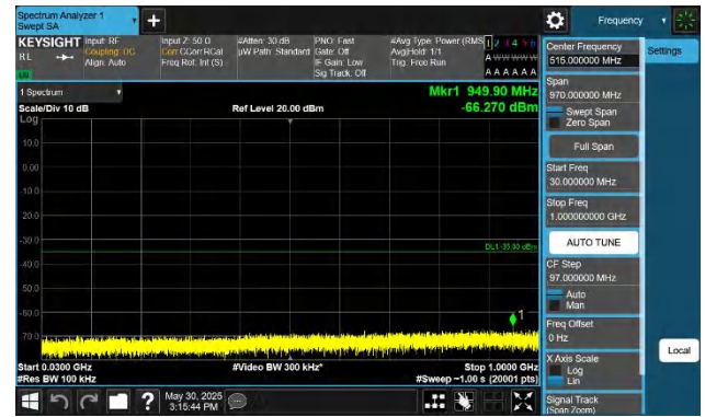
Band38-10MHz-QPSK-37800-1RB#49-30~1000-PASS
