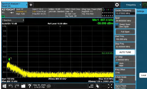
Band38-5MHz-QPSK-38225-1RB#24-0.15~30-PASS
