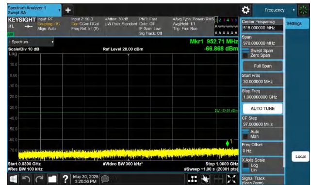
Band38-15MHz-QPSK-38175-1RB#74-30~1000-PASS
