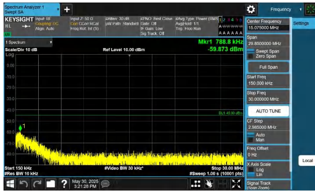
Band38-20MHz-QPSK-37850-1RB#99-0.15~30-PASS
