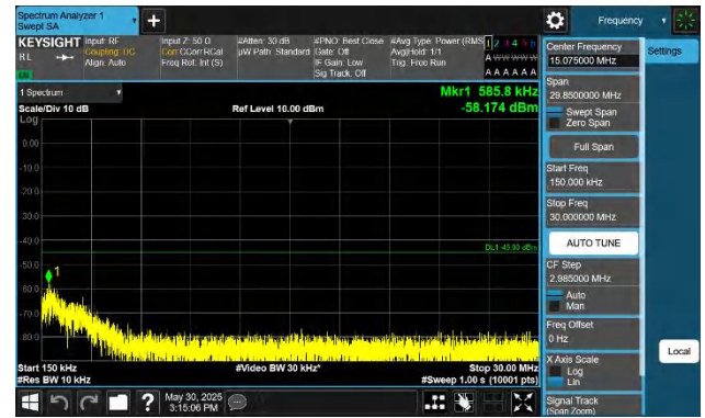
Band38-10MHz-QPSK-37800-1RB#0-0.15~30-PASS
