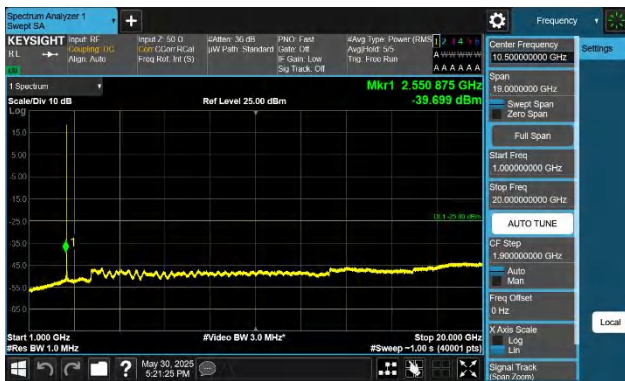
Band38-15MHz-QPSK-38175-1RB#74-1000~20000-PASS
