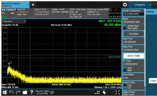
Band38-5MHz-QPSK-37775-1RB#24-0.15~30-PASS
