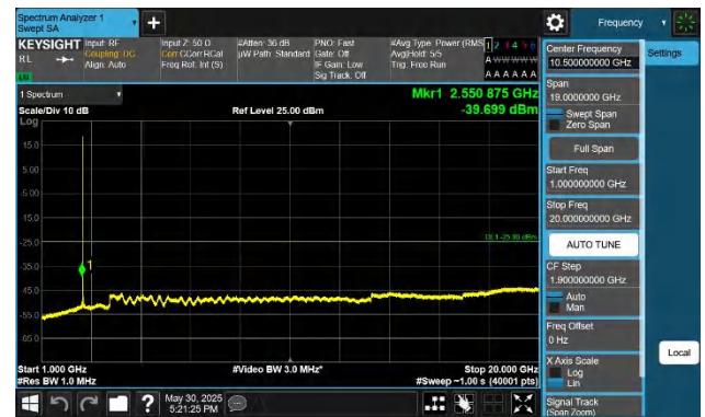
Band38-10MHz-QPSK-37800-1RB#0-1000~20000-PASS
