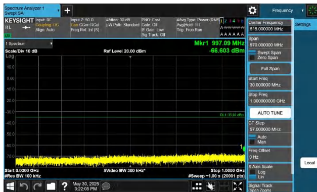
Band38-20MHz-QPSK-38000-1RB#0-30~1000-PASS
