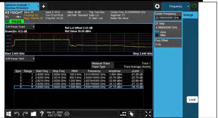
Band38-15MHz-QPSK-38175-75RB#0-PASS
