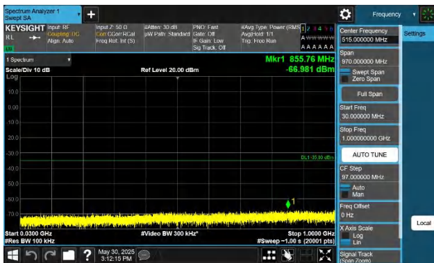
Band38-5MHz-QPSK-37775-1RB#0-30~1000-PASS
