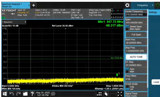
Band38-20MHz-QPSK-37850-1RB#0-30~1000-PASS
