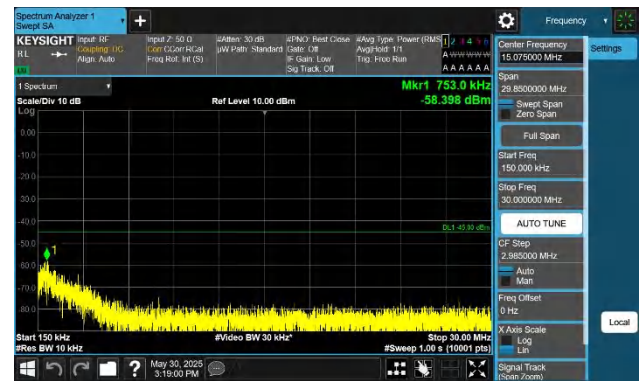
Band38-15MHz-QPSK-38000-1RB#0-0.15~30-PASS
