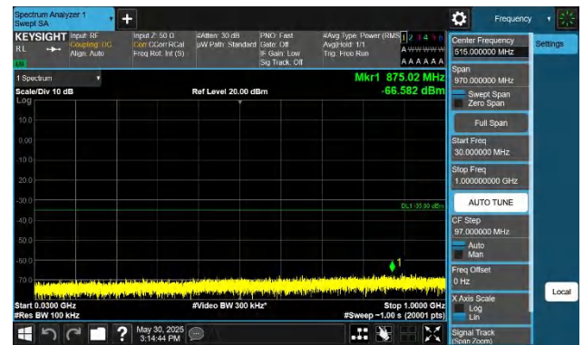
Band38-5MHz-QPSK-38225-1RB#24-30~1000-PASS
