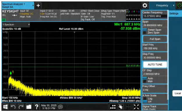
Band38-15MHz-QPSK-37825-1RB#74-0.15~30-PASS
