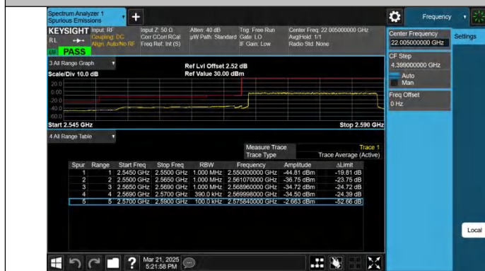
Band38-20MHz-QPSK-37850-100RB#0-PASS
