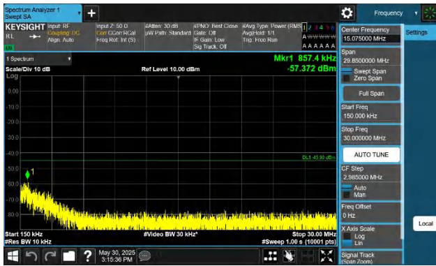
Band38-10MHz-QPSK-37800-1RB#49-0.15~30-PASS
