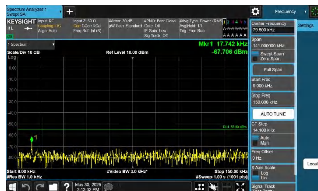
Band38-5MHz-QPSK-38000-1RB#24-0.009~0.15-PASS
