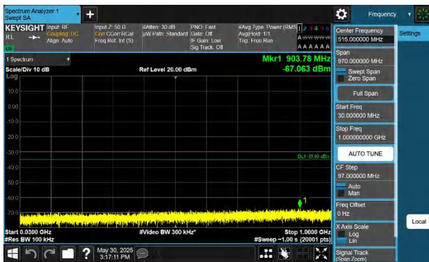
Band38-10MHz-QPSK-38200-1RB#0-30~1000-PASS
