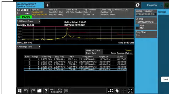
Band38-15MHz-QPSK-38175-1RB#74-PASS
