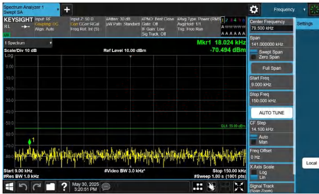
Band38-20MHz-QPSK-37850-1RB#0-0.009~0.15-PASS
