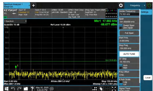
Band38-20MHz-QPSK-38000-1RB#99-0.009~0.15-PASS
