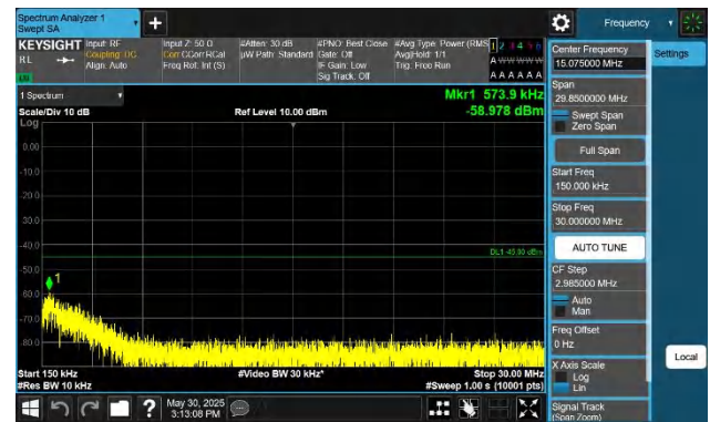
Band38-5MHz-QPSK-38000-1RB#0-0.15~30-PASS
