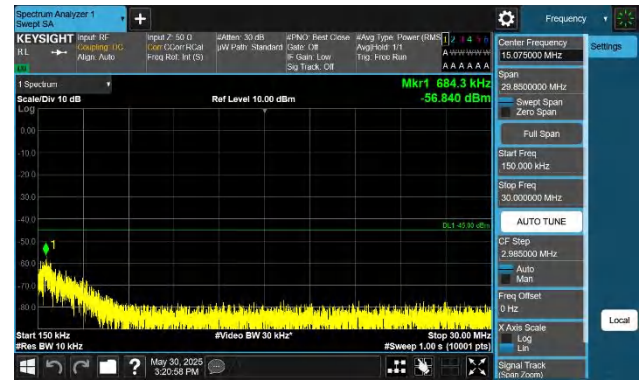
Band38-20MHz-QPSK-37850-1RB#0-0.15~30-PASS
