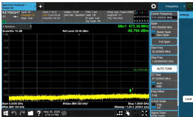
Band38-10MHz-QPSK-37800-1RB#0-30~1000-PASS
