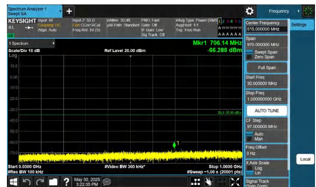
Band38-20MHz-QPSK-38000-1RB#99-30~1000-PASS
