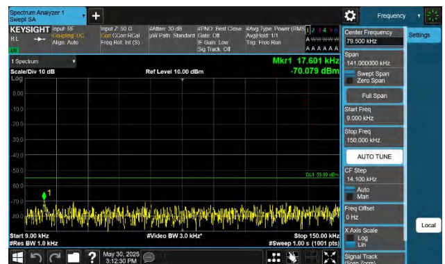
Band38-5MHz-QPSK-37775-1RB#24-0.009~0.15-PASS
