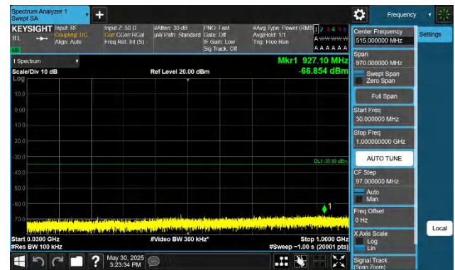
Band38-20MHz-QPSK-38150-1RB#99-30~1000-PASS
