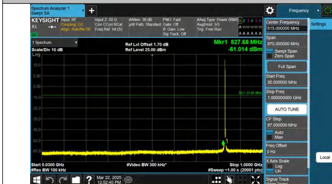
Band26(824-849)-3MHz-QPSK-26915-1RB#0-30~1000-PASS
