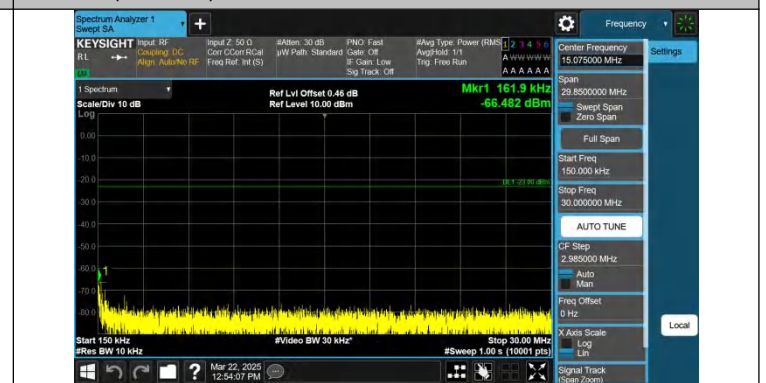
Band26(824-849)-3MHz-QPSK-27025-1RB#0-0.15~30-PASS
