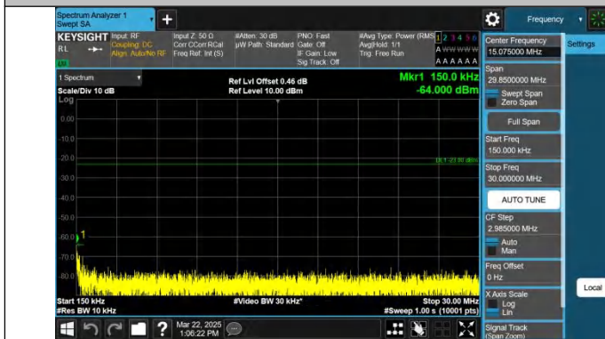
Band26(824-849)-5MHz-QPSK-26815-1RB#24-0.15~30-PASS
