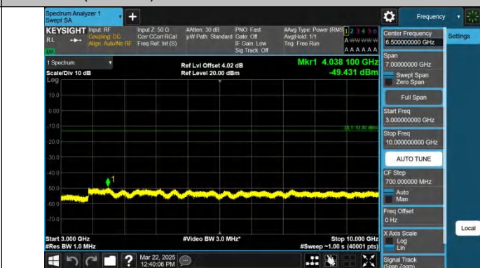
Band26(824-849)-1.4MHz-QPSK-27033-1RB#5-3000~10000-PAS
