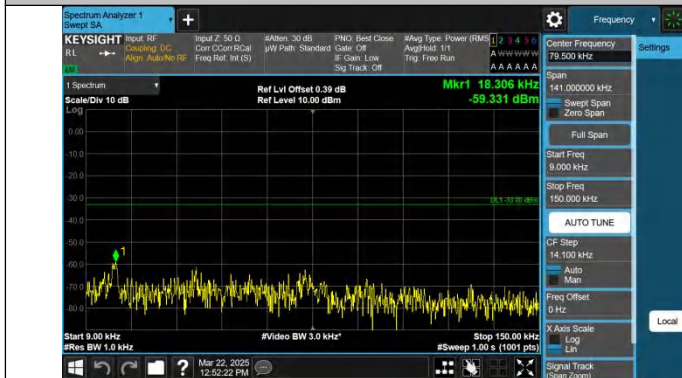
Band26(824-849)-3MHz-QPSK-26915-1RB#0-0.009~0.15-PASS
