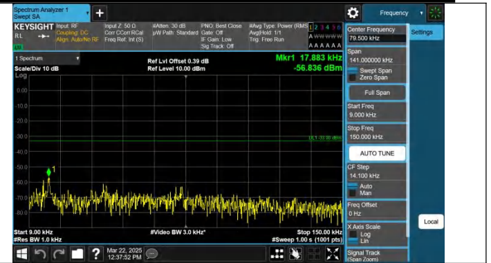
Band26(824-849)-1.4MHz-QPSK-26915-1RB#5-0.009~0.15-PASS
