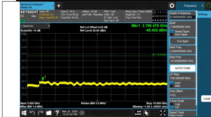
Band26(824-849)-1.4MHz-QPSK-26915-1RB#0-3000~10000-PASS S
