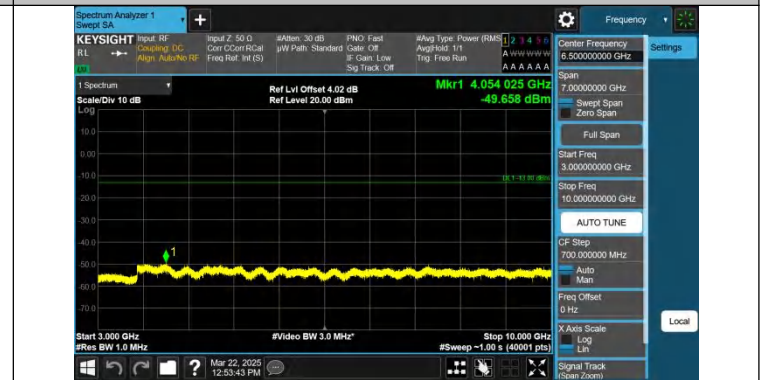
Band26(824-849)-3MHz-QPSK-26915-1RB#14-3000~10000-PASS
