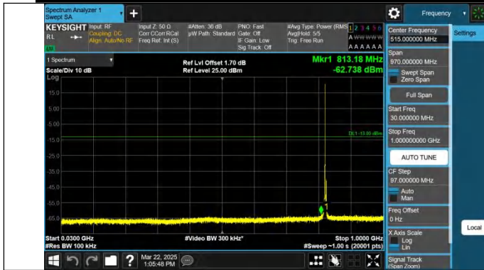
Band26(824-849)-5MHz-QPSK-26815-1RB#0-30~1000-PASS
