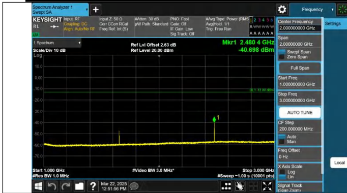
Band26(824-849)-3MHz-QPSK-26805-1RB#14-1000~3000-PASS
