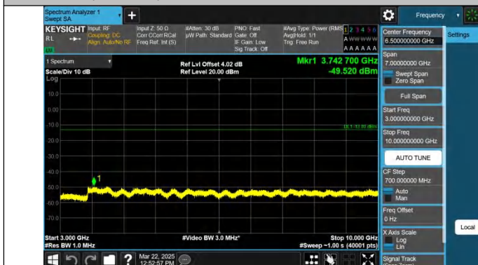
Band26(824-849)-3MHz-QPSK-26915-1RB#0-3000~10000-PASS
