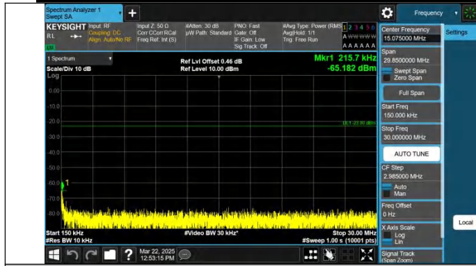
Band26(824-849)-3MHz-QPSK-26915-1RB#14-0.15~30-PASS
