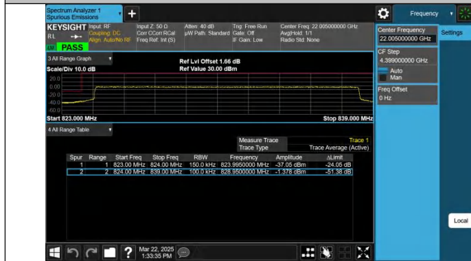
Band26(824-849)-15MHz-QPSK-26865-75RB#0-PASS
