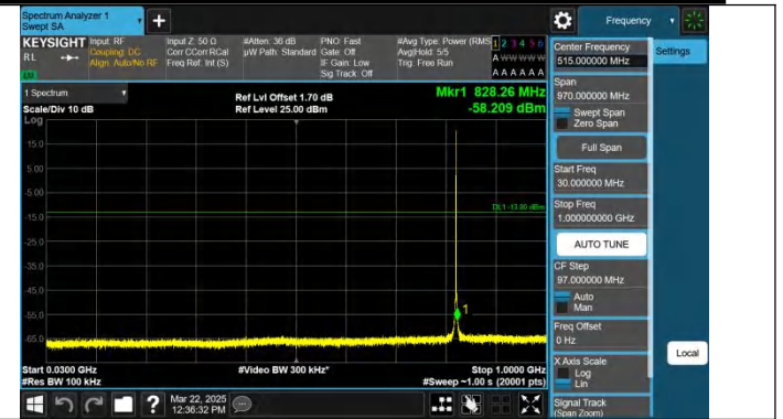
Band26(824-849)-1.4MHz-QPSK-26797-1RB#5-30~1000-PASS
