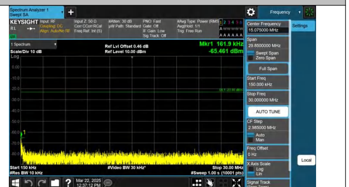
Band26(824-849)-1.4MHz-QPSK-26915-1RB#0-0.15~30-PASS
