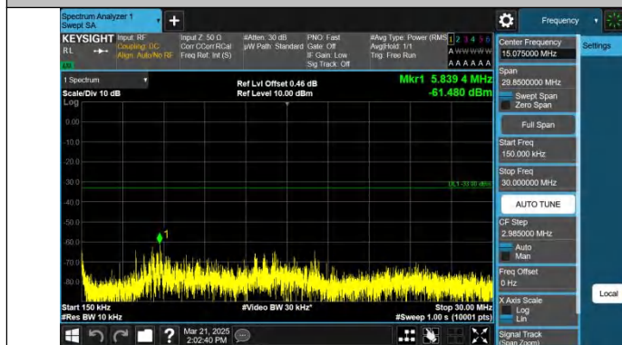
Band25-15MHz-QPSK-26615-1RB#74-0.15~30-PASS
