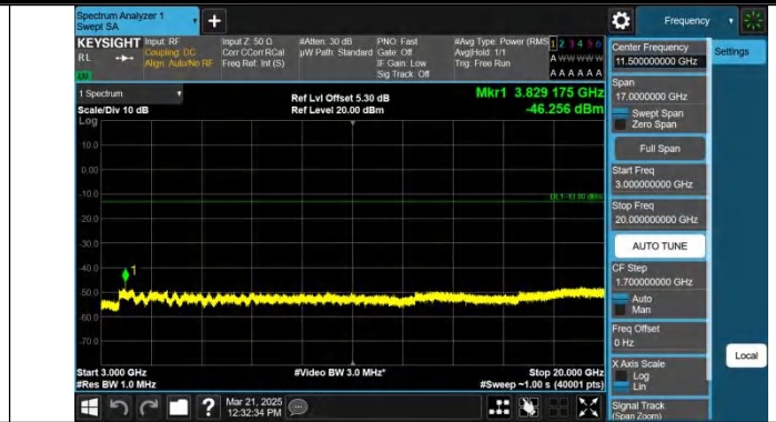
Band25-5MHz-QPSK-26665-1RB#24-3000~20000-PASS
