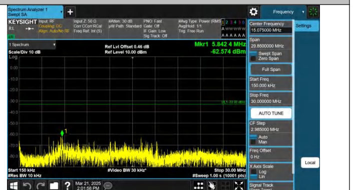
Band25-15MHz-QPSK-26615-1RB#0-0.15~30-PASS
