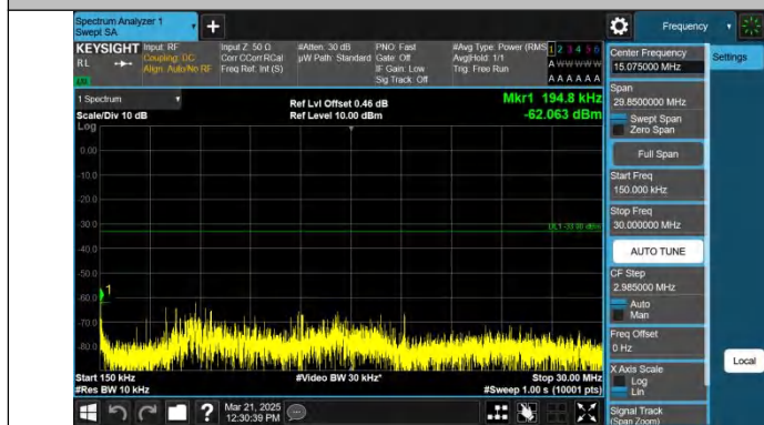
Band25-5MHz-QPSK-26365-1RB#24-0.15~30-PASS
