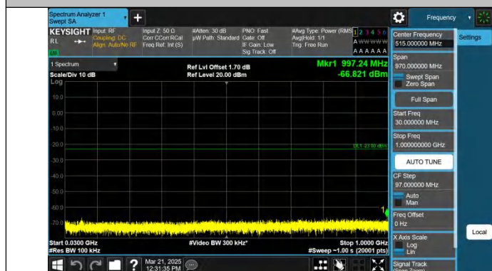
Band25-5MHz-QPSK-26665-1RB#0-30~1000-PASS
