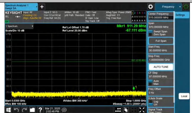
Band25-15MHz-QPSK-26615-1RB#74-30~1000-PASS
