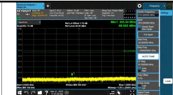
Band25-3MHz-QPSK-26675-1RB#14-30~1000-PASS
