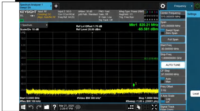
Band25-20MHz-QPSK-26140-1RB#0-30~1000-PASS
