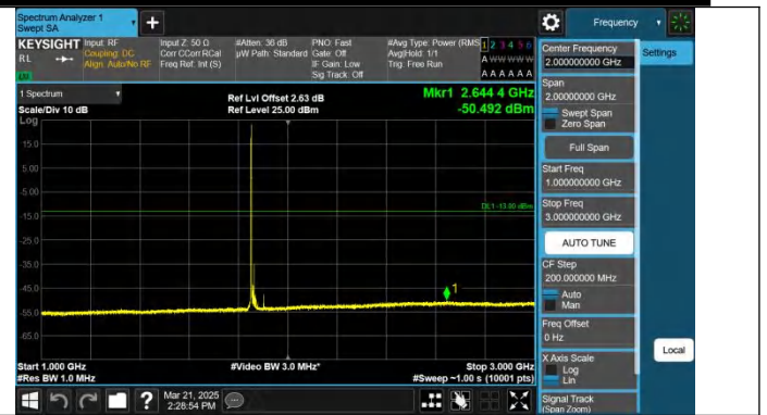
Band25-20MHz-QPSK-26140-1RB#0-1000~3000-PASS
