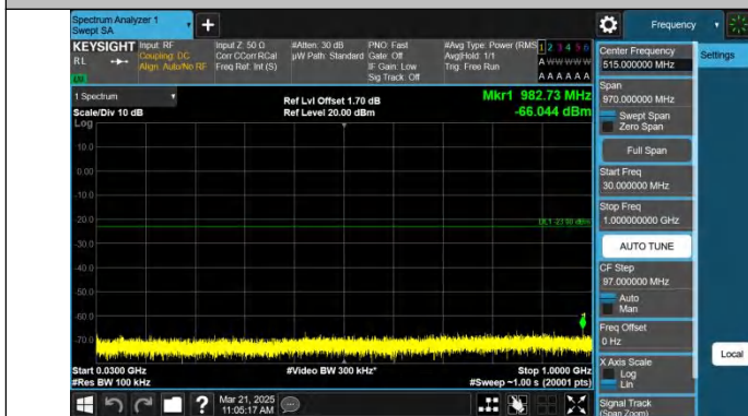
Band25-3MHz-QPSK-26365-1RB#0-30~1000-PASS
