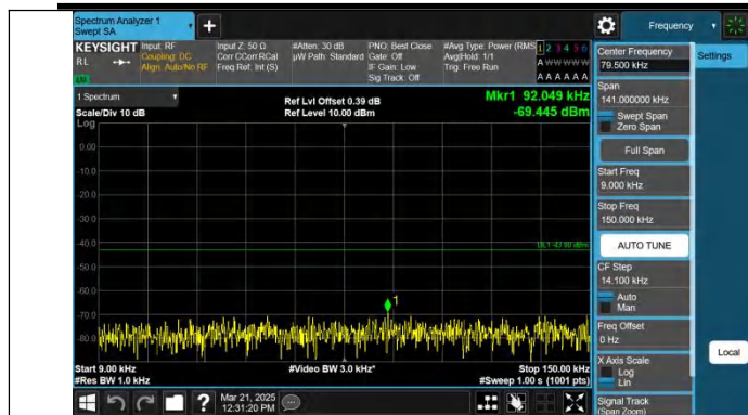
Band25-5MHz-QPSK-26665-1RB#0-0.009~0.15-PASS
