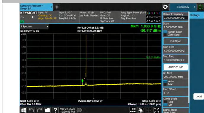
Band25-5MHz-QPSK-26365-1RB#24-1000~3000-PASS
