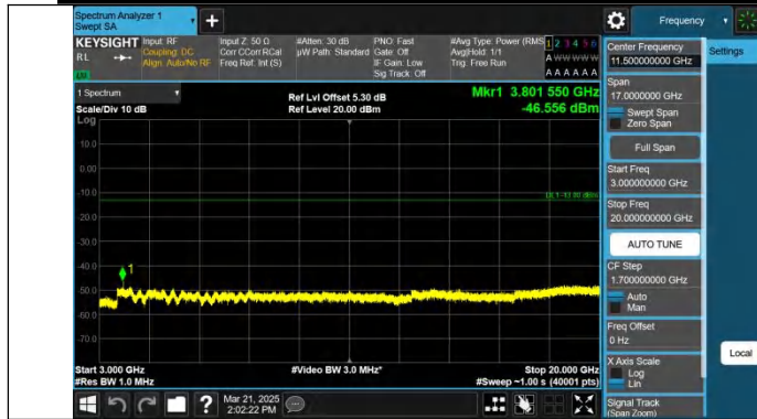
Band25-15MHz-QPSK-26615-1RB#0-3000~20000-PASS
