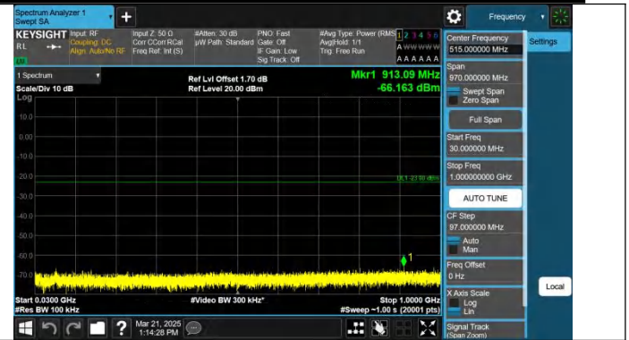
Band25-10MHz-QPSK-26090-1RB#49-30~1000-PASS
