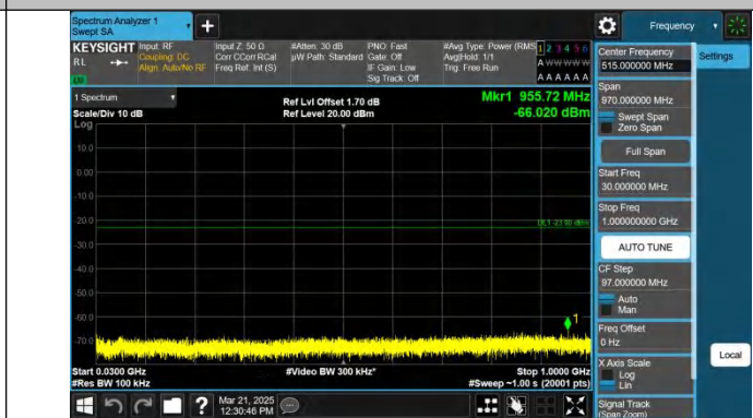
Band25-5MHz-QPSK-26365-1RB#24-30~1000-PASS
