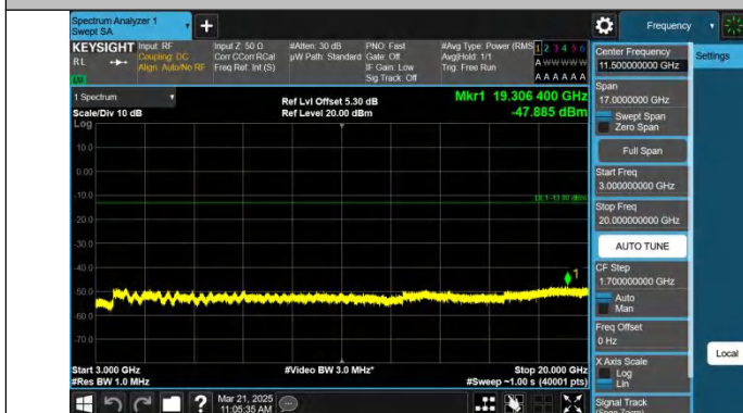
Band25-3MHz-QPSK-26365-1RB#0-3000~20000-PASS
