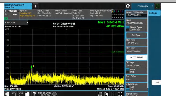
Band25-10MHz-QPSK-26640-1RB#0-0.15~30-PASS
