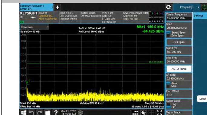
Band25-3MHz-QPSK-26365-1RB#14-0.15~30-PASS
