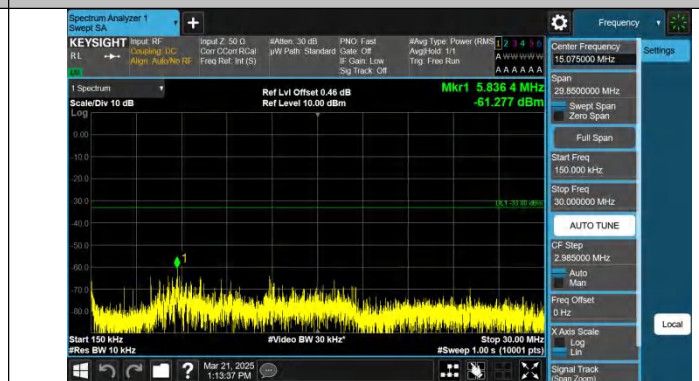
Band25-10MHz-QPSK-26090-1RB#0-0.15~30-PASS
