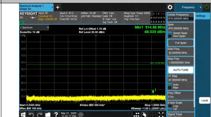
Band25-5MHz-QPSK-26665-1RB#24-30~1000-PASS
