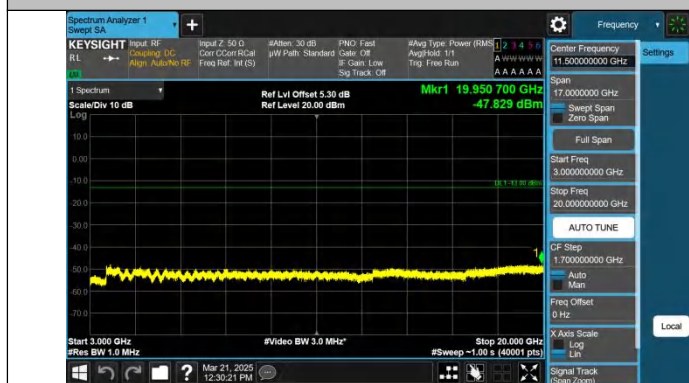
Band25-5MHz-QPSK-26365-1RB#0-3000~20000-PASS
