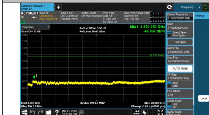
Band25-5MHz-QPSK-26665-1RB#0-3000~20000-PASS
