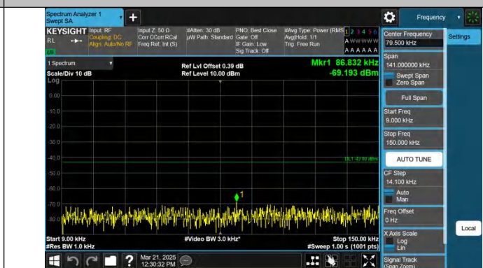
Band25-5MHz-QPSK-26365-1RB#24-0.009~0.15-PASS
