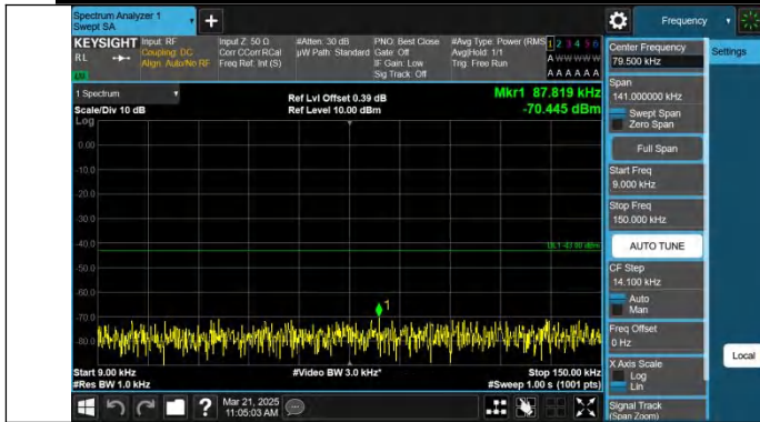
Band25-3MHz-QPSK-26365-1RB#0-0.009~0.15-PASS
