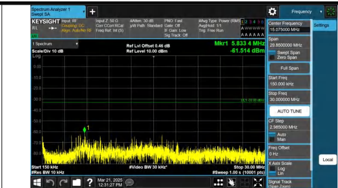
Band25-5MHz-QPSK-26665-1RB#0-0.15~30-PASS
