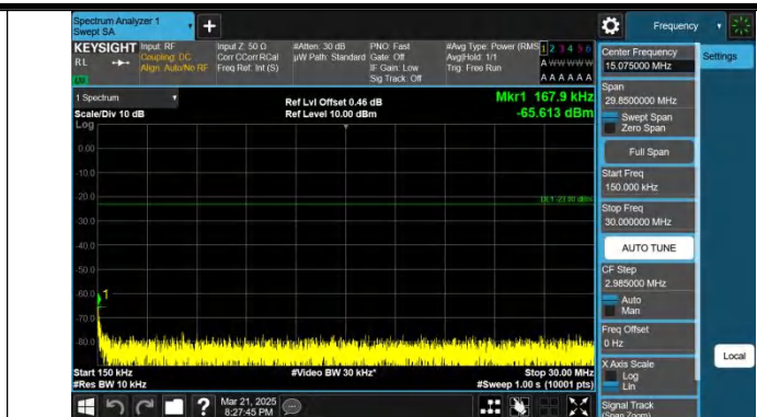
Band12-5MHz-QPSK-23155-1RB#0-0.15~30-PASS
