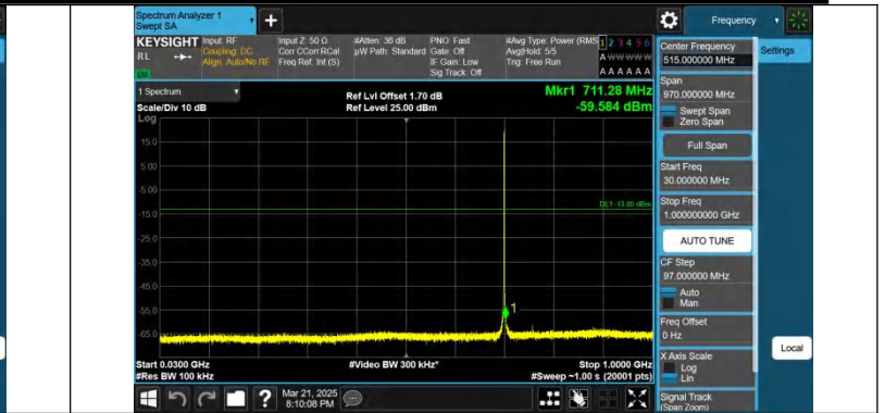
Band12-1.4MHz-QPSK-23095-1RB#5-30~1000-PASS
