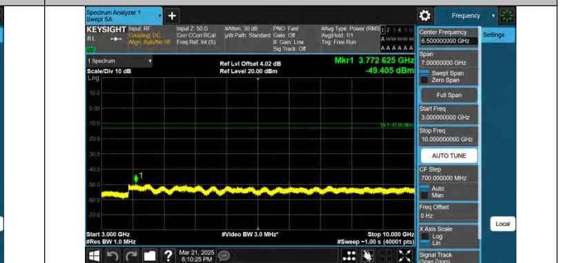
Band12-1.4MHz-QPSK-23095-1RB#5-3000~10000-PASS
