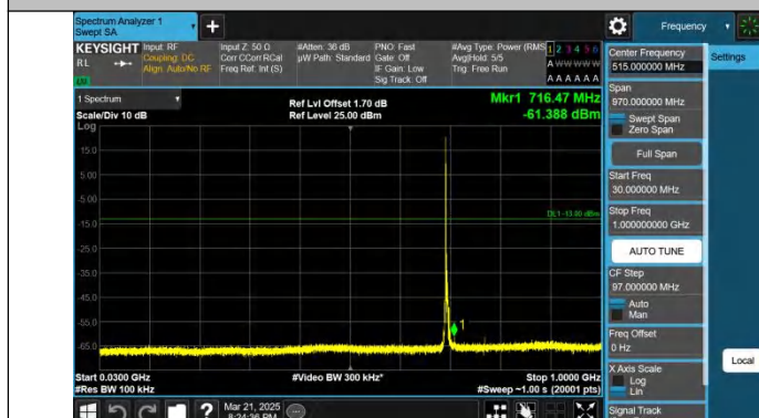
Band12-5MHz-QPSK-23035-1RB#0-30~1000-PASS
