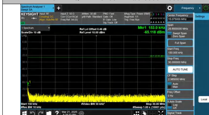
Band12-5MHz-QPSK-23155-1RB#24-0.15~30-PASS
