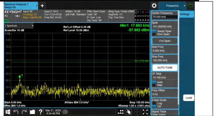
Band12-10MHz-QPSK-23095-1RB#49-0.009~0.15-PASS
