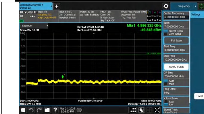
Band12-5MHz-QPSK-23035-1RB#0-3000~10000-PASS
