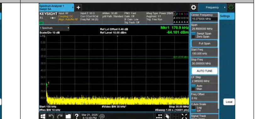
Band12-1.4MHz-QPSK-23173-1RB#0-0.15~30-PASS
