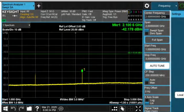
Band12-1.4MHz-QPSK-23017-1RB#5-1000~3000-PASS
