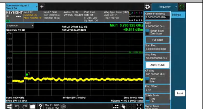
Band12-5MHz-QPSK-23035-1RB#24-3000~10000-PASS
