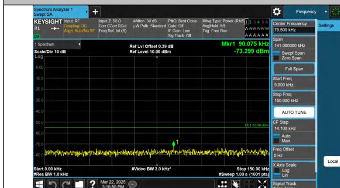
Band7-15MHz-QPSK-21100-1RB#0-0.009~0.15-PASS
