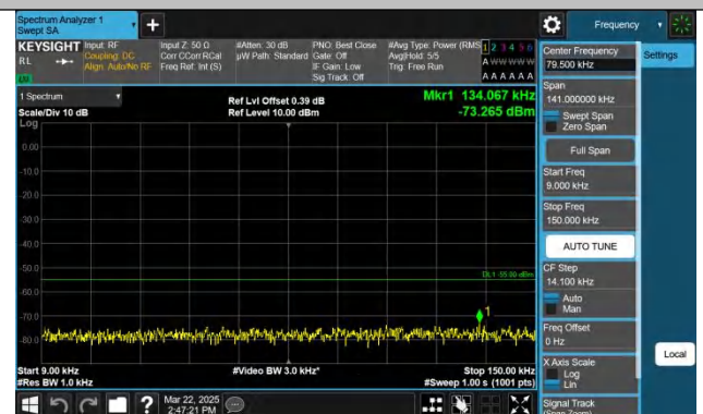
Band7-5MHz-QPSK-21100-1RB#24-0.009~0.15-PASS
