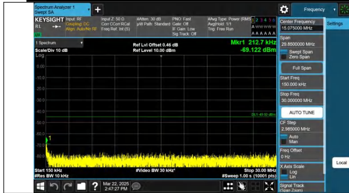
Band7-5MHz-QPSK-21100-1RB#24-0.15~30-PASS
