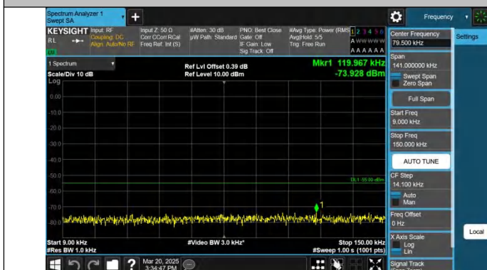
Band7-20MHz-QPSK-21350-1RB#0-0.009-0.15-PASS
