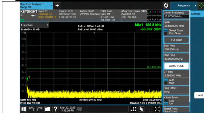
Band7-20MHz-QPSK-20850-1RB#99-0.15~30-PASS
