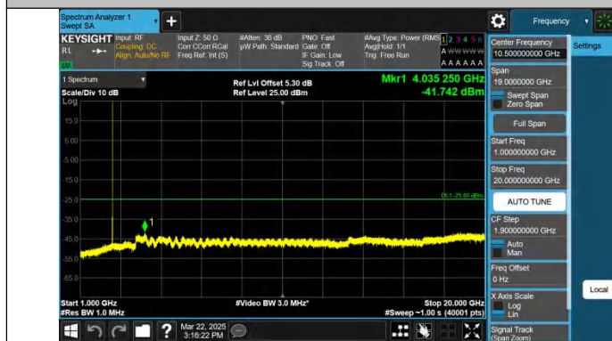
Band7-15MHz-QPSK-20825-1RB#74-1000~20000-PASS
