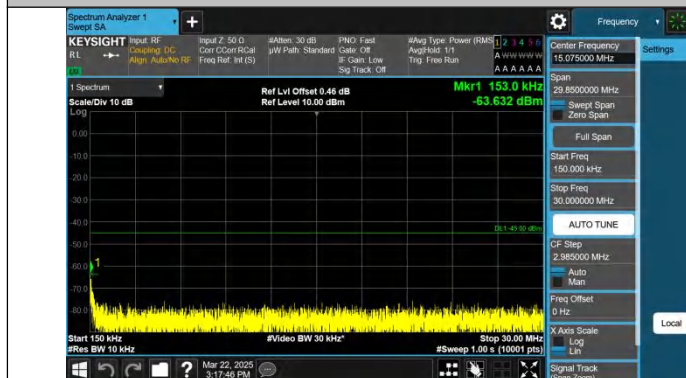
Band7-15MHz-QPSK-21100-1RB#74-0.15~30-PASS
