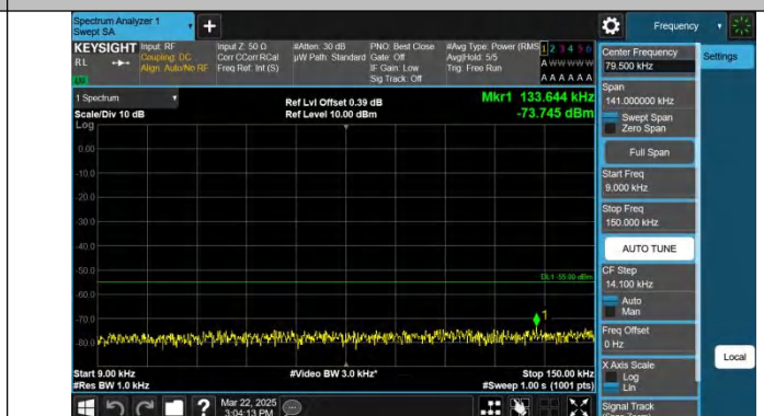
Band7-10MHz-QPSK-21400-1RB#49-0.009~0.15-PASS
