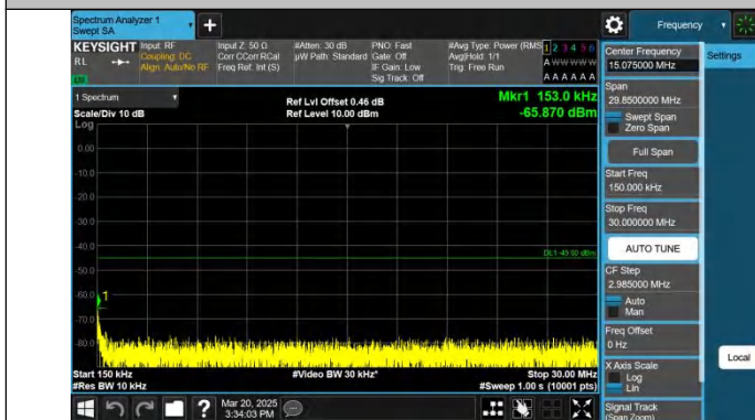
Band7-20MHz-QPSK-21100-1RB#99-0.15-30-PASS
