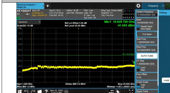
Band7-15MHz-QPSK-21100-1RB#74-1000~20000-PASS
