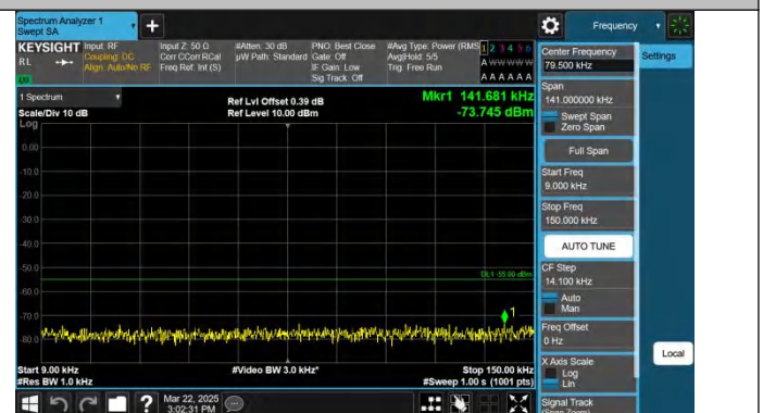
Band7-10MHz-QPSK-21100-1RB#49-0.009~0.15-PASS
