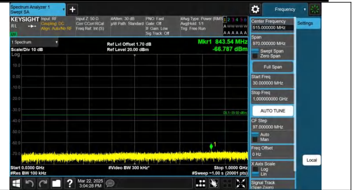
Band7-10MHz-QPSK-21400-1RB#49-30~1000-PASS
