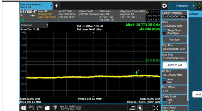
Band7-15MHz-QPSK-21100-1RB#0-20000~27000-PASS
