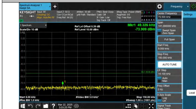
Band7-10MHz-QPSK-21400-1RB#0-0.009~0.15-PASS
