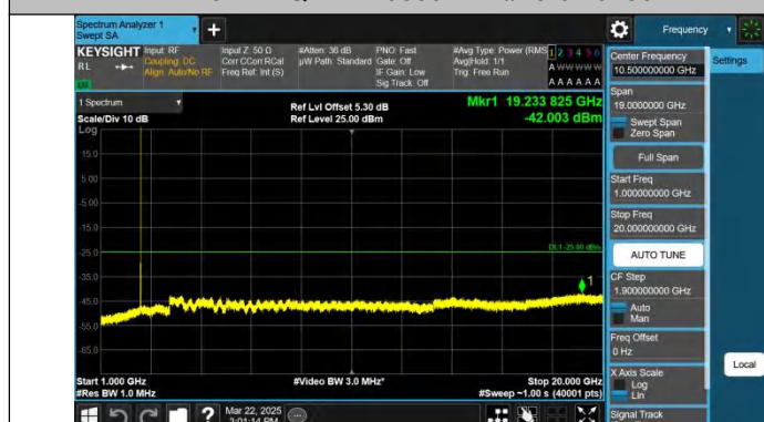
Band7-10MHz-QPSK-20800-1RB#49-1000~20000-PASS
