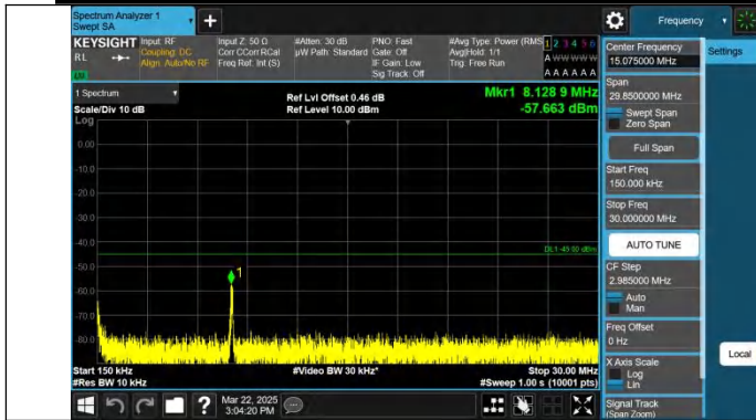
Band7-10MHz-QPSK-21400-1RB#49-0.15~30-PASS
