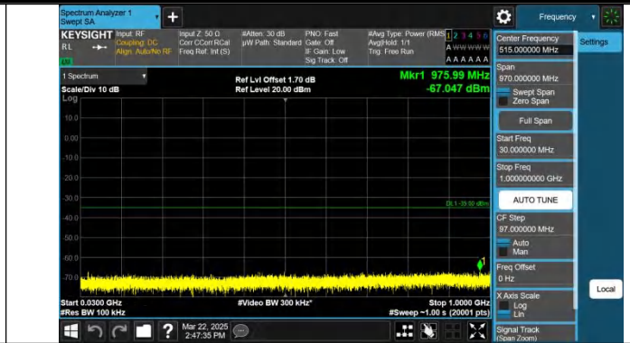
Band7-5MHz-QPSK-21100-1RB#24-30~1000-PASS
