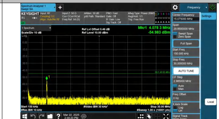
Band7-5MHz-QPSK-21425-1RB#0-0.15~30-PASS
