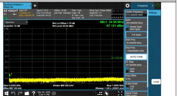
Band7-20MHz-QPSK-21100-1RB#99-30-1000-PASS
