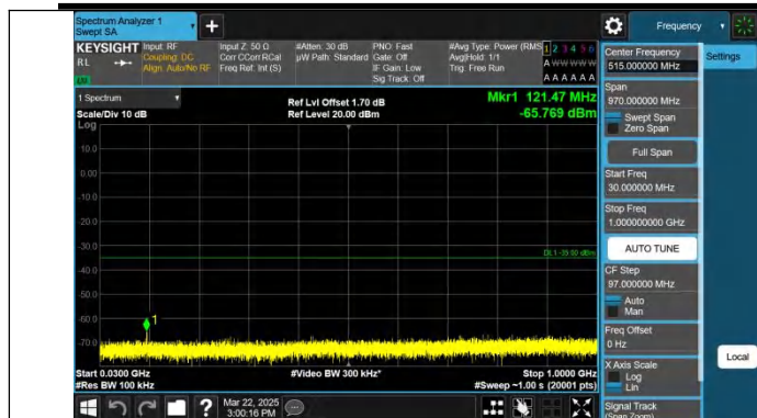
Band7-10MHz-QPSK-20800-1RB#0-30~1000-PASS
