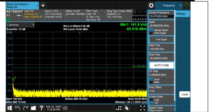
Band7-15MHz-QPSK-21375-1RB#0-0.15~30-PASS
