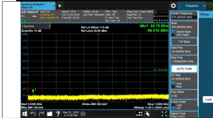
Band7-15MHz-QPSK-21100-1RB#0-30~1000-PASS
