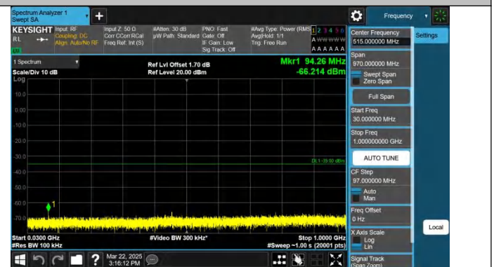
Band7-15MHz-QPSK-20825-1RB#74-30~1000-PASS
