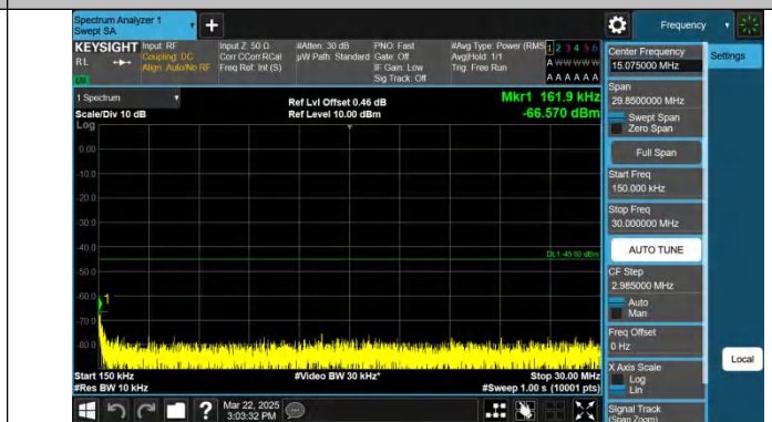
Band7-10MHz-QPSK-21400-1RB#0-0.15~30-PASS
