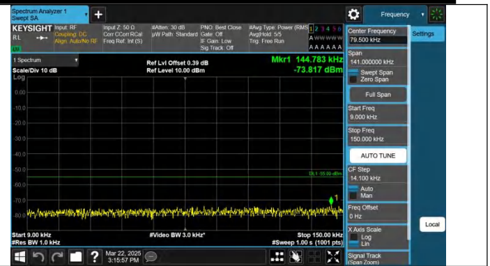
Band7-15MHz-QPSK-20825-1RB#74-0.009~0.15-PASS
