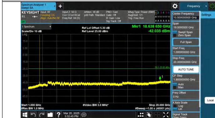
Band7-20MHz-QPSK-20850-1RB#99-1000~20000-PASS
