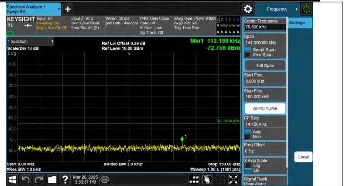
Band7-20MHz-QPSK-21100-1RB#99-0.009-0.15-PASS
