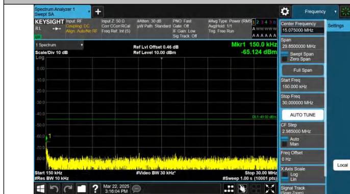
Band7-15MHz-QPSK-20825-1RB#74-0.15~30-PASS
