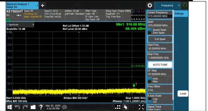
Band7-20MHz-QPSK-20850-1RB#99-30~1000-PASS
