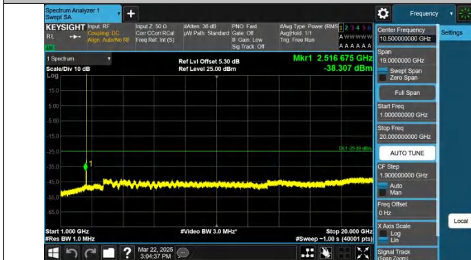
Band7-10MHz-QPSK-21400-1RB#49-1000~20000-PASS
