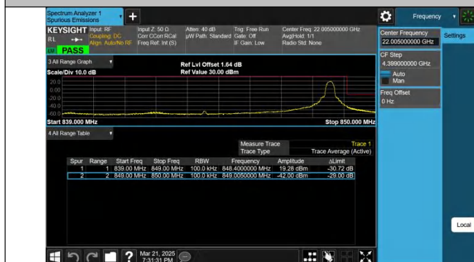
Band5-10MHz-QPSK-20600-1RB#49-PASS
