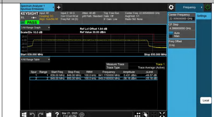
Band5-10MHz-QPSK-20600-50RB#0-PASS
