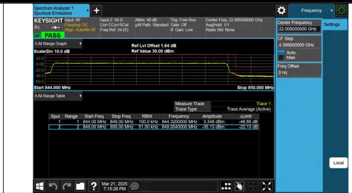
Band5-5MHz-QPSK-20625-25RB#0-PASS
