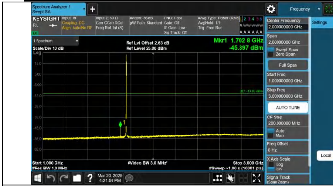
Band4-5MHz-QPSK-20375-1RB#24-1000~3000-PASS
