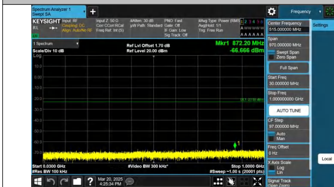
Band4-10MHz-QPSK-20000-1RB#0-30~1000-PASS
