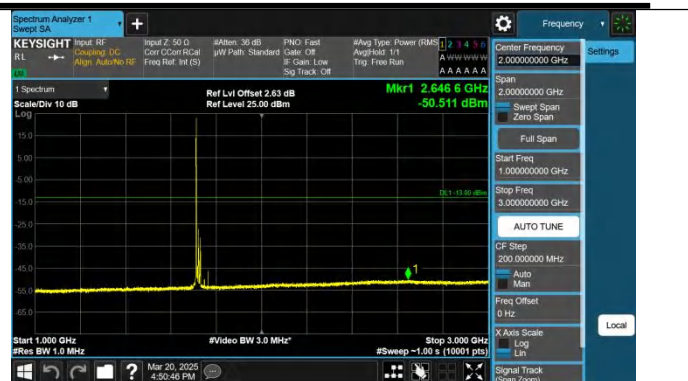
Band4-20MHz-QPSK-20050-1RB#0-1000~3000-PASS
