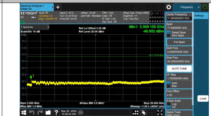
Band4-1.4MHz-QPSK-20393-1RB#5-3000~20000-PASS
