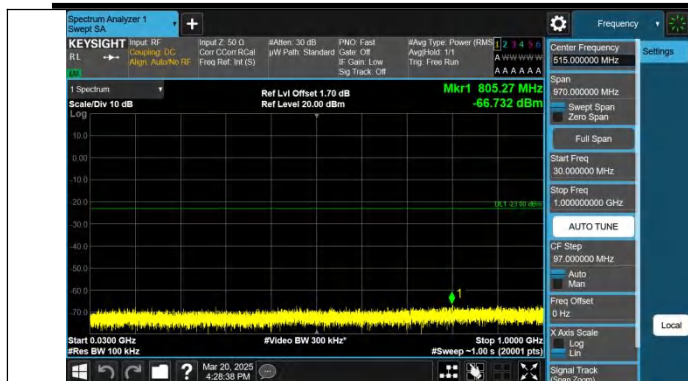
Band4-10MHz-QPSK-20350-1RB#0-30~1000-PASS
