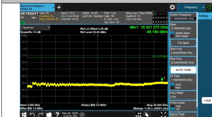
Band4-10MHz-QPSK-20000-1RB#0-3000~20000-PASS
