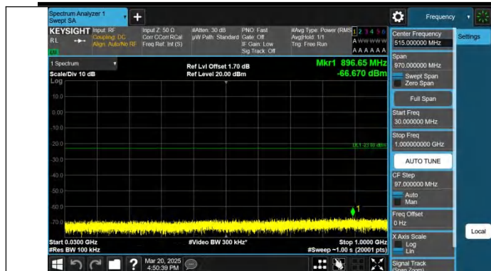
Band4-20MHz-QPSK-20050-1RB#0-30~1000-PASS
