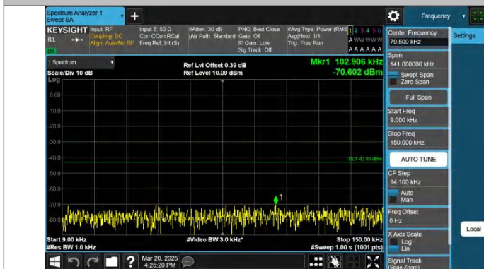
Band4-10MHz-QPSK-20000-1RB#0-0.009~0.15-PASS
