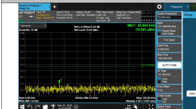
Band4-5MHz-QPSK-20175-1RB#0-0.009~0.15-PASS
