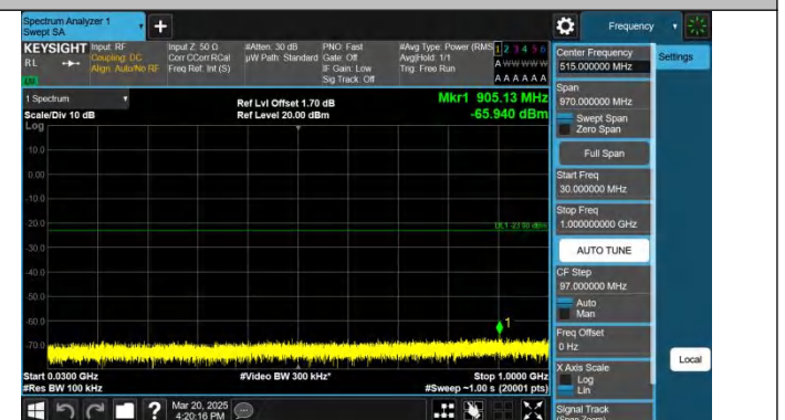
Band4-5MHz-QPSK-20175-1RB#24-30~1000-PASS
