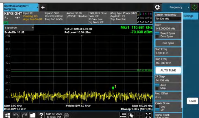
Band2-15MHz-QPSK-18675-1RB#74-0.009~0.15-PASS
