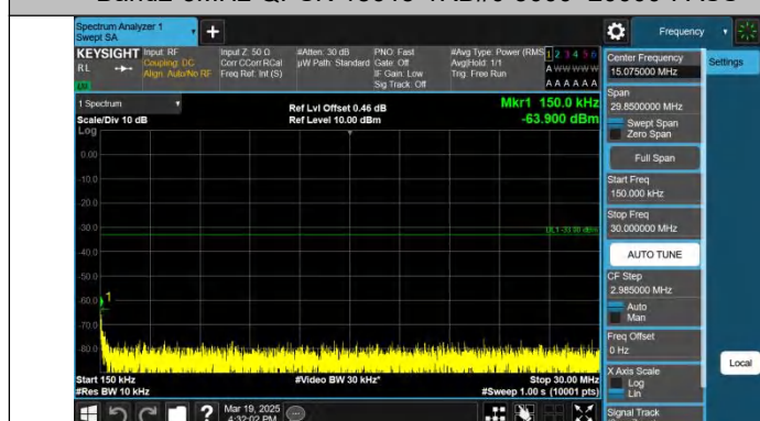
Band2-3MHz-QPSK-18615-1RB#14-0.15~30-PASS
