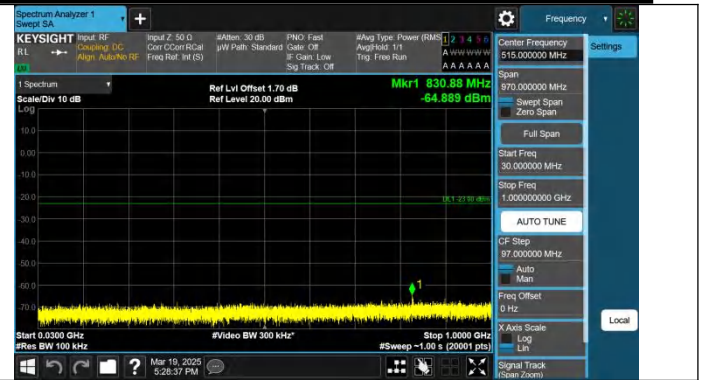
Band2-10MHz-QPSK-18650-1RB#49-30~1000-PASS
