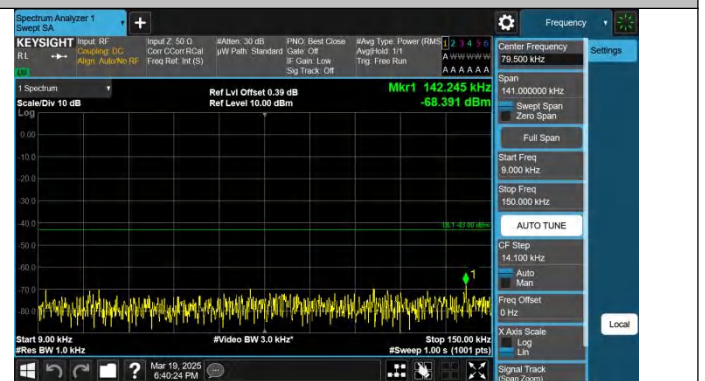
Band2-20MHz-QPSK-18700-1RB#99-0.009~0.15-PASS
