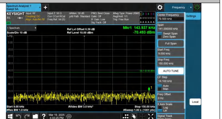
Band2-3MHz-QPSK-18900-1RB#14-0.009~0.15-PASS
