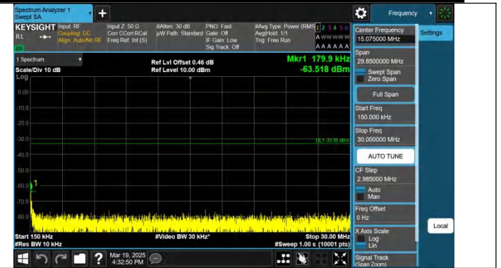
Band2-3MHz-QPSK-18900-1RB#0-0.15~30-PASS
