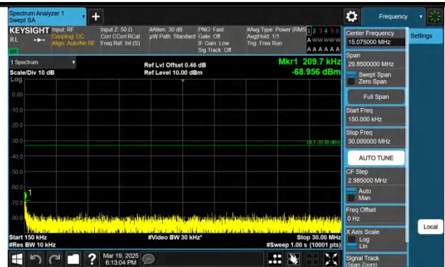
Band2-15MHz-QPSK-18675-1RB#0-0.15~30-PASS
