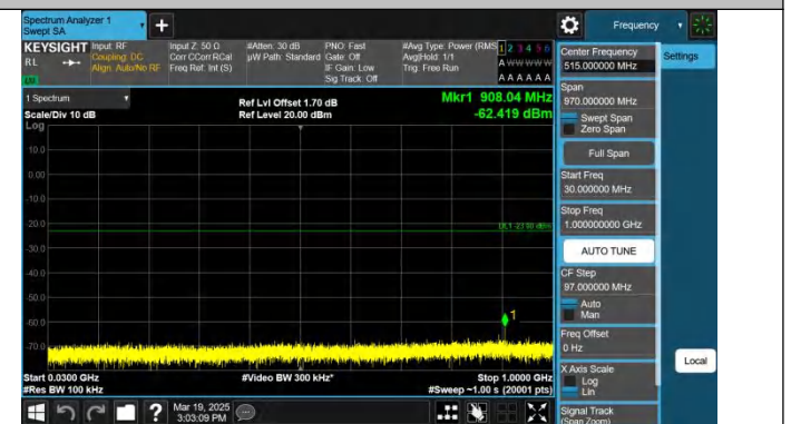
Band2-5MHz-QPSK-18625-1RB#24-30~1000-PASS
