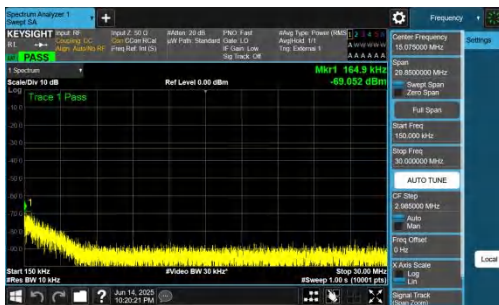
NTNV-DC_2A-n78A(3700-3800)-PC2-30-5+80-M+M-QPSK-IDLE-DFT-QPSK-Inner_1RB_Right-0.15-30-PASS
