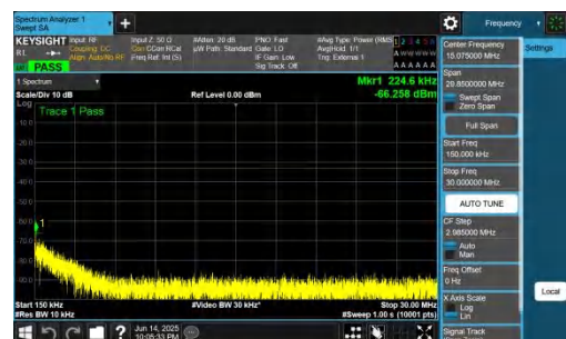
NTNV-DC_2A-n78A(3700-3800)-PC2-30-5+80-M+L-QPSK-IDLE-D FT-QPSK-Inner_1RB_Left-0.15-30-PASS
