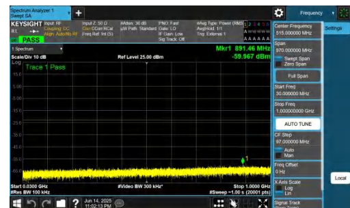
NTNV-DC_2A-n78A(3700-3800)-PC2-30-5+90-M+H-QPSK-IDLE-D FT-BPSK-Inner_1RB_Right-30-1000-PASS
