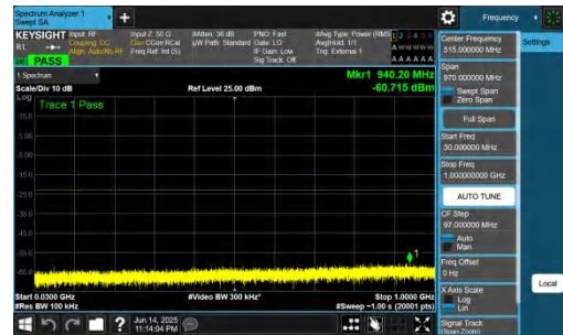
NTNV-DC_2A-n78A(3700-3800)-PC2-30-5+100-M+L-QPSK-IDLE-DFT-BPSK-Inner_1RB_Right-30-1000-PASS
