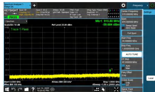
NTNV-DC_2A-n78A(3700-3800)-PC2-30-5+80-M+M-QPSK-IDLE-DFT-QPSK-Inner_1RB_Right-30-1000-PASS
