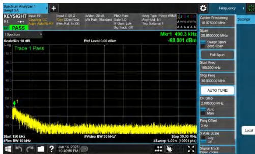
NTNV-DC_2A-n78A(3700-3800)-PC2-30-5+90-M+M-QPSK-IDLE-DFT-BPSK-Inner_1RB_Right-0.15-30-PASS
