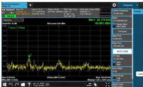
NTNV-DC_2A-n78A(3700-3800)-PC2-30-5+90-M+H-QPSK-IDLE-D FT-QPSK-Inner_1RB_Left-0.009-0.15-PASS
