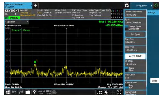
NTNV-DC_2A-n78A(3700-3800)-PC2-30-5+90-M+H-QPSK-IDLE-D FT-BPSK-Inner_1RB_Right-0.009-0.15-PASS
