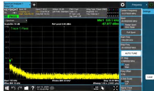
NTNV-DC_2A-n78A(3700-3800)-PC2-30-5+100-M+L-QPSK-IDLE-DFT-BPSK-Inner_1RB_Left-0.15-30-PASS
