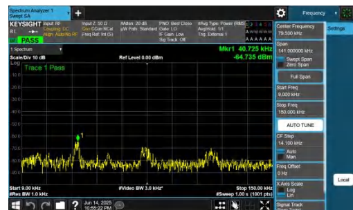
NTNV-DC_2A-n78A(3700-3800)-PC2-30-5+90-M+M-QPSK-IDLE-DFT-QPSK-Inner_1RB_Right-0.009-0.15-PASS
