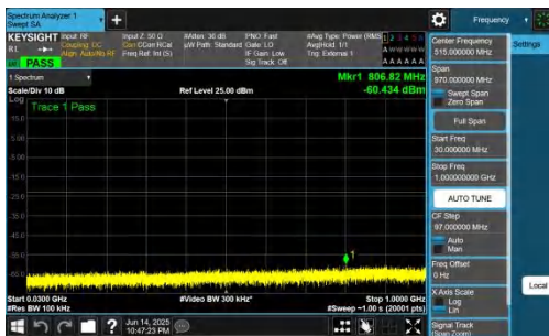
NTNV-DC_2A-n78A(3700-3800)-PC2-30-5+90-M+M-QPSK-IDLE-DFT-BPSK-Inner_1RB_Left-30-1000-PASS
