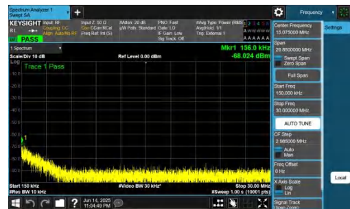
NTNV-DC_2A-n78A(3700-3800)-PC2-30-5+90-M+H-QPSK-IDLE-D FT-QPSK-Inner_1RB_Left-0.15-30-PASS
