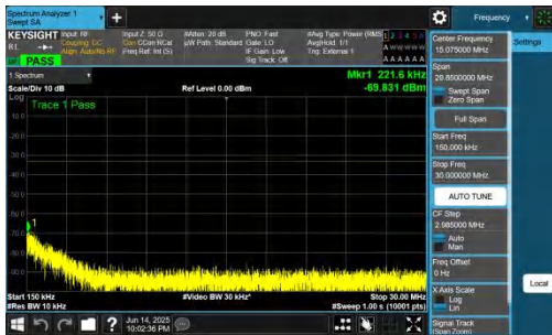
NTNV-DC_2A-n78A(3700-3800)-PC2-30-5+80-M+L-QPSK-IDLE-D FT-BPSK-Inner_1RB_Right-0.15-30-PASS
