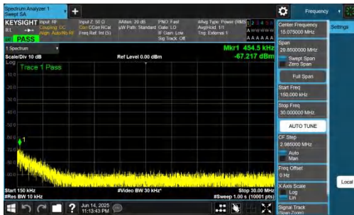
NTNV-DC_2A-n78A(3700-3800)-PC2-30-5+100-M+L-QPSK-IDLE-DFT-BPSK-Inner_1RB_Right-0.15-30-PASS
