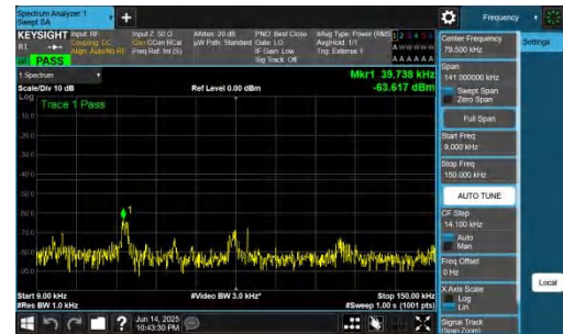
NTNV-DC_2A-n78A(3700-3800)-PC2-30-5+90-M+L-QPSK-IDLE-D FT-QPSK-Inner_1RB_Right-0.009-0.15-PASS
