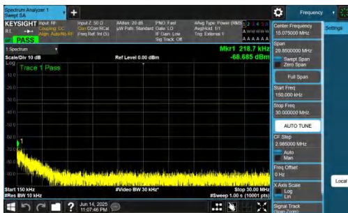
NTNV-DC_2A-n78A(3700-3800)-PC2-30-5+90-M+H-QPSK-IDLE-D FT-QPSK-Inner_1RB_Right-0.15-30-PASS
