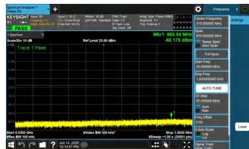
NTNV-DC_2A-n78A(3700-3800)-PC2-30-5+80-M+M-QPSK-IDLE-DFT-BPSK-Inner_1RB_Right-30-1000-PASS
