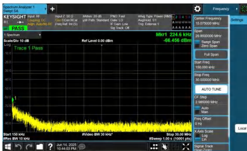
NTNV-DC_2A-n78A(3700-3800)-PC2-30-5+90-M+L-QPSK-IDLE-D FT-QPSK-Inner_1RB_Right-0.15-30-PASS
