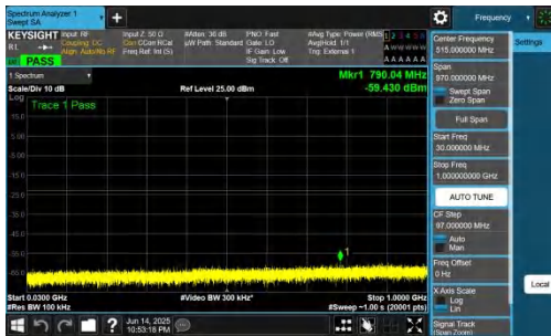
NTNV-DC_2A-n78A(3700-3800)-PC2-30-5+90-M+M-QPSK-IDLE-DFT-QPSK-Inner_1RB_Left-30-1000-PASS
