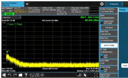
NTNV-DC_2A-n78A(3700-3800)-PC2-30-5+80-M+H-QPSK-IDLE-D FT-BPSK-Inner_1RB_Right-0.15-30-PASS
