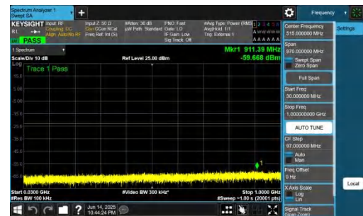
NTNV-DC_2A-n78A(3700-3800)-PC2-30-5+90-M+L-QPSK-IDLE-D FT-QPSK-Inner_1RB_Right-30-1000-PASS
