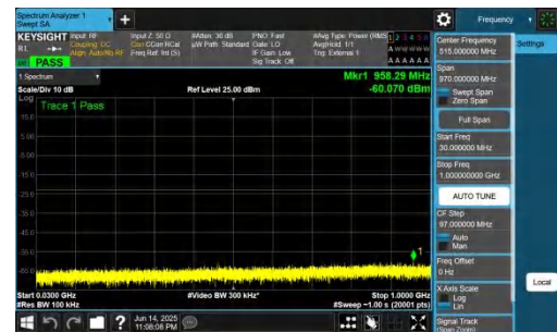
NTNV-DC_2A-n78A(3700-3800)-PC2-30-5+90-M+H-QPSK-IDLE-D FT-QPSK-Inner_1RB_Right-30-1000-PASS
