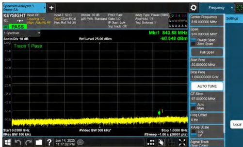
NTNV-DC_2A-n78A(3700-3800)-PC2-30-5+100-M+L-QPSK-IDLE-DFT-QPSK-Inner_1RB_Left-30-1000-PASS
