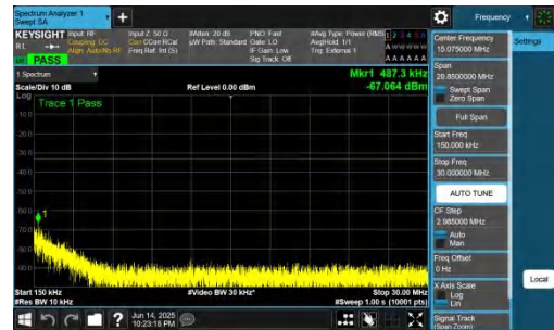
NTNV-DC_2A-n78A(3700-3800)-PC2-30-5+80-M+H-QPSK-IDLE-D FT-BPSK-Inner_1RB_Left-0.15-30-PASS
