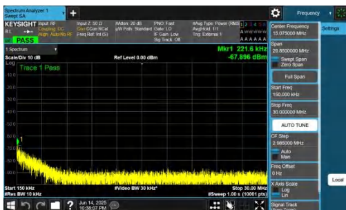
NTNV-DC_2A-n78A(3700-3800)-PC2-30-5+90-M+L-QPSK-IDLE-D FT-BPSK-Inner_1RB_Right-0.15-30-PASS
