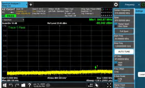
NTNV-DC_2A-n78A(3700-3800)-PC2-30-5+80-M+L-QPSK-IDLE-D FT-QPSK-Inner_1RB_Left-30-1000-PASS
