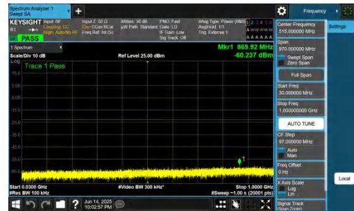
NTNV-DC_2A-n78A(3700-3800)-PC2-30-5+80-M+L-QPSK-IDLE-D FT-BPSK-Inner_1RB_Right-30-1000-PASS
