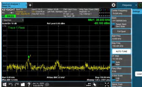
NTNV-DC_2A-n78A(3700-3800)-PC2-30-5+70-M+H-QPSK-IDLE-D FT-QPSK-Inner_1RB_Left-0.009-0.15-PASS
