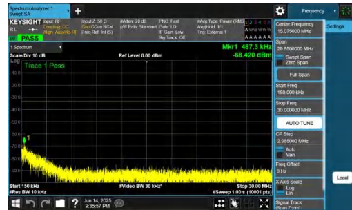
NTNV-DC_2A-n78A(3700-3800)-PC2-30-5+70-M+M-QPSK-IDLE-DFT-BPSK-Inner_1RB_Left-0.15-30-PASS
