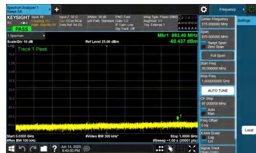
NTNV-DC_2A-n78A(3700-3800)-PC2-30-5+50-M+H-QPSK-IDLE-D FT-BPSK-Inner_1RB_Right-30-1000-PASS
