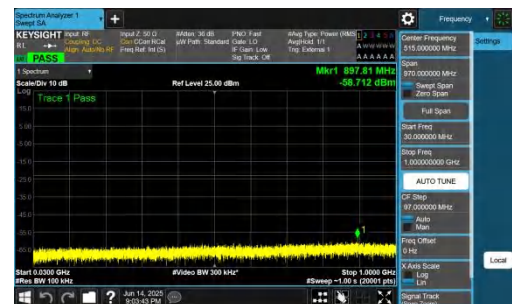
NTNV-DC_2A-n78A(3700-3800)-PC2-30-5+60-M+M-QPSK-IDLE-DFT-BPSK-Inner_1RB_Right-30-1000-PASS
