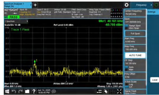
NTNV-DC_2A-n78A(3700-3800)-PC2-30-5+60-M+M-QPSK-IDLE-DFT-QPSK-Inner_1RB_Right-0.009-0.15-PASS
