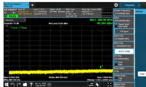
NTNV-DC_2A-n78A(3700-3800)-PC2-30-5+60-M+M-QPSK-IDLE-DFT-QPSK-Inner_1RB_Right-30-1000-PASS
