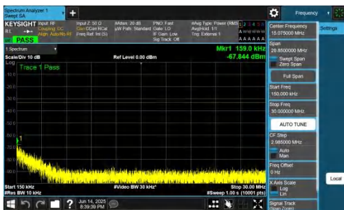
NTNV-DC_2A-n78A(3700-3800)-PC2-30-5+50-M+H-QPSK-IDLE-D FT-BPSK-Inner_1RB_Right-0.15-30-PASS
