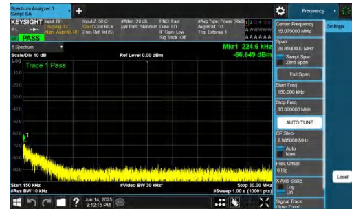
NTNV-DC_2A-n78A(3700-3800)-PC2-30-5+60-M+H-QPSK-IDLE-D FT-BPSK-Inner_1RB_Left-0.15-PASS
