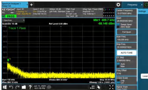
NTNV-DC_2A-n78A(3700-3800)-PC2-30-5+60-M+L-QPSK-IDLE-D FT-BPSK-Inner_1RB_Right-0.15-30-PASS
