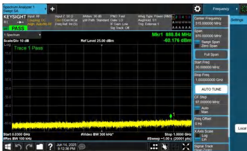
NTNV-DC_2A-n78A(3700-3800)-PC2-30-5+60-M+H-QPSK-IDLE-D FT-BPSK-Inner_1RB_Left-30-1000-PASS
