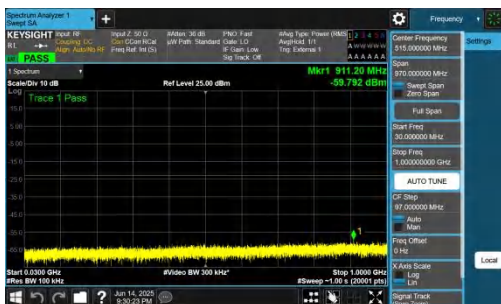
NTNV-DC_2A-n78A(3700-3800)-PC2-30-5+70-M+L-QPSK-IDLE-D FT-QPSK-Inner_1RB_Left-30-1000-PASS
