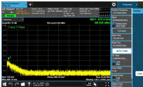
NTNV-DC_2A-n78A(3700-3800)-PC2-30-5+70-M+M-QPSK-IDLE-DFT-BPSK-Inner_1RB_Right-0.15-30-PASS
