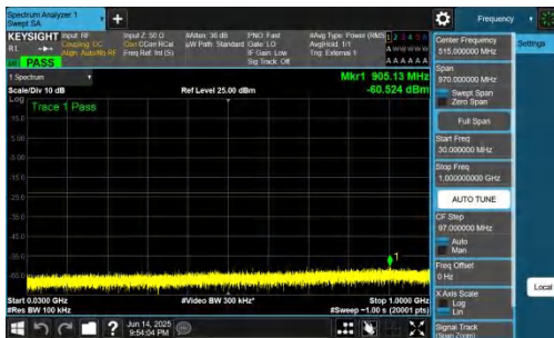
NTNV-DC_2A-n78A(3700-3800)-PC2-30-5+70-M+H-QPSK-IDLE-D FT-QPSK-Inner_1RB_Left-30-1000-PASS
