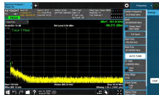
NTNV-DC_2A-n78A(3700-3800)-PC2-30-5+50-M+H-QPSK-IDLE-D FT-QPSK-Inner_1RB_Left-0.15-30-PASS
