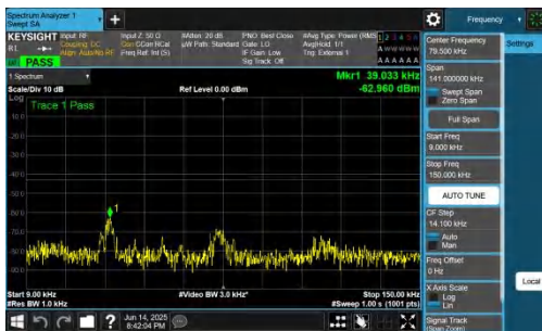
NTNV-DC_2A-n78A(3700-3800)-PC2-30-5+50-M+H-QPSK-IDLE-D FT-QPSK-Inner_1RB_Left-0.009-0.15-PASS
