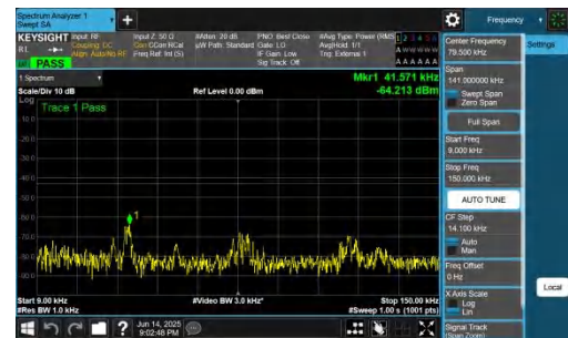
NTNV-DC_2A-n78A(3700-3800)-PC2-30-5+60-M+M-QPSK-IDLE-DFT-BPSK-Inner_1RB_Right-0.009-0.15-PASS
