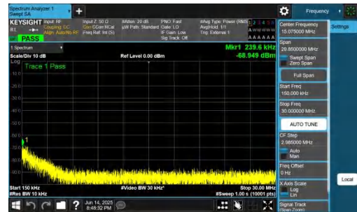
NTNV-DC_2A-n78A(3700-3800)-PC2-30-5+60-M+L-QPSK-IDLE-D FT-BPSK-Inner_1RB_Left-0.15-30-PASS
