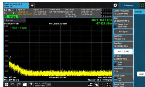
NTNV-DC_2A-n78A(3700-3800)-PC2-30-5+70-M+H-QPSK-IDLE-DFT-BPSK-Inner_1RB_Left-0.15-30-PASS
