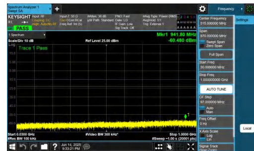
NTNV-DC_2A-n78A(3700-3800)-PC2-30-5+70-M+L-QPSK-IDLE-D FT-QPSK-Inner_1RB_Right-30-1000-PASS
