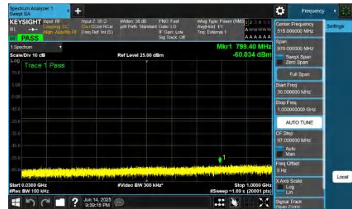
NTNV-DC_2A-n78A(3700-3800)-PC2-30-5+70-M+M-QPSK-IDLE-DFT-BPSK-Inner_1RB_Right-30-1000-PASS
