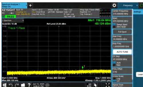
NTNV-DC_2A-n78A(3700-3800)-PC2-30-5+60-M+M-QPSK-IDLE-DFT-QPSK-Inner_1RB_Left-30-1000-PASS
