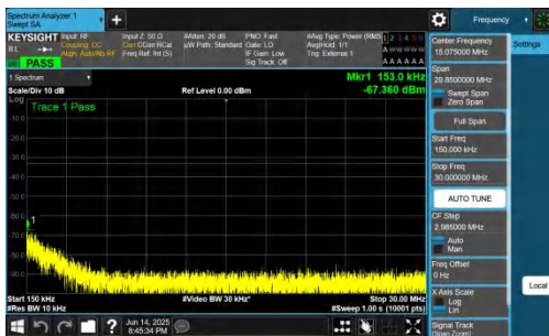
NTNV-DC_2A-n78A(3700-3800)-PC2-30-5+50-M+H-QPSK-IDLE-D FT-QPSK-Inner_1RB_Right-0.15-30-PASS
