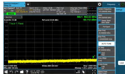
NTNV-DC_2A-n78A(3700-3800)-PC2-30-5+50-M+H-QPSK-IDLE-D FT-QPSK-Inner_1RB_Right-30-1000-PASS
