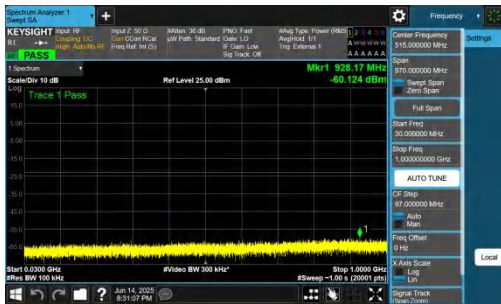
NTNV-DC_2A-n78A(3700-3800)-PC2-30-5+50-M+M-QPSK-IDLE-DFT-QPSK-Inner_1RB_Left-30-1000-PASS
