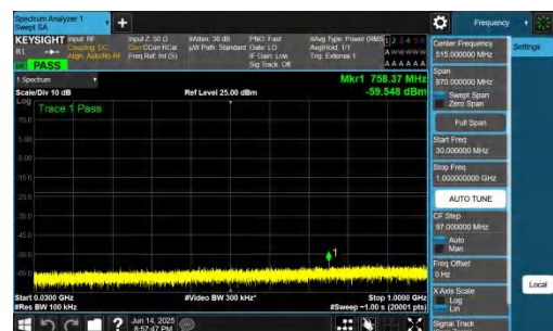
NTNV-DC_2A-n78A(3700-3800)-PC2-30-5+60-M+L-QPSK-IDLE-D FT-QPSK-Inner_1RB_Right-30-1000-PASS
