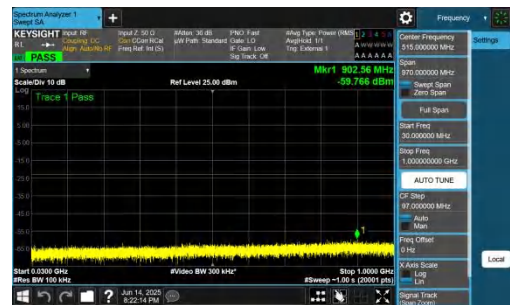
NTNV-DC_2A-n78A(3700-3800)-PC2-30-5+50-M+L-QPSK-IDLE-D FT-QPSK-Inner_1RB_Right-30-1000-PASS
