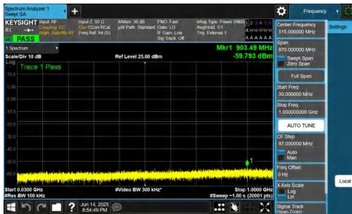
NTNV-DC_2A-n78A(3700-3800)-PC2-30-5+60-M+L-QPSK-IDLE-D FT-QPSK-Inner_1RB_Left-30-1000-PASS
