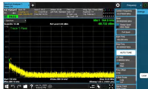
NTNV-DC_2A-n78A(3700-3800)-PC2-30-5+70-M+H-QPSK-IDLE-D FT-QPSK-Inner_1RB_Left-0.15-30-PASS
