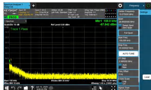
NTNV-DC_2A-n78A(3700-3800)-PC2-30-5+60-M+M-QPSK-IDLE-D FT-BPSK-Inner_1RB_Left-0.15-30-PASS
