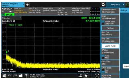
NTNV-DC_2A-n78A(3700-3800)-PC2-30-5+70-M+L-QPSK-IDLE-D FT-QPSK-Inner_1RB_Right-0.15-30-PASS
