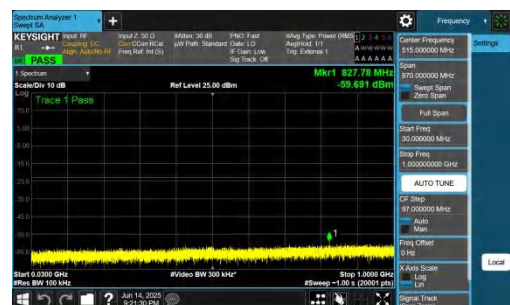
NTNV-DC_2A-n78A(3700-3800)-PC2-30-5+60-M+H-QPSK-IDLE-D FT-QPSK-Inner_1RB_Right-30-1000-PASS
