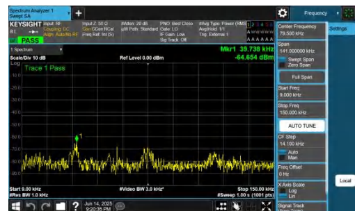
NTNV-DC_2A-n78A(3700-3800)-PC2-30-5+60-M+H-QPSK-IDLE-D FT-QPSK-Inner_1RB_Right-0.009-0.15-PASS
