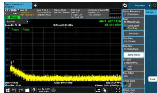
NTNV-DC_2A-n78A(3700-3800)-PC2-30-5+60-M+M-QPSK-IDLE-DFT-QPSK-Inner_1RB_Left-0.15-30-PASS
