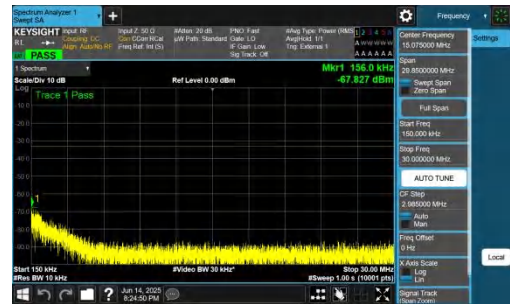
NTNV-DC_2A-n78A(3700-3800)-PC2-30-5+50-M+M-QPSK-IDLE-DFT-BPSK-Inner_1RB_Left-0.15-30-PASS
