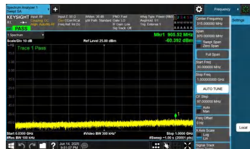
NTNV-DC_2A-n78A(3700-3800)-PC2-30-5+70-M+H-QPSK-IDLE-D FT-BPSK-Inner_1RB_Right-30-1000-PASS
