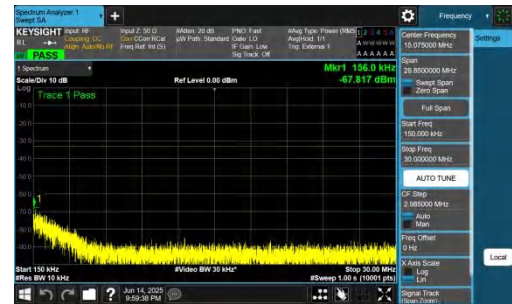
NTNV-DC_2A-n78A(3700-3800)-PC2-30-5+80-M+L-QPSK-IDLE-D FT-BPSK-Inner_1RB_Left-0.15-30-PASS
