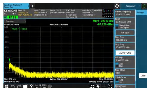
NTNV-DC_2A-n78A(3700-3800)-PC2-30-5+70-M+M-QPSK-IDLE-DFT-QPSK-Inner_1RB_Left-0.15-30-PASS
