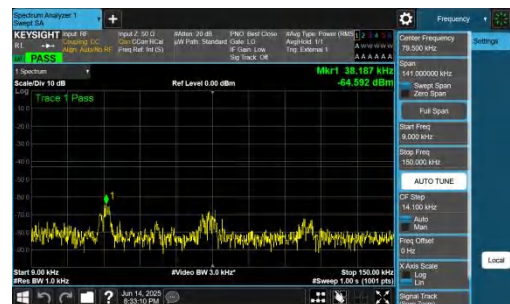
NTNV-DC_2A-n78A(3700-3800)-PC2-30-5+50-M+M-QPSK-IDLE-DFT-QPSK-Inner_1RB_Right-0.009-0.15-PASS
