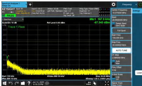
NTNV-DC_2A-n78A(3700-3800)-PC2-30-5+60-M+H-QPSK-IDLE-D FT-BPSK-Inner_1RB_Right-0.15-30-PASS
