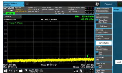
NTNV-DC_2A-n78A(3700-3800)-PC2-30-5+50-M+L-QPSK-IDLE-D FT-BPSK-Inner_1RB_Right-30-1000-PASS
