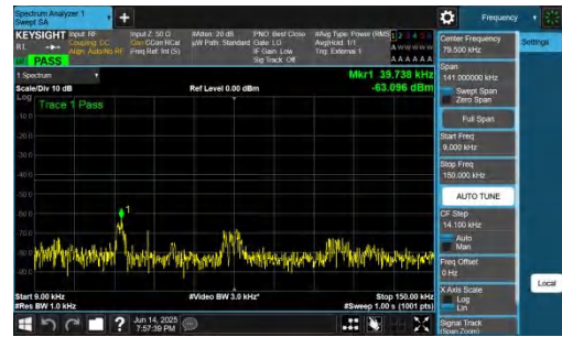
NTNV-DC_2A-n78A(3700-3800)-PC2-30-5+40-M+M-QPSK-IDLE-DFT-QPSK-Inner_1RB_Right-0.009-0.15-PASS
