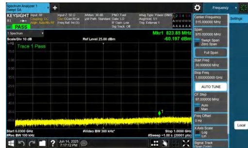
NTNV-DC_2A-n78A(3700-3800)-PC2-30-5+30-M+M-QPSK-IDLE-DFT-BPSK-Inner_1RB_Right-30-1000-PASS
