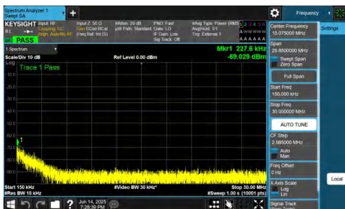
NTNV-DC_2A-n78A(3700-3800)-PC2-30-5+30-M+H-QPSK-IDLE-D FT-BPSK-Inner_1RB_Right-0.15-30-PASS
