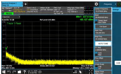
NTNV-DC_2A-n78A(3700-3800)-PC2-30-5+50-M+L-QPSK-IDLE-D FT-BPSK-Inner_1RB_Right-0.15-30-PASS
