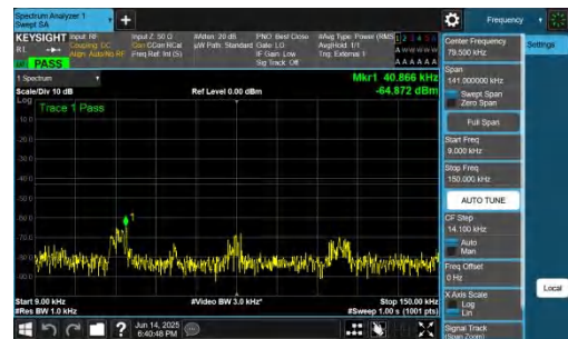
NTNV-DC_2A-n78A(3700-3800)-PC2-30-5+20-M+M-QPSK-IDLE-DFT-BPSK-Inner_1RB_Right-0.009-0.15-PASS
