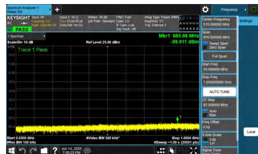
NTNV-DC_2A-n78A(3700-3800)-PC2-30-5+30-M+L-QPSK-IDLE-D FT-BPSK-Inner_1RB_Right-30-1000-PASS
