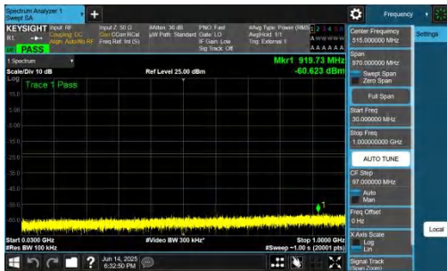
NTNV-DC_2A-n78A(3700-3800)-PC2-30-5+20-M+L-QPSK-IDLE-D FT-QPSK-Inner_1RB_Left-30-1000-PASS
