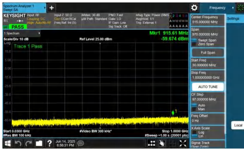
NTNV-DC_2A-n78A(3700-3800)-PC2-30-5+20-M+H-QPSK-IDLE-D FT-QPSK-Inner_1RB_Left-30-1000-PASS
