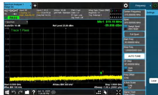
NTNV-DC_2A-n78A(3700-3800)-PC2-30-5+30-M+H-QPSK-IDLE-D FT-QPSK-Inner_1RB_Right-30-1000-PASS
