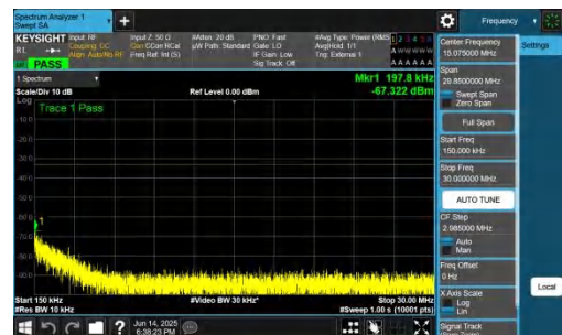
NTNV-DC_2A-n78A(3700-3800)-PC2-30-5+20-M+M-QPSK-IDLE-D FT-BPSK-Inner_1RB_Left-0.15-30-PASS
