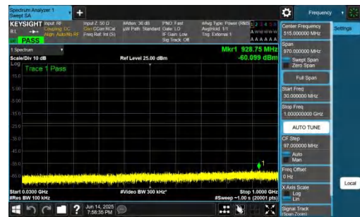
NTNV-DC_2A-n78A(3700-3800)-PC2-30-5+40-M+M-QPSK-IDLE-DFT-QPSK-Inner_1RB_Right-30-1000-PASS
