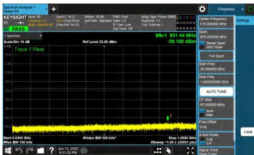
NTNV-DC_2A-n78A(3700-3800)-PC2-30-5+40-M+H-QPSK-IDLE-D FT-BPSK-Inner_1RB_Left-30-1000-PASS
