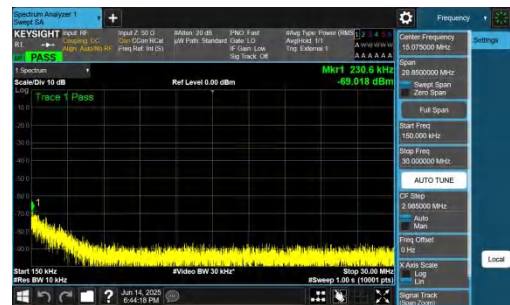
NTNV-DC_2A-n78A(3700-3800)-PC2-30-5+20-M+M-QPSK-IDLE-DFT-QPSK-Inner_1RB_Left-0.15-30-PASS
