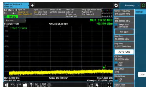
NTNV-DC_2A-n78A(3700-3800)-PC2-30-5+30-M+H-QPSK-IDLE-D FT-BPSK-Inner_1RB_Right-30-1000-PASS
