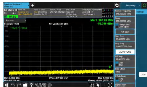
NTNV-DC_2A-n78A(3700-3800)-PC2-30-5+40-M+M-QPSK-IDLE-DFT-BPSK-Inner_1RB_Right-30-1000-PASS
