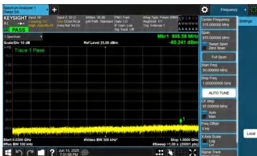
NTNV-DC_2A-n78A(3700-3800)-PC2-30-5+30-M+H-QPSK-IDLE-D FT-QPSK-Inner_1RB_Left-30-1000-PASS
