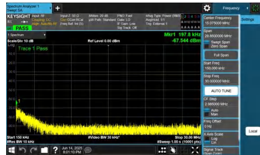
NTNV-DC_2A-n78A(3700-3800)-PC2-30-5+40-M+H-QPSK-IDLE-D FT-BPSK-Inner_1RB_Left-0.15-30-PASS
