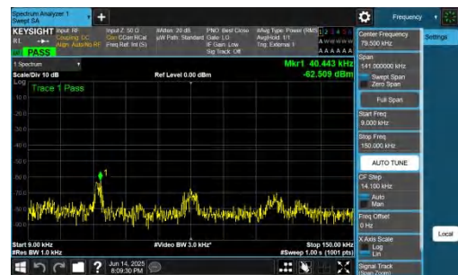
NTNV-DC_2A-n78A(3700-3800)-PC2-30-5+40-M+H-QPSK-IDLE-D FT-QPSK-Inner_1RB_Right-0.009-0.15-PASS
