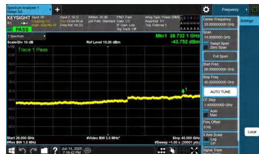
NTNV-DC_2A-n78A(3700-3800)-PC2-30-5+30-M+M-QPSK-IDLE-DFT-BPSK-Inner_1RB_Right-26000-40000-PASS
