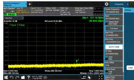
NTNV-DC_2A-n78A(3700-3800)-PC2-30-5+40-M+L-QPSK-IDLE-D FT-BPSK-Inner_1RB_Right-30-1000-PASS
