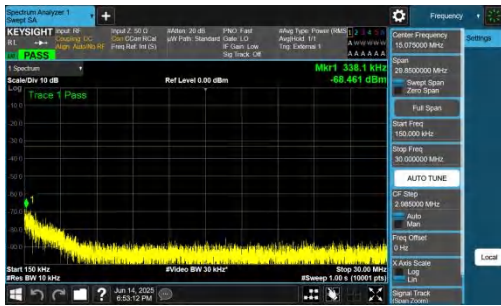
NTNV-DC_2A-n78A(3700-3800)-PC2-30-5+20-M+H-QPSK-IDLE-D FT-BPSK-Inner_1RB_Right-0.15-30-PASS
