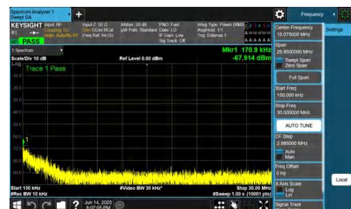
NTNV-DC_2A-n78A(3700-3800)-PC2-30-5+40-M+H-QPSK-IDLE-D FT-QPSK-Inner_1RB_Left-0.15-30-PASS
