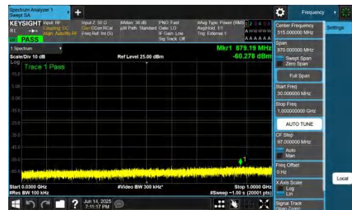
NTNV-DC_2A-n78A(3700-3800)-PC2-30-5+30-M+L-QPSK-IDLE-D FT-QPSK-Inner_1RB_Right-30-1000-PASS
