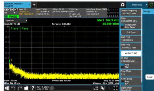
NTNV-DC_2A-n78A(3700-3800)-PC2-30-5+20-M+H-QPSK-IDLE-D FT-BPSK-Inner_1RB_Left-0.15-PASS
