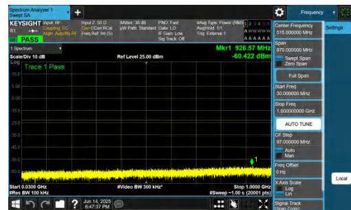
NTNV-DC_2A-n78A(3700-3800)-PC2-30-5+20-M+M-QPSK-IDLE-DFT-QPSK-Inner_1RB_Right-30-1000-PASS
