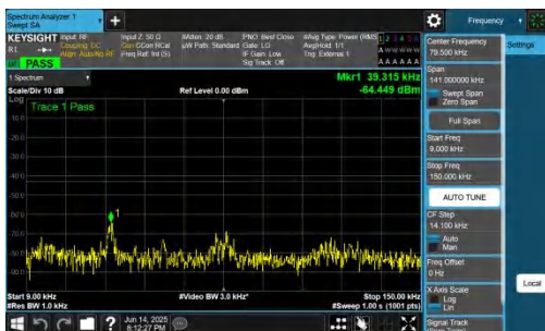
NTNV-DC_2A-n78A(3700-3800)-PC2-30-5+50-M+L-QPSK-IDLE-D FT-BPSK-Inner_1RB_Left-0.009-0.15-PASS
