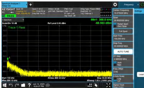
NTNV-DC_2A-n78A(3700-3800)-PC2-30-5+40-M+H-QPSK-IDLE-D FT-BPSK-Inner_1RB_Right-0.15-30-PASS
