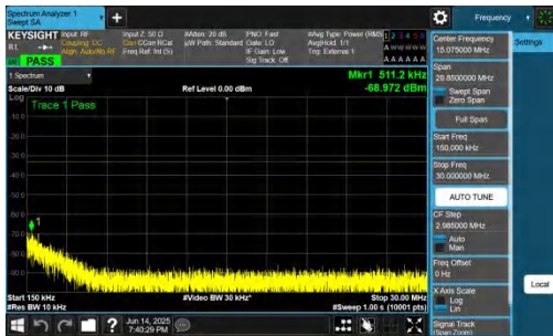
NTNV-DC_2A-n78A(3700-3800)-PC2-30-5+40-M+L-QPSK-IDLE-D FT-BPSK-Inner_1RB_Right-0.15-30-PASS
