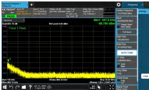
NTNV-DC_2A-n78A(3700-3800)-PC2-30-5+30-M+M-QPSK-IDLE-DFT-BPSK-Inner_1RB_Right-0.15-30-PASS
