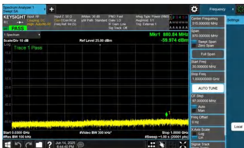
NTNV-DC_2A-n78A(3700-3800)-PC2-30-5+20-M+M-QPSK-IDLE-DFT-QPSK-Inner_1RB_Left-30-1000-PASS
