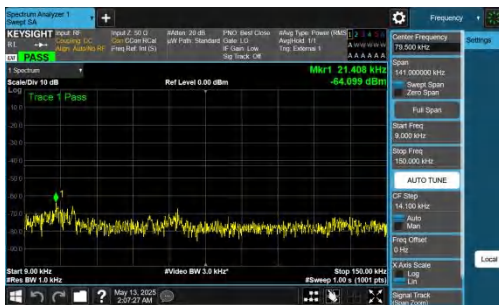
NTNV-DC_2A-n78A(3450-3550)-PC2-30-5+80-M+M-QPSK-IDLE-DFT-QPSK-Inner_1RB_Left-0.009-0.15-PASS
