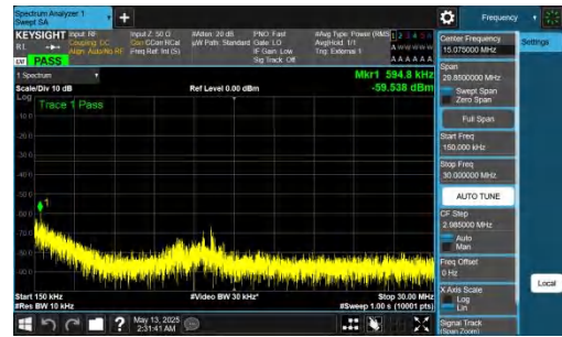
NTNV-DC_2A-n78A(3450-3550)-PC2-30-5+90-M+M-QPSK-IDLE-DFT-BPSK-Inner_1RB_Left-0.15-30-PASS
