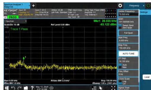
NTNV-DC_2A-n78A(3450-3550)-PC2-30-5+100-M+L-QPSK-IDLE-DFT-QPSK-Inner_1RB_Right-0.009-0.15-PASS
