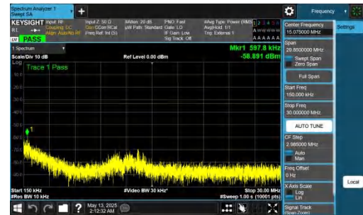
NTNV-DC_2A-n78A(3450-3550)-PC2-30-5+80-M+H-QPSK-IDLE-D FT-BPSK-Inner_1RB_Left-0.15-30-PASS
