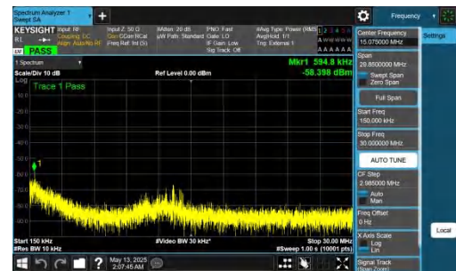
NTNV-DC_2A-n78A(3450-3550)-PC2-30-5+80-M+M-QPSK-IDLE-DFT-QPSK-Inner_1RB_Left-0.15-30-PASS
