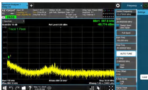
NTNV-DC_2A-n78A(3450-3550)-PC2-30-5+90-M+L-QPSK-IDLE-D FT-BPSK-Inner_1RB_Right-0.15-30-PASS
