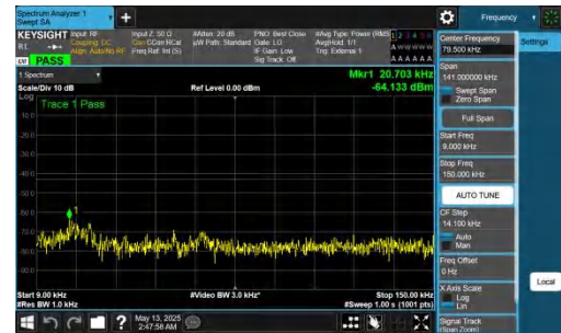
NTNV-DC_2A-n78A(3450-3550)-PC2-30-5+90-M+H-QPSK-IDLE-D FT-QPSK-Inner_1RB_Right-0.009-0.15-PASS
