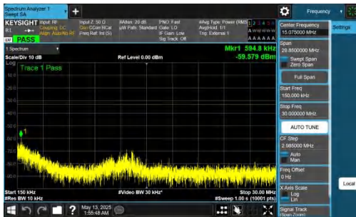
NTNV-DC_2A-n78A(3450-3550)-PC2-30-5+80-M+L-QPSK-IDLE-D FT-BPSK-Inner_1RB_Right-0.15-30-PASS
