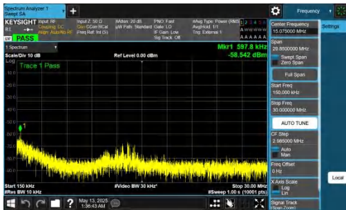
NTNV-DC_2A-n78A(3450-3550)-PC2-30-5+70-M+M-QPSK-IDLE-DFT-BPSK-Inner_1RB_Right-0.15-30-PASS
