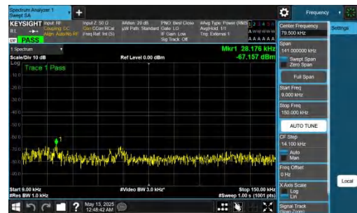
NTNV-DC_2A-n78A(3450-3550)-PC2-30-5+50-M+H-QPSK-IDLE-D FT-BPSK-Inner_1RB_Right-0.009-0.15-PASS
