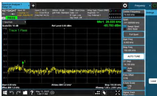
NTNV-DC_2A-n78A(3450-3550)-PC2-30-5+70-M+L-QPSK-IDLE-D FT-QPSK-Inner_1RB_Left-0.009-0.15-PASS
