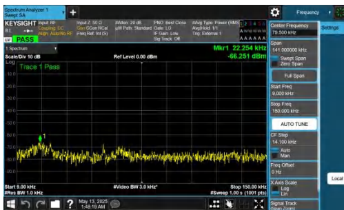
NTNV-DC_2A-n78A(3450-3550)-PC2-30-5+70-M+H-QPSK-IDLE-D FT-QPSK-Inner_1RB_Left-0.009-0.15-PASS
