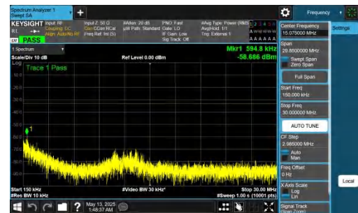
NTNV-DC_2A-n78A(3450-3550)-PC2-30-5+70-M+H-QPSK-IDLE-D FT-QPSK-Inner_1RB_Left-0.15-30-PASS
