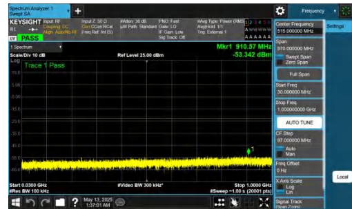
NTNV-DC_2A-n78A(3450-3550)-PC2-30-5+70-M+M-QPSK-IDLE-DFT-BPSK-Inner_1RB_Right-30-1000-PASS
