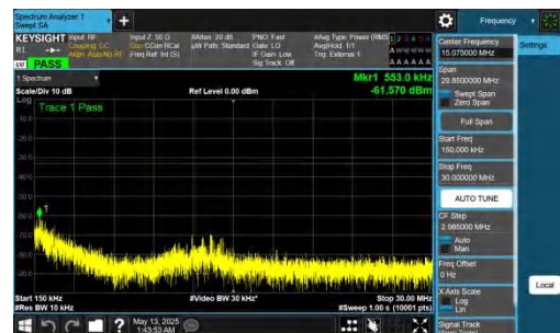
NTNV-DC_2A-n78A(3450-3550)-PC2-30-5+70-M+H-QPSK-IDLE-DFT-BPSK-Inner_1RB_Left-0.15-30-PASS
