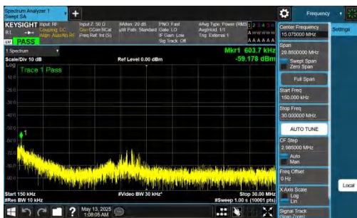
NTNV-DC_2A-n78A(3450-3550)-PC2-30-5+60-M+M-QPSK-IDLE-DFT-BPSK-Inner_1RB_Right-0.15-30-PASS
