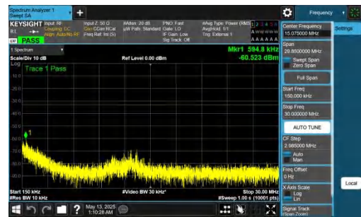
NTNV-DC_2A-n78A(3450-3550)-PC2-30-5+60-M+M-QPSK-IDLE-DFT-QPSK-Inner_1RB_Left-0.15-30-PASS
