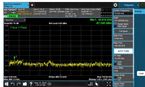
NTNV-DC_2A-n78A(3450-3550)-PC2-30-5+60-M+M-QPSK-IDLE-DFT-BPSK-Inner_1RB_Right-0.009-0.15-PASS
