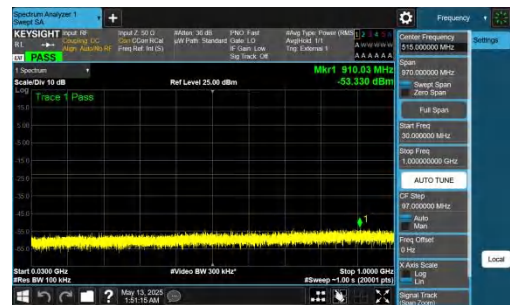
NTNV-DC_2A-n78A(3450-3550)-PC2-30-5+70-M+H-QPSK-IDLE-D FT-QPSK-Inner_1RB_Right-30-1000-PASS
