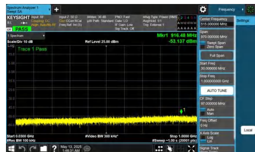
NTNV-DC_2A-n78A(3450-3550)-PC2-30-5+70-M+H-QPSK-IDLE-D FT-BPSK-Inner_1RB_Right-30-1000-PASS
