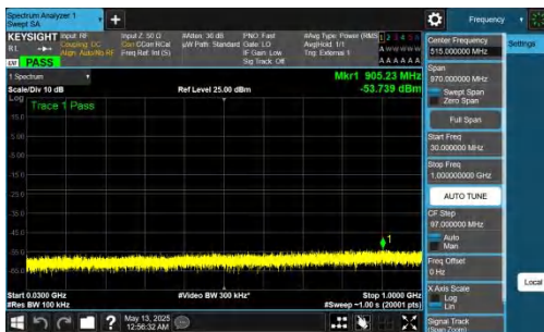
NTNV-DC_2A-n78A(3450-3550)-PC2-30-5+60-M+L-QPSK-IDLE-D FT-BPSK-Inner_1RB_Left-30-1000-PASS
