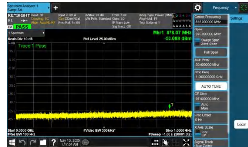
NTNV-DC_2A-n78A(3450-3550)-PC2-30-5+60-M+H-QPSK-IDLE-D FT-BPSK-Inner_1RB_Right-30-1000-PASS
