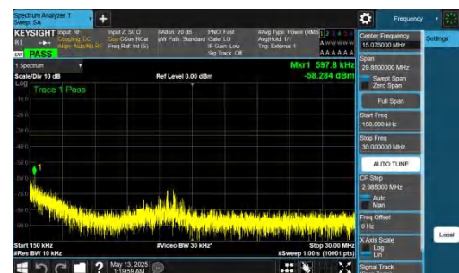
NTNV-DC_2A-n78A(3450-3550)-PC2-30-5+60-M+H-QPSK-IDLE-D FT-QPSK-Inner_1RB_Left-0.15-30-PASS
