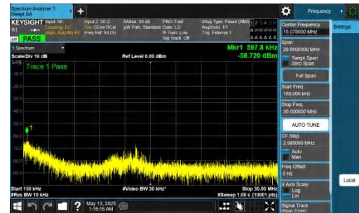
NTNV-DC_2A-n78A(3450-3550)-PC2-30-5+60-M+H-QPSK-IDLE-D FT-BPSK-Inner_1RB_Left-0.15-30-PASS
