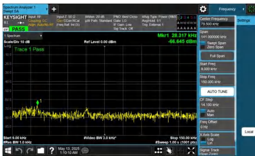
NTNV-DC_2A-n78A(3450-3550)-PC2-30-5+60-M+M-QPSK-IDLE-DFT-QPSK-Inner_1RB_Left-0.009-0.15-PASS
