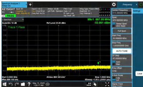
NTNV-DC_2A-n78A(3450-3550)-PC2-30-5+60-M+H-QPSK-IDLE-D FT-QPSK-Inner_1RB_Left-30-1000-PASS
