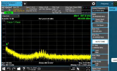
NTNV-DC_2A-n78A(3450-3550)-PC2-30-5+60-M+H-QPSK-IDLE-D FT-BPSK-Inner_1RB_Right-0.15-30-PASS
