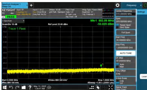
NTNV-DC_2A-n78A(3450-3550)-PC2-30-5+70-M+M-QPSK-IDLE-DFT-BPSK-Inner_1RB_Left-30-1000-PASS
