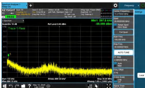
NTNV-DC_2A-n78A(3450-3550)-PC2-30-5+70-M+H-QPSK-IDLE-D FT-BPSK-Inner_1RB_Right-0.15-30-PASS
