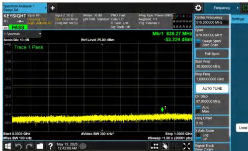
NTNV-DC_2A-n78A(3450-3550)-PC2-30-5+50-M+M-QPSK-IDLE-DFT-QPSK-Inner_1RB_Left-30-1000-PASS
