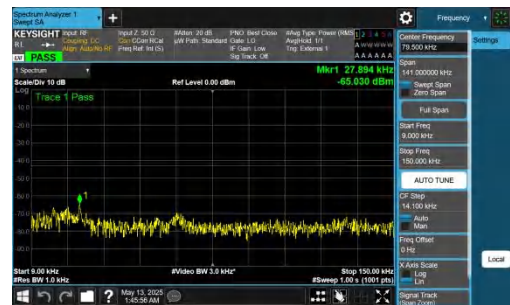
NTNV-DC_2A-n78A(3450-3550)-PC2-30-5+70-M+H-QPSK-IDLE-D FT-BPSK-Inner_1RB_Right-0.009-0.15-PASS
