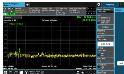
NTNV-DC_2A-n78A(3450-3550)-PC2-30-5+50-M+M-QPSK-IDLE-DFT-QPSK-Inner_1RB_Right-0.009-0.15-PASS
