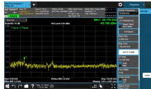
NTNV-DC_2A-n78A(3450-3550)-PC2-30-5+60-M+M-QPSK-IDLE-DFT-QPSK-Inner_1RB_Right-0.009-0.15-PASS
