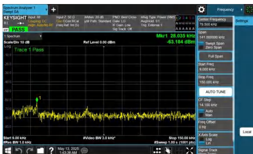
NTNV-DC_2A-n78A(3450-3550)-PC2-30-5+70-M+H-QPSK-IDLE-DFT-BPSK-Inner_1RB_Left-0.009-0.15-PASS
