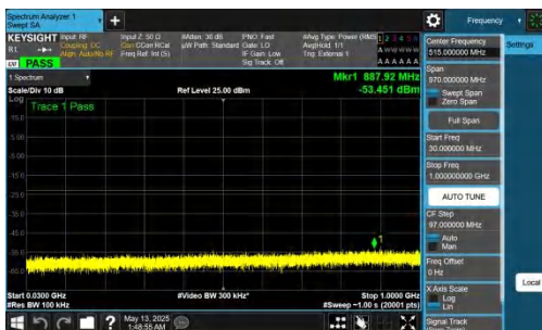
NTNV-DC_2A-n78A(3450-3550)-PC2-30-5+70-M+H-QPSK-IDLE-D FT-QPSK-Inner_1RB_Left-30-1000-PASS
