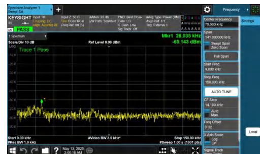
NTNV-DC_2A-n78A(3450-3550)-PC2-30-5+80-M+L-QPSK-IDLE-D FT-QPSK-Inner_1RB_Right-0.009-0.15-PASS
