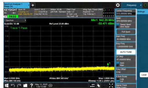
NTNV-DC_2A-n78A(3450-3550)-PC2-30-5+70-M+L-QPSK-IDLE-D FT-QPSK-Inner_1RB_Right-30-1000-PASS
