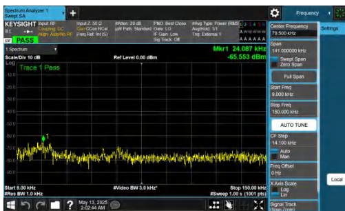
NTNV-DC_2A-n78A(3450-3550)-PC2-30-5+80-M+M-QPSK-IDLE-D DFT-BPSK-Inner_1RB_Left-0.009-0.15-PASS
