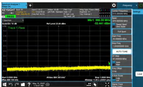
NTNV-DC_2A-n78A(3450-3550)-PC2-30-5+60-M+M-QPSK-IDLE-DFT-QPSK-Inner_1RB_Left-30-1000-PASS
