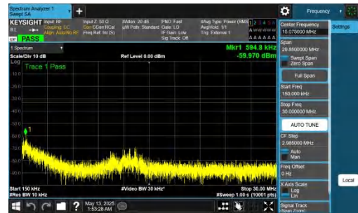
NTNV-DC_2A-n78A(3450-3550)-PC2-30-5+80-M+L-QPSK-IDLE-D FT-BPSK-Inner_1RB_Left-0.15-30-PASS
