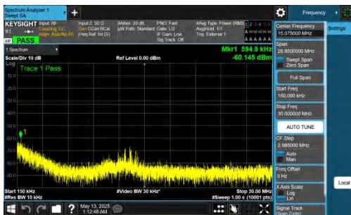
NTNV-DC_2A-n78A(3450-3550)-PC2-30-5+60-M+M-QPSK-IDLE-DFT-QPSK-Inner_1RB_Right-0.15-30-PASS
