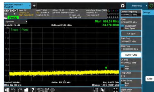
NTNV-DC_2A-n78A(3450-3550)-PC2-30-5+70-M+L-QPSK-IDLE-D FT-BPSK-Inner_1RB_Right-30-1000-PASS
