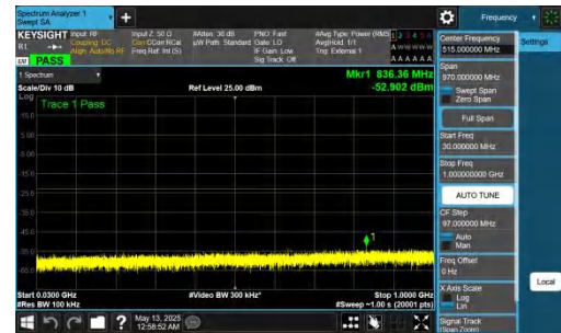
NTNV-DC_2A-n78A(3450-3550)-PC2-30-5+60-M+L-QPSK-IDLE-D FT-BPSK-Inner_1RB_Right-30-1000-PASS
