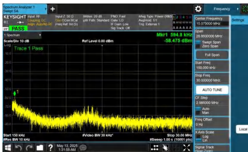
NTNV-DC_2A-n78A(3450-3550)-PC2-30-5+70-M+L-QPSK-IDLE-D FT-QPSK-Inner_1RB_Right-0.15-30-PASS
