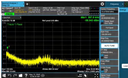
NTNV-DC_2A-n78A(3450-3550)-PC2-30-5+60-M+L-QPSK-IDLE-D FT-BPSK-Inner_1RB_Right-0.15-30-PASS
