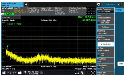
NTNV-DC_2A-n78A(3450-3550)-PC2-30-5+70-M+H-QPSK-IDLE-D FT-QPSK-Inner_1RB_Right-0.15-30-PASS
