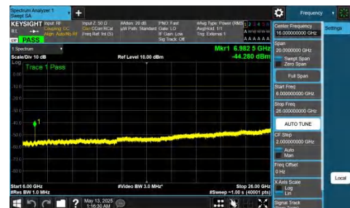
NTNV-DC_2A-n78A(3450-3550)-PC2-30-5+60-M+H-QPSK-IDLE-D FT-BPSK-Inner_1RB_Left-6000-26000-PASS
