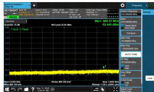
NTNV-DC_2A-n78A(3450-3550)-PC2-30-5+50-M+H-QPSK-IDLE-D FT-QPSK-Inner_1RB_Right-30-1000-PASS
