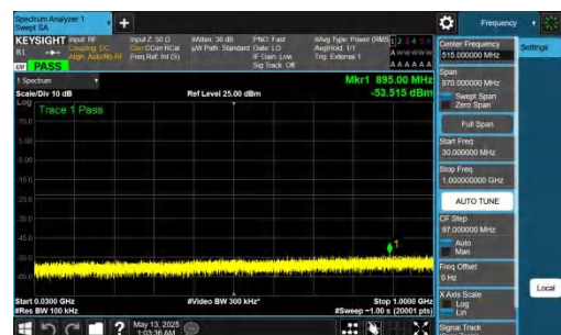
NTNV-DC_2A-n78A(3450-3550)-PC2-30-5+60-M+L-QPSK-IDLE-D FT-QPSK-Inner_1RB_Right-30-1000-PASS
