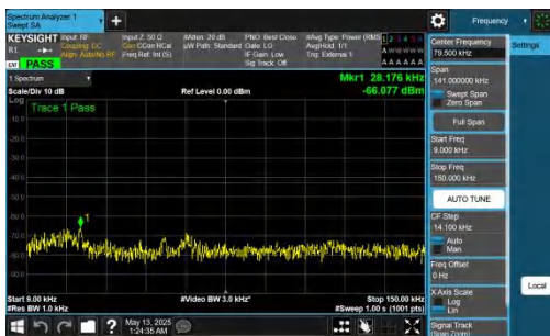
NTNV-DC_2A-n78A(3450-3550)-PC2-30-5+70-M+L-QPSK-IDLE-D FT-BPSK-Inner_1RB_Left-0.009-0.15-PASS
