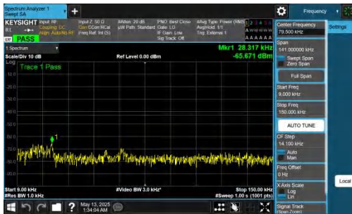
NTNV-DC_2A-n78A(3450-3550)-PC2-30-5+70-M+M-QPSK-IDLE-DFT-BPSK-Inner_1RB_Left-0.009-0.15-PASS
