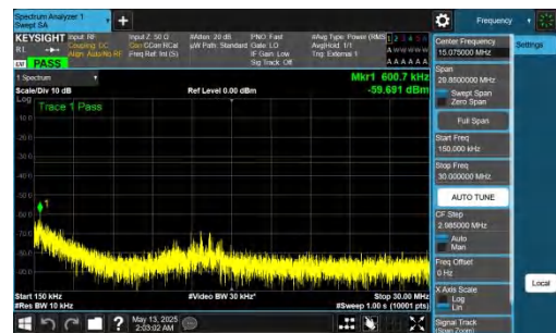
NTNV-DC_2A-n78A(3450-3550)-PC2-30-5+80-M+M-QPSK-IDLE-D FT-BPSK-Inner_1RB_Left-0.15-30-PASS
