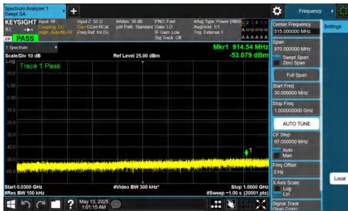
NTNV-DC_2A-n78A(3450-3550)-PC2-30-5+60-M+L-QPSK-IDLE-D FT-QPSK-Inner_1RB_Left-30-1000-PASS
