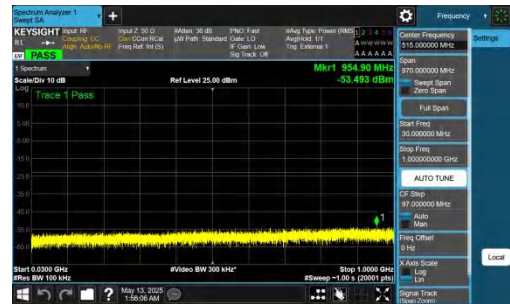
NTNV-DC_2A-n78A(3450-3550)-PC2-30-5+80-M+L-QPSK-IDLE-D FT-BPSK-Inner_1RB_Right-30-1000-PASS
