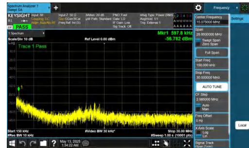
NTNV-DC_2A-n78A(3450-3550)-PC2-30-5+70-M+M-QPSK-IDLE-DFT-BPSK-Inner_1RB_Left-0.15-30-PASS
