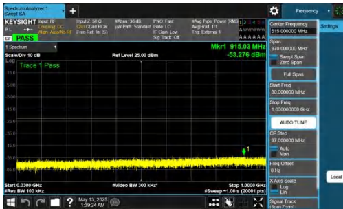
NTNV-DC_2A-n78A(3450-3550)-PC2-30-5+70-M+M-QPSK-IDLE-DFT-QPSK-Inner_1RB_Left-30-1000-PASS
