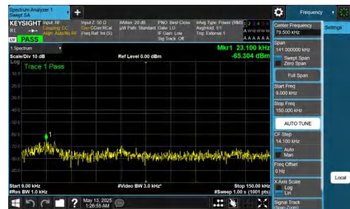
NTNV-DC_2A-n78A(3450-3550)-PC2-30-5+70-M+L-QPSK-IDLE-D FT-BPSK-Inner_1RB_Right-0.009-0.15-PASS
