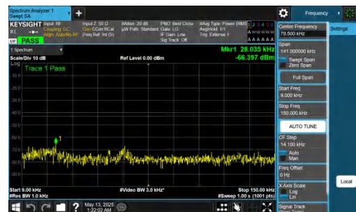
NTNV-DC_2A-n78A(3450-3550)-PC2-30-5+60-M+H-QPSK-IDLE-D FT-QPSK-Inner_1RB_Right-0.009-0.15-PASS
