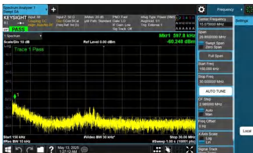
NTNV-DC_2A-n78A(3450-3550)-PC2-30-5+70-M+L-QPSK-IDLE-D FT-BPSK-Inner_1RB_Right-0.15-30-PASS
