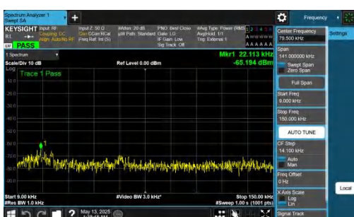
NTNV-DC_2A-n78A(3450-3550)-PC2-30-5+70-M+M-QPSK-IDLE-DFT-QPSK-Inner_1RB_Left-0.009-0.15-PASS
