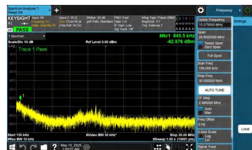
NTNV-DC_2A-n78A(3450-3550)-PC2-30-5+60-M+L-QPSK-IDLE-D FT-QPSK-Inner_1RB_Left-0.15-30-PASS
