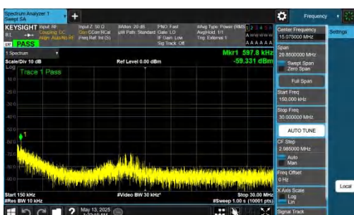
NTNV-DC_2A-n78A(3450-3550)-PC2-30-5+60-M+H-QPSK-IDLE-D FT-QPSK-Inner_1RB_Right-0.15-30-PASS
