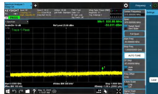
NTNV-DC_2A-n78A(3450-3550)-PC2-30-5+60-M+M-QPSK-IDLE-DFT-QPSK-Inner_1RB_Right-30-1000-PASS
