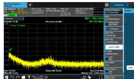
NTNV-DC_2A-n78A(3450-3550)-PC2-30-5+50-M+H-QPSK-IDLE-DFT-BPSK-Inner_1RB_Left-0.15-30-PASS
