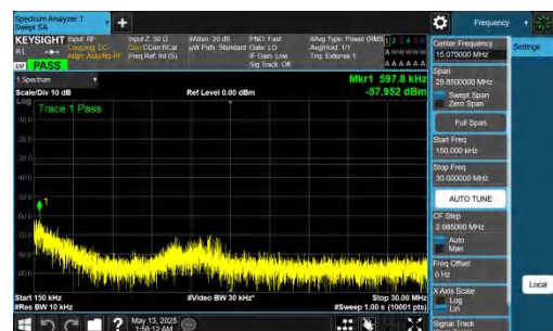
NTNV-DC_2A-n78A(3450-3550)-PC2-30-5+80-M+L-QPSK-IDLE-D FT-QPSK-Inner_1RB_Left-0.15-30-PASS
