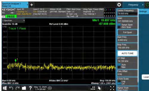
NTNV-DC_2A-n78A(3450-3550)-PC2-30-5+60-M+H-QPSK-IDLE-D FT-BPSK-Inner_1RB_Left-0.009-0.15-PASS
