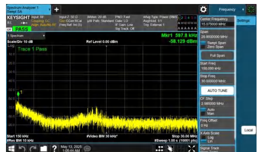
NTNV-DC_2A-n78A(3450-3550)-PC2-30-5+60-M+M-QPSK-IDLE-D FT-BPSK-Inner_1RB_Left-0.15-30-PASS
