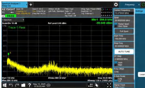
NTNV-DC_2A-n78A(3450-3550)-PC2-30-5+40-M+H-QPSK-IDLE-D FT-BPSK-Inner_1RB_Right-0.15-30-PASS
