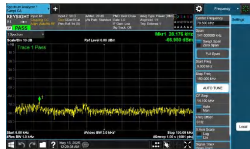
NTNV-DC_2A-n78A(3450-3550)-PC2-30-5+50-M+L-QPSK-IDLE-D FT-BPSK-Inner_1RB_Right-0.009-0.15-PASS
