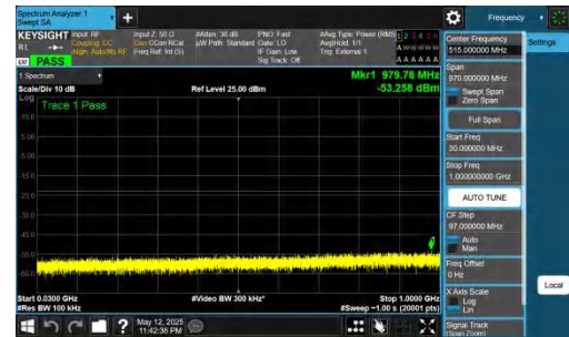
NTNV-DC_2A-n78A(3450-3550)-PC2-30-5+30-M+M-QPSK-IDLE-DFT-BPSK-Inner_1RB_Right-30-1000-PASS
