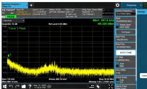
NTNV-DC_2A-n78A(3450-3550)-PC2-30-5+20-M+M-QPSK-IDLE-DFT-QPSK-Inner_1RB_Right-0.15-30-PASS
