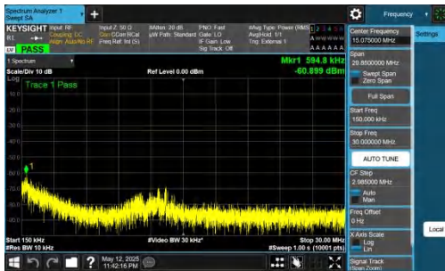
NTNV-DC_2A-n78A(3450-3550)-PC2-30-5+30-M+M-QPSK-IDLE-DFT-BPSK-Inner_1RB_Right-0.15-30-PASS
