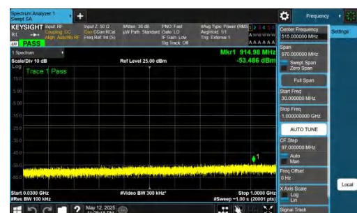
NTNV-DC_2A-n78A(3450-3550)-PC2-30-5+20-M+H-QPSK-IDLE-D FT-QPSK-Inner_1RB_Right-30-1000-PASS
