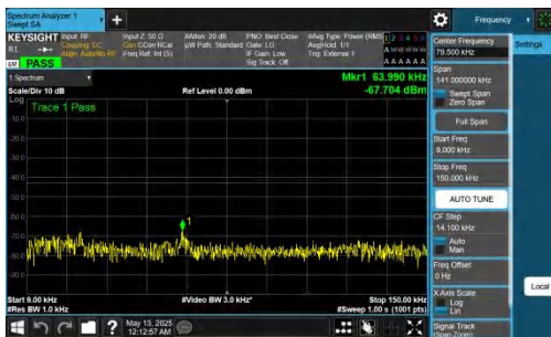
NTNV-DC_2A-n78A(3450-3550)-PC2-30-5+40-M+M-QPSK-IDLE-DFT-QPSK-Inner_1RB_Left-0.009-0.15-PASS
