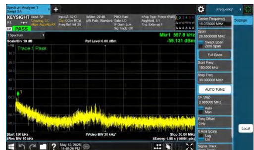
NTNV-DC_2A-n78A(3450-3550)-PC2-30-5+30-M+H-QPSK-IDLE-DFT-BPSK-Inner_1RB_Left-0.15-30-PASS
