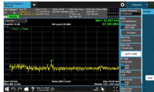
NTNV-DC_2A-n78A(3450-3550)-PC2-30-5+30-M+L-QPSK-IDLE-D FT-QPSK-Inner_1RB_Right-0.009-0.15-PASS
