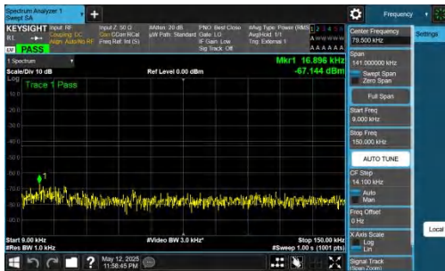
NTNV-DC_2A-n78A(3450-3550)-PC2-30-5+40-M+L-QPSK-IDLE-D FT-BPSK-Inner_1RB_Left-0.009-0.15-PASS
