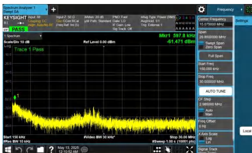
NTNV-DC_2A-n78A(3450-3550)-PC2-30-5+40-M+M-QPSK-IDLE-DFT-BPSK-Inner_1RB_Right-0.15-30-PASS
