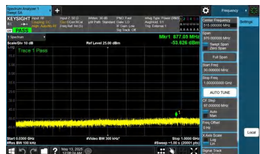
NTNV-DC_2A-n78A(3450-3550)-PC2-30-5+40-M+L-QPSK-IDLE-D FT-QPSK-Inner_1RB_Right-30-1000-PASS
