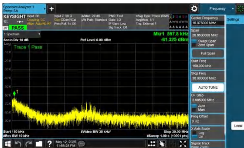
NTNV-DC_2A-n78A(3450-3550)-PC2-30-5+30-M+H-QPSK-IDLE-D FT-QPSK-Inner_1RB_Right-0.15-30-PASS
