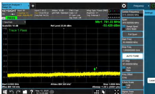
NTNV-DC_2A-n78A(3450-3550)-PC2-30-5+40-M+M-QPSK-IDLE-DFT-QPSK-Inner_1RB_Left-30-1000-PASS
