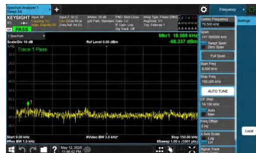
NTNV-DC_2A-n78A(3450-3550)-PC2-30-5+30-M+M-QPSK-IDLE-DFT-QPSK-Inner_1RB_Right-0.009-0.15-PASS
