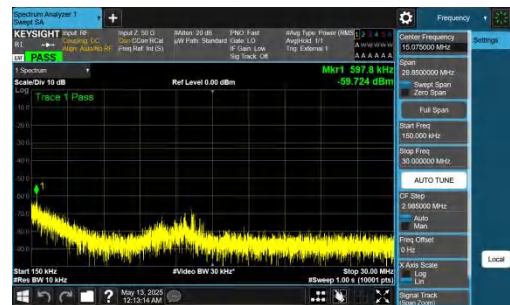
NTNV-DC_2A-n78A(3450-3550)-PC2-30-5+40-M+M-QPSK-IDLE-DFT-QPSK-Inner_1RB_Left-0.15-30-PASS
