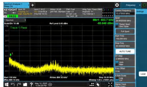
NTNV-DC_2A-n78A(3450-3550)-PC2-30-5+30-M+H-QPSK-IDLE-D FT-QPSK-Inner_1RB_Left-0.15-30-PASS
