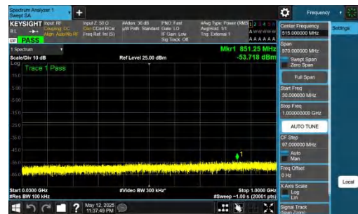
NTNV-DC_2A-n78A(3450-3550)-PC2-30-5+30-M+L-QPSK-IDLE-D FT-QPSK-Inner_1RB_Right-30-1000-PASS
