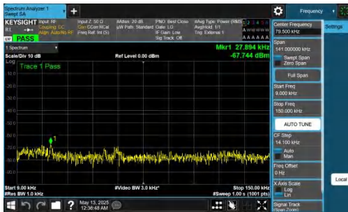
NTNV-DC_2A-n78A(3450-3550)-PC2-30-5+50-M+M-QPSK-IDLE-DFT-BPSK-Inner_1RB_Left-0.009-0.15-PASS
