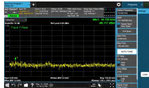
NTNV-DC_2A-n78A(3450-3550)-PC2-30-5+20-M+M-QPSK-IDLE-DFT-QPSK-Inner_1RB_Right-0.009-0.15-PASS
