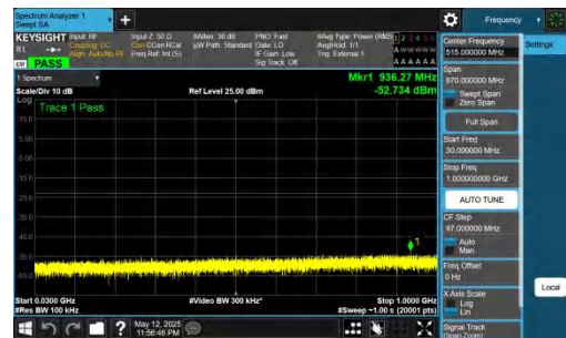
NTNV-DC_2A-n78A(3450-3550)-PC2-30-5+30-M+H-QPSK-IDLE-D FT-QPSK-Inner_1RB_Right-30-1000-PASS
