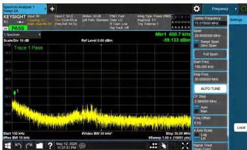
NTNV-DC_2A-n78A(3450-3550)-PC2-30-5+30-M+L-QPSK-IDLE-D FT-QPSK-Inner_1RB_Right-0.15-30-PASS
