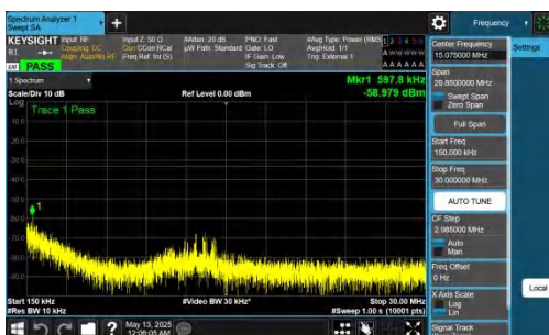
NTNV-DC_2A-n78A(3450-3550)-PC2-30-5+40-M+L-QPSK-IDLE-D FT-QPSK-Inner_1RB_Right-0.15-30-PASS
