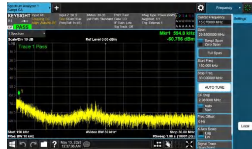
NTNV-DC_2A-n78A(3450-3550)-PC2-30-5+50-M+M-QPSK-IDLE-DFT-BPSK-Inner_1RB_Left-0.15-30-PASS
