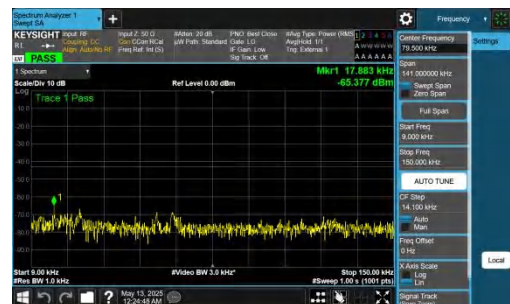
NTNV-DC_2A-n78A(3450-3550)-PC2-30-5+40-M+H-QPSK-IDLE-D FT-QPSK-Inner_1RB_Right-0.009-0.15-PASS
