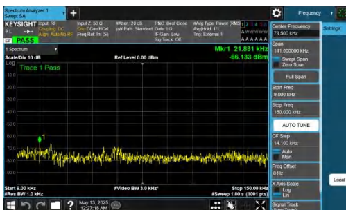
NTNV-DC_2A-n78A(3450-3550)-PC2-30-5+50-M+L-QPSK-IDLE-D FT-BPSK-Inner_1RB_Left-0.009-0.15-PASS
