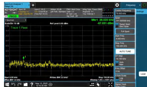
NTNV-DC_2A-n78A(3450-3550)-PC2-30-5+40-M+M-QPSK-IDLE-DFT-BPSK-Inner_1RB_Right-0.009-0.15-PASS
