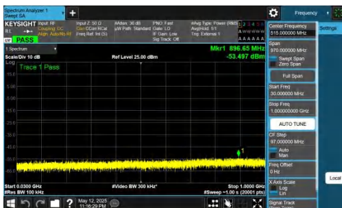
NTNV-DC_2A-n78A(3450-3550)-PC2-30-5+20-M+M-QPSK-IDLE-DFT-QPSK-Inner_1RB_Left-30-1000-PASS
