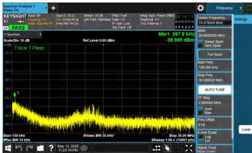
NTNV-DC_2A-n78A(3450-3550)-PC2-30-5+20-M+H-QPSK-IDLE-D FT-BPSK-Inner_1RB_Right-0.15-30-PASS
