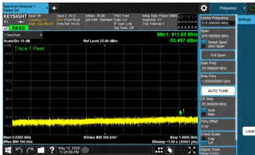
NTNV-DC_2A-n78A(3450-3550)-PC2-30-5+20-M+H-QPSK-IDLE-D FT-QPSK-Inner_1RB_Left-30-1000-PASS
