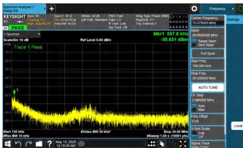
NTNV-DC_2A-n78A(3450-3550)-PC2-30-5+40-M+M-QPSK-IDLE-DFT-QPSK-Inner_1RB_Right-0.15-30-PASS
