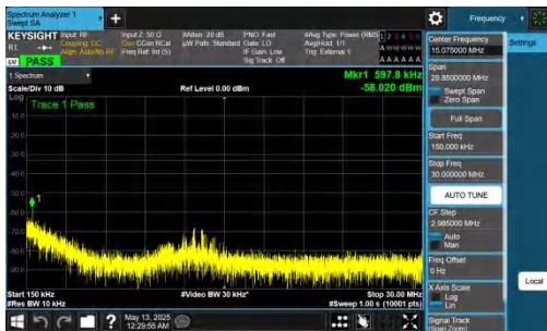
NTNV-DC_2A-n78A(3450-3550)-PC2-30-5+50-M+L-QPSK-IDLE-D FT-BPSK-Inner_1RB_Right-0.15-30-PASS
