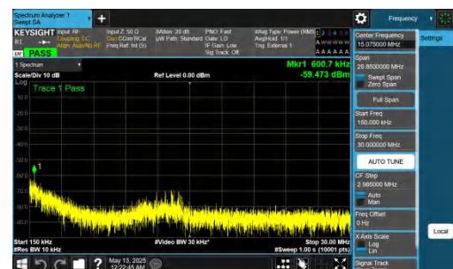
NTNV-DC_2A-n78A(3450-3550)-PC2-30-5+40-M+H-QPSK-IDLE-D FT-QPSK-Inner_1RB_Left-0.15-30-PASS
