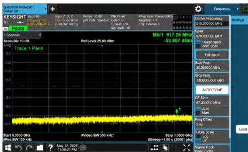
NTNV-DC_2A-n78A(3450-3550)-PC2-30-5+40-M+L-QPSK-IDLE-D FT-BPSK-Inner_1RB_Left-30-1000-PASS
