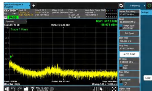
NTNV-DC_2A-n78A(3450-3550)-PC2-30-5+30-M+L-QPSK-IDLE-D FT-BPSK-Inner_1RB_Left-0.15-30-PASS
