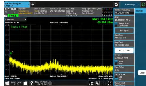
NTNV-DC_2A-n78A(3450-3550)-PC2-30-5+20-M+H-QPSK-IDLE-D FT-BPSK-Inner_1RB_Left-0.15-30-PASS
