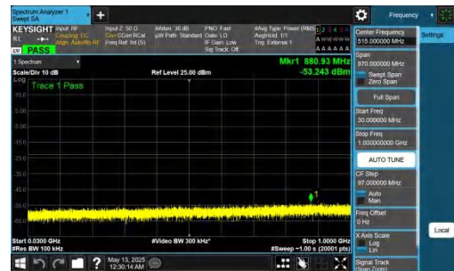
NTNV-DC_2A-n78A(3450-3550)-PC2-30-5+50-M+L-QPSK-IDLE-D FT-BPSK-Inner_1RB_Right-30-1000-PASS
