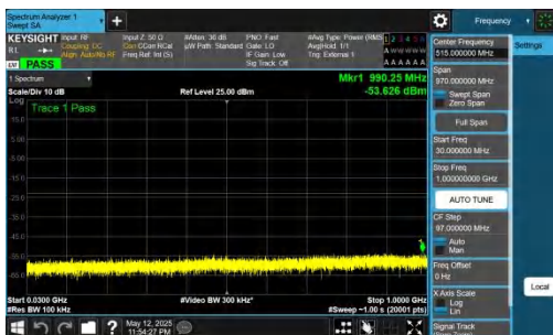
NTNV-DC_2A-n78A(3450-3550)-PC2-30-5+30-M+H-QPSK-IDLE-D FT-QPSK-Inner_1RB_Left-30-1000-PASS
