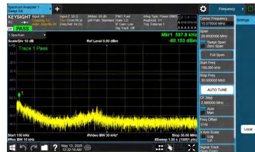
NTNV-DC_2A-n78A(3450-3550)-PC2-30-5+50-M+L-QPSK-IDLE-D FT-QPSK-Inner_1RB_Left-0.15-30-PASS
