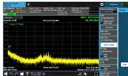
NTNV-DC_2A-n78A(3450-3550)-PC2-30-5+20-M+M-QPSK-IDLE-DFT-QPSK-Inner_1RB_Left-0.15-30-PASS
