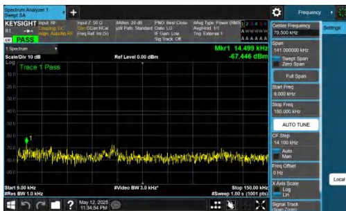
NTNV-DC_2A-n78A(3450-3550)-PC2-30-5+30-M+L-QPSK-IDLE-D FT-QPSK-Inner_1RB_Left-0.009-0.15-PASS
