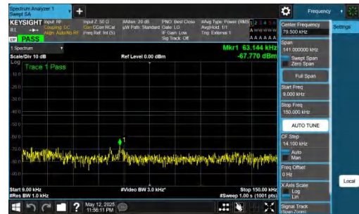
NTNV-DC_2A-n78A(3450-3550)-PC2-30-5+30-M+H-QPSK-IDLE-D FT-QPSK-Inner_1RB_Right-0.009-0.15-PASS
