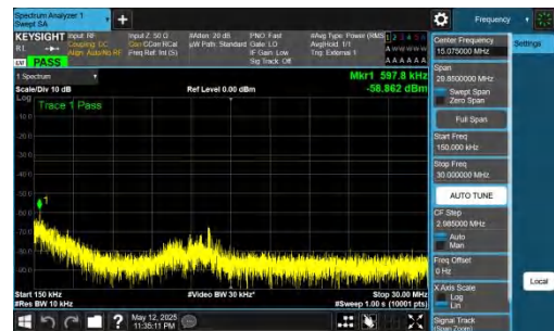
NTNV-DC_2A-n78A(3450-3550)-PC2-30-5+30-M+L-QPSK-IDLE-D FT-QPSK-Inner_1RB_Left-0.15-30-PASS
