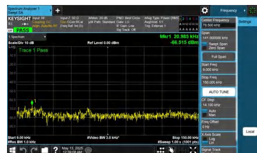
NTNV-DC_2A-n78A(3450-3550)-PC2-30-5+50-M+M-QPSK-IDLE-DFT-BPSK-Inner_1RB_Right-0.009-0.15-PASS
