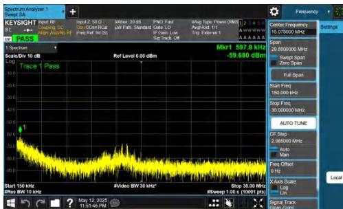
NTNV-DC_2A-n78A(3450-3550)-PC2-30-5+30-M+H-QPSK-IDLE-D FT-BPSK-Inner_1RB_Right-0.15-30-PASS
