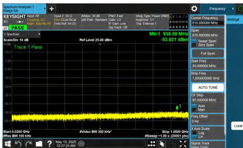
NTNV-DC_2A-n78A(3450-3550)-PC2-30-5+50-M+M-QPSK-IDLE-DFT-BPSK-Inner_1RB_Left-30-1000-PASS
