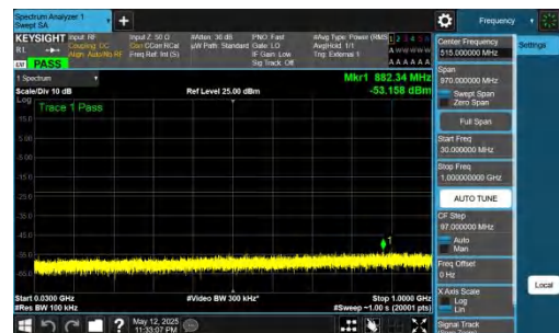
NTNV-DC_2A-n78A(3450-3550)-PC2-30-5+30-M+L-QPSK-IDLE-D FT-BPSK-Inner_1RB_Right-30-1000-PASS
