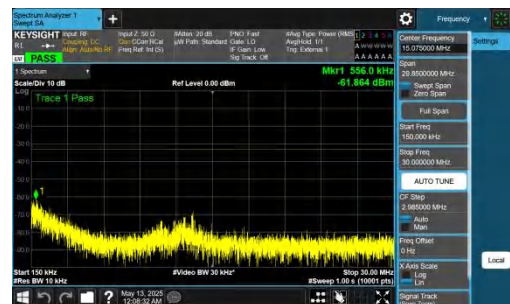
NTNV-DC_2A-n78A(3450-3550)-PC2-30-5+40-M+M-QPSK-IDLE-D FT-BPSK-Inner_1RB_Left-0.15-30-PASS
