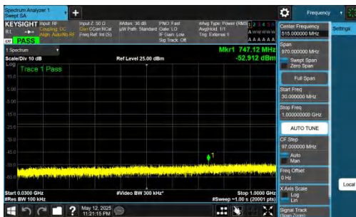
NTNV-DC_2A-n78A(3450-3550)-PC2-30-5+20-M+H-QPSK-IDLE-D FT-BPSK-Inner_1RB_Left-30-1000-PASS
