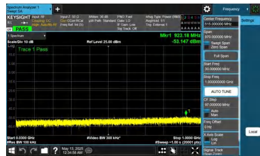
NTNV-DC_2A-n78A(3450-3550)-PC2-30-5+50-M+L-QPSK-IDLE-D FT-QPSK-Inner_1RB_Right-30-1000-PASS
