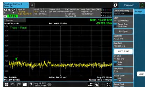
NTNV-DC_2A-n78A(3450-3550)-PC2-30-5+30-M+H-QPSK-IDLE-D FT-BPSK-Inner_1RB_Right-0.009-0.15-PASS
