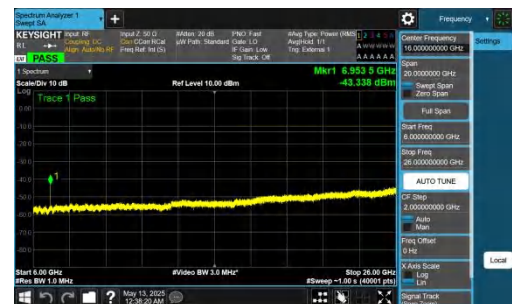
NTNV-DC_2A-n78A(3450-3550)-PC2-30-5+50-M+M-QPSK-IDLE-DFT-BPSK-Inner_1RB_Left-6000-26000-PASS
