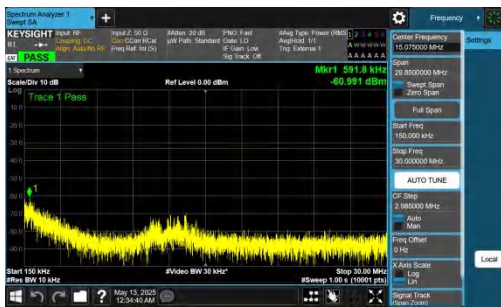
NTNV-DC_2A-n78A(3450-3550)-PC2-30-5+50-M+L-QPSK-IDLE-D FT-QPSK-Inner_1RB_Right-0.15-30-PASS
