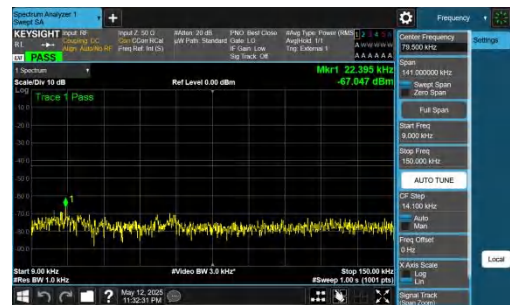
NTNV-DC_2A-n78A(3450-3550)-PC2-30-5+30-M+L-QPSK-IDLE-D FT-BPSK-Inner_1RB_Right-0.009-0.15-PASS
