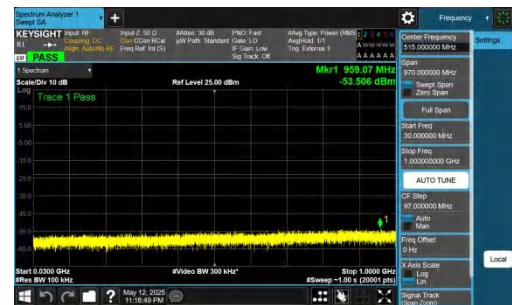
NTNV-DC_2A-n78A(3450-3550)-PC2-30-5+20-M+M-QPSK-IDLE-DFT-QPSK-Inner_1RB_Right-30-1000-PASS
