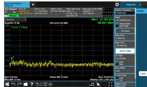
NTNV-DC_2A-n78A(3450-3550)-PC2-30-5+40-M+M-QPSK-IDLE-DFT-QPSK-Inner_1RB_Right-0.009-0.15-PASS
