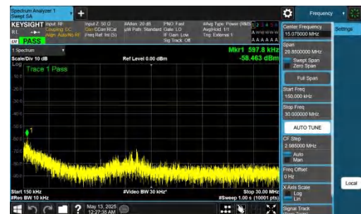
NTNV-DC_2A-n78A(3450-3550)-PC2-30-5+50-M+L-QPSK-IDLE-D FT-BPSK-Inner_1RB_Left-0.15-30-PASS
