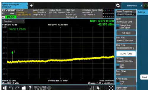
NTNV-DC_2A-n78A(3450-3550)-PC2-30-5+40-M+L-QPSK-IDLE-D FT-BPSK-Inner_1RB_Right-6000-26000-PASS
