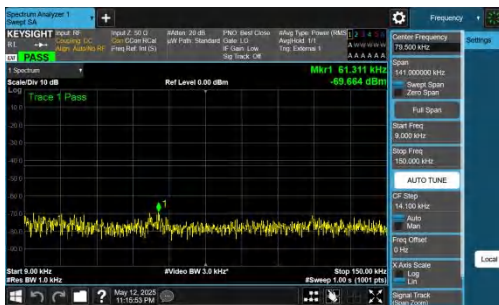
NTNV-DC_2A-n78A(3450-3550)-PC2-30-5+20-M+M-QPSK-IDLE-DFT-QPSK-Inner_1RB_Left-0.009-0.15-PASS
