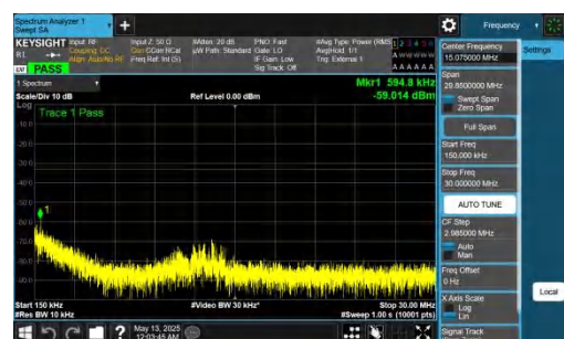
NTNV-DC_2A-n78A(3450-3550)-PC2-30-5+40-M+L-QPSK-IDLE-D FT-QPSK-Inner_1RB_Left-0.15-30-PASS
