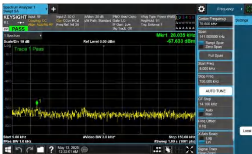
NTNV-DC_2A-n78A(3450-3550)-PC2-30-5+50-M+L-QPSK-IDLE-D FT-QPSK-Inner_1RB_Left-0.009-0.15-PASS
