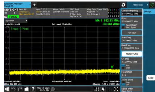
NTNV-DC_2A-n78A(3450-3550)-PC2-30-5+20-M+H-QPSK-IDLE-D FT-BPSK-Inner_1RB_Right-30-1000-PASS
