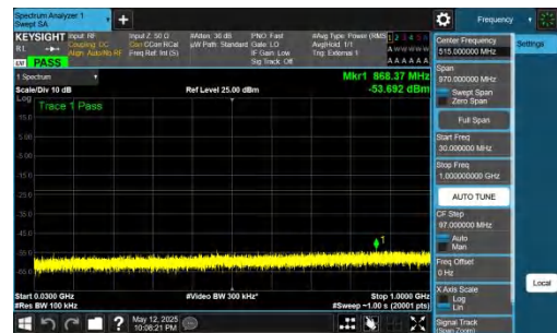
NTNV-DC_2A-n77A(3700-3980)-PC2-30-5+100-M+L-QPSK-IDLE-DFT-QPSK-Inner_1RB_Right-30-1000-PASS
