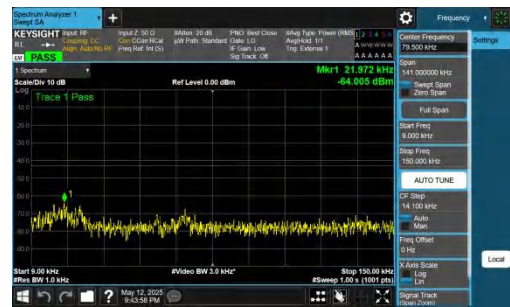
NTNV-DC_2A-n77A(3700-3980)-PC2-30-5+80-M+M-QPSK-IDLE-DFT-BPSK-Inner_1RB_Right-0.009-0.15-PASS
