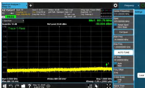
NTNV-DC_2A-n77A(3700-3980)-PC2-30-5+80-M+M-QPSK-IDLE-DFT-QPSK-Inner_1RB_Left-30-1000-PASS
