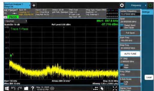
NTNV-DC_2A-n77A(3700-3980)-PC2-30-5+100-M+L-QPSK-IDLE-DFT-QPSK-Inner_1RB_Left-0.15-30-PASS
