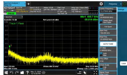
NTNV-DC_2A-n77A(3700-3980)-PC2-30-5+100-M+M-QPSK-IDLE-DFT-BPSK-Inner_1RB_Left-0.15-30-PASS
