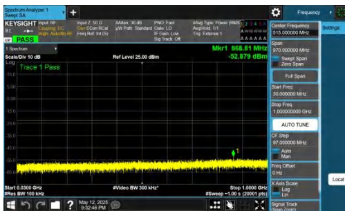
NTNV-DC_2A-n77A(3700-3980)-PC2-30-5+80-M+L-QPSK-IDLE-D FT-BPSK-Inner_1RB_Left-30-1000-PASS
