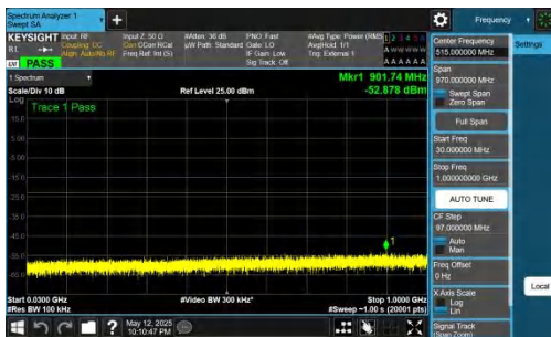
NTNV-DC_2A-n77A(3700-3980)-PC2-30-5+100-M+M-QPSK-IDLE-DFT-BPSK-Inner_1RB_Left-30-1000-PASS
