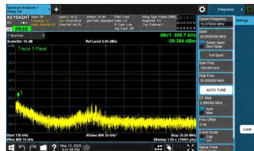
NTNV-DC_2A-n77A(3700-3980)-PC2-30-5+80-M+M-QPSK-IDLE-D FT-BPSK-Inner_1RB_Left-0.15-30-PASS
