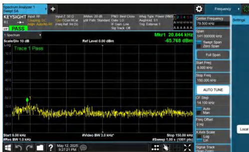
NTNV-DC_2A-n77A(3700-3980)-PC2-30-5+60-M+H-QPSK-IDLE-D FT-QPSK-Inner_1RB_Left-0.009-0.15-PASS
