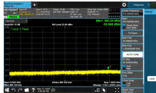
NTNV-DC_2A-n77A(3700-3980)-PC2-30-5+80-M+L-QPSK-IDLE-D FT-BPSK-Inner_1RB_Right-30-1000-PASS
