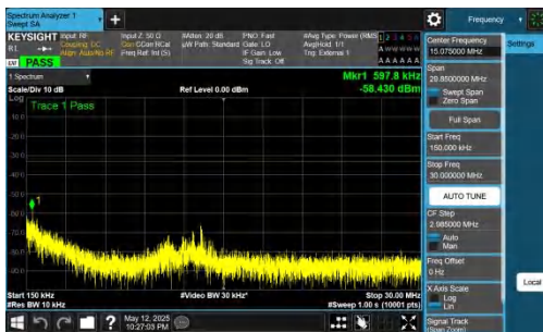
NTNV-DC_2A-n77A(3700-3980)-PC2-30-5+100-M+H-QPSK-IDLE-DFT-QPSK-Inner_1RB_Right-0.15-30-PASS
