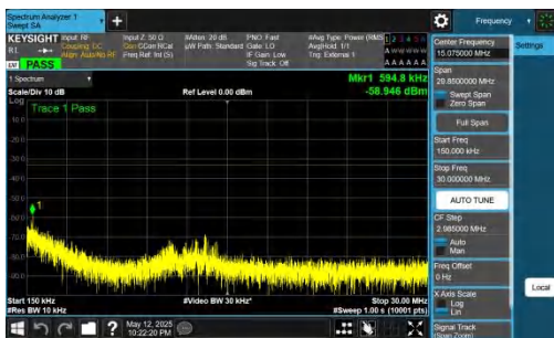
NTNV-DC_2A-n77A(3700-3980)-PC2-30-5+100-M+H-QPSK-IDLE-DFT-BPSK-Inner_1RB_Right-0.15-30-PASS
