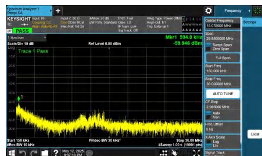
NTNV-DC_2A-n77A(3700-3980)-PC2-30-5+80-M+L-QPSK-IDLE-D FT-QPSK-Inner_1RB_Left-0.15-30-PASS
