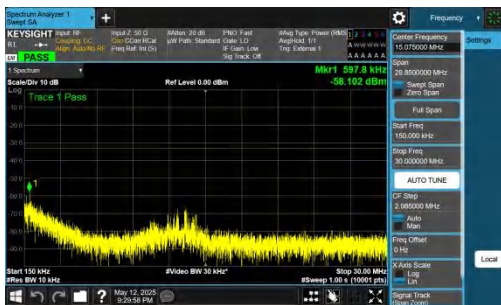
NTNV-DC_2A-n77A(3700-3980)-PC2-30-5+60-M+H-QPSK-IDLE-D FT-QPSK-Inner_1RB_Right-0.15-30-PASS
