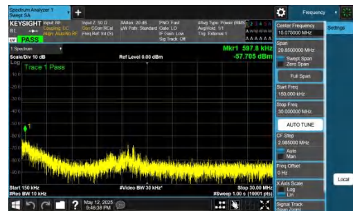
NTNV-DC_2A-n77A(3700-3980)-PC2-30-5+80-M+M-QPSK-IDLE-DFT-QPSK-Inner_1RB_Left-0.15-30-PASS
