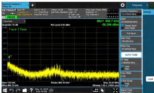
NTNV-DC_2A-n77A(3700-3980)-PC2-30-5+80-M+M-QPSK-IDLE-DFT-BPSK-Inner_1RB_Right-0.15-30-PASS
