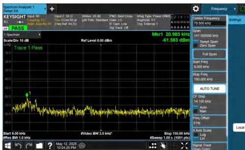
NTNV-DC_2A-n77A(3700-3980)-PC2-30-5+100-M+H-QPSK-IDLE-DFT-QPSK-Inner_1RB_Left-0.009-0.15-PASS
