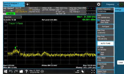
NTNV-DC_2A-n77A(3700-3980)-PC2-30-5+100-M+H-QPSK-IDLE-DFT-BPSK-Inner_1RB_Right-0.009-0.15-PASS
