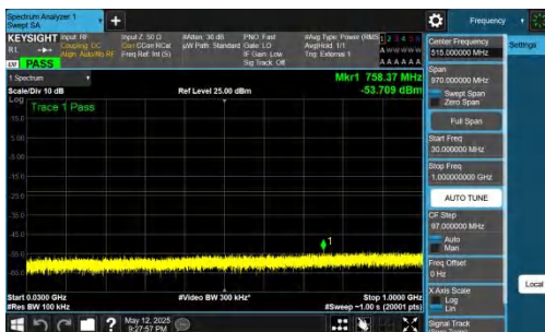
NTNV-DC_2A-n77A(3700-3980)-PC2-30-5+60-M+H-QPSK-IDLE-D FT-QPSK-Inner_1RB_Left-30-1000-PASS
