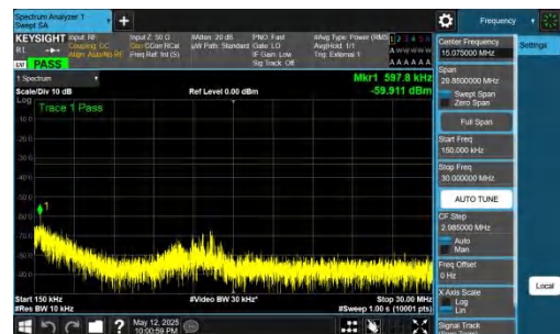
NTNV-DC_2A-n77A(3700-3980)-PC2-30-5+100-M+L-QPSK-IDLE-D FT-BPSK-Inner_1RB_Left-0.15-30-PASS
