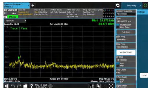
NTNV-DC_2A-n77A(3700-3980)-PC2-30-5+80-M+H-QPSK-IDLE-D FT-QPSK-Inner_1RB_Right-0.009-0.15-PASS
