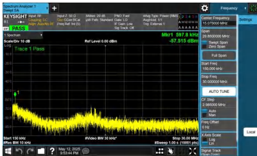
NTNV-DC_2A-n77A(3700-3980)-PC2-30-5+80-M+H-QPSK-IDLE-D FT-BPSK-Inner_1RB_Right-0.15-30-PASS
