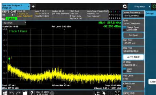
NTNV-DC_2A-n77A(3700-3980)-PC2-30-5+80-M+L-QPSK-IDLE-D FT-QPSK-Inner_1RB_Right-0.15-30-PASS
