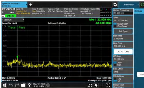
NTNV-DC_2A-n77A(3700-3980)-PC2-30-5+80-M+L-QPSK-IDLE-D FT-BPSK-Inner_1RB_Left-0.009-0.15-PASS
