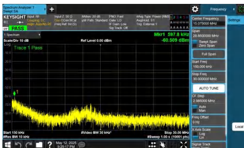
NTNV-DC_2A-n77A(3700-3980)-PC2-30-5+60-M+H-QPSK-IDLE-D FT-BPSK-Inner_1RB_Right-0.15-30-PASS
