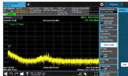
NTNV-DC_2A-n77A(3700-3980)-PC2-30-5+100-M+H-QPSK-IDLE-DFT-QPSK-Inner_1RB_Left-0.15-30-PASS
