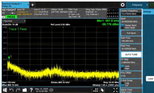
NTNV-DC_2A-n77A(3700-3980)-PC2-30-5+100-M+M-QPSK-IDLE-DFT-BPSK-Inner_1RB_Right-0.15-30-PASS
