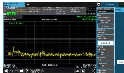
NTNV-DC_2A-n77A(3700-3980)-PC2-30-5+60-M+H-QPSK-IDLE-D FT-BPSK-Inner_1RB_Right-0.009-0.15-PASS
