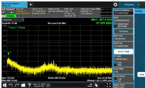
NTNV-DC_2A-n77A(3700-3980)-PC2-30-5+80-M+L-QPSK-IDLE-D FT-BPSK-Inner_1RB_Right-0.15-30-PASS
