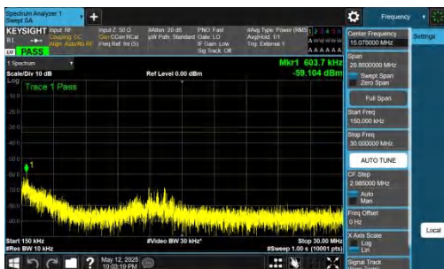
NTNV-DC_2A-n77A(3700-3980)-PC2-30-5+100-M+L-QPSK-IDLE-DFT-BPSK-Inner_1RB_Right-0.15-30-PASS
