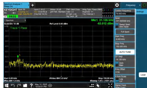
NTNV-DC_2A-n77A(3700-3980)-PC2-30-5+100-M+L-QPSK-IDLE-DFT-BPSK-Inner_1RB_Right-0.009-0.15-PASS
