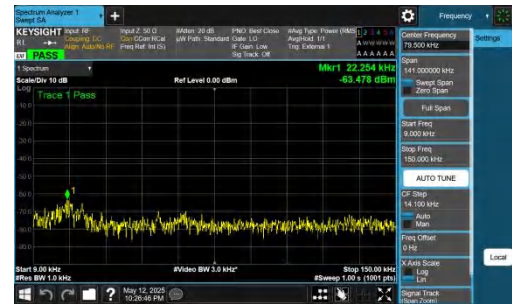
NTNV-DC_2A-n77A(3700-3980)-PC2-30-5+100-M+H-QPSK-IDLE-DFT-QPSK-Inner_1RB_Right-0.009-0.15-PASS
