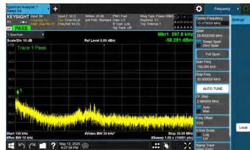
NTNV-DC_2A-n77A(3700-3980)-PC2-30-5+60-M+H-QPSK-IDLE-D FT-QPSK-Inner_1RB_Left-0.15-30-PASS
