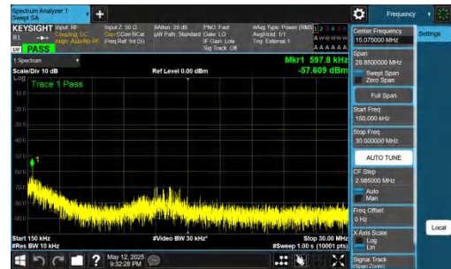
NTNV-DC_2A-n77A(3700-3980)-PC2-30-5+80-M+L-QPSK-IDLE-D FT-BPSK-Inner_1RB_Left-0.15-30-PASS
