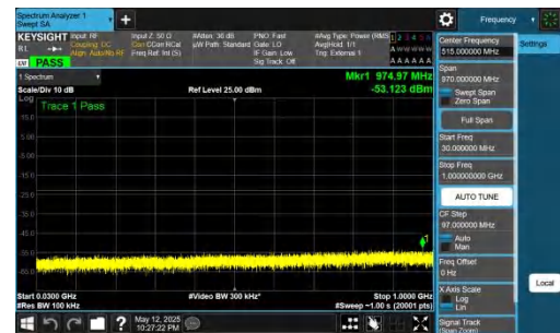
NTNV-DC_2A-n77A(3700-3980)-PC2-30-5+100-M+H-QPSK-IDLE-DFT-QPSK-Inner_1RB_Right-30-1000-PASS
