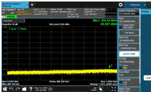
NTNV-DC_2A-n77A(3700-3980)-PC2-30-5+80-M+L-QPSK-IDLE-D FT-QPSK-Inner_1RB_Left-30-1000-PASS
