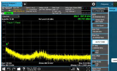
NTNV-DC_2A-n77A(3700-3980)-PC2-30-5+100-M+L-QPSK-IDLE-DFT-QPSK-Inner_1RB_Right-0.15-30-PASS
