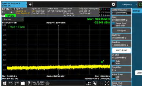
NTNV-DC_2A-n77A(3700-3980)-PC2-30-5+80-M+H-QPSK-IDLE-D FT-QPSK-Inner_1RB_Left-30-1000-PASS
