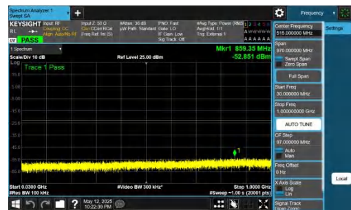
NTNV-DC_2A-n77A(3700-3980)-PC2-30-5+100-M+H-QPSK-IDLE-DFT-BPSK-Inner_1RB_Right-30-1000-PASS
