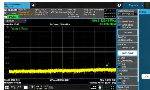
NTNV-DC_2A-n77A(3700-3980)-PC2-30-5+60-M+H-QPSK-IDLE-D FT-QPSK-Inner_1RB_Right-30-1000-PASS
