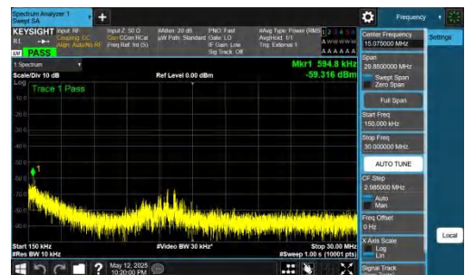
NTNV-DC_2A-n77A(3700-3980)-PC2-30-5+100-M+H-QPSK-IDLE-DFT-BPSK-Inner_1RB_Left-0.15-30-PASS
