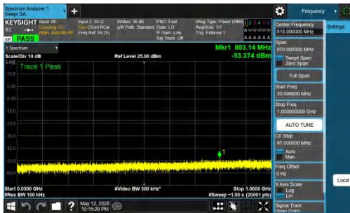
NTNV-DC_2A-n77A(3700-3980)-PC2-30-5+100-M+M-QPSK-IDLE-DFT-QPSK-Inner_1RB_Left-30-1000-PASS
