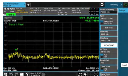
NTNV-DC_2A-n77A(3700-3980)-PC2-30-5+80-M+L-QPSK-IDLE-D FT-QPSK-Inner_1RB_Right-0.009-0.15-PASS
