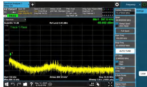
NTNV-DC_2A-n77A(3700-3980)-PC2-30-5+30-M+M-QPSK-IDLE-DFT-BPSK-Inner_1RB_Left-0.15-30-PASS
