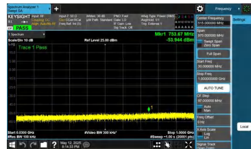
NTNV-DC_2A-n77A(3700-3980)-PC2-30-5+30-M+L-QPSK-IDLE-D FT-QPSK-Inner_1RB_Right-30-1000-PASS
