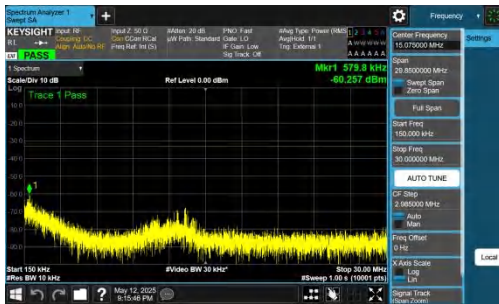
NTNV-DC_2A-n77A(3700-3980)-PC2-30-5+60-M+M-QPSK-IDLE-DFT-BPSK-Inner_1RB_Right-0.15-30-PASS
