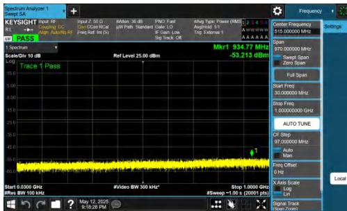
NTNV-DC_2A-n77A(3700-3980)-PC2-30-5+60-M+M-QPSK-IDLE-DFT-QPSK-Inner_1RB_Left-30-1000-PASS
