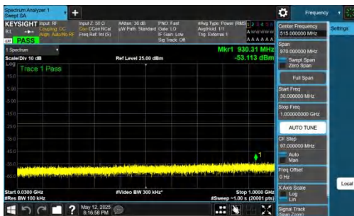
NTNV-DC_2A-n77A(3700-3980)-PC2-30-5+30-M+M-QPSK-IDLE-DFT-BPSK-Inner_1RB_Left-30-1000-PASS
