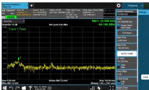
NTNV-DC_2A-n77A(3700-3980)-PC2-30-5+60-M+L-QPSK-IDLE-D FT-BPSK-Inner_1RB_Left-0.009-0.15-PASS
