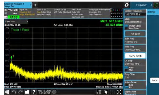
NTNV-DC_2A-n77A(3700-3980)-PC2-30-5+40-M+L-QPSK-IDLE-D FT-BPSK-Inner_1RB_Left-0.15-30-PASS
