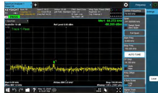
NTNV-DC_2A-n77A(3700-3980)-PC2-30-5+30-M+L-QPSK-IDLE-D FT-QPSK-Inner_1RB_Right-0.009-0.15-PASS
