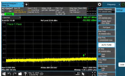
NTNV-DC_2A-n77A(3700-3980)-PC2-30-5+40-M+L-QPSK-IDLE-D FT-BPSK-Inner_1RB_Left-30-1000-PASS
