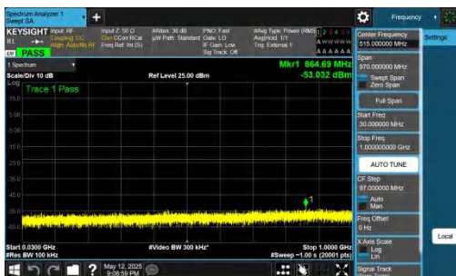
NTNV-DC_2A-n77A(3700-3980)-PC2-30-5+60-M+L-QPSK-IDLE-D FT-QPSK-Inner_1RB_Left-30-1000-PASS
