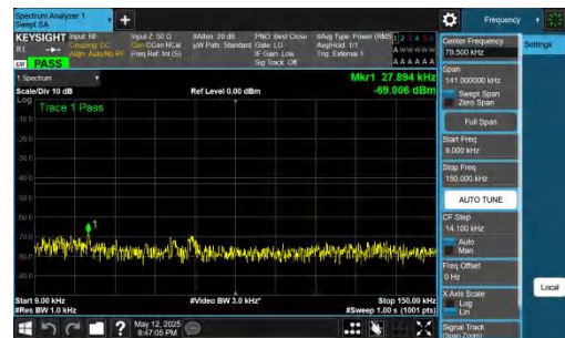
NTNV-DC_2A-n77A(3700-3980)-PC2-30-5+40-M+M-QPSK-IDLE-DFT-BPSK-Inner_1RB_Right-0.009-0.15-PASS
