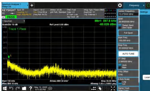
NTNV-DC_2A-n77A(3700-3980)-PC2-30-5+60-M+L-QPSK-IDLE-D FT-QPSK-Inner_1RB_Right-0.15-30-PASS
