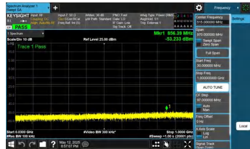
NTNV-DC_2A-n77A(3700-3980)-PC2-30-5+40-M+H-QPSK-IDLE-D FT-BPSK-Inner_1RB_Right-30-1000-PASS
