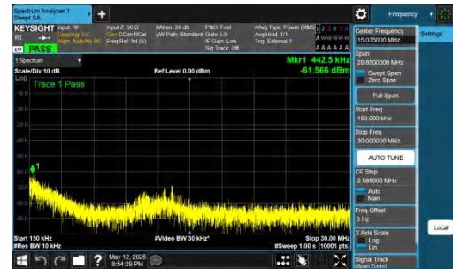
NTNV-DC_2A-n77A(3700-3980)-PC2-30-5+40-M+H-QPSK-IDLE-D FT-BPSK-Inner_1RB_Left-0.15-30-PASS
