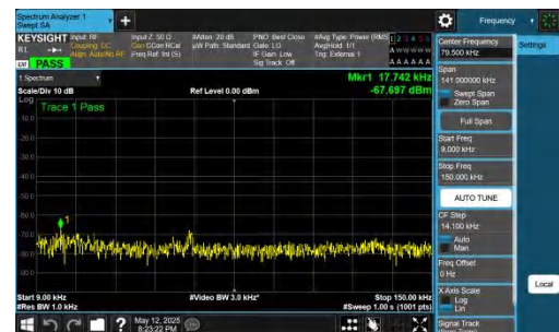
NTNV-DC_2A-n77A(3700-3980)-PC2-30-5+30-M+M-QPSK-IDLE-DFT-QPSK-Inner_1RB_Right-0.009-0.15-PASS
