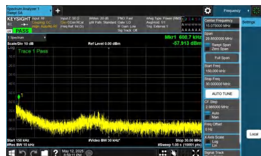
NTNV-DC_2A-n77A(3700-3980)-PC2-30-5+40-M+H-QPSK-IDLE-D FT-QPSK-Inner_1RB_Left-0.15-30-PASS
