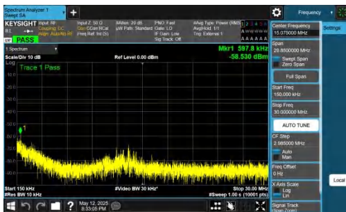
NTNV-DC_2A-n77A(3700-3980)-PC2-30-5+30-M+H-QPSK-IDLE-D FT-QPSK-Inner_1RB_Right-0.15-30-PASS
