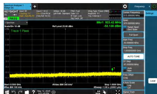
NTNV-DC_2A-n77A(3700-3980)-PC2-30-5+40-M+H-QPSK-IDLE-D FT-QPSK-Inner_1RB_Right-30-1000-PASS
