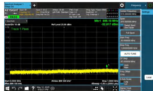
NTNV-DC_2A-n77A(3700-3980)-PC2-30-5+40-M+M-QPSK-IDLE-D FT-QPSK-Inner_1RB_Right-30-1000-PASS
