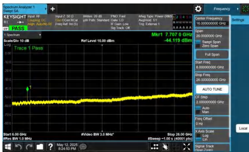
NTNV-DC_2A-n77A(3700-3980)-PC2-30-5+30-M+M-QPSK-IDLE-DFT-QPSK-Inner_1RB_Right-6000-26000-PASS
