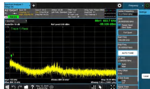
NTNV-DC_2A-n77A(3700-3980)-PC2-30-5+40-M+M-QPSK-IDLE-D FT-BPSK-Inner_1RB_Left-0.15-30-PASS
