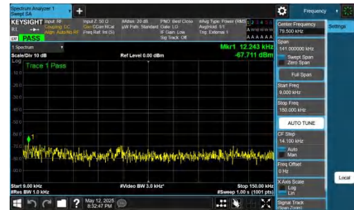
NTNV-DC_2A-n77A(3700-3980)-PC2-30-5+30-M+H-QPSK-IDLE-D FT-QPSK-Inner_1RB_Right-0.009-0.15-PASS
