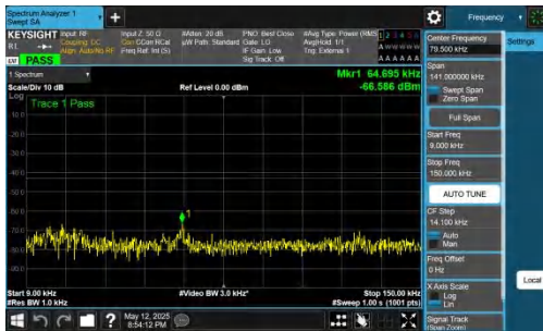
NTNV-DC_2A-n77A(3700-3980)-PC2-30-5+40-M+H-QPSK-IDLE-D FT-BPSK-Inner_1RB_Left-0.009-0.15-PASS
