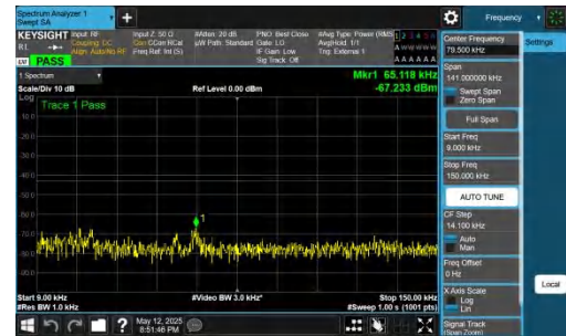
NTNV-DC_2A-n77A(3700-3980)-PC2-30-5+40-M+M-QPSK-IDLE-D FT-QPSK-Inner_1RB_Right-0.009-0.15-PASS
