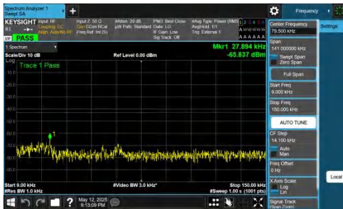
NTNV-DC_2A-n77A(3700-3980)-PC2-30-5+60-M+M-QPSK-IDLE-DFT-BPSK-Inner_1RB_Left-0.009-0.15-PASS
