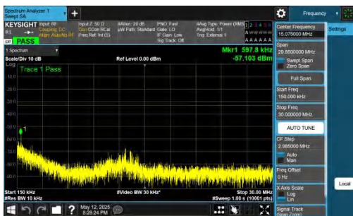
NTNV-DC_2A-n77A(3700-3980)-PC2-30-5+30-M+H-QPSK-IDLE-D FT-BPSK-Inner_1RB_Right-0.15-30-PASS
