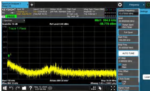
NTNV-DC_2A-n77A(3700-3980)-PC2-30-5+40-M+L-QPSK-IDLE-D FT-BPSK-Inner_1RB_Right-0.15-30-PASS
