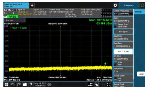
NTNV-DC_2A-n77A(3700-3980)-PC2-30-5+60-M+L-QPSK-IDLE-D FT-BPSK-Inner_1RB_Right-30-1000-PASS
