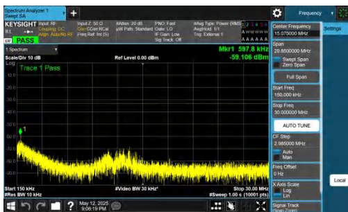
NTNV-DC_2A-n77A(3700-3980)-PC2-30-5+60-M+L-QPSK-IDLE-D FT-BPSK-Inner_1RB_Right-0.15-30-PASS
