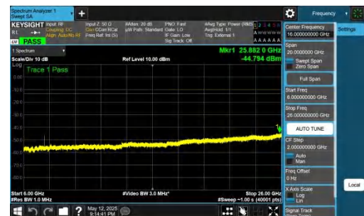
NTNV-DC_2A-n77A(3700-3980)-PC2-30-5+60-M+M-QPSK-IDLE-DFT-BPSK-Inner_1RB_Left-6000-26000-PASS
