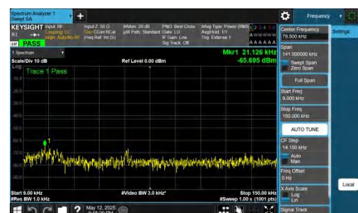
NTNV-DC_2A-n77A(3700-3980)-PC2-30-5+60-M+M-QPSK-IDLE-DFT-BPSK-Inner_1RB_Right-0.009-0.15-PASS
