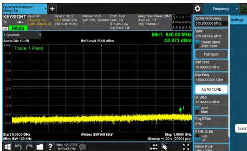
NTNV-DC_2A-n77A(3700-3980)-PC2-30-5+60-M+M-QPSK-IDLE-DFT-BPSK-Inner_1RB_Left-30-1000-PASS
