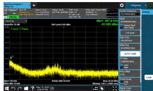
NTNV-DC_2A-n77A(3700-3980)-PC2-30-5+60-M+L-QPSK-IDLE-D FT-QPSK-Inner_1RB_Left-0.15-30-PASS
