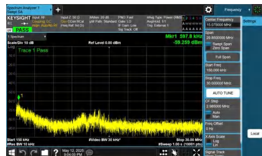
NTNV-DC_2A-n77A(3700-3980)-PC2-30-5+60-M+L-QPSK-IDLE-D FT-BPSK-Inner_1RB_Left-0.15-30-PASS
