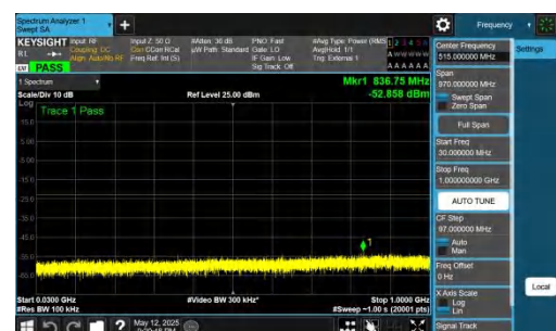
NTNV-DC_2A-n77A(3700-3980)-PC2-30-5+60-M+M-QPSK-IDLE-DFT-QPSK-Inner_1RB_Right-30-1000-PASS
