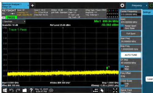
NTNV-DC_2A-n77A(3700-3980)-PC2-30-5+40-M+H-QPSK-IDLE-D FT-BPSK-Inner_1RB_Left-30-1000-PASS
