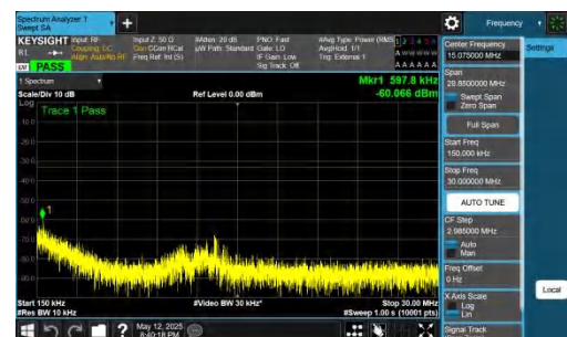
NTNV-DC_2A-n77A(3700-3980)-PC2-30-5+40-M+L-QPSK-IDLE-D FT-QPSK-Inner_1RB_Left-0.15-30-PASS
