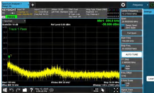
NTNV-DC_2A-n77A(3700-3980)-PC2-30-5+40-M+H-QPSK-IDLE-D FT-BPSK-Inner_1RB_Right-0.15-30-PASS
