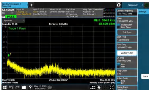
NTNV-DC_2A-n77A(3700-3980)-PC2-30-5+40-M+M-QPSK-IDLE-DFT-BPSK-Inner_1RB_Right-0.15-30-PASS
