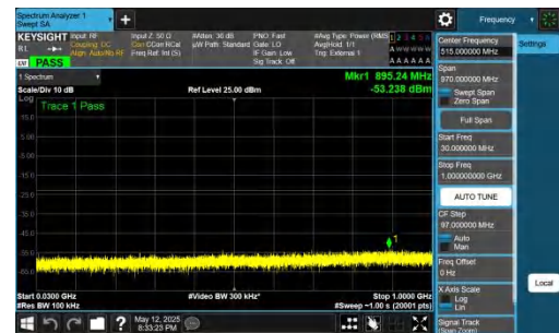
NTNV-DC_2A-n77A(3700-3980)-PC2-30-5+30-M+H-QPSK-IDLE-D FT-QPSK-Inner_1RB_Right-30-1000-PASS
