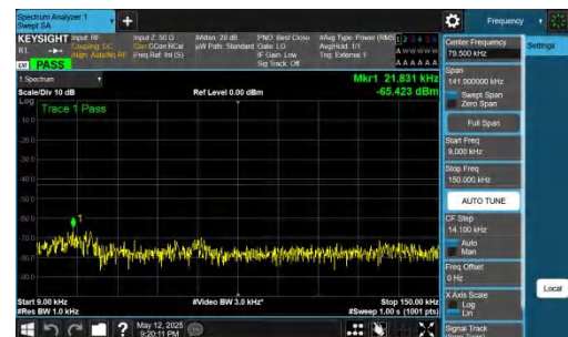
NTNV-DC_2A-n77A(3700-3980)-PC2-30-5+60-M+M-QPSK-IDLE-DFT-QPSK-Inner_1RB_Right-0.009-0.15-PASS
