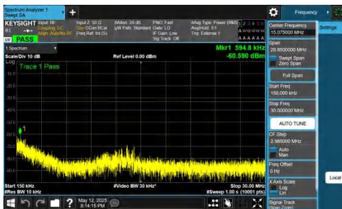
NTNV-DC_2A-n77A(3700-3980)-PC2-30-5+30-M+L-QPSK-IDLE-D FT-QPSK-Inner_1RB_Right-0.15-30-PASS
