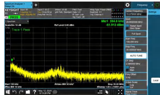
NTNV-DC_2A-n77A(3700-3980)-PC2-30-5+60-M+M-QPSK-IDLE-DFT-BPSK-Inner_1RB_Left-0.15-30-PASS
