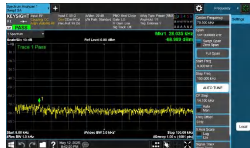
NTNV-DC_2A-n77A(3700-3980)-PC2-30-5+40-M+L-QPSK-IDLE-D FT-QPSK-Inner_1RB_Right-0.009-0.15-PASS
