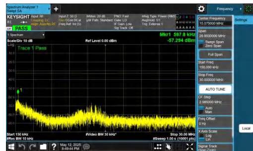
NTNV-DC_2A-n77A(3700-3980)-PC2-30-5+40-M+M-QPSK-IDLE-DFT-QPSK-Inner_1RB_Left-0.15-30-PASS
