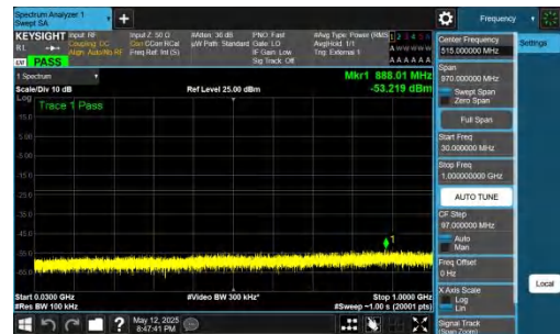
NTNV-DC_2A-n77A(3700-3980)-PC2-30-5+40-M+M-QPSK-IDLE-DFT-BPSK-Inner_1RB_Right-30-1000-PASS
