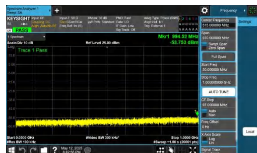
NTNV-DC_2A-n77A(3700-3980)-PC2-30-5+40-M+L-QPSK-IDLE-D FT-QPSK-Inner_1RB_Right-30-1000-PASS
