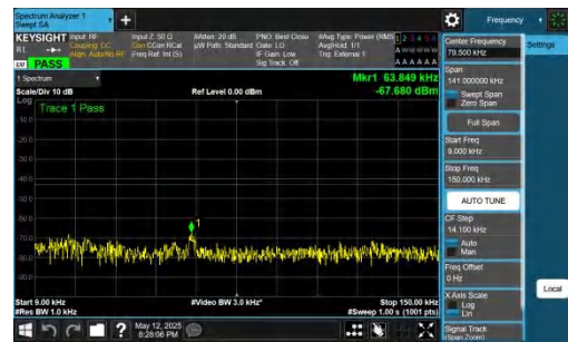
NTNV-DC_2A-n77A(3700-3980)-PC2-30-5+30-M+H-QPSK-IDLE-D FT-BPSK-Inner_1RB_Right-0.009-0.15-PASS
