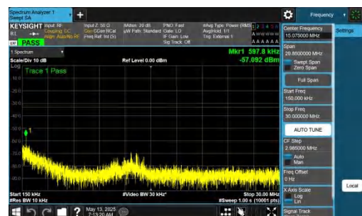
NTNV-DC_2A-n77A(3450-3550)-PC2-30-5+80-M+H-QPSK-IDLE-D FT-QPSK-Inner_1RB_Left-0.15-30-PASS
