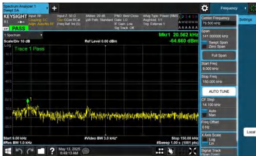
NTNV-DC_2A-n77A(3450-3550)-PC2-30-5+80-M+L-QPSK-IDLE-D FT-BPSK-Inner_1RB_Left-0.009-0.15-PASS
