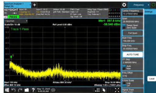
NTNV-DC_2A-n77A(3450-3550)-PC2-30-5+80-M+L-QPSK-IDLE-D FT-BPSK-Inner_1RB_Left-0.15-30-PASS
