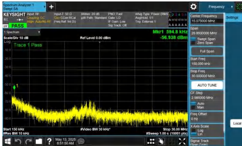
NTNV-DC_2A-n77A(3450-3550)-PC2-30-5+80-M+L-QPSK-IDLE-D FT-BPSK-Inner_1RB_Right-0.15-30-PASS
