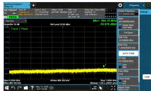
NTNV-DC_2A-n77A(3450-3550)-PC2-30-5+60-M+H-QPSK-IDLE-D FT-QPSK-Inner_1RB_Right-30-1000-PASS
