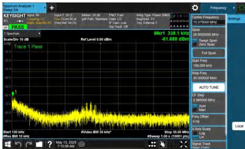
NTNV-DC_2A-n77A(3450-3550)-PC2-30-5+80-M+H-QPSK-IDLE-D FT-BPSK-Inner_1RB_Right-0.15-30-PASS
