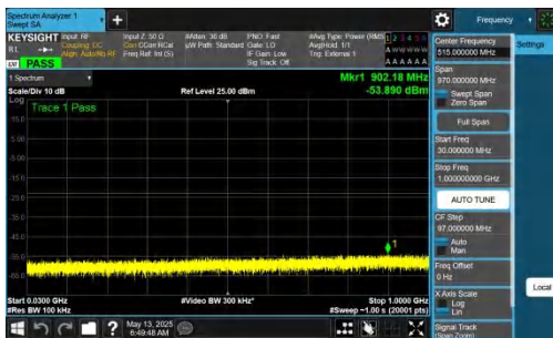
NTNV-DC_2A-n77A(3450-3550)-PC2-30-5+80-M+L-QPSK-IDLE-D FT-BPSK-Inner_1RB_Left-30-1000-PASS
