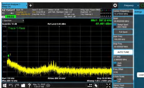
NTNV-DC_2A-n77A(3450-3550)-PC2-30-5+100-M+M-QPSK-IDLE-DFT-BPSK-Inner_1RB_Right-0.15-30-PASS
