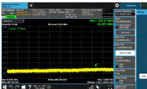
NTNV-DC_2A-n77A(3450-3550)-PC2-30-5+100-M+M-QPSK-IDLE-DFT-QPSK-Inner_1RB_Left-30-1000-PASS
