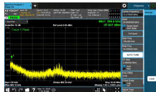
NTNV-DC_2A-n77A(3450-3550)-PC2-30-5+100-M+M-QPSK-IDLE- DFT-BPSK-Inner_1RB_Left-0.15-30-PASS
