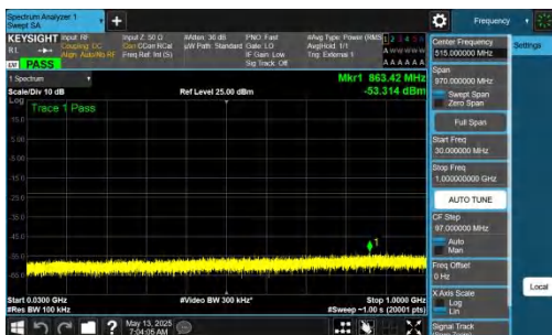
NTNV-DC_2A-n77A(3450-3550)-PC2-30-5+80-M+M-QPSK-IDLE-DFT-QPSK-Inner_1RB_Left-30-1000-PASS
