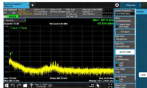
NTNV-DC_2A-n77A(3450-3550)-PC2-30-5+80-M+M-QPSK-IDLE-DFT-QPSK-Inner_1RB_Left-0.15-30-PASS
