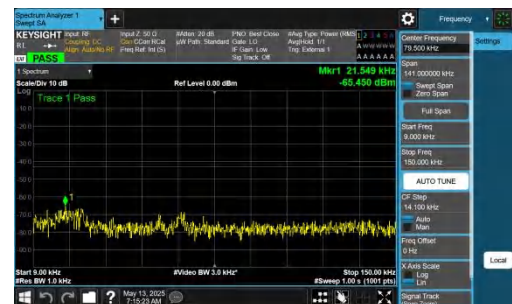
NTNV-DC_2A-n77A(3450-3550)-PC2-30-5+80-M+H-QPSK-IDLE-D FT-QPSK-Inner_1RB_Right-0.009-0.15-PASS
