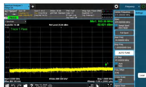
NTNV-DC_2A-n77A(3450-3550)-PC2-30-5+80-M+H-QPSK-IDLE-D FT-QPSK-Inner_1RB_Right-30-1000-PASS
