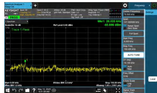
NTNV-DC_2A-n77A(3450-3550)-PC2-30-5+60-M+H-QPSK-IDLE-D FT-BPSK-Inner_1RB_Right-0.009-0.15-PASS
