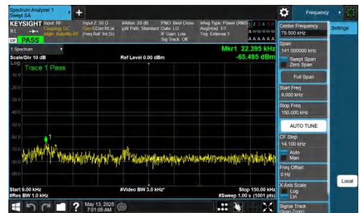
NTNV-DC_2A-n77A(3450-3550)-PC2-30-5+80-M+M-QPSK-IDLE-DFT-BPSK-Inner_1RB_Right-0.009-0.15-PASS
