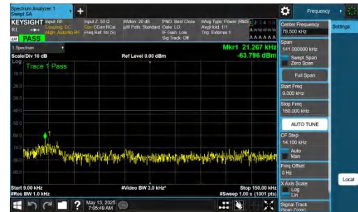
NTNV-DC_2A-n77A(3450-3550)-PC2-30-5+80-M+M-QPSK-IDLE-DFT-QPSK-Inner_1RB_Right-0.009-0.15-PASS
