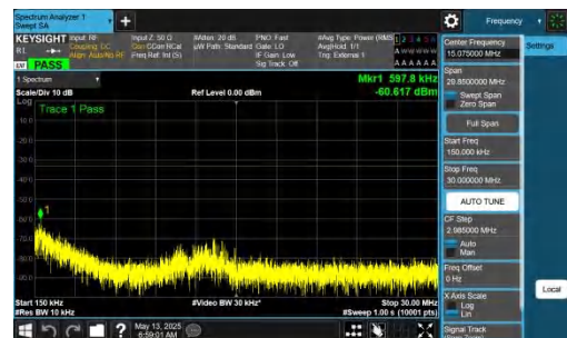
NTNV-DC_2A-n77A(3450-3550)-PC2-30-5+80-M+M-QPSK-IDLE-D FT-BPSK-Inner_1RB_Left-0.15-30-PASS
