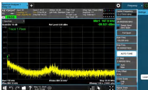
NTNV-DC_2A-n77A(3450-3550)-PC2-30-5+60-M+H-QPSK-IDLE-D FT-BPSK-Inner_1RB_Right-0.15-30-PASS
