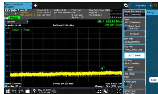
NTNV-DC_2A-n77A(3450-3550)-PC2-30-5+80-M+M-QPSK-IDLE-DFT-QPSK-Inner_1RB_Right-30-1000-PASS
