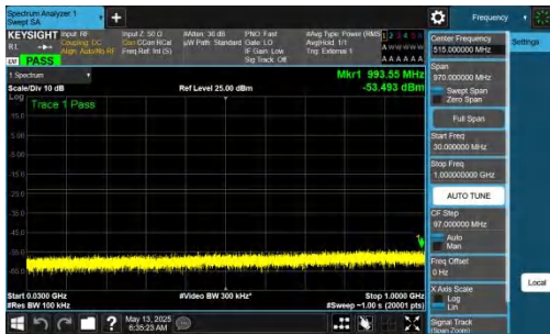
NTNV-DC_2A-n77A(3450-3550)-PC2-30-5+60-M+M-QPSK-IDLE-DFT-QPSK-Inner_1RB_Left-30-1000-PASS
