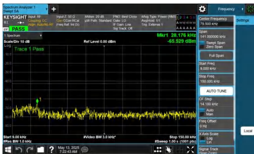
NTNV-DC_2A-n77A(3450-3550)-PC2-30-5+100-M+M-QPSK-IDLE-DFT-QPSK-Inner_1RB_Left-0.009-0.15-PASS
