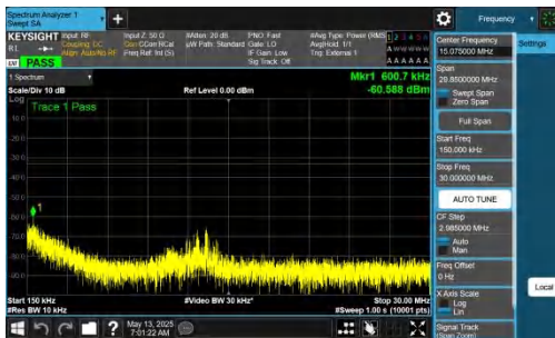
NTNV-DC_2A-n77A(3450-3550)-PC2-30-5+80-M+M-QPSK-IDLE-DFT-BPSK-Inner_1RB_Right-0.15-30-PASS
