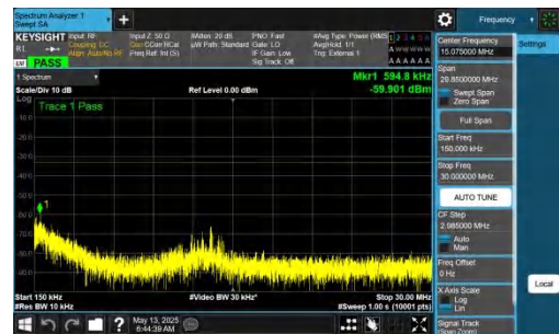
NTNV-DC_2A-n77A(3450-3550)-PC2-30-5+60-M+H-QPSK-IDLE-D FT-QPSK-Inner_1RB_Left-0.15-30-PASS
