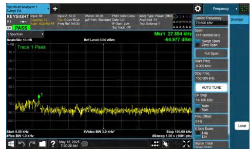
NTNV-DC_2A-n77A(3450-3550)-PC2-30-5+100-M+M-QPSK-IDLE-DFT-BPSK-Inner_1RB_Right-0.009-0.15-PASS
