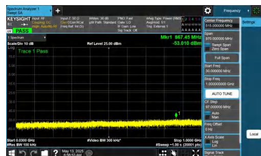
NTNV-DC_2A-n77A(3450-3550)-PC2-30-5+80-M+L-QPSK-IDLE-D FT-QPSK-Inner_1RB_Right-30-1000-PASS
