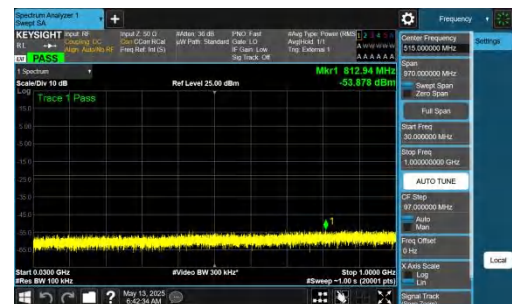
NTNV-DC_2A-n77A(3450-3550)-PC2-30-5+60-M+H-QPSK-IDLE-D FT-BPSK-Inner_1RB_Right-30-1000-PASS
