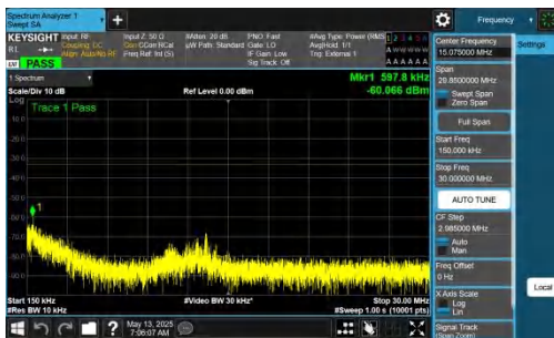
NTNV-DC_2A-n77A(3450-3550)-PC2-30-5+80-M+M-QPSK-IDLE-DFT-QPSK-Inner_1RB_Right-0.15-30-PASS
