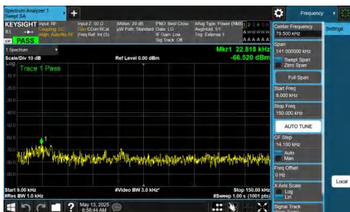
NTNV-DC_2A-n77A(3450-3550)-PC2-30-5+80-M+M-QPSK-IDLE-D DFT-BPSK-Inner_1RB_Left-0.009-0.15-PASS
