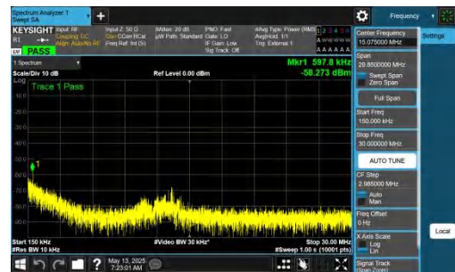
NTNV-DC_2A-n77A(3450-3550)-PC2-30-5+100-M+M-QPSK-IDLE-DFT-QPSK-Inner_1RB_Left-0.15-30-PASS
