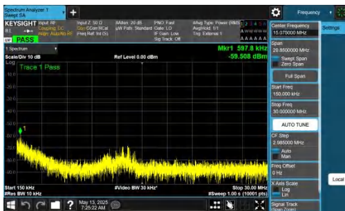
NTNV-DC_2A-n77A(3450-3550)-PC2-30-5+100-M+M-QPSK-IDLE-DFT-QPSK-Inner_1RB_Right-0.15-30-PASS
