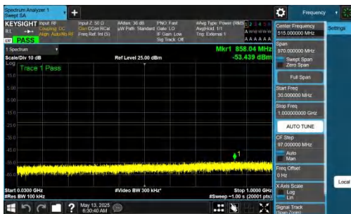
NTNV-DC_2A-n77A(3450-3550)-PC2-30-5+60-M+M-QPSK-IDLE-DFT-BPSK-Inner_1RB_Left-30-1000-PASS
