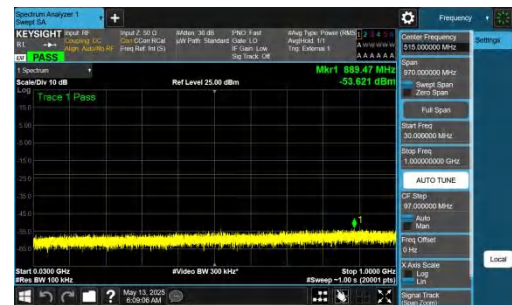
NTNV-DC_2A-n77A(3450-3550)-PC2-30-5+40-M+M-QPSK-IDLE-DFT-QPSK-Inner_1RB_Right-30-1000-PASS
