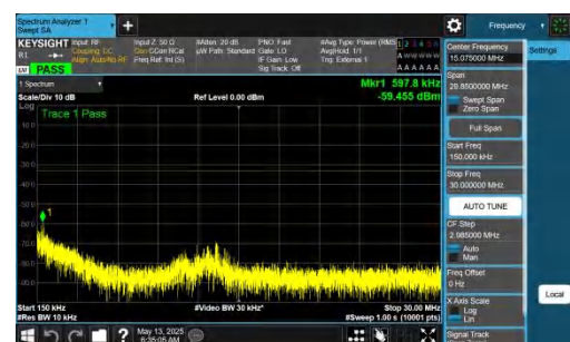
NTNV-DC_2A-n77A(3450-3550)-PC2-30-5+60-M+M-QPSK-IDLE-DFT-QPSK-Inner_1RB_Left-0.15-30-PASS
