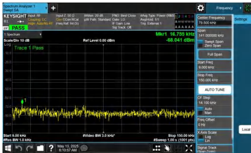
NTNV-DC_2A-n77A(3450-3550)-PC2-30-5+40-M+H-QPSK-IDLE-D FT-BPSK-Inner_1RB_Left-0.009-0.15-PASS
