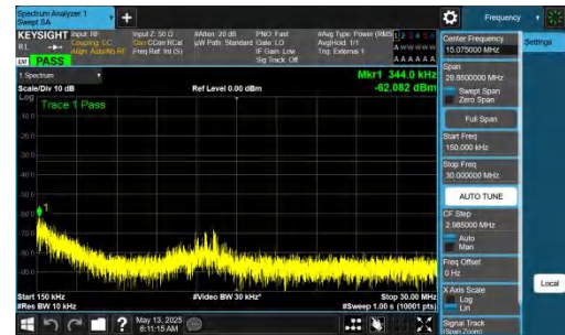
NTNV-DC_2A-n77A(3450-3550)-PC2-30-5+40-M+H-QPSK-IDLE-D FT-BPSK-Inner_1RB_Left-0.15-0.30-PASS
