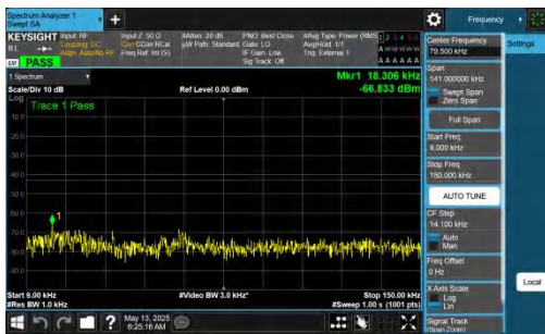
NTNV-DC_2A-n77A(3450-3550)-PC2-30-5+60-M+L-QPSK-IDLE-D FT-QPSK-Inner_1RB_Left-0.009-0.15-PASS
