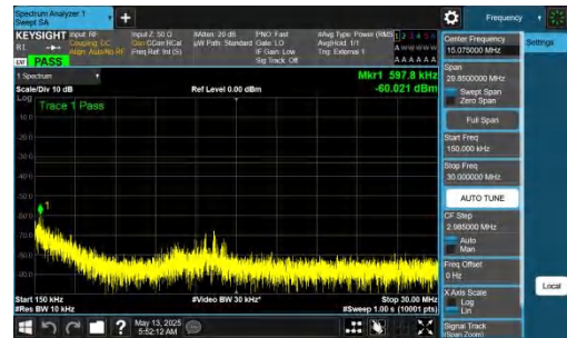
NTNV-DC_2A-n77A(3450-3550)-PC2-30-5+40-M+L-QPSK-IDLE-D FT-BPSK-Inner_1RB_Left-0.15-30-PASS
