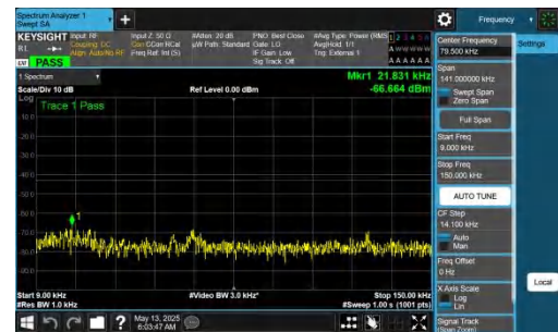
NTNV-DC_2A-n77A(3450-3550)-PC2-30-5+40-M+M-QPSK-IDLE-DFT-BPSK-Inner_1RB_Right-0.009-0.15-PASS
