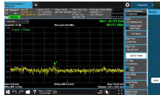
NTNV-DC_2A-n77A(3450-3550)-PC2-30-5+30-M+H-QPSK-IDLE-D FT-QPSK-Inner_1RB_Right-0.009-0.15-PASS
