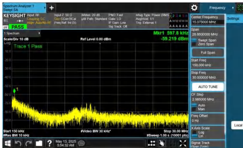
NTNV-DC_2A-n77A(3450-3550)-PC2-30-5+40-M+L-QPSK-IDLE-D FT-BPSK-Inner_1RB_Right-0.15-30-PASS
