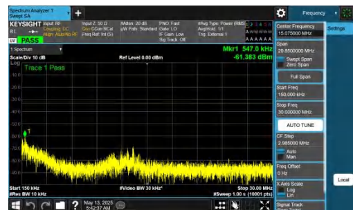
NTNV-DC_2A-n77A(3450-3550)-PC2-30-5+30-M+H-QPSK-IDLE-DFT-BPSK-Inner_1RB_Left-0.15-30-PASS
