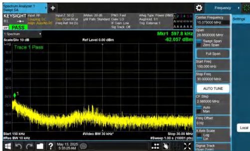
NTNV-DC_2A-n77A(3450-3550)-PC2-30-5+30-M+M-QPSK-IDLE-DFT-BPSK-Inner_1RB_Right-0.15-30-PASS
