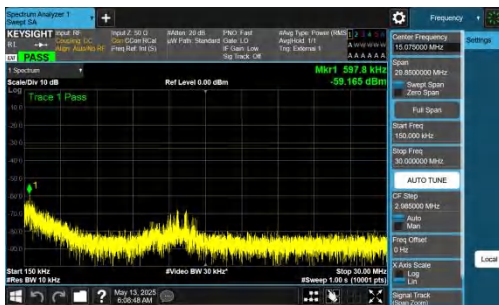
NTNV-DC_2A-n77A(3450-3550)-PC2-30-5+40-M+M-QPSK-IDLE-DFT-QPSK-Inner_1RB_Right-0.15-30-PASS
