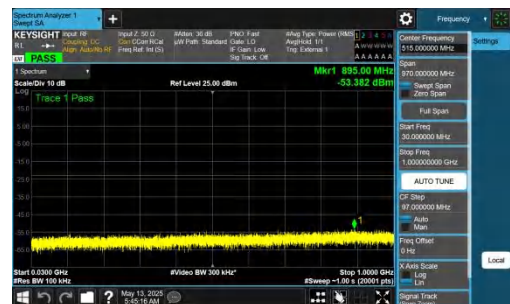
NTNV-DC_2A-n77A(3450-3550)-PC2-30-5+30-M+H-QPSK-IDLE-D FT-BPSK-Inner_1RB_Right-30-1000-PASS
