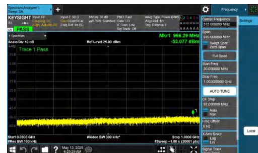
NTNV-DC_2A-n77A(3450-3550)-PC2-30-5+60-M+L-QPSK-IDLE-D FT-BPSK-Inner_1RB_Right-30-1000-PASS
