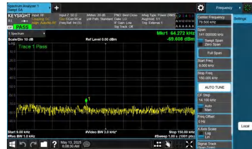
NTNV-DC_2A-n77A(3450-3550)-PC2-30-5+40-M+M-QPSK-IDLE-DFT-QPSK-Inner_1RB_Right-0.009-0.15-PASS
