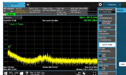
NTNV-DC_2A-n77A(3450-3550)-PC2-30-5+40-M+M-QPSK-IDLE-D FT-BPSK-Inner_1RB_Left-0.15-30-PASS
