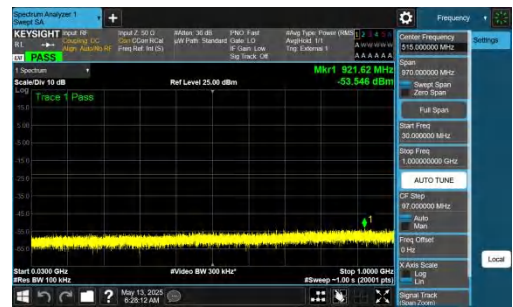
NTNV-DC_2A-n77A(3450-3550)-PC2-30-5+60-M+L-QPSK-IDLE-D FT-QPSK-Inner_1RB_Right-30-1000-PASS
