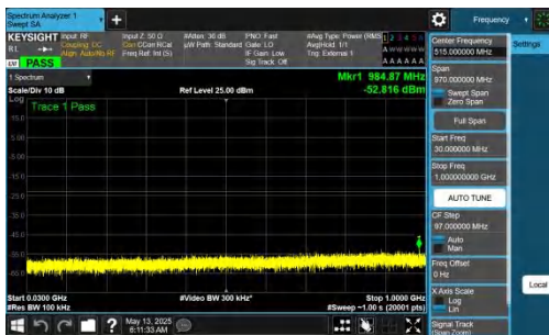
NTNV-DC_2A-n77A(3450-3550)-PC2-30-5+40-M+H-QPSK-IDLE-D FT-BPSK-Inner_1RB_Left-30-1000-PASS
