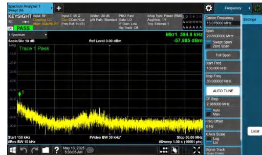
NTNV-DC_2A-n77A(3450-3550)-PC2-30-5+30-M+M-QPSK-IDLE-DFT-BPSK-Inner_1RB_Left-0.15-30-PASS
