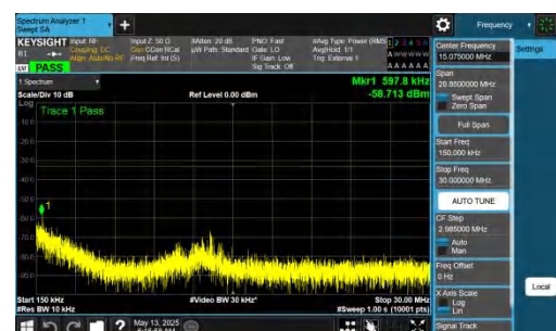
NTNV-DC_2A-n77A(3450-3550)-PC2-30-5+40-M+H-QPSK-IDLE-D FT-QPSK-Inner_1RB_Left-0.15-30-PASS
