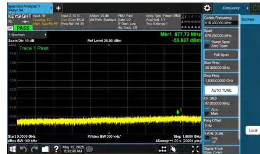
NTNV-DC_2A-n77A(3450-3550)-PC2-30-5+60-M+M-QPSK-IDLE-DFT-BPSK-Inner_1RB_Right-30-1000-PASS
