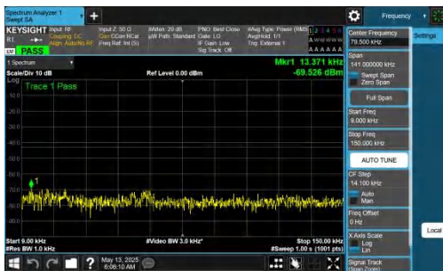
NTNV-DC_2A-n77A(3450-3550)-PC2-30-5+40-M+M-QPSK-IDLE-DFT-QPSK-Inner_1RB_Left-0.009-0.15-PASS
