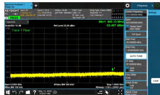
NTNV-DC_2A-n77A(3450-3550)-PC2-30-5+30-M+H-QPSK-IDLE-D FT-QPSK-Inner_1RB_Right-30-1000-PASS
