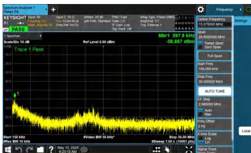
NTNV-DC_2A-n77A(3450-3550)-PC2-30-5+60-M+L-QPSK-IDLE-D FT-BPSK-Inner_1RB_Right-0.15-30-PASS
