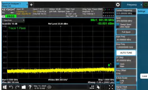
NTNV-DC_2A-n77A(3450-3550)-PC2-30-5+40-M+H-QPSK-IDLE-D FT-QPSK-Inner_1RB_Left-30-1000-PASS
