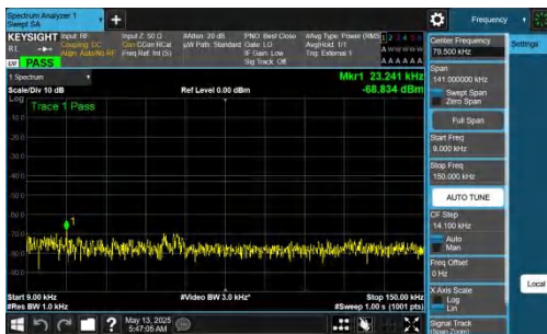
NTNV-DC_2A-n77A(3450-3550)-PC2-30-5+30-M+H-QPSK-IDLE-D FT-QPSK-Inner_1RB_Left-0.009-0.15-PASS
