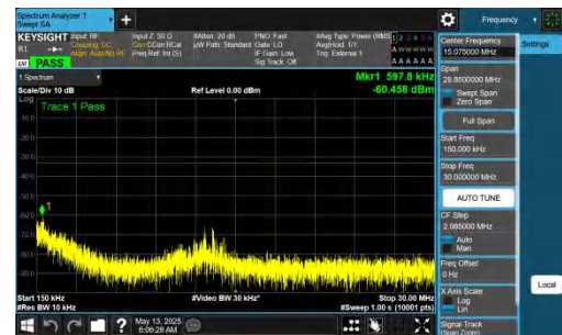
NTNV-DC_2A-n77A(3450-3550)-PC2-30-5+40-M+M-QPSK-IDLE-DFT-QPSK-Inner_1RB_Left-0.15-30-PASS
