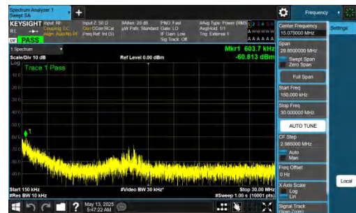
NTNV-DC_2A-n77A(3450-3550)-PC2-30-5+30-M+H-QPSK-IDLE-D FT-QPSK-Inner_1RB_Left-0.15-30-PASS
