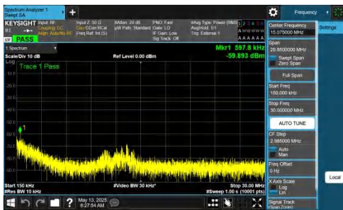
NTNV-DC_2A-n77A(3450-3550)-PC2-30-5+60-M+L-QPSK-IDLE-D FT-QPSK-Inner_1RB_Right-0.15-30-PASS
