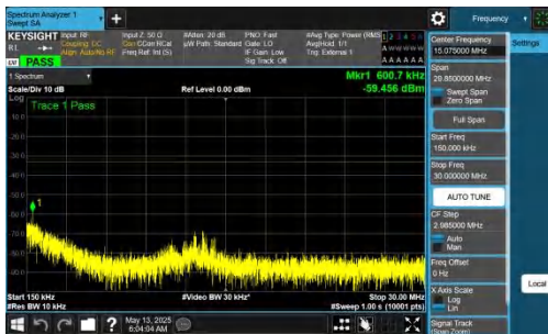
NTNV-DC_2A-n77A(3450-3550)-PC2-30-5+40-M+M-QPSK-IDLE-DFT-BPSK-Inner_1RB_Right-0.15-30-PASS
