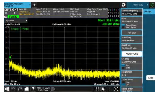
NTNV-DC_2A-n77A(3450-3550)-PC2-30-5+60-M+M-QPSK-IDLE-DFT-BPSK-Inner_1RB_Left-0.15-30-PASS
