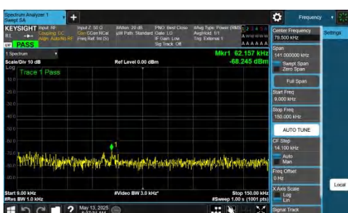
NTNV-DC_2A-n77A(3450-3550)-PC2-30-5+30-M+M-QPSK-IDLE-DFT-QPSK-Inner_1RB_Left-0.009-0.15-PASS
