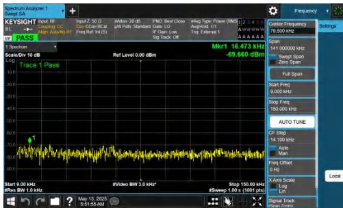
NTNV-DC_2A-n77A(3450-3550)-PC2-30-5+40-M+L-QPSK-IDLE-D FT-BPSK-Inner_1RB_Left-0.009-0.15-PASS
