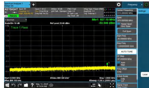
NTNV-DC_2A-n77A(3450-3550)-PC2-30-5+40-M+H-QPSK-IDLE-D FT-BPSK-Inner_1RB_Right-30-1000-PASS
