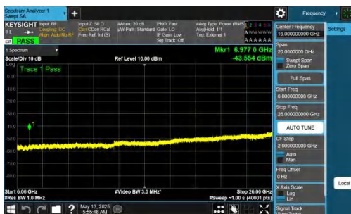
NTNV-DC_2A-n77A(3450-3550)-PC2-30-5+40-M+L-QPSK-IDLE-D FT-BPSK-Inner_1RB_Right-6000-26000-PASS
