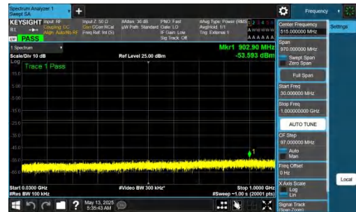
NTNV-DC_2A-n77A(3450-3550)-PC2-30-5+30-M+M-QPSK-IDLE-DFT-BPSK-Inner_1RB_Right-30-1000-PASS
