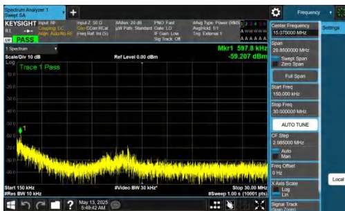
NTNV-DC_2A-n77A(3450-3550)-PC2-30-5+30-M+H-QPSK-IDLE-D FT-QPSK-Inner_1RB_Right-0.15-30-PASS
