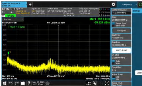
NTNV-DC_2A-n77A(3450-3550)-PC2-30-5+40-M+H-QPSK-IDLE-D FT-BPSK-Inner_1RB_Right-0.15-30-PASS
