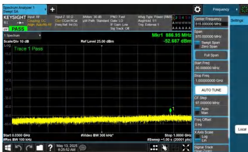
NTNV-DC_2A-n77A(3450-3550)-PC2-30-5+60-M+L-QPSK-IDLE-D FT-QPSK-Inner_1RB_Left-30-1000-PASS
