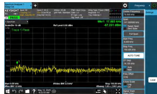
NTNV-DC_2A-n77A(3450-3550)-PC2-30-5+60-M+L-QPSK-IDLE-D FT-BPSK-Inner_1RB_Right-0.009-0.15-PASS
