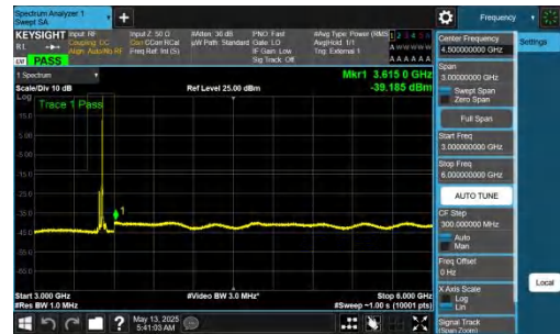
NTNV-DC_2A-n77A(3450-3550)-PC2-30-5+30-M+M-QPSK-IDLE-DFT-QPSK-Inner_1RB_Right-3000-6000-PASS
