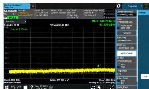
NTNV-DC_2A-n77A(3450-3550)-PC2-30-5+40-M+L-QPSK-IDLE-D FT-QPSK-Inner_1RB_Right-30-1000-PASS
