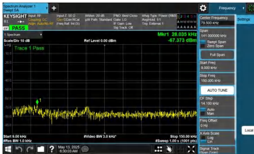
NTNV-DC_2A-n77A(3450-3550)-PC2-30-5+60-M+M-QPSK-IDLE-DFT-BPSK-Inner_1RB_Left-0.009-0.15-PASS
