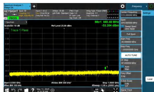
NTNV-DC_2A-n77A(3450-3550)-PC2-30-5+40-M+H-QPSK-IDLE-D FT-QPSK-Inner_1RB_Right-30-1000-PASS
