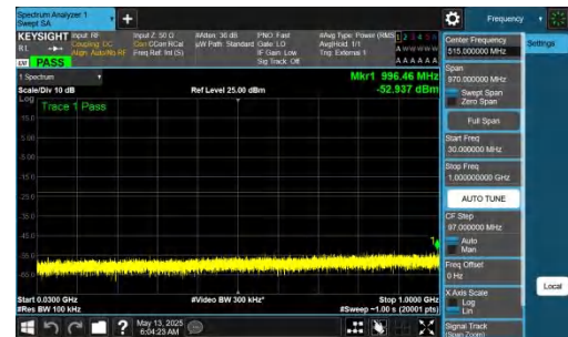
NTNV-DC_2A-n77A(3450-3550)-PC2-30-5+40-M+M-QPSK-IDLE-DFT-BPSK-Inner_1RB_Right-30-1000-PASS
