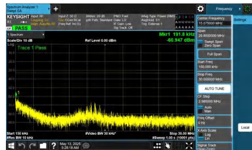
NTNV-DC_2A-n77A(3450-3550)-PC2-30-5+30-M+L-QPSK-IDLE-D FT-QPSK-Inner_1RB_Left-0.15-30-PASS
