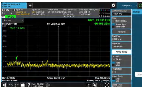
NTNV-DC_2A-n77A(3450-3550)-PC2-30-5+60-M+L-QPSK-IDLE-D FT-BPSK-Inner_1RB_Left-0.009-0.15-PASS
