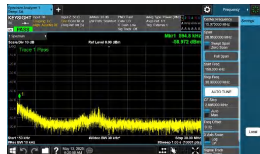
NTNV-DC_2A-n77A(3450-3550)-PC2-30-5+60-M+L-QPSK-IDLE-D FT-BPSK-Inner_1RB_Left-0.15-30-PASS
