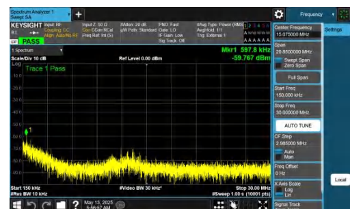
NTNV-DC_2A-n77A(3450-3550)-PC2-30-5+40-M+L-QPSK-IDLE-D FT-QPSK-Inner_1RB_Left-0.15-30-PASS
