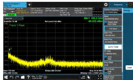
NTNV-DC_2A-n77A(3450-3550)-PC2-30-5+60-M+L-QPSK-IDLE-D FT-QPSK-Inner_1RB_Left-0.15-30-PASS
