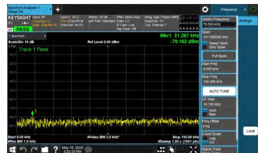
NTNV-DC_2A-n48A-PC3-30-5+40-M+H-QPSK-IDLE-DFT-QPSK-In ner_1RB_Right-0.009-0.15-PASS
