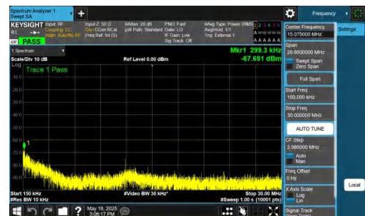
NTNV-DC_2A-n48A-PC3-30-5+40-M+M-QPSK-IDLE-DFT-BPSK-In ner_1RB_Left-0.15-30-PASS
