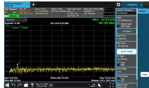
NTNV-DC_2A-n48A-PC3-30-5+20-M+H-QPSK-IDLE-DFT-QPSK-In ner_1RB_Right-0.009-0.15-PASS
