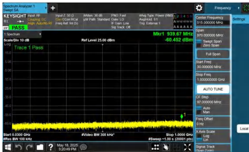
NTNV-DC_2A-n48A-PC3-30-5+40-M+H-QPSK-IDLE-DFT-QPSK-In ner_1RB_Left-30-1000-PASS
