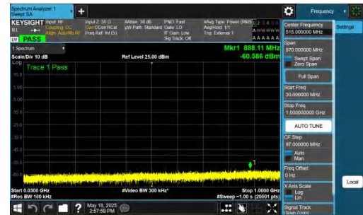
NTNV-DC_2A-n48A-PC3-30-5+40-M+L-QPSK-IDLE-DFT-BPSK-Inner_1RB_Right-30-1000-PASS
