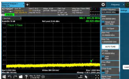
NTNV-DC_2A-n48A-PC3-30-5+40-M+H-QPSK-IDLE-DFT-BPSK-In ner_1RB_Left-30-1000-PASS
