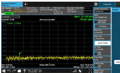
NTNV-DC_2A-n48A-PC3-30-5+40-M+M-QPSK-IDLE-DFT-QPSK-I nner_1RB_Left-0.009-0.15-PASS
