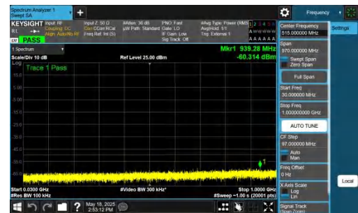
NTNV-DC_2A-n48A-PC3-30-5+20-M+H-QPSK-IDLE-DFT-QPSK-In ner_1RB_Right-30-1000-PASS
