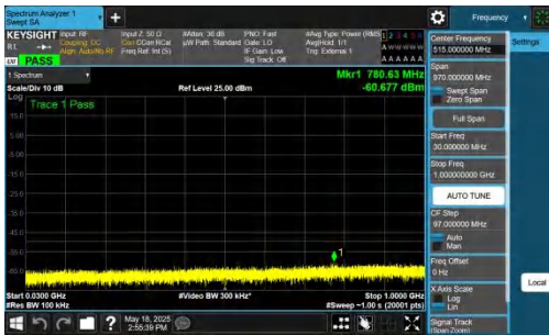
NTNV-DC_2A-n48A-PC3-30-5+40-M+L-QPSK-IDLE-DFT-BPSK-Inner_1RB_Left-30-1000-PASS
