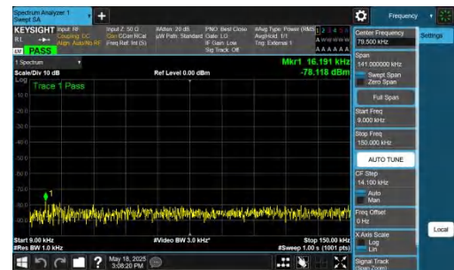
NTNV-DC_2A-n48A-PC3-30-5+40-M+M-QPSK-IDLE-DFT-BPSK-In ner_1RB_Right-0.009-0.15-PASS
