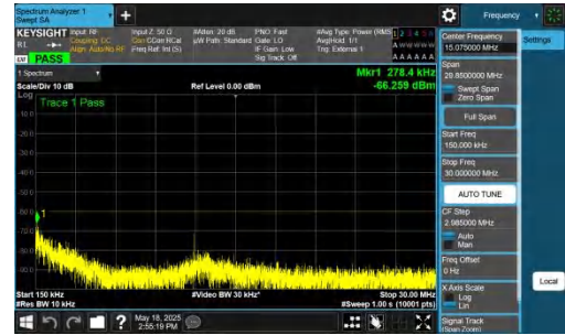
NTNV-DC_2A-n48A-PC3-30-5+40-M+L-QPSK-IDLE-DFT-BPSK-Inner_1RB_Left-0.15-30-PASS
