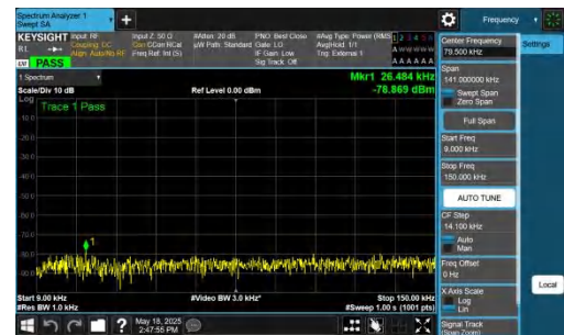
NTNV-DC_2A-n48A-PC3-30-5+20-M+H-QPSK-IDLE-DFT-BPSK-Inner_1RB_Right-0.009-0.15-PASS
