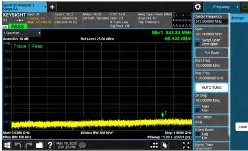
NTNV-DC_2A-n48A-PC3-30-5+20-M+M-QPSK-IDLE-DFT-QPSK-Inner_1RB_Left-30-1000-PASS
