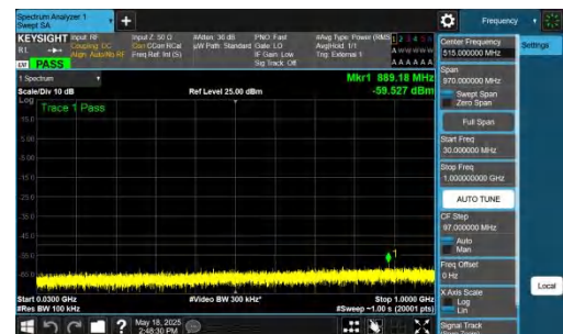
NTNV-DC_2A-n48A-PC3-30-5+20-M+H-QPSK-IDLE-DFT-BPSK-Inner_1RB_Right-30-1000-PASS
