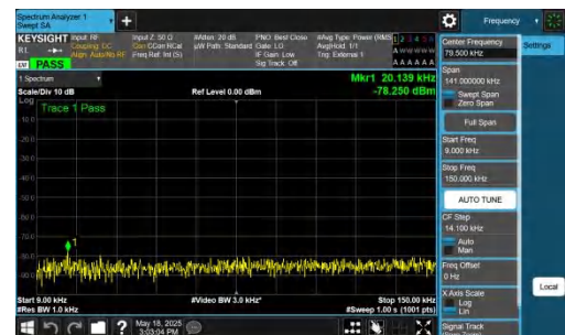
NTNV-DC_2A-n48A-PC3-30-5+40-M+L-QPSK-IDLE-DFT-QPSK-Inner_1RB_Right-0.009-0.15-PASS
