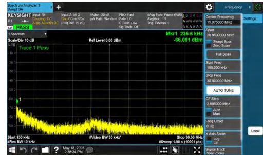
NTNV-DC_2A-n48A-PC3-30-5+20-M+M-QPSK-IDLE-DFT-BPSK-In ner_1RB_Left-0.15-30-PASS
