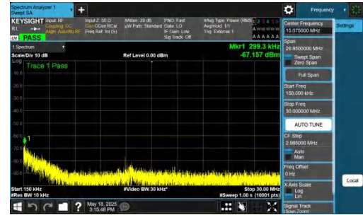
NTNV-DC_2A-n48A-PC3-30-5+40-M+H-QPSK-IDLE-DFT-BPSK-Inn er_1RB_Left-0.15-30-PASS
