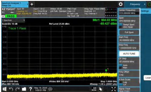
NTNV-DC_2A-n48A-PC3-30-5+40-M+L-QPSK-IDLE-DFT-QPSK-Inner_1RB_Left-30-1000-PASS
