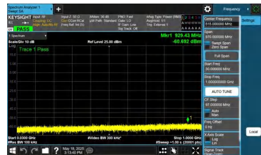
NTNV-DC_2A-n48A-PC3-30-5+40-M+M-QPSK-IDLE-DFT-QPSK-Inner_1RB_Right-30-1000-PASS
