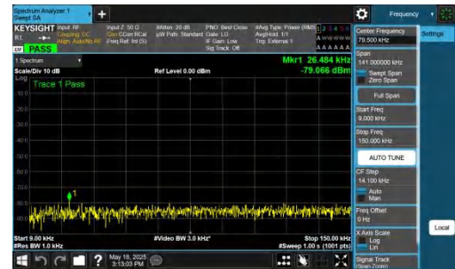
NTNV-DC_2A-n48A-PC3-30-5+40-M+M-QPSK-IDLE-DFT-QPSK-Inner_1RB_Right-0.009-0.15-PASS
