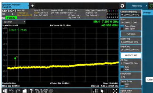
NTNV-DC_2A-n48A-PC3-30-5+40-M+H-QPSK-IDLE-DFT-BPSK-In ner_1RB_Right-6000-26000-PASS
