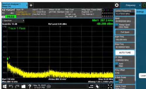
NTNV-DC_2A-n48A-PC3-30-5+40-M+M-QPSK-IDLE-DFT-QPSK-Inner_1RB_Right-0.15-30-PASS
