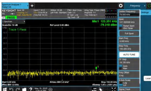
NTNV-DC_2A-n48A-PC3-30-5+20-M+H-QPSK-IDLE-DFT-BPSK-Inner_1RB_Left-0.009-0.15-PASS
