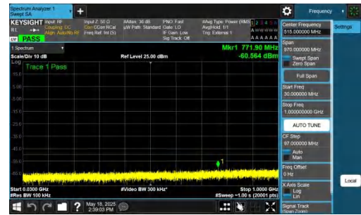
NTNV-DC_2A-n48A-PC3-30-5+20-M+M-QPSK-IDLE-DFT-BPSK-In ner_1RB_Right-30-1000-PASS
