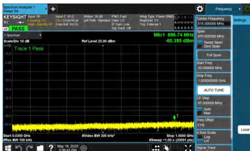
NTNV-DC_2A-n48A-PC3-30-5+20-M+M-QPSK-IDLE-DFT-BPSK-In ner_1RB_Left-30-1000-PASS
