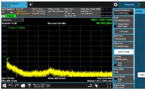
NTNV-DC_2A-n48A-PC3-30-5+20-M+M-QPSK-IDLE-DFT-BPSK-In ner_1RB_Right-0.15-30-PASS
