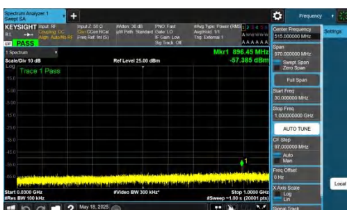
NTNV-DC_2A-n48A-PC3-30-5+20-M+H-QPSK-IDLE-DFT-BPSK-Inner_1RB_Left-30-1000-PASS
