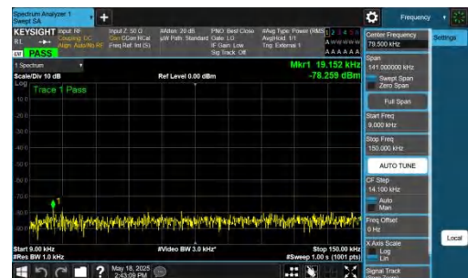
NTNV-DC_2A-n48A-PC3-30-5+20-M+M-QPSK-IDLE-DFT-QPSK-Inner_1RB_Right-0.009-0.15-PASS
