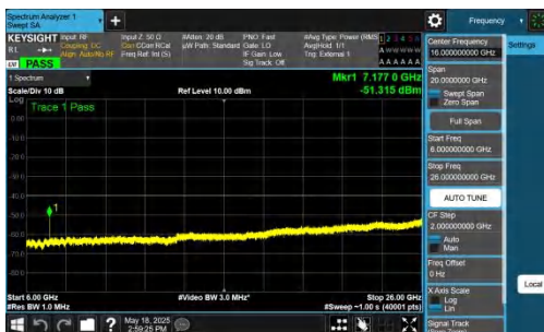
NTNV-DC_2A-n48A-PC3-30-5+40-M+L-QPSK-IDLE-DFT-BPSK-Inner_1RB_Right-6000-26000-PASS
