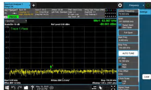
NTNV-DC_2A-n48A-PC3-30-5+40-M+L-QPSK-IDLE-DFT-BPSK-Inner_1RB_Right-0.009-0.15-PASS
