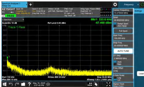
NTNV-DC_2A-n48A-PC3-30-5+40-M+L-QPSK-IDLE-DFT-BPSK-Inner_1RB_Right-0.15-30-PASS
