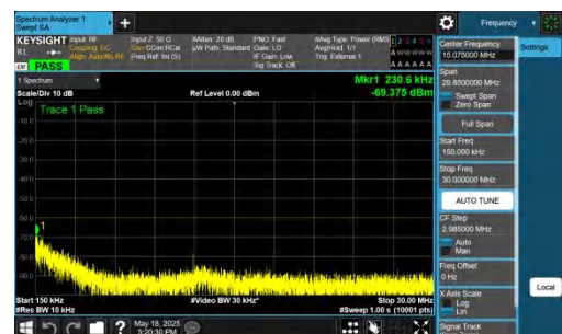
NTNV-DC_2A-n48A-PC3-30-5+40-M+H-QPSK-IDLE-DFT-QPSK-In ner_1RB_Left-0.15-30-PASS
