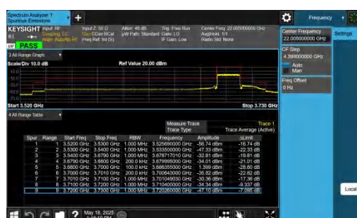
NTNV-DC_2A-n48A-PC3-30-5+20-M+H-QPSK-IDLE-DFT-QPSK-O uter Full-PASS
