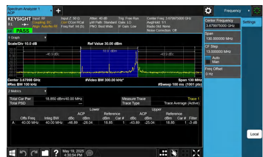
NTNV-DC_2A-n48A-PC3-30-5+40-M+H-QPSK-IDLE-CP-QPSK-Edge_1RB_Right-PASS
