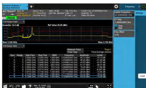
NTNV-DC_2A-n48A-PC3-30-5+20-M+L-QPSK-IDLE-DFT-QPSK-Ed ge 1RB Right-PASS
