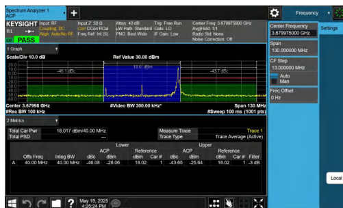
NTNV-DC_2A-n48A-PC3-30-5+40-M+H-QPSK-IDLE-DFT-16QAM-Edge_1RB_Right-PASS
