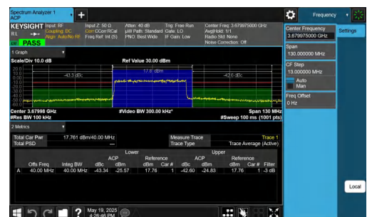
NTNV-DC_2A-n48A-PC3-30-5+40-M+H-QPSK-IDLE-DFT-16QAM-Outer_Full-PASS
