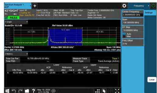
NTN-DC_2A-n48A-PC3-30-5+40-M+L-QPSK-IDLE-CP-16QAM-Edge_1RB_Left-PASS
