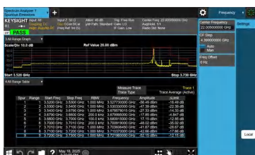
NTNV-DC_2A-n48A-PC3-30-5+20-M+H-QPSK-IDLE-DFT-BPSK-Ed ge 1RB Left-PASS
