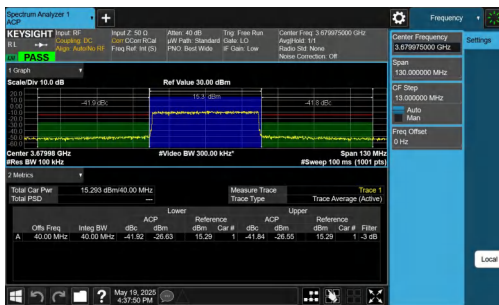
NTNV-DC_2A-n48A-PC3-30-5+40-M+H-QPSK-IDLE-CP-256QAM- Outer_Full-PASS
