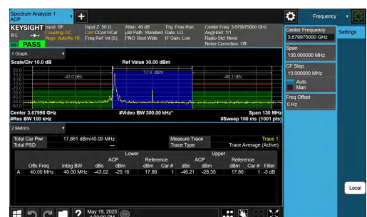
NTNV-DC_2A-n48A-PC3-30-5+40-M+H-QPSK-IDLE-DFT-256QAM-Edge_1RB_Left-PASS
