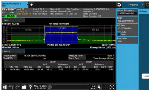
NTN-DC_2A-n48A-PC3-30-5+40-M+H-QPSK-IDLE-CP-QPSK-Outer_Full-PASS
