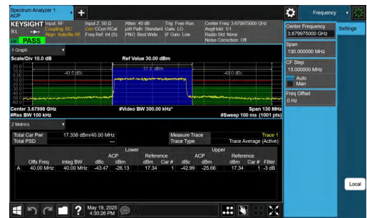
NTNV-DC_2A-n48A-PC3-30-5+40-M+H-QPSK-IDLE-DFT-256QAM -Outer_Full-PASS
