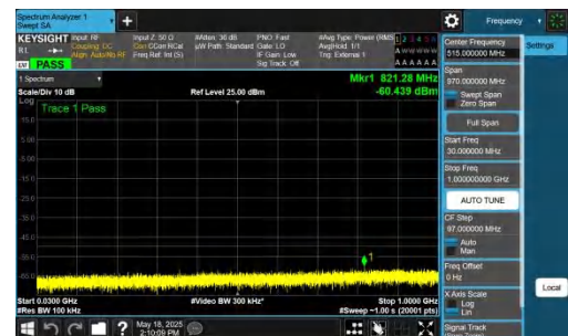
NTNV-DC_2A-n48A-PC3-30-5+10-M+M-QPSK-IDLE-DFT-BPSK-In ner_1RB_Right-30-1000-PASS
