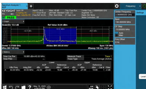
NTNV-DC_2A-n48A-PC3-30-5+40-M+L-QPSK-IDLE-CP-QPSK-Edge_1RB_Left-PASS
