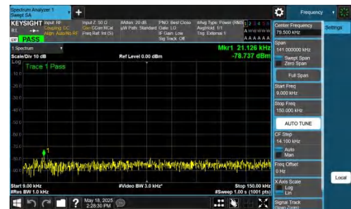
NTNV-DC_2A-n48A-PC3-30-5+20-M+L-QPSK-IDLE-DFT-BPSK-Inner_1RB_Right-0.009-0.15-PASS
