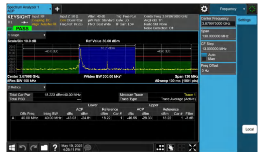
NTNV-DC_2A-n48A-PC3-30-5+40-M+H-QPSK-IDLE-DFT-16QAM-Edge_1RB_Left-PASS
