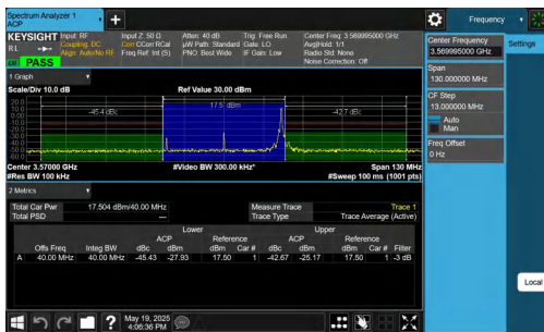
NTNV-DC_2A-n48A-PC3-30-5+40-M+L-QPSK-IDLE-DFT-256QAM-Edge_1RB_Right-PASS
