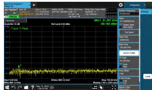
NTNV-DC_2A-n48A-PC3-30-5+10-M+L-QPSK-IDLE-DFT-QPSK-Inner_1RB_Right-0.009-0.15-PASS
