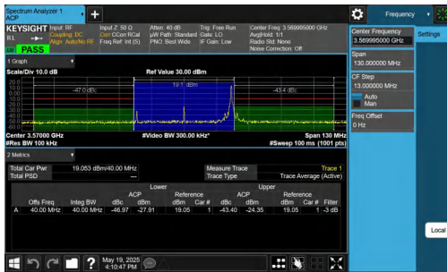
NTN-DC_2A-n48A-PC3-30-5+40-M+L-QPSK-IDLE-CP-QPSK-Edge_1RB_Right-PASS
