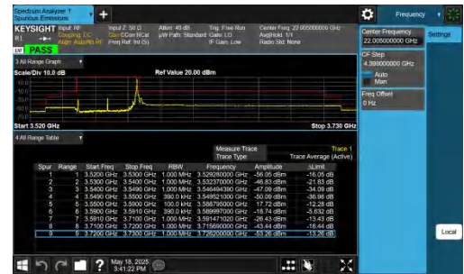
NTNV-DC_2A-n48A-PC3-30-5+40-M+L-QPSK-IDLE-DFT-BPSK-Edge_1RB_Right-PASS
