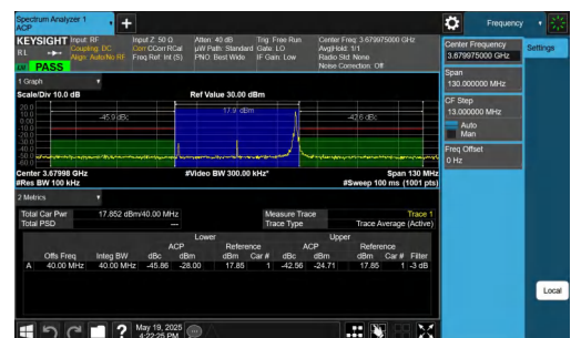
NTNV-DC_2A-n48A-PC3-30-5+40-M+H-QPSK-IDLE-DFT-QPSK-E dge_1RB_Right-PASS
