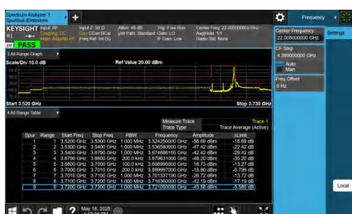
NTNV-DC_2A-n48A-PC3-30-5+20-M+H-QPSK-IDLE-DFT-QPSK-E dae 1RB Right-PASS
