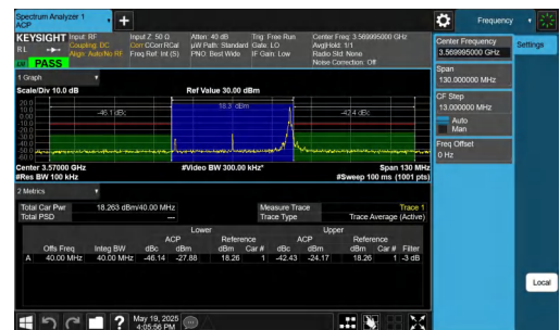
NTNV-DC_2A-n48A-PC3-30-5+40-M+L-QPSK-IDLE-DFT-64QAM-Edge_1RB_Right-PASS
