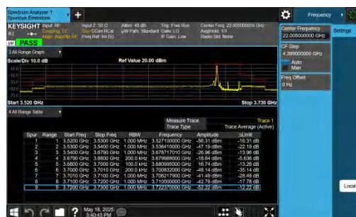
NTNV-DC_2A-n48A-PC3-30-5+20-M+H-QPSK-IDLE-DFT-QPSK-E dqe 1RB Left-PASS
