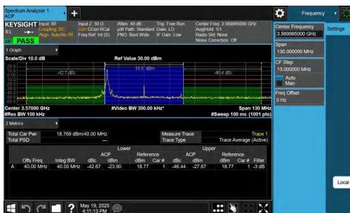
NTN-DC_2A-n48A-PC3-30-5+40-M+L-QPSK-IDLE-CP-16QAM-Edge_1RB_Left-PASS
