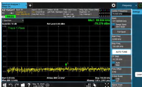
NTNV-DC_2A-n48A-PC3-30-5+20-M+L-QPSK-IDLE-DFT-BPSK-In ner_1RB_Left-0.009-0.15-PASS
