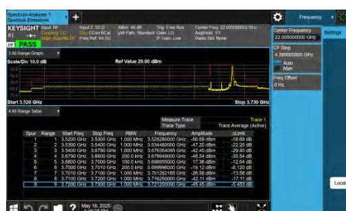
NTNV-DC_2A-n48A-PC3-30-5+20-M+H-QPSK-IDLE-DFT-BPSK-E dqe 1RB Right-PASS
