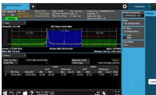
NTNV-DC_2A-n48A-PC3-30-5+40-M+L-QPSK-IDLE-DFT-QPSK-Edge_1RB_Left-PASS
