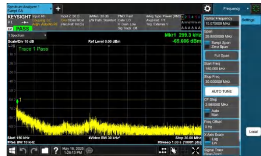
NTNV-DC_2A-n48A-PC3-30-5+10-M+L-QPSK-IDLE-DFT-BPSK-Inner_1RB_Left-0.15-30-PASS
